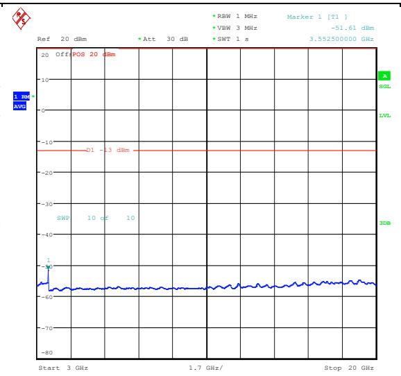
Band66_1.4MHz_16QAM_132665_1RB#0_3000~20000_3000~20000
