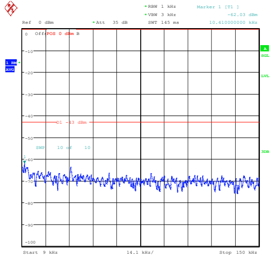
Band66_1.4MHz_16QAM_132322_6RB#0_0.009~ 0.15_0.009~0.15
