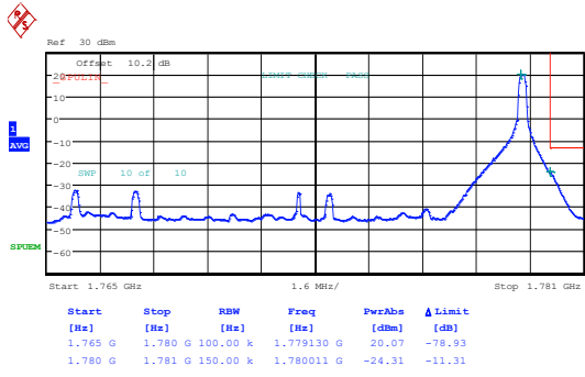
Band66_15MHz_QPSK_132597_1RB#0
