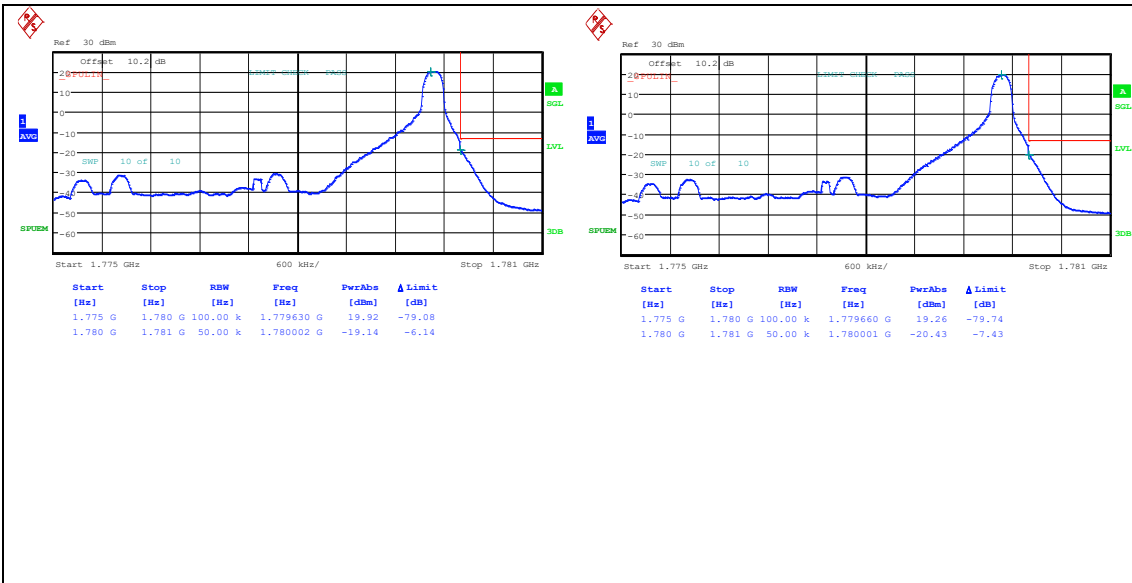
Band66_5MHz_QPSK_132647_1RB#24 Band66_5MHz_16QAM_132647_1RB#24
