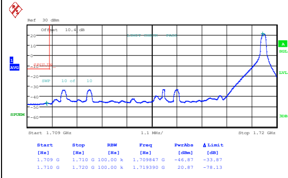
Band66_10MHz_QPSK_132022_1RB#0
