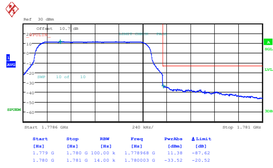
Band66_1.4MHz_16QAM_132665_1RB#5
