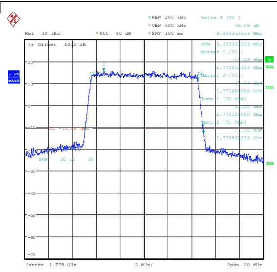
Band66-10MHz-16QAM-132622-50RB#0-PASS
