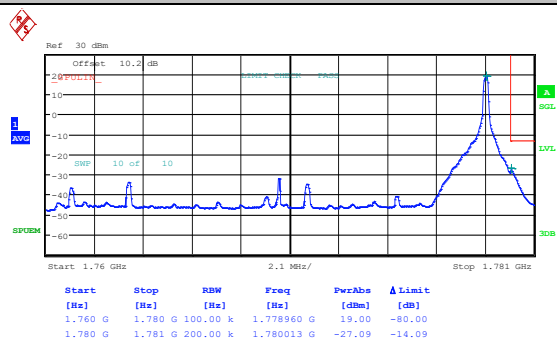
Band66_20MHz_16QAM_132572_1RB#0
