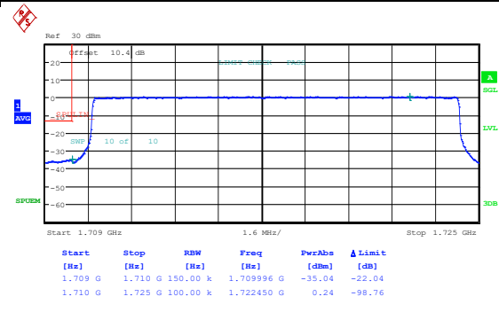
Band66_15MHz_16QAM_132047_1RB#74
