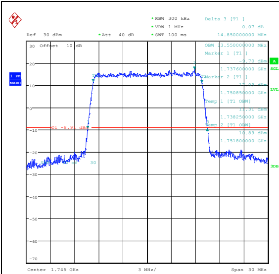
Band66-15MHz-QPSK-132322-75RB#0-PASS
