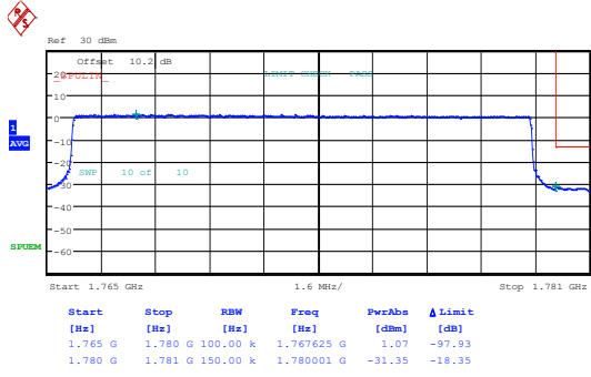
Band66_15MHz_QPSK_132597_1RB#74
