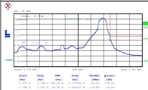
Band66_3MHz_QPSK_132657_1RB#0
