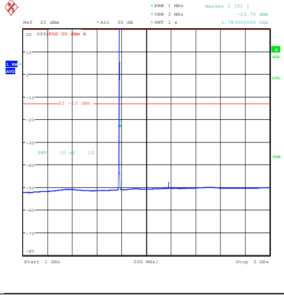
Band66_1.4MHz_QPSK_132665_6RB#0_1000~3000_000_1000~3000
