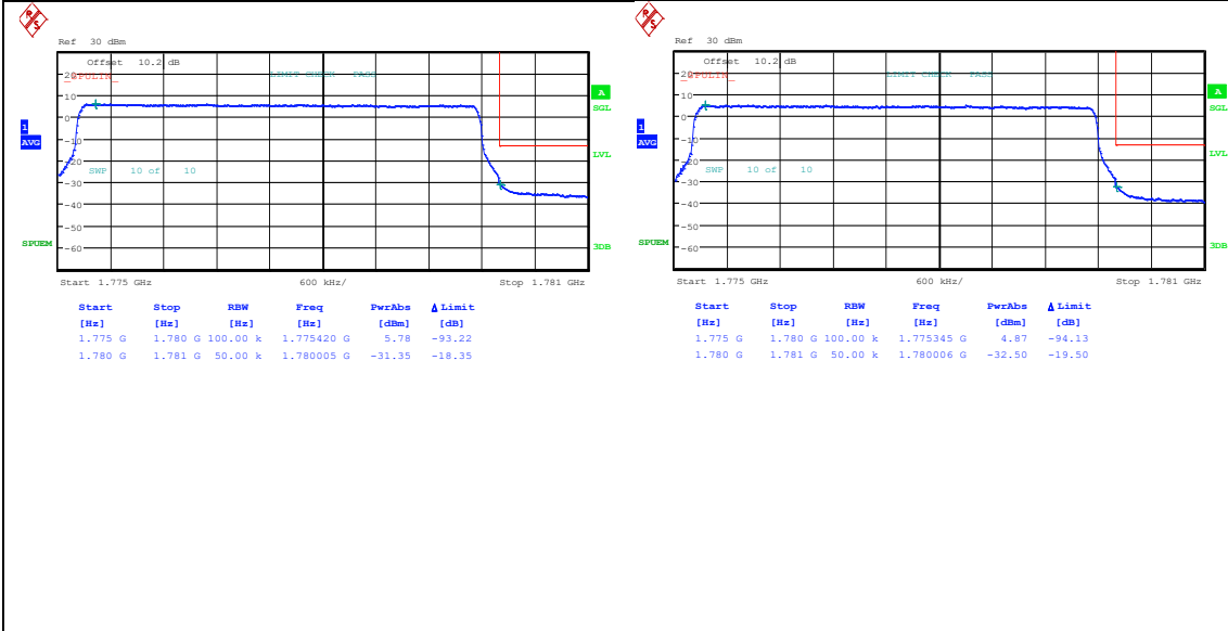
Band66_5MHz_QPSK_132647_25RB#0 Band66_5MHz_16QAM_132647_25RB#0
