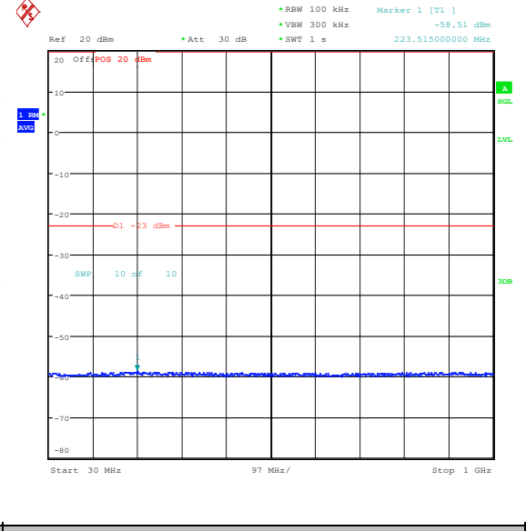
Band66_1.4MHz_16QAM_132665_1RB#0_30~1000_30~1000
