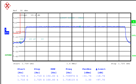
Band66_15MHz_QPSK_132047_1RB#74
