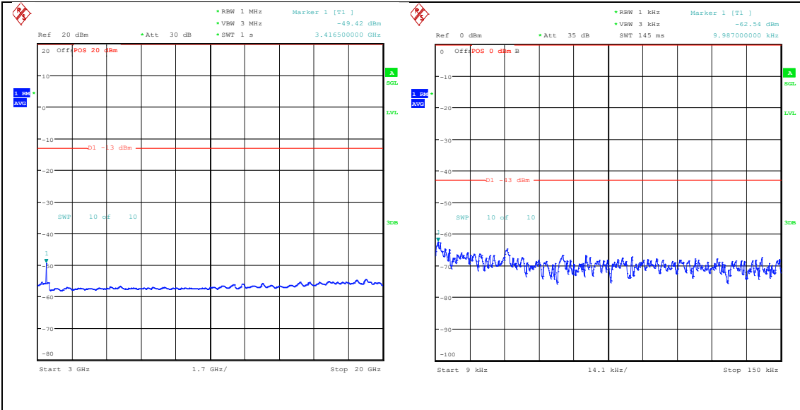
Band66_1.4MHz_QPSK_131979_1RB#0_3000~20000_3000~20000
