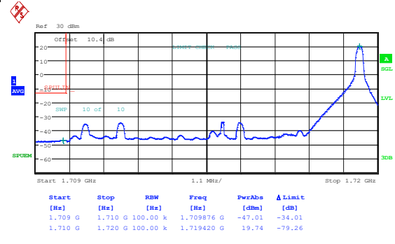
Band66_10MHz_16QAM_132022_1RB#0
