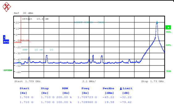
Band66_20MHz_16QAM_132072_1RB#0
