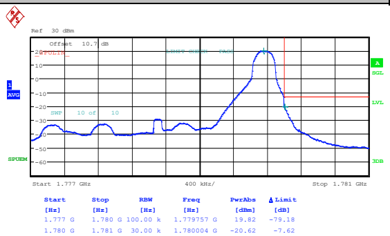
Band66_3MHz_16QAM_132657_1RB#0
