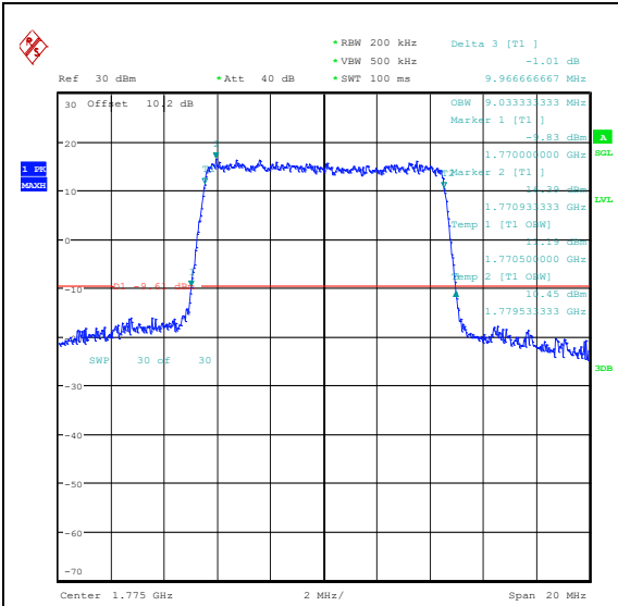
Band66-10MHz-QPSK-132622-50RB#0-PASS
