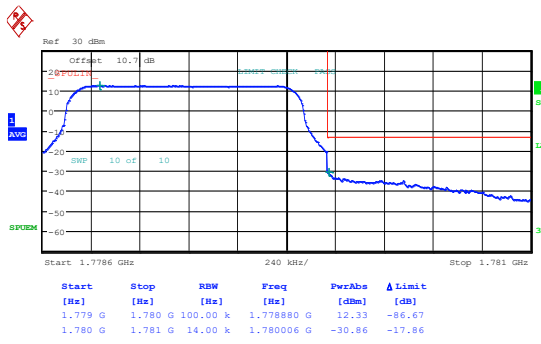
Band66_1.4MHz_QPSK_132665_1RB#5
