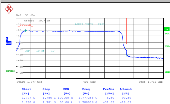
Band66_3MHz_QPSK_132657_1RB#14
