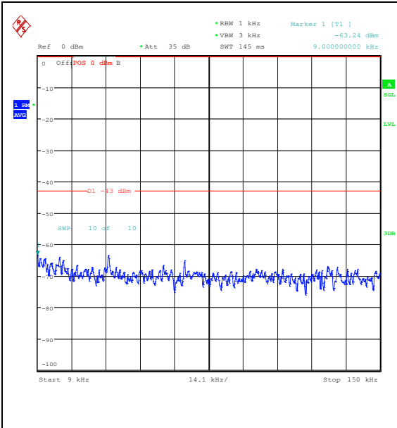
Band25_5MHz_QPSK_26065_25RB#0_0.009~0.15_0.009~0.15
