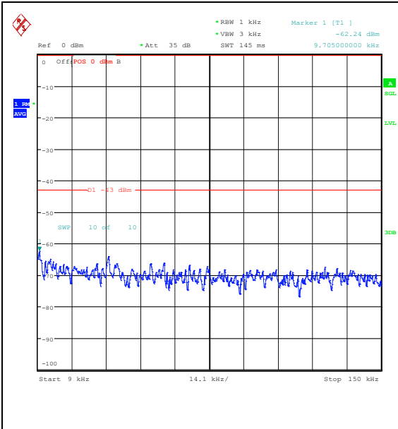
Band25_10MHz_QPSK_26365_1RB#0_0.009~0.15_0.009~0.15
