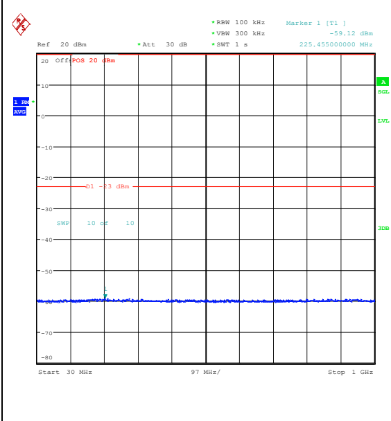
Band25_3MHz_QPSK_26675_1RB#14_30~1000
