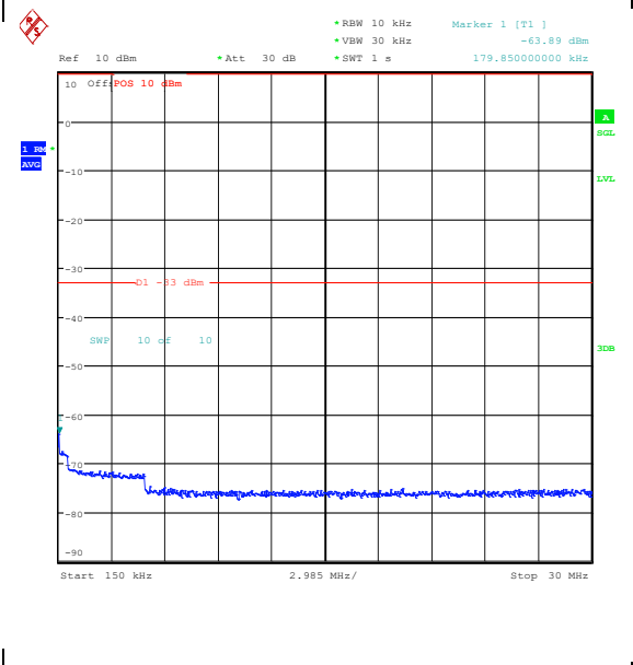
Band25_3MHz_QPSK_26675_1RB#0_0.15~30_0.15~30
