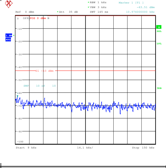
Band25_3MHz_16QAM_26365_1RB#14_0.009~0.15 15_0.009~0.15
