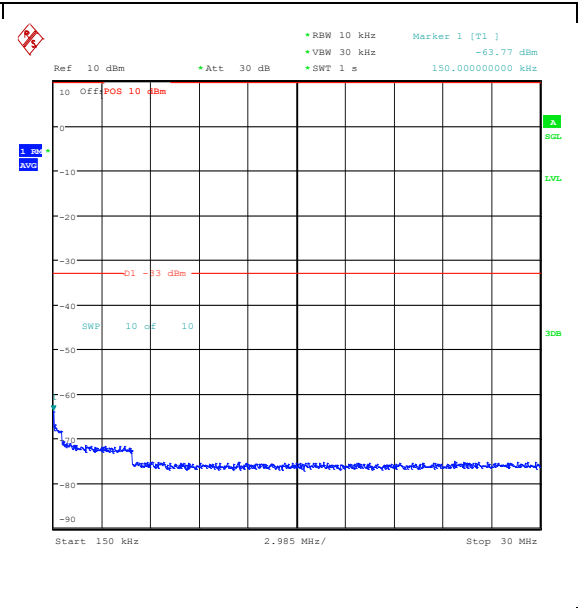
Band25_10MHz_QPSK_26365_1RB#0_0.15~30_0.15~30
