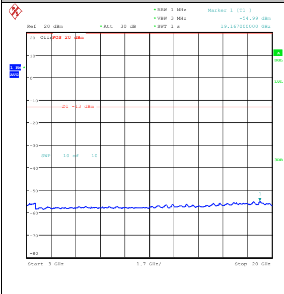
Band25_1.4MHz_QPSK_26683_1RB#5_3000~20000 000_3000~20000
