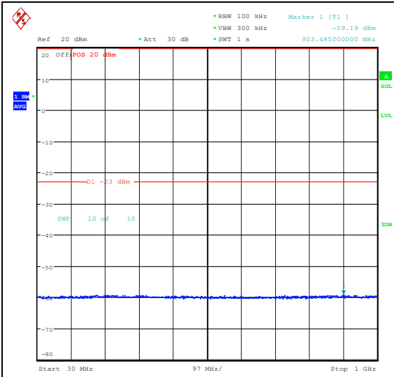
Band25_5MHz_QPSK_26065_1RB#24_30~1000_30~1000
