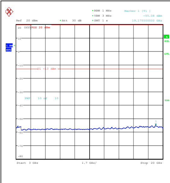
Band25_5MHz_QPSK_26065_25RB#0_3000~2000_3000~20000
