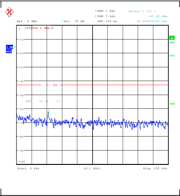
Band25_3MHz_16QAM_26055_1RB#14_0.009~0.15_0.009~0.15
