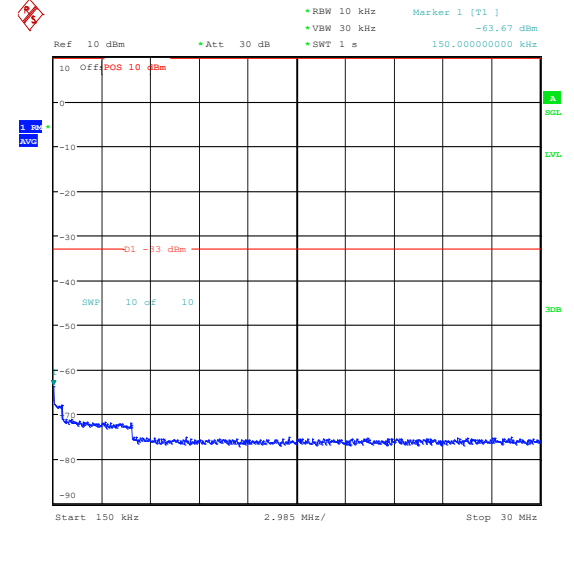
Band25_5MHz_QPSK_26065_1RB#24_0.15~30_0.15~30
