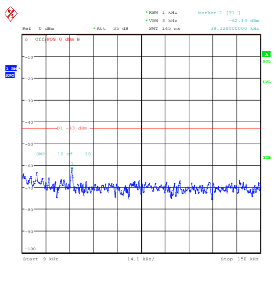
Band25_5MHz_16QAM_26665_1RB#24_0.009~0.15_0.009~0.15
