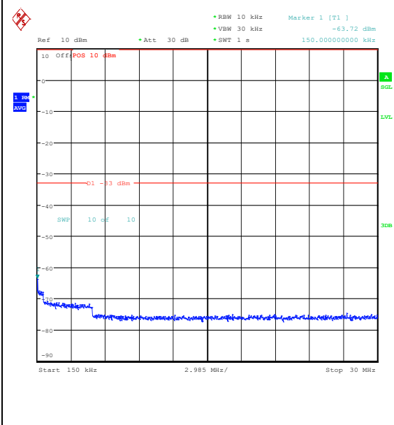
Band25_10MHz_16QAM_26090_1RB#49_0.15~30_0.15~30
