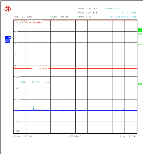
Band25_10MHz_QPSK_26365_1RB#49_30~100 0_30~1000
