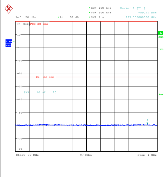
Band25_3MHz_QPSK_26055_1RB#14_30~1000_30~1000
