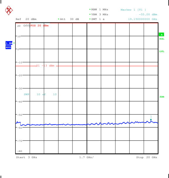
Band25_5MHz_16QAM_26665_1RB#24_3000~20 000_3000~20000
