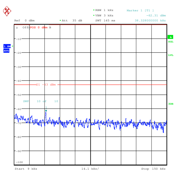
Band25_10MHz_16QAM_26365_1RB#49_0.009~ 0.15_0.009~0.15
