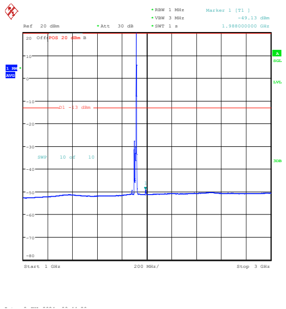
Band25_10MHz_QPSK_26640_1RB#49_1000~3000_00_1000~3000
