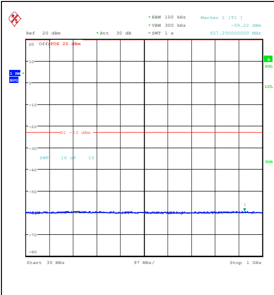
Band25_3MHz_QPSK_26055_1RB#0_30~1000_30~1000
