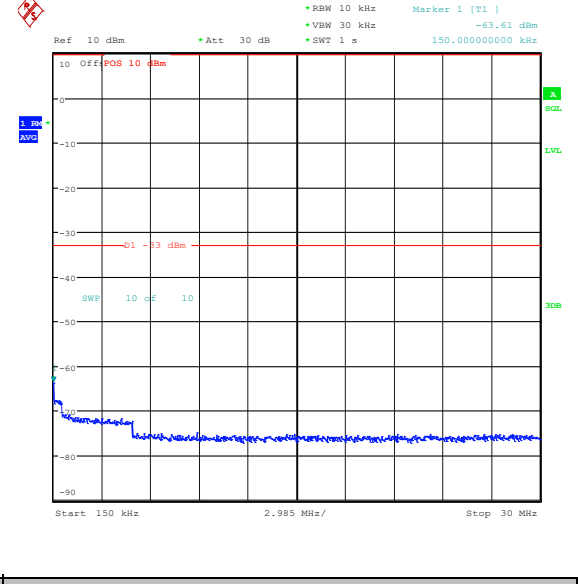
Band25_1.4MHz_QPSK_26683_1RB#5_0.15~30_0.15~30
