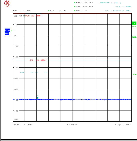
Band25_5MHz_QPSK_26365_1RB#24_30~1000_30~1000
