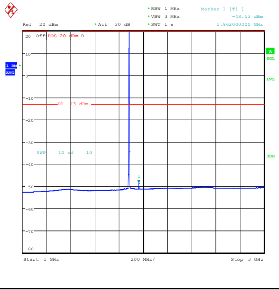
Band25_3MHz_QPSK_26365_1RB#0_1000~3000_1000~3000
