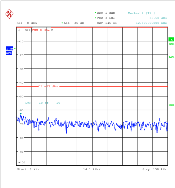
Band25_5MHz_QPSK_26665_25RB#0_0.009~0.15_0.009~0.15
