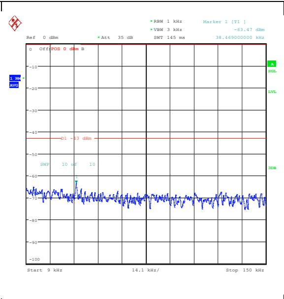
Band25_5MHz_16QAM_26065_25RB#0_0.009~0.15_0.009~0.15
