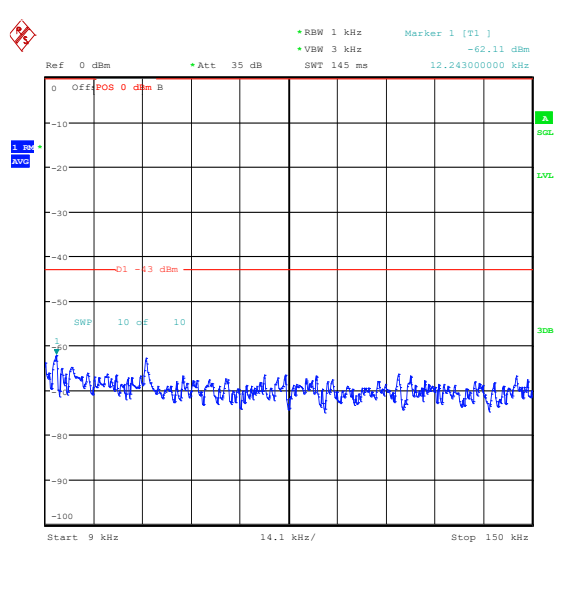
Band25_10MHz_16QAM_26090_1RB#0_0.009~0.15_0.009~0.15
