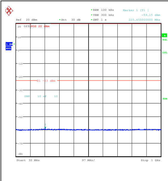
Band25_10MHz_QPSK_26640_1RB#0_30~1000_30~1000
