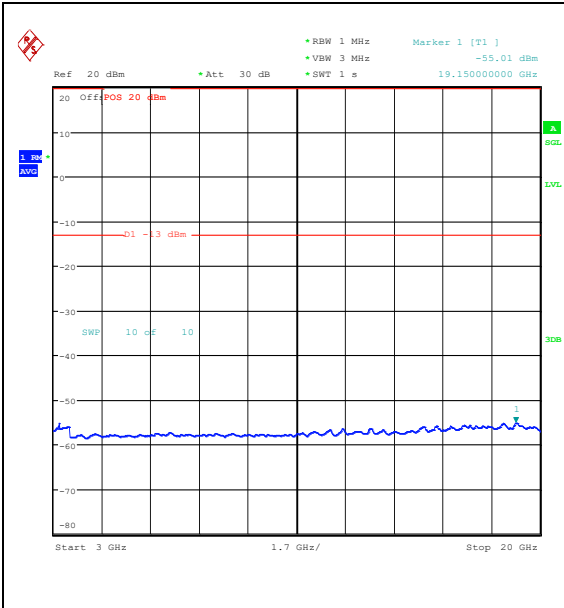
Band25_10MHz_QPSK_26640_1RB#49_3000~20000
