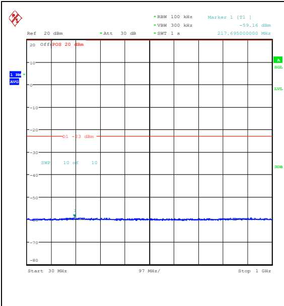
Band25_5MHz_QPSK_26665_1RB#24_30~1000_30~1000
