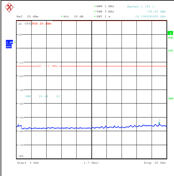
Band25_3MHz_QPSK_26055_15RB#0_3000~20000 000_3000~20000
