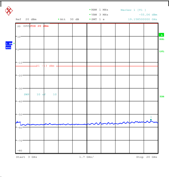
Band25_10MHz_16QAM_26365_50RB#0_3000~0000_3000~20000
