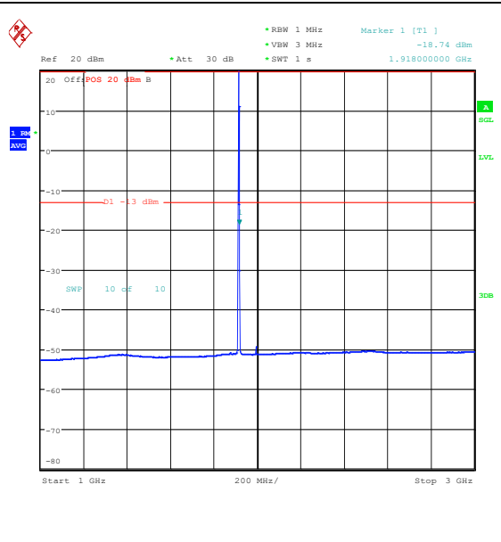
Band25_1.4MHz_QPSK_26683_1RB#5_1000~3000 00_1000~3000
