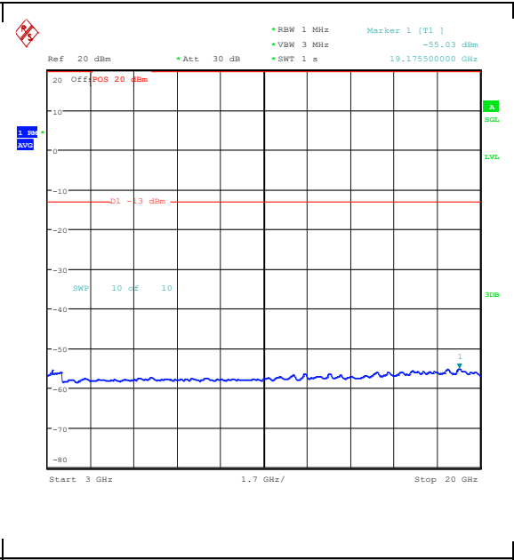
Band25_3MHz_16QAM_26365_1RB#0_3000~20000_00_3000~20000
