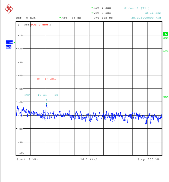
Band25_10MHz_QPSK_26090_1RB#0_0.009~0.15_0.009~0.15
