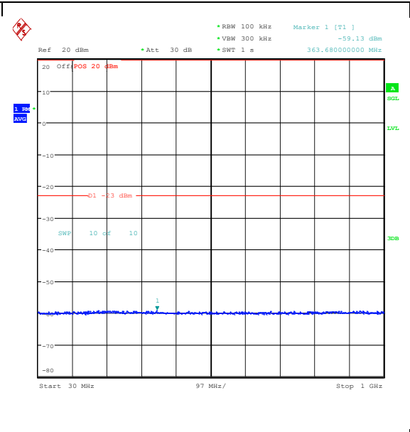
Band25_1.4MHz_16QAM_26683_1RB#5_30~100 0_30~1000
