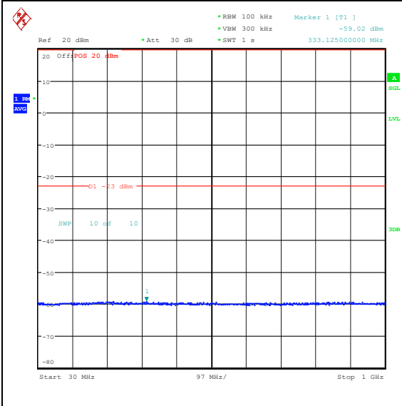
Band25_10MHz_QPSK_26365_1RB#0_30~1000_30~1000
