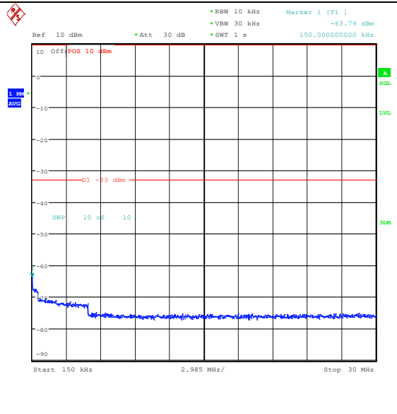
Band25_3MHz_QPSK_26365_15RB#0_0.15~30_0.15~30
