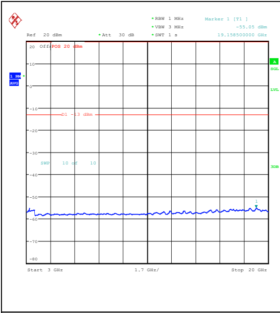
Band25_3MHz_QPSK_26055_1RB#14_3000~20000_000_3000~20000
