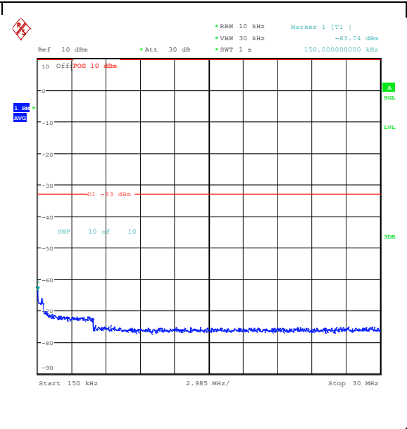
Band25_1.4MHz_QPSK_26683_6RB#0_0.15-30_0.15-30
