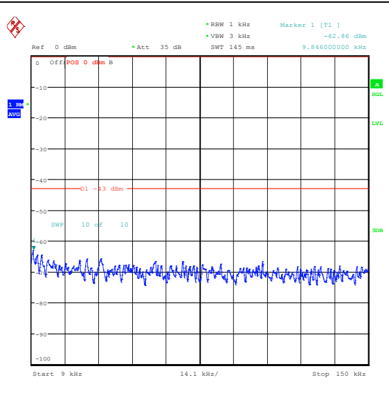
Band25_10MHz_16QAM_26090_1RB#49_0.009~0.15_0.15_0.009~0.15
