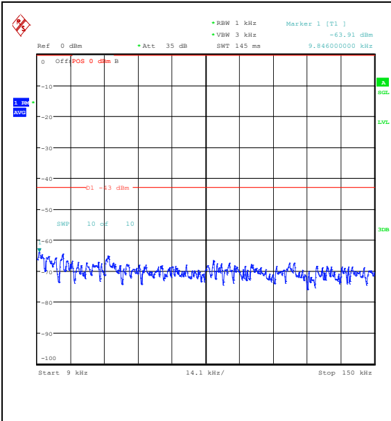
Band25_10MHz_QPSK_26640_1RB#49_0.009~0.15_0.009~0.15
