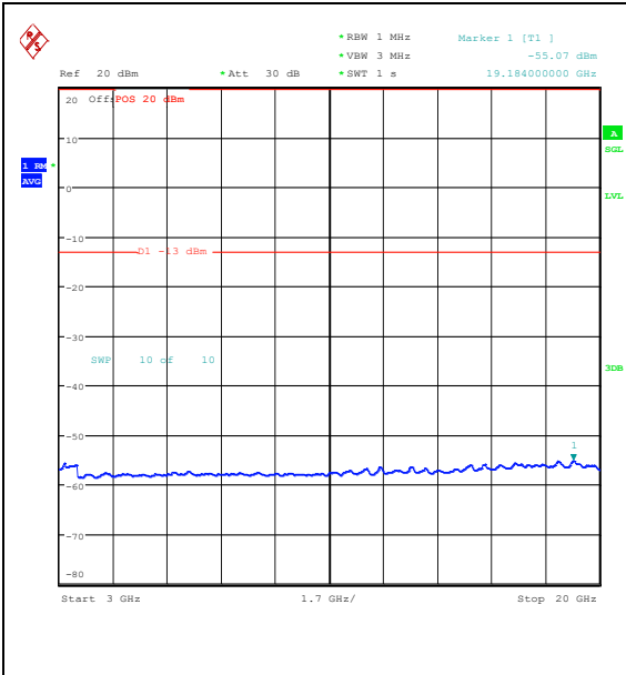
Band25_5MHz_QPSK_26065_1RB#0_3000~20000_00_3000~20000
