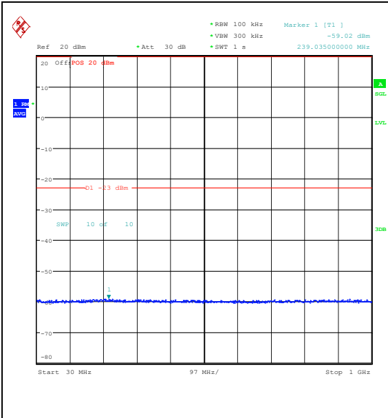
Band25_10MHz_QPSK_26090_50RB#0_30~100 0_30~1000
