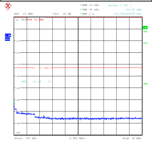
Band25_10MHz_QPSK_26090_50RB#0_0.15~30.15_0.15~30
