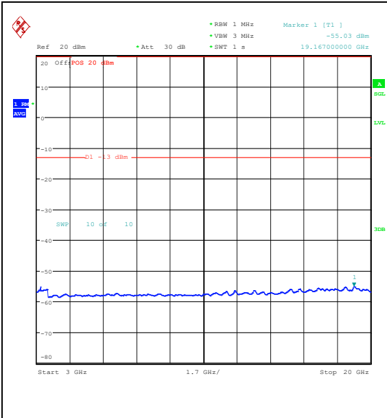
Band25_3MHz_QPSK_26365_15RB#0_3000~2000_3000~20000
