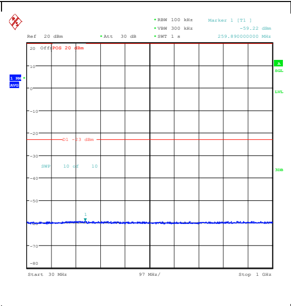
Band25_3MHz_16QAM_26055_1RB#0_30~1000_30~1000
