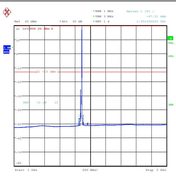
Band25_10MHz_QPSK_26365_1RB#49_1000~30 00_1000~3000
