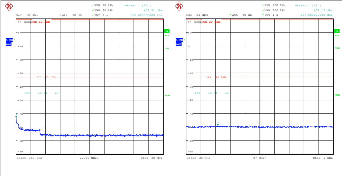
Band25_1.4MHz_16QAM_26683_6RB#0_0.15~30_0.15~30 Band25_1.4MHz_16QAM_26683_6RB#0_30~100_0_30~1000
