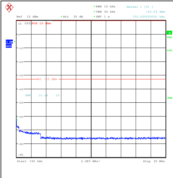
Band25_3MHz_16QAM_26675_15RB#0_0.15~30_0.15~30
