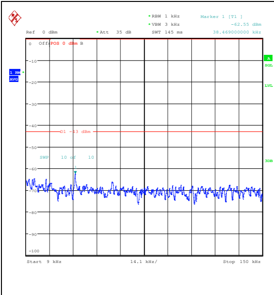
Band25_1.4MHz_QPSK_26683_6RB#0_0.009-0.15
