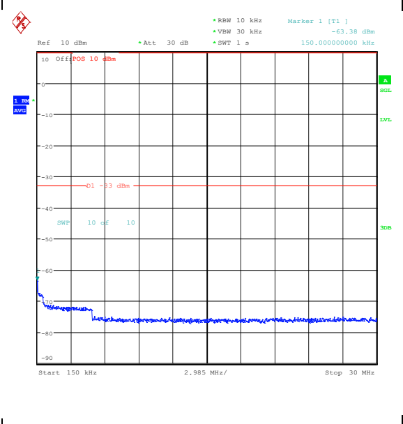
Band25_10MHz_QPSK_26090_1RB#0_0.15~30_0.15~30
