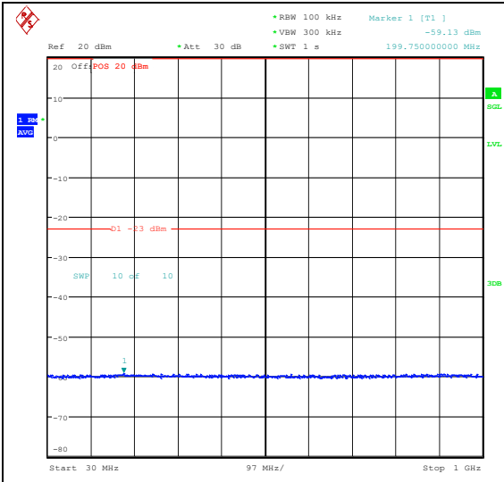
Band25_5MHz_QPSK_26365_1RB#0_30~1000_30~1000
