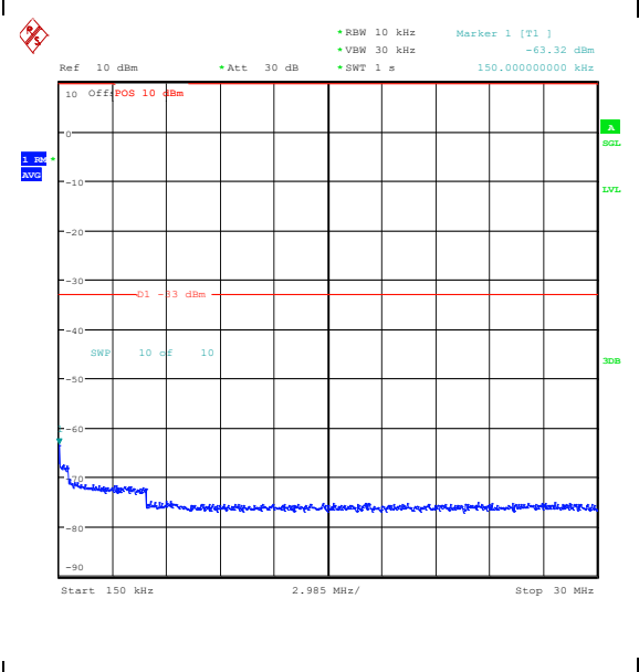
Band25_10MHz_QPSK_26640_1RB#0_0.15~30_0.15~30
