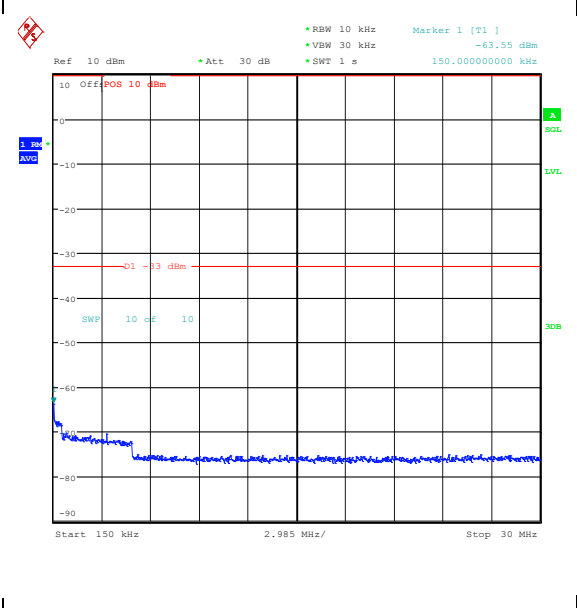
Band25_5MHz_QPSK_26365_25RB#0_0.15~30_0.15~30
