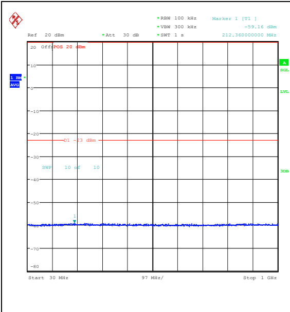
Band25_5MHz_QPSK_26365_25RB#0_30~1000 _30~1000
