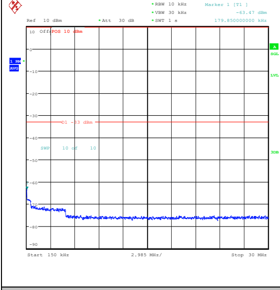
Band25_3MHz_16QAM_26365_1RB#0_0.15~30_0.15~30
