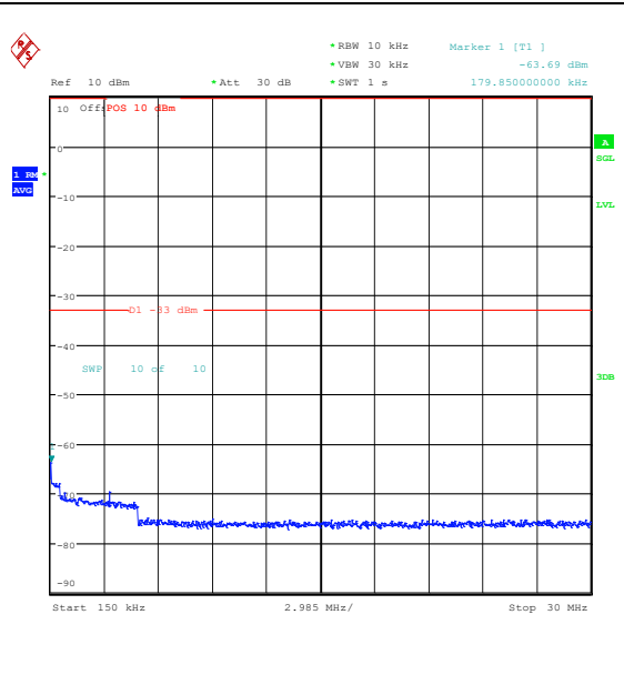
Band25_5MHz_QPSK_26065_25RB#0_0.15~30_0.15~30
