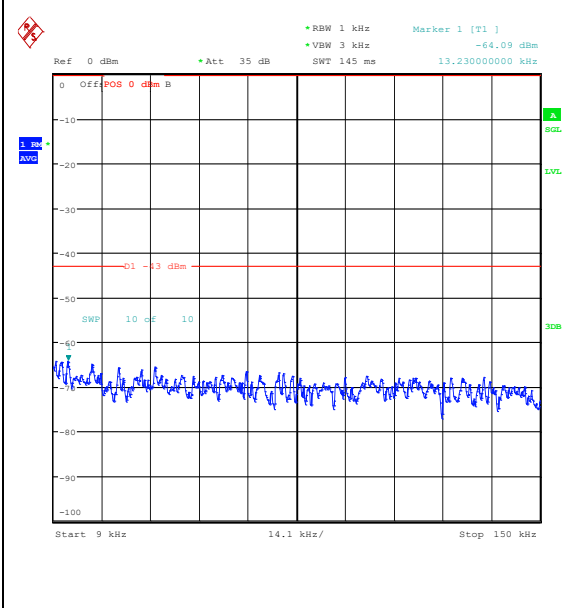
Band25_10MHz_QPSK_26365_1RB#49_0.009~0.15_0.009~0.15
