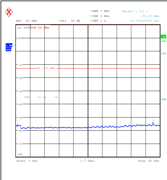
Band25_3MHz_QPSK_26365_1RB#0_3000~20000_00_3000~20000
