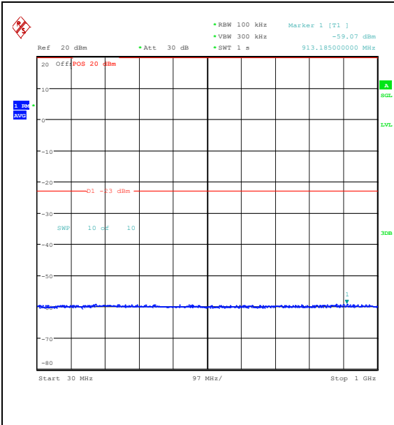
Band25_3MHz_QPSK_26365_1RB#14_30~1000 _30~1000
