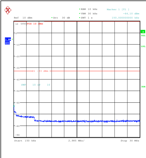
Band25_3MHz_16QAM_26055_1RB#0_0.15~30_0.15~30
