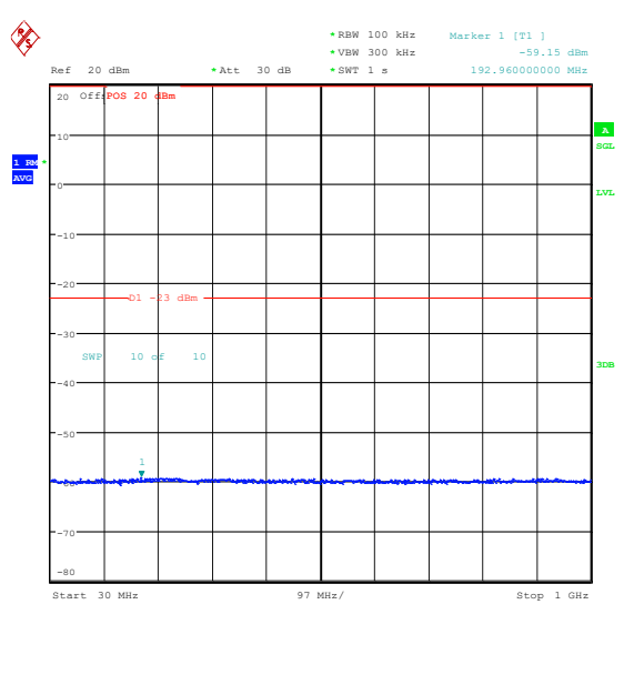
Band25_10MHz_16QAM_26090_1RB#49_30~100_0_30~1000
