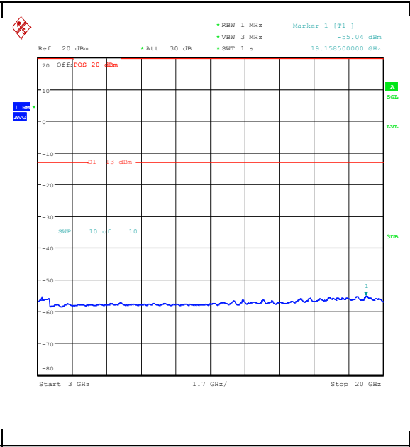
Band25_5MHz_16QAM_26665_1RB#0_3000~20000_00_3000~20000
