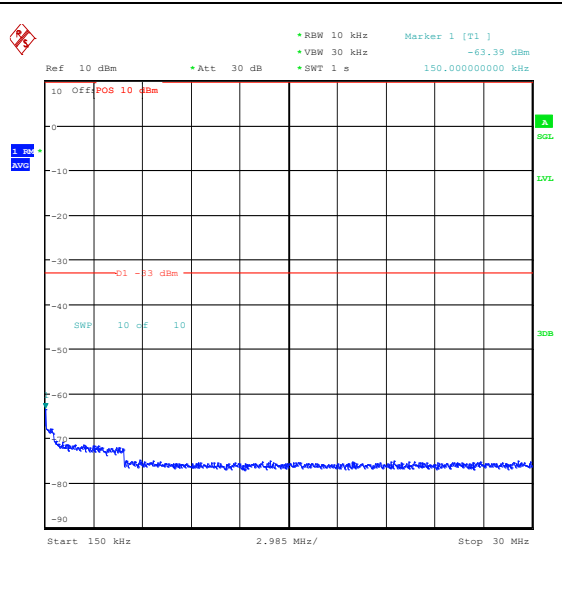
Band25_10MHz_QPSK_26640_1RB#49_0.15~30_0.15~30
