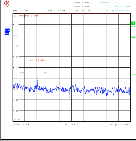
Band25_1.4MHz_QPSK_26683_1RB#5_0.009~0.15_0.009~0.15
