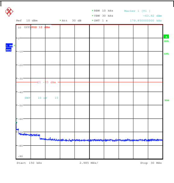
Band25_10MHz_QPSK_26365_50RB#0_0.15~30_0.15~30
