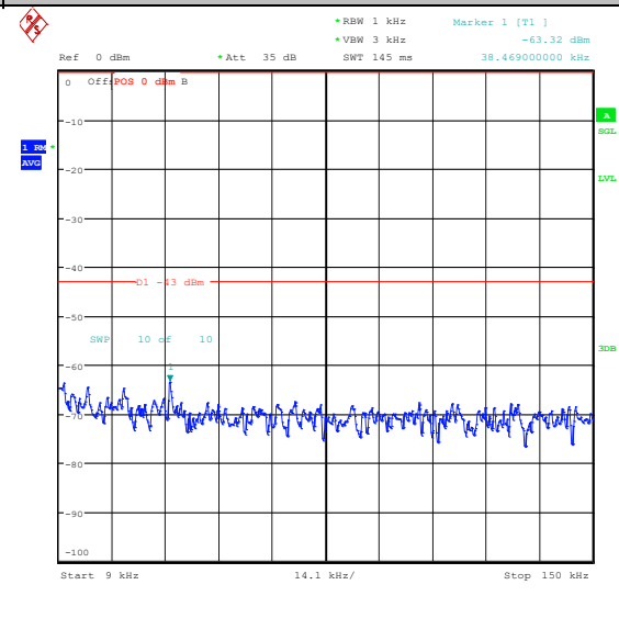
Band25_5MHz_16QAM_26365_25RB#0_0.009~0.15 15_0.009~0.15
