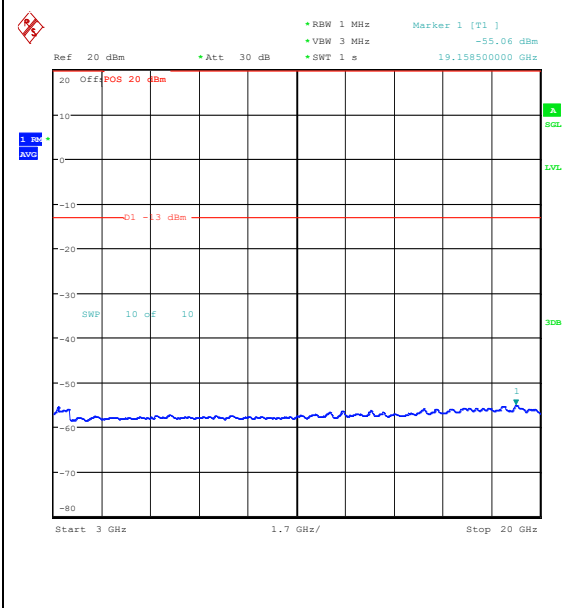
Band25_10MHz_QPSK_26090_1RB#0_3000~20000_000_3000~20000
