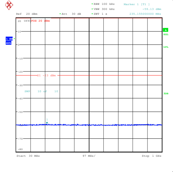
Band25_3MHz_16QAM_26365_15RB#0_30~1000_30~1000
