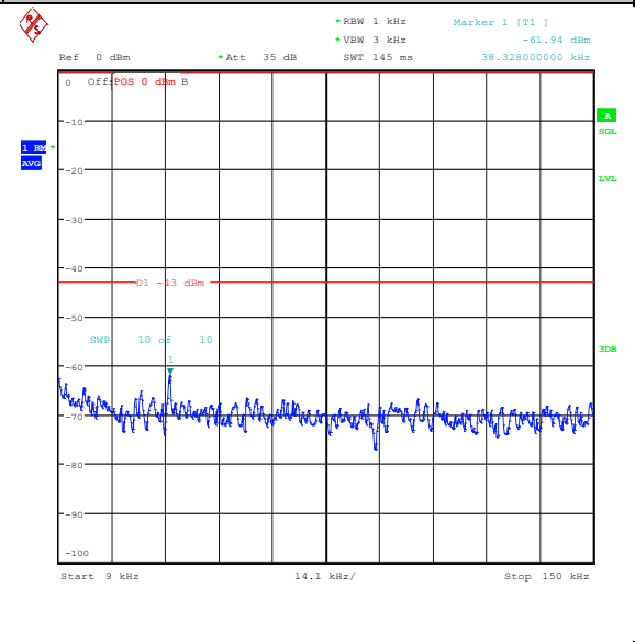
Band25_3MHz_16QAM_26055_1RB#0_0.009~0.15_5_0.009~0.15
