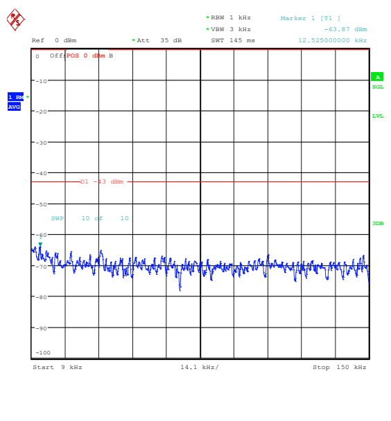
Band25_10MHz_16QAM_26640_1RB#0_0.009~0.15_0.009~0.15
