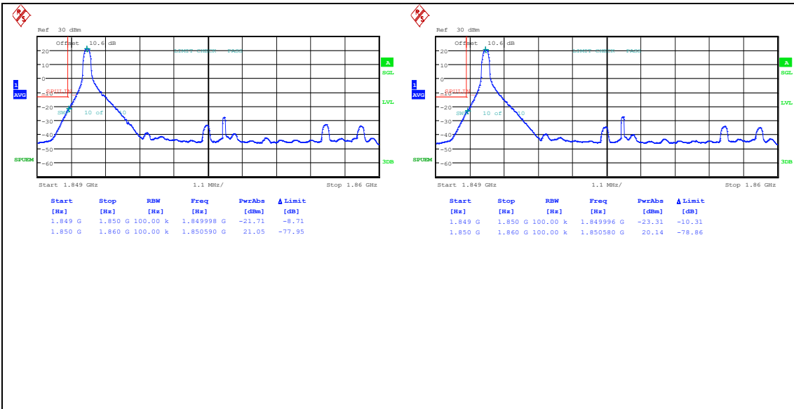
Band25_10MHz_QPSK_26090_1RB#0
