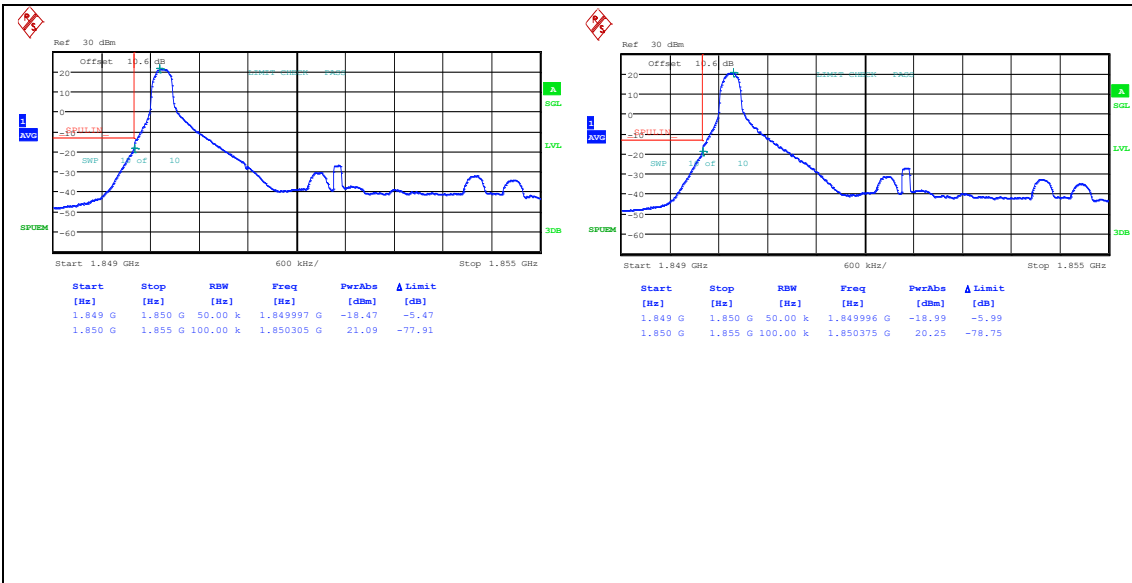
Band25_5MHz_QPSK_26065_1RB#0
