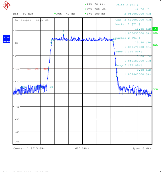
Band25-3MHz-16QAM-26055-15RB#0-PASS
