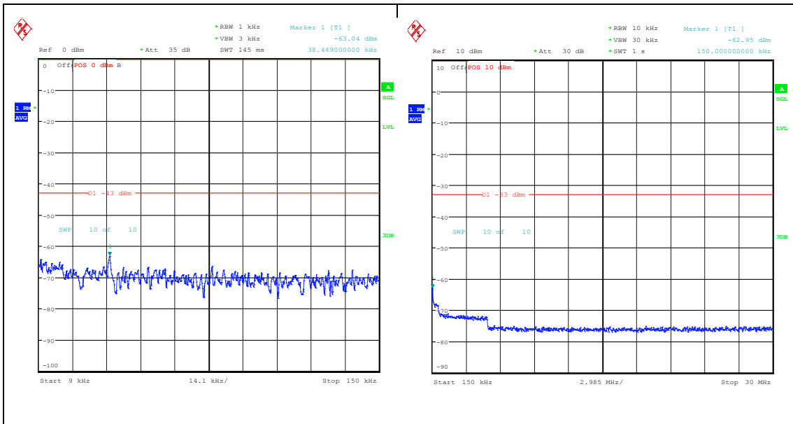
Band25_1.4MHz_QPSK_26047_1RB#0_0.009~0.15_0.009~0.15 Band25_1.4MHz_QPSK_26047_1RB#0_0.15~30_0.15~30
