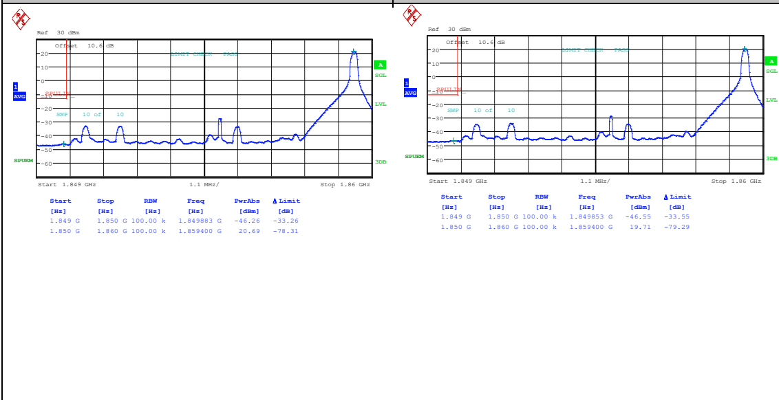
Band25_10MHz_QPSK_26090_1RB#49
