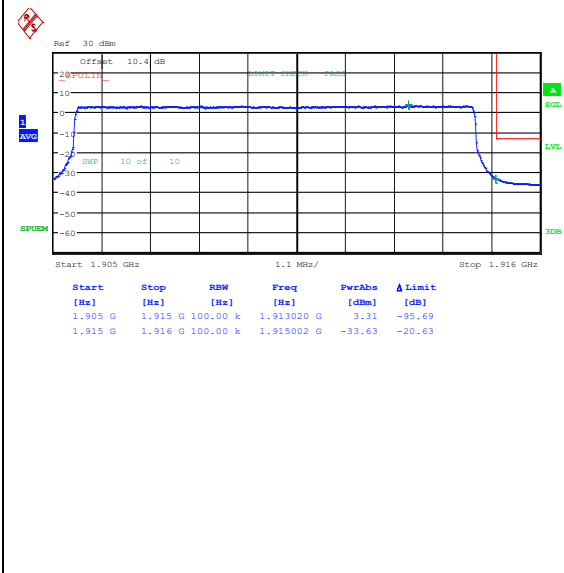
Band25_10MHz_QPSK_26640_50RB#0
