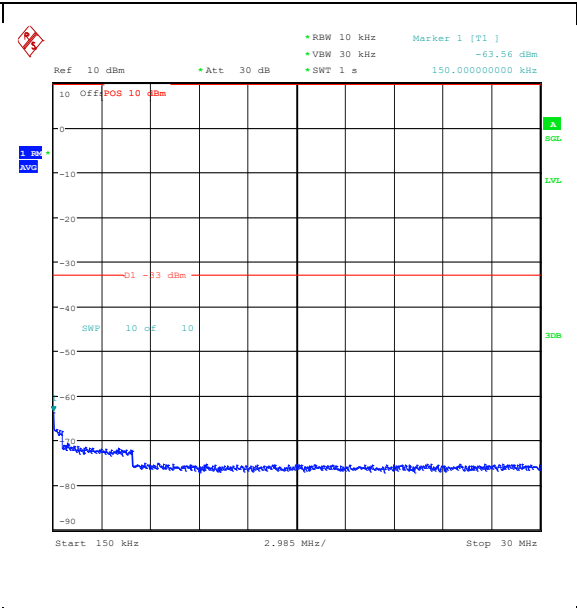
Band25_1.4MHz_QPSK_26365_1RB#5_0.15~30_0.15~30
