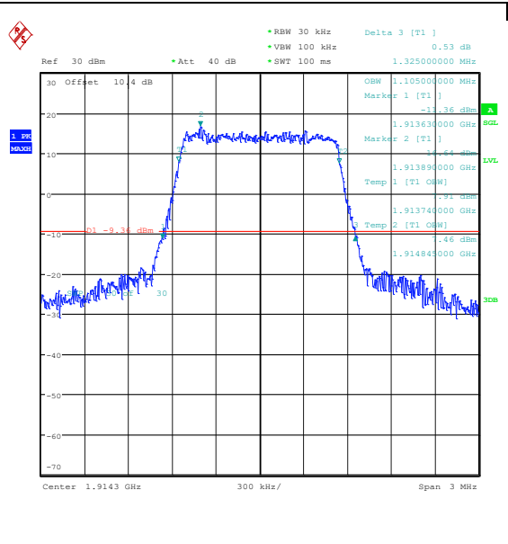
Band25-1.4MHz-16QAM-26683-6RB#0-PASS
