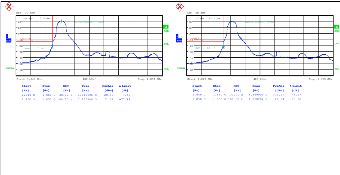
Band25_3MHz_QPSK_26055_1RB#0
