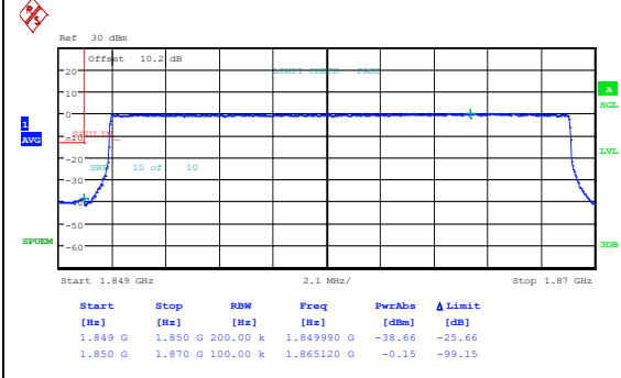
Band25_20MHz_QPSK_26140_1RB#99
