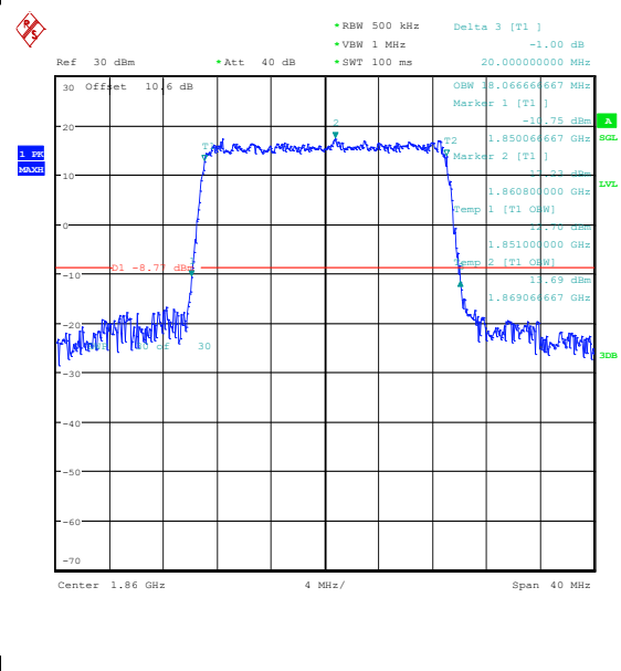
Band25-20MHz-16QAM-26140-100RB#0-PASS
