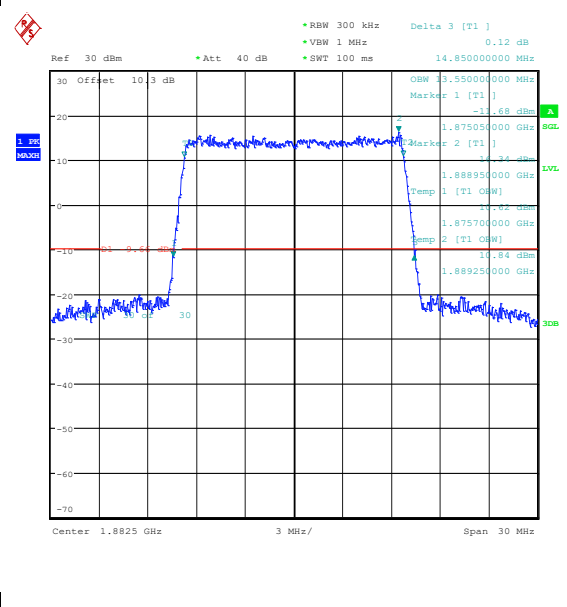
Band25-15MHz-16QAM-26365-75RB#0-PASS
