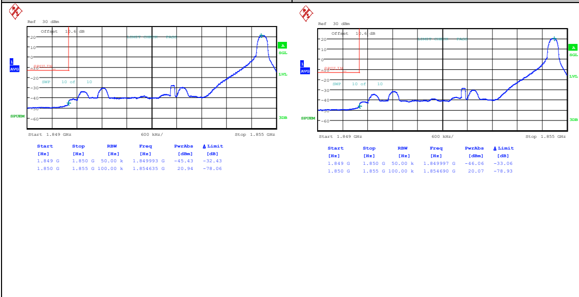
Band25_5MHz_QPSK_26065_1RB#24
