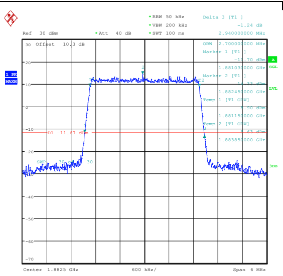
Band25-3MHz-16QAM-26365-15RB#0-PASS
