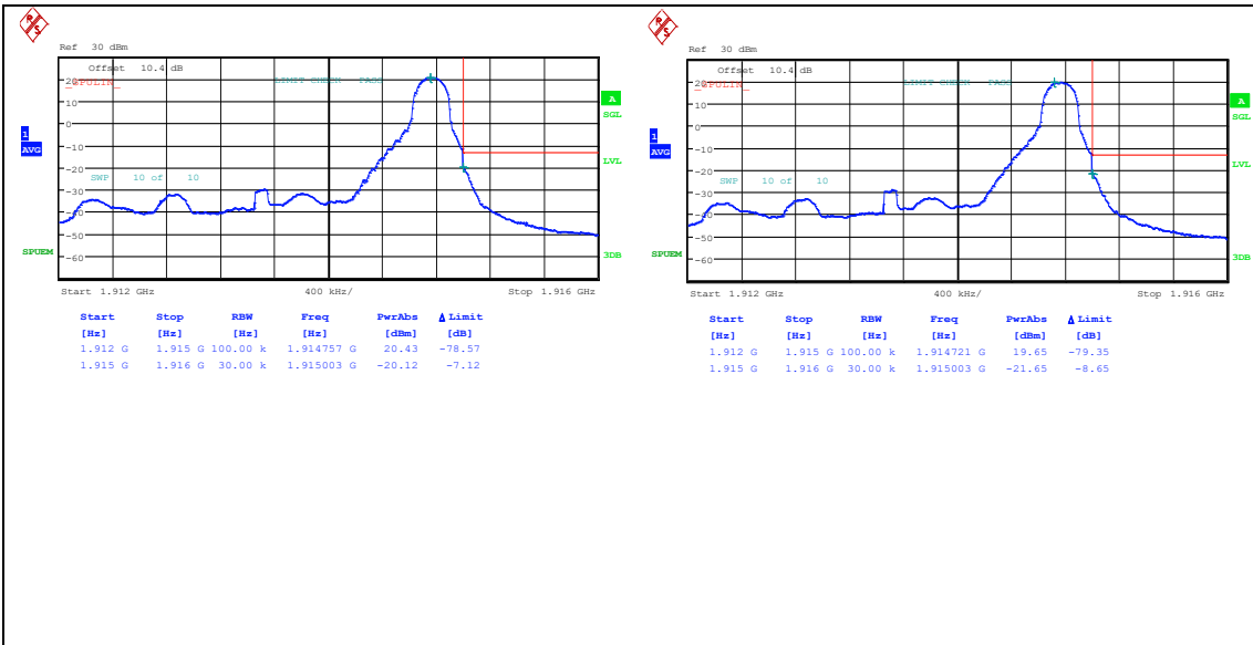
Band25_3MHz_QPSK_26675_1RB#14
