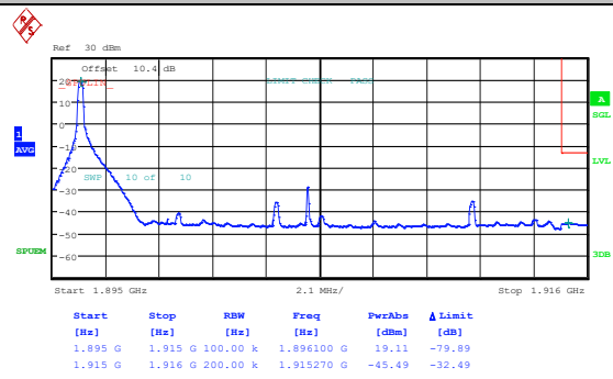
Band25_20MHz_16QAM_26140_100RB#0
