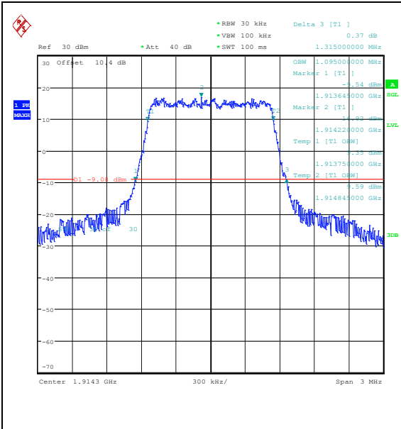
Band25-1.4MHz-QPSK-26683-6RB#0-PASS
