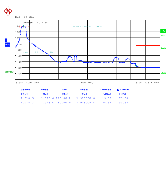
Band25_5MHz_16QAM_26665_1RB#0
