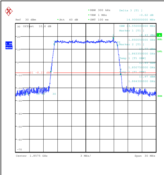
Band25-15MHz-QPSK-26115-75RB#0-PASS
