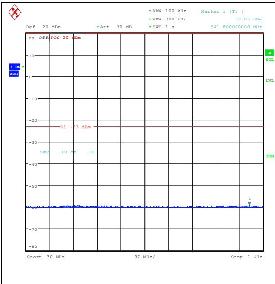
Band25_1.4MHz_QPSK_26047_1RB#5_30~1000_30~1000
