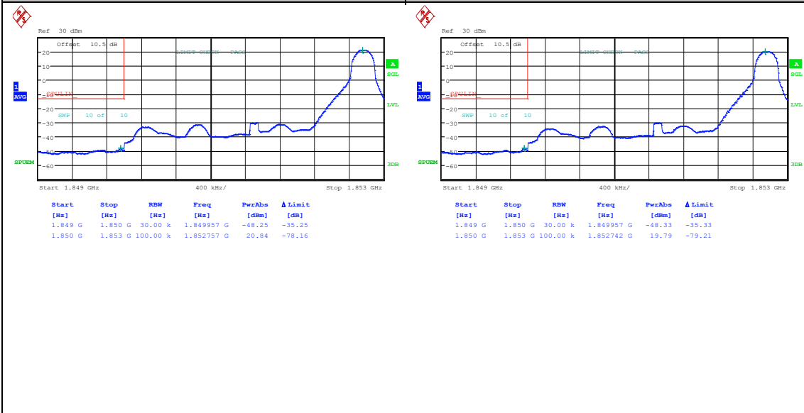
Band25_3MHz_QPSK_26055_1RB#14
