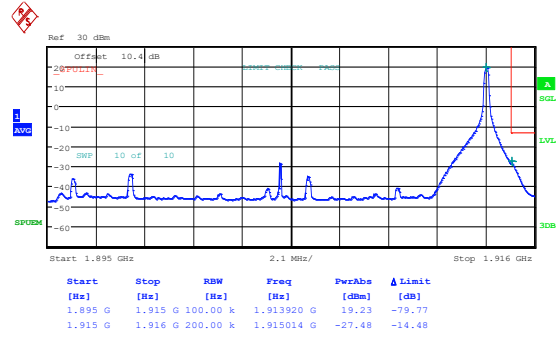
Band25_20MHz_16QAM_26590_1RB#0
