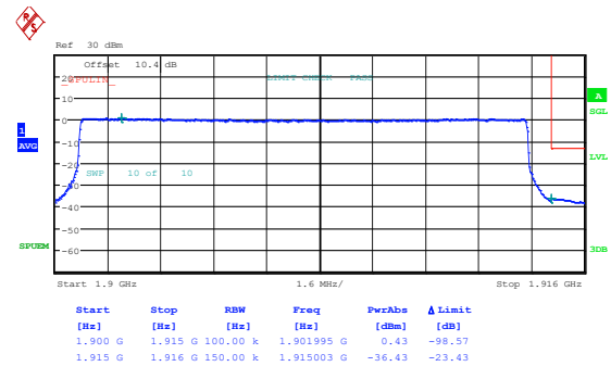
Band25_15MHz_16QAM_26615_1RB#74
