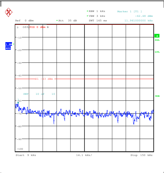
Band25_1.4MHz_16QAM_26047_6RB#0_0.009~0.15_0.009~0.15
