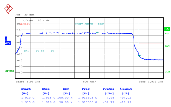
Band25_5MHz_16QAM_26665_1RB#24
