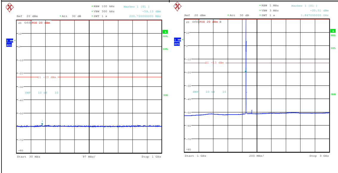
Band25_1.4MHz_QPSK_26047_1RB#0_30~1000_30~1000 Band25_1.4MHz_QPSK_26047_1RB#0_1000~3000_00_1000~3000
