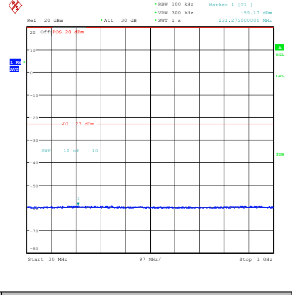
Band25_1.4MHz_16QAM_26683_1RB#0_30~100_30~100
