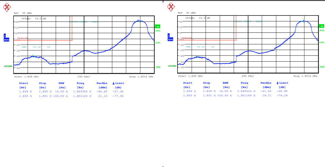
Band25_1.4MHz_QPSK_26047_1RB#5
