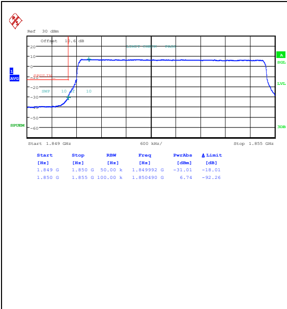
Band25_5MHz_QPSK_26065_25RB#0
