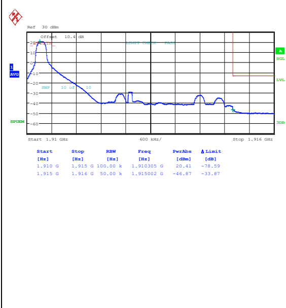
Band25_5MHz_QPSK_26665_1RB#0
