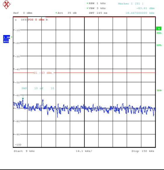
Band25_1.4MHz_16QAM_26047_1RB#5_0.009~0.15_009_0.009~0.15
