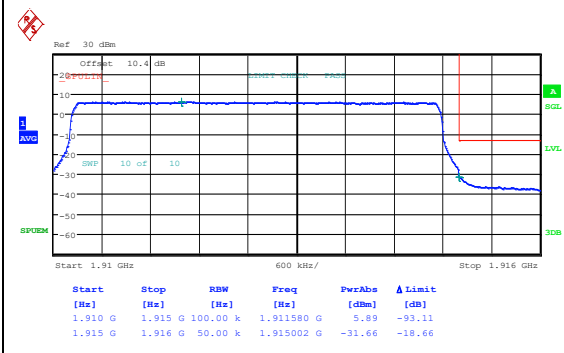
Band25_5MHz_QPSK_26665_1RB#24
