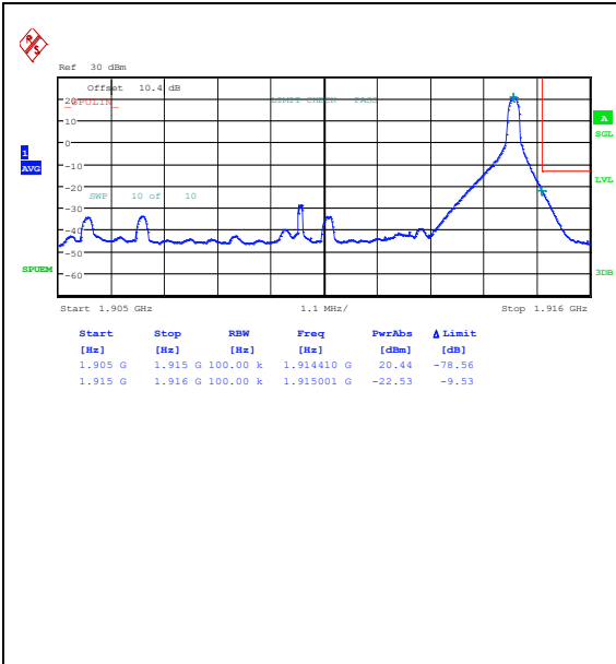
Band25_10MHz_QPSK_26640_1RB#49
