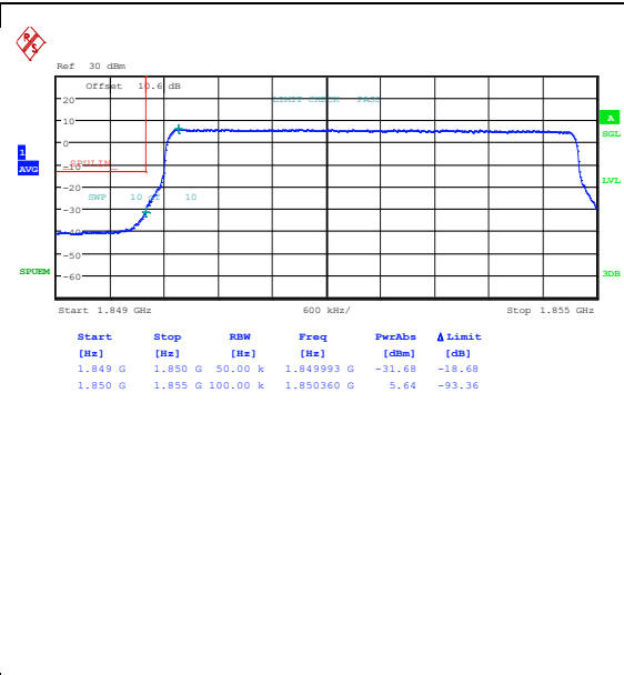
Band25_5MHz_16QAM_26065_25RB#0
