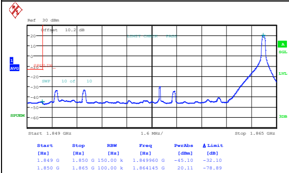
Band25_15MHz_QPSK_26115_1RB#0
