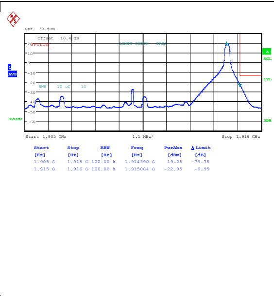
Band25_10MHz_16QAM_26640_1RB#49
