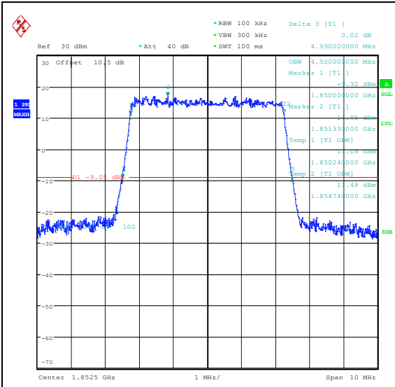
Band25-5MHz-QPSK-26065-25RB#0-PASS
