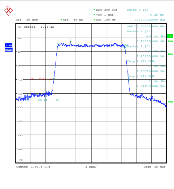
Band25-15MHz-16QAM-26615-75RB#0-PASS
