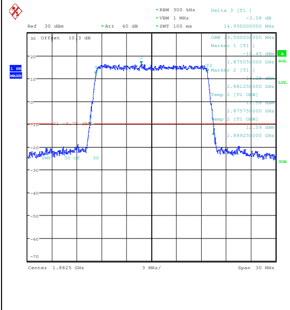
Band25-15MHz-QPSK-26365-75RB#0-PASS
