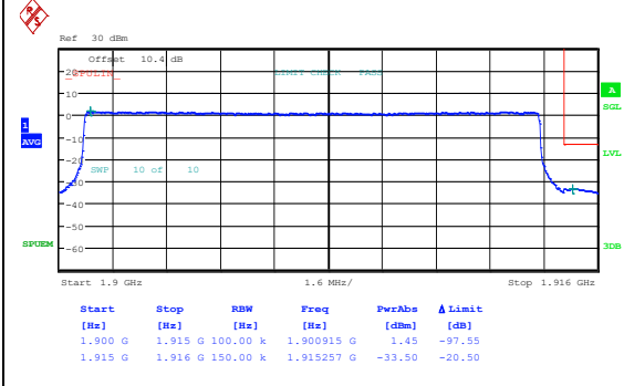
Band25_15MHz_QPSK_26615_1RB#74
