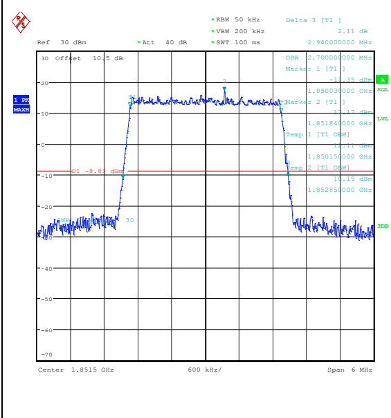
Band25-3MHz-QPSK-26055-15RB#0-PASS
