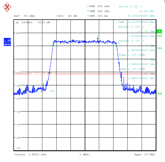
Band25-5MHz-16QAM-26365-25RB#0-PASS
