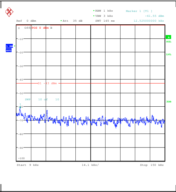
Band25_1.4MHz_16QAM_26683_1RB#0_0.009~0.15_0.009~0.15
