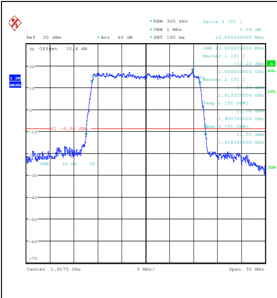
Band25-15MHz-QPSK-26615-75RB#0-PASS
