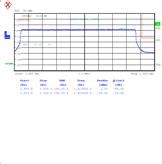
Band25_10MHz_16QAM_26640_50RB#0
