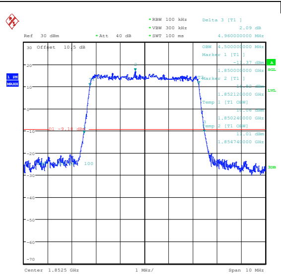
Band25-5MHz-16QAM-26065-25RB#0-PASS
