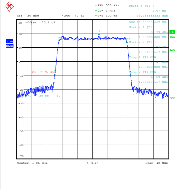
Band25-20MHz-QPSK-26140-100RB#0-PASS
