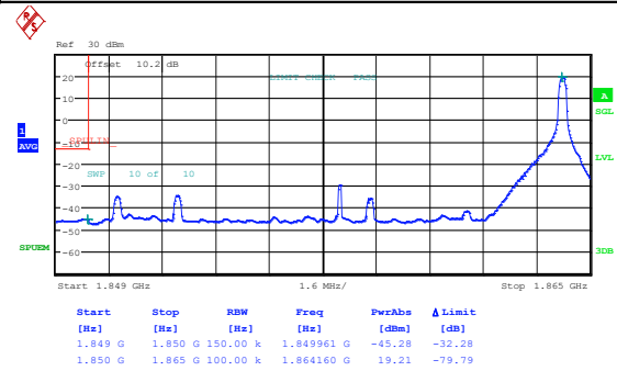
Band25_15MHz_16QAM_26115_1RB#0
