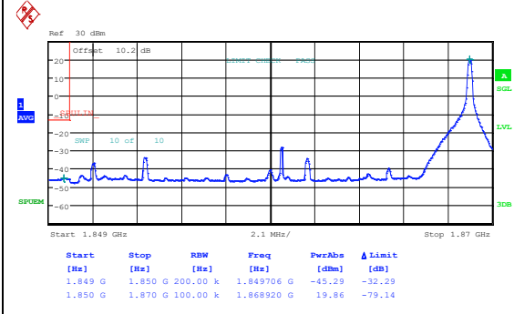
Band25_20MHz_QPSK_26140_1RB#0
