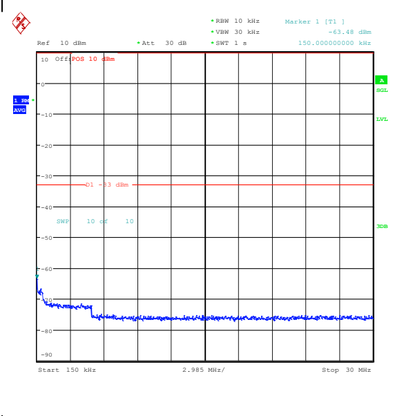
Band25_1.4MHz_QPSK_26365_6RB#0_0.15~30_0.15~30
