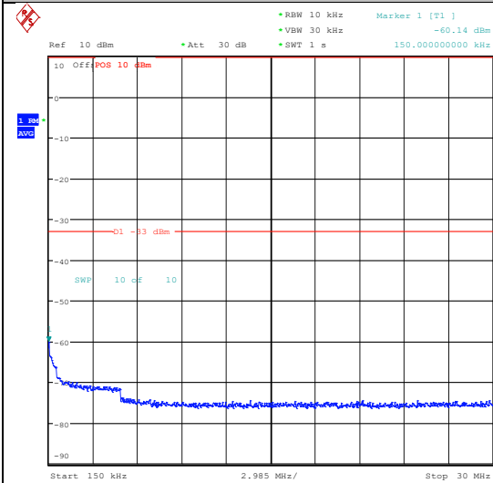
Band4_15MHz_QPSK_20325_1RB#0_3000~2000_00_3000~20000
