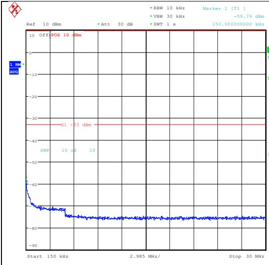
Band2_3MHz_16QAM_18900_1RB#14_0.15~30 _0.15~30
