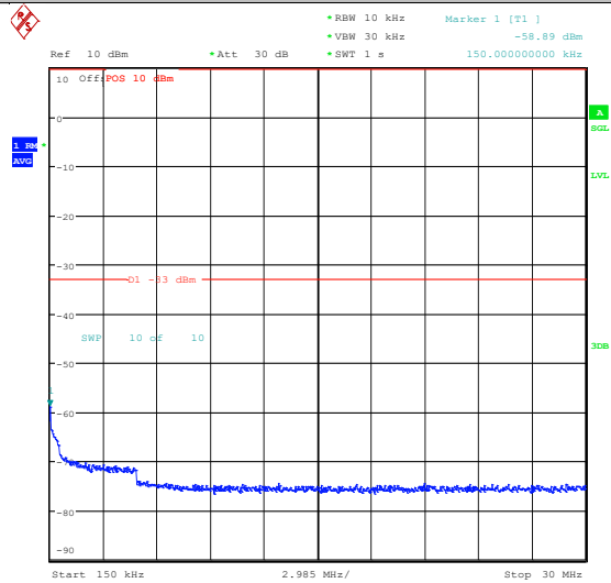
Band2_3MHz_16QAM_18900_1RB#0_3000~2000 0_3000~20000
