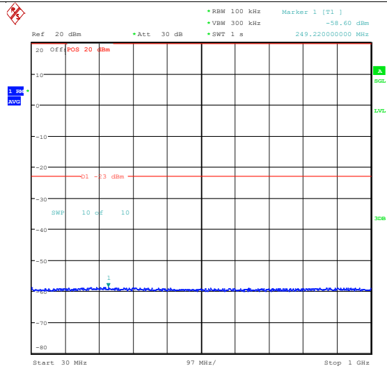
Band2_3MHz_16QAM_18900_1RB#14_30~1000_ 30~1000
