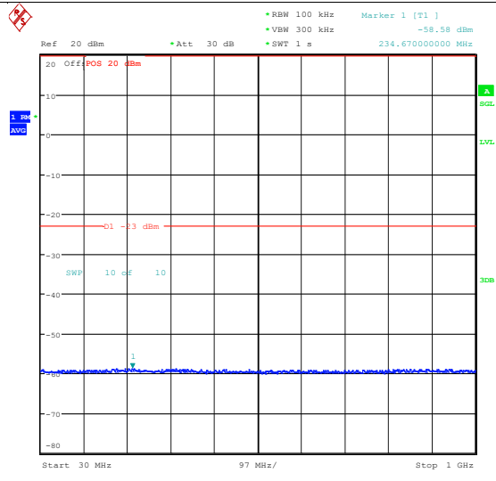
Band2_3MHz_16QAM_19185_15RB#0_30~1000_ 30~1000
