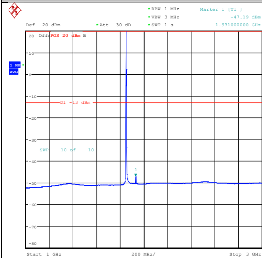
Band2_3MHz_16QAM_18615_1RB#0_0.15~30_0.15~30
