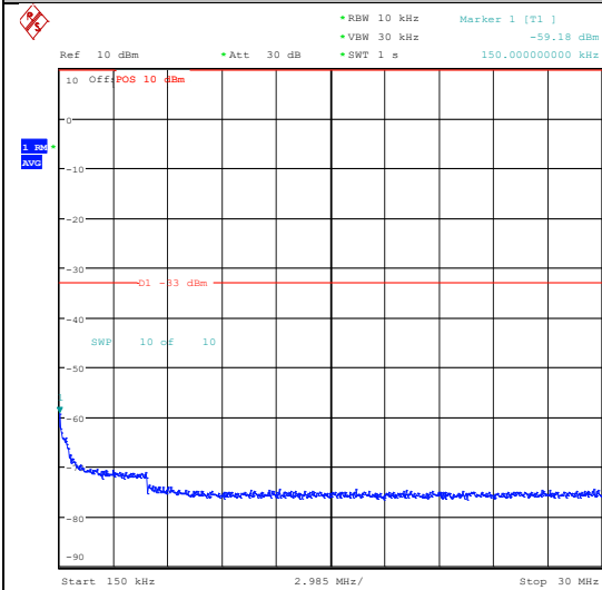
Band2_1.4MHz_QPSK_19193_6RB#0_3000~2000_00_3000~20000
