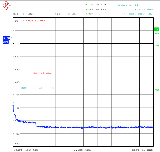
Band2_1.4MHz_16QAM_19193_1RB#0_3000~20000_3000~20000
