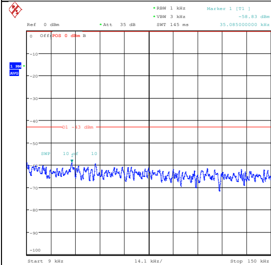
Band2_5MHz_16QAM_18625_1RB#0_1000~300 0_1000~3000
