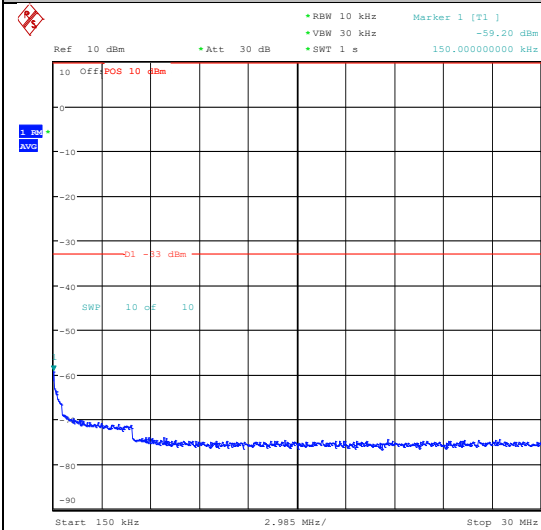
Band2_3MHz_QPSK_18615_1RB#14_3000~20000_00_3000~20000
