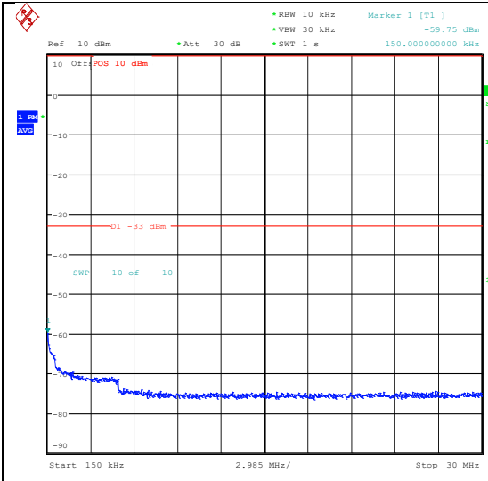
Band2_3MHz_16QAM_19185_15RB#0_0.15~30 _0.15~30
