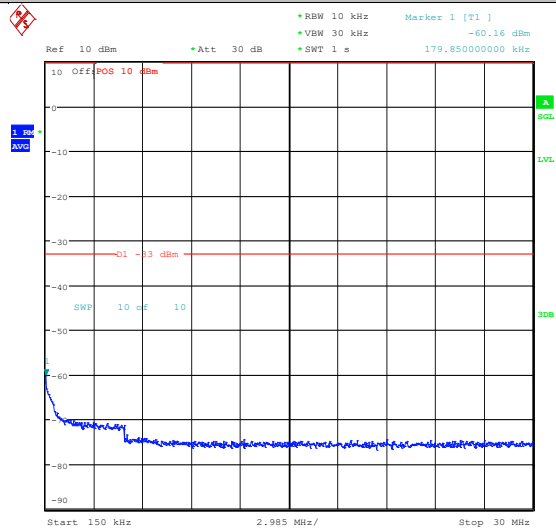
Band2_1.4MHz_16QAM_19193_6RB#0_3000~20000_3000~20000
