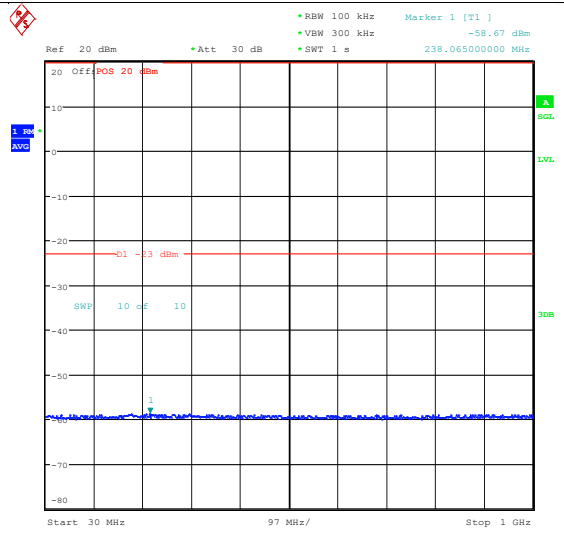
Band2_10MHz_16QAM_19150_1RB#0_30~1000_30~1000
