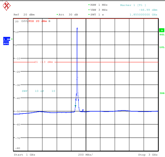
Band2_10MHz_QPSK_18900_50RB#0_0.15~30_0.15~30
