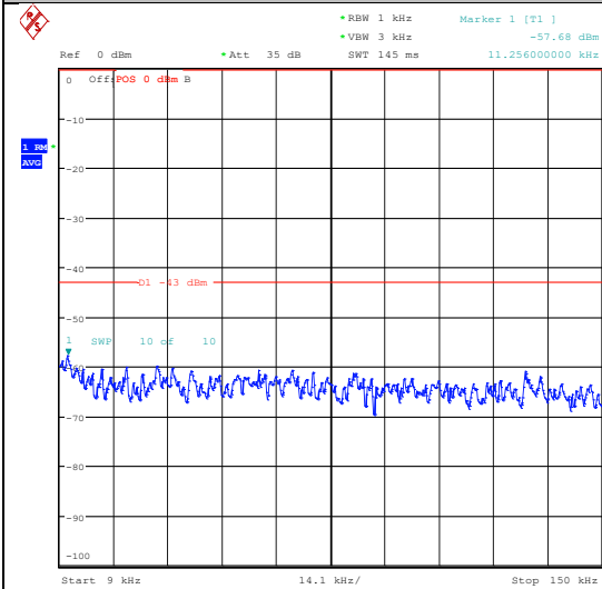
Band2_3MHz_16QAM_18900_1RB#0_1000~300 0_1000~3000
