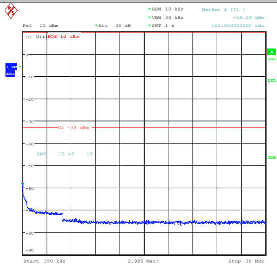
Band2_5MHz_16QAM_19175_1RB#0_3000~2000 0_3000~20000
