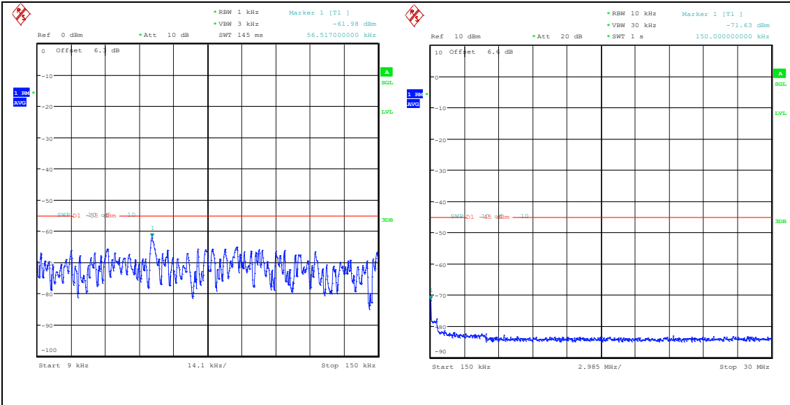
Band41(2535-2655)-15MHz-QPSK-40115-1RB#0-0.009~0.15-PASS
