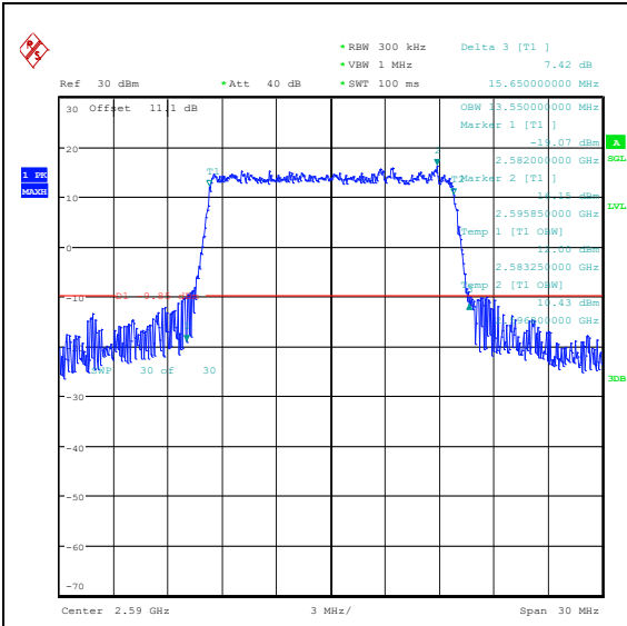
Band41(2535-2655)-15MHz-QPSK-40590-75RB#
