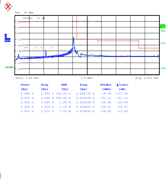
Band41_15MHz_16QAM_41165_1RB#74
