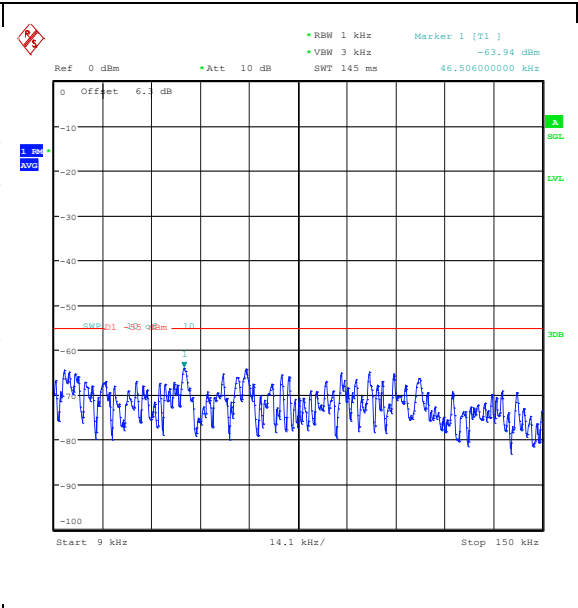
Band41(2535-2655)-5MHz-16QAM-41215-1RB#0-0.009~0.15-PASS
