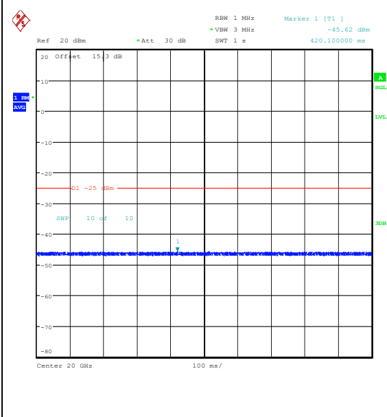
Band41(2535-2655)-5MHz-QPSK-40590-1RB#0-20000~27000-PASS
