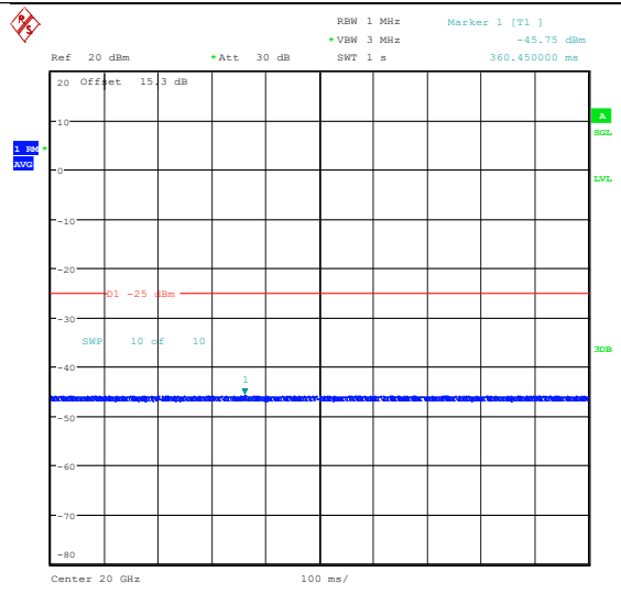
Band41(2535-2655)-15MHz-16QAM-41165-1RB#0 -20000~27000-PASS
