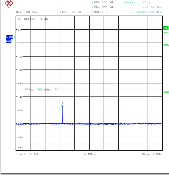
Band41(2535-2655)-5MHz-QPSK-41215-1RB#0-0.30~1000-PASS
