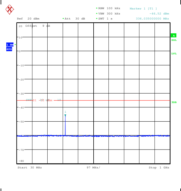
Band41(2535-2655)-5MHz-16QAM-41215-1RB#0-30~1000-PASS
