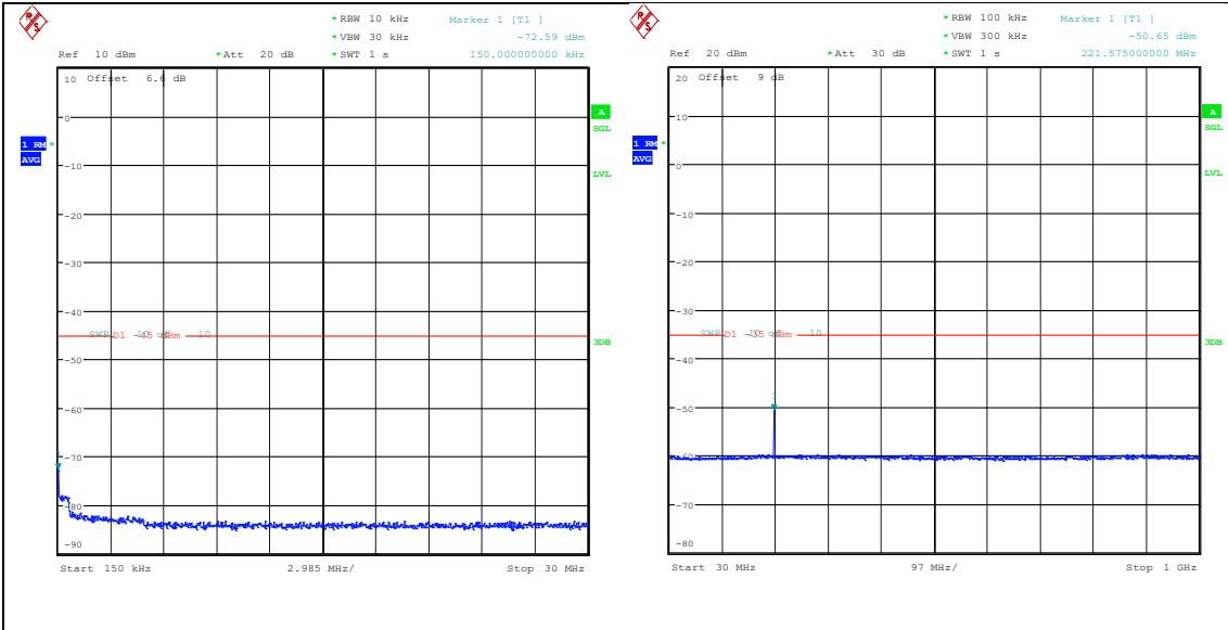
Band41(2535-2655)-20MHz-16QAM-40140-1RB# 0-0.15~30-PASS Band41(2535-2655)-20MHz-16QAM-40140-1RB# -30~1000-PASS
