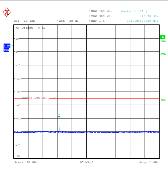
Band41(2535-2655)-10MHz-16QAM-41190-1RB#0 -30~1000-PASS
