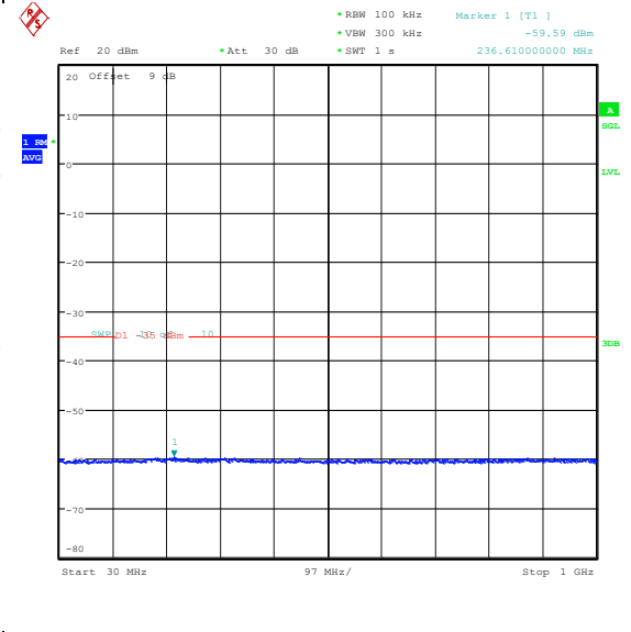
Band41(2535-2655)-15MHz-16QAM-40115-1RB#0-30~1000-PASS
