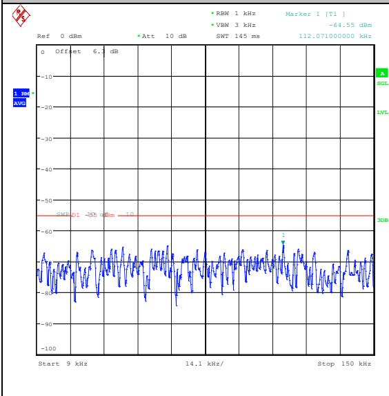
Band41(2535-2655)-10MHz-QPSK-40090-1RB#0 -0.009~0.15-PASS
