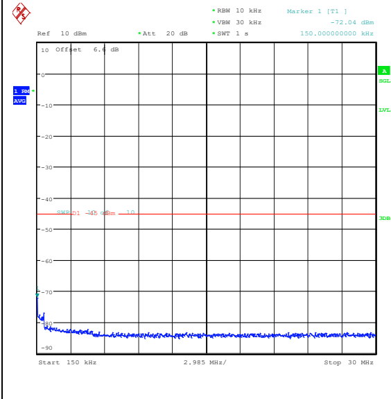
Band41(2535-2655)-15MHz-16QAM-40115-1RB#0-0.15~30-PASS
