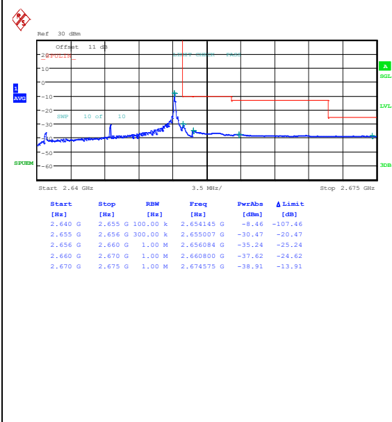
Band41_15MHz_QPSK_41165_1RB#74
