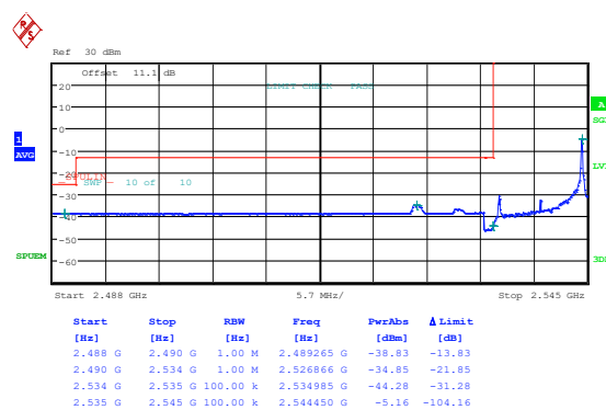
Band41_10MHz_16QAM_40090_1RB#0
