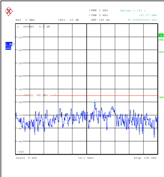
Band41(2535-2655)-20MHz-QPSK-40590-1RB#0 -0.009~0.15-PASS
