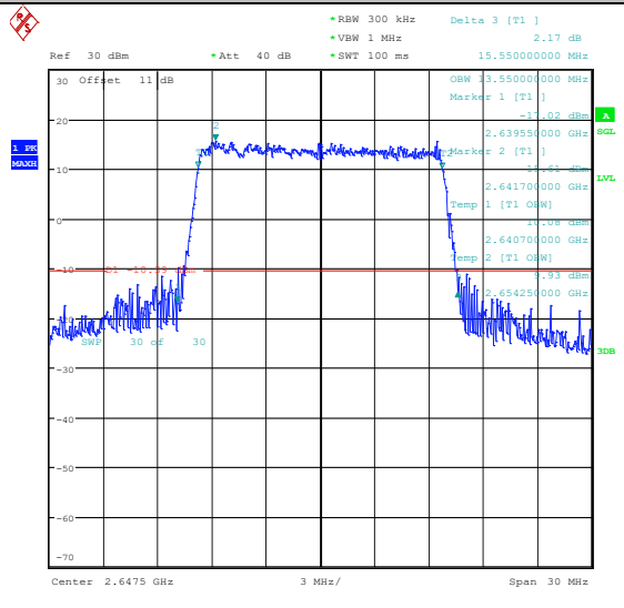
Band41(2535-2655)-15MHz-16QAM-41165-75RB#
