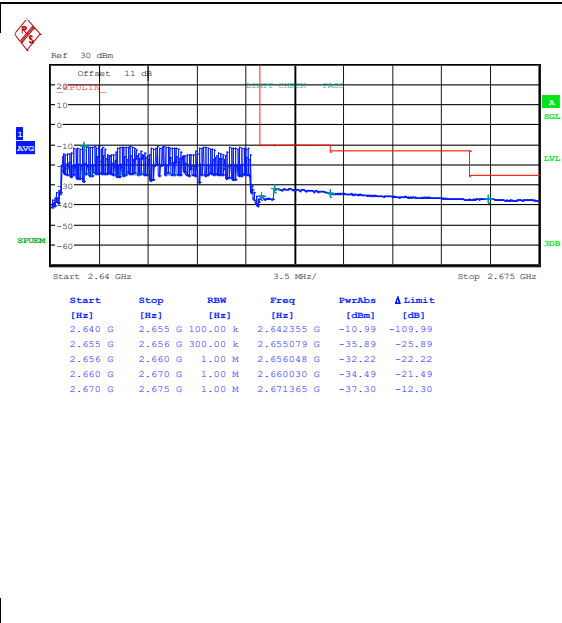
Band41_15MHz_16QAM_41165_75RB#0
