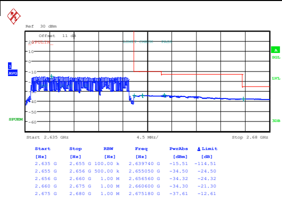
Band41_20MHz_16QAM_41140_1RB#99
