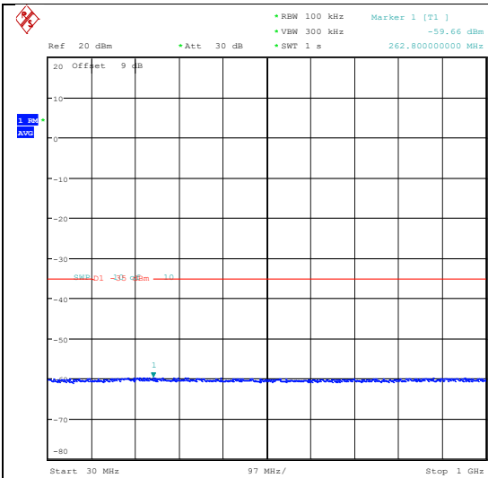
Band41(2535-2655)-15MHz-QPSK-40590-1RB#0 -30~1000-PASS
