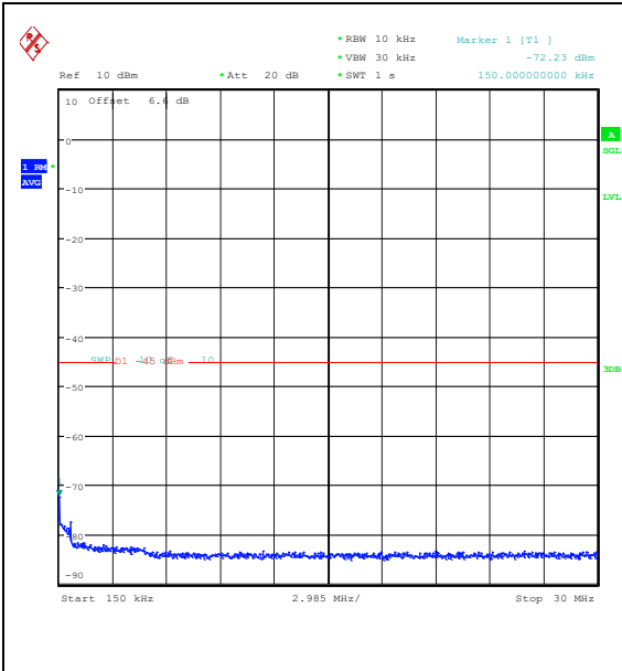
Band41(2535-2655)-10MHz-16QAM-41190-1RB#0 0-0.15~30-PASS
