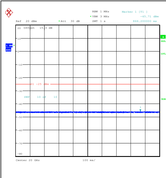
Band41(2535-2655)-15MHz-QPSK-41165-1RB#0-20000~27000-PASS
