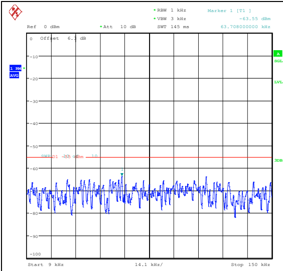
Band41(2535-2655)-15MHz-QPSK-41165-1RB#0-0.009~0.15-PASS
