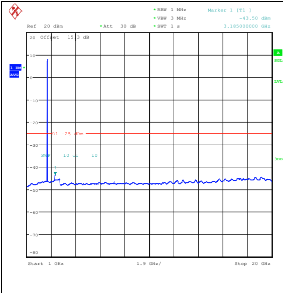
Band41(2535-2655)-10MHz-16QAM-40590-1RB# 0-1000-20000-PASS
