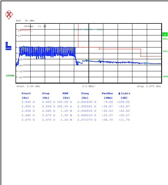
Band41_15MHz_QPSK_41165_75RB#0
