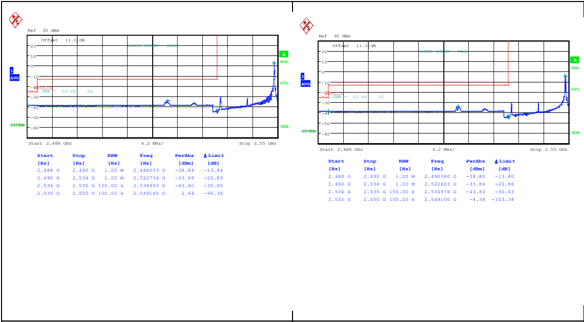
Band41_15MHz_QPSK_40115_1RB#74 Band41_15MHz_16QAM_40115_1RB#74
