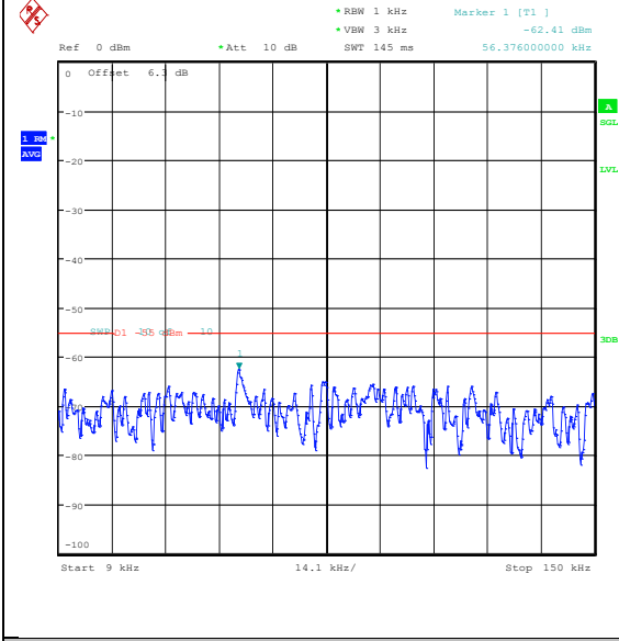
Band41(2535-2655)-10MHz-QPSK-41190-1RB#0- 0.009-0.15-PASS
