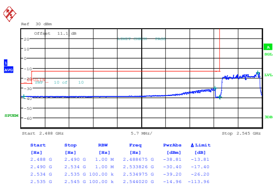
Band41_10MHz_QPSK_40090_1RB#49
