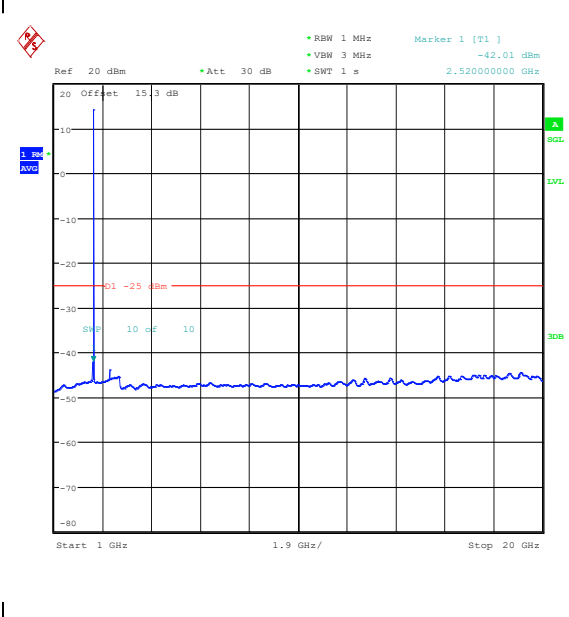
Band41(2535-2655)-5MHz-QPSK-40065-1RB#0-1000~20000-PASS
