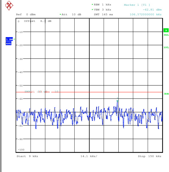
Band41(2535-2655)-15MHz-QPSK-40590-1RB#0-0.009~0.15-PASS
