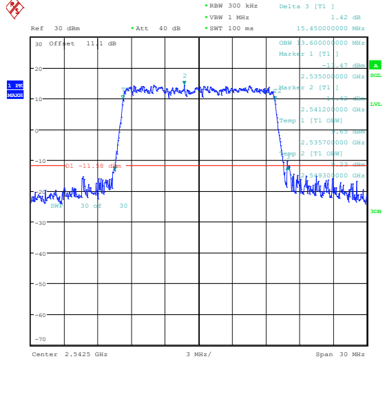
Band41(2535-2655)-15MHz-16QAM-40115-75RB# 0-PASS
