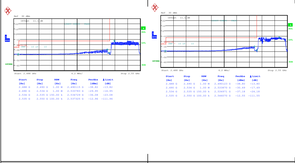
Band41_15MHz_QPSK_40115_75RB#0 Band41_15MHz_16QAM_40115_75RB#0
