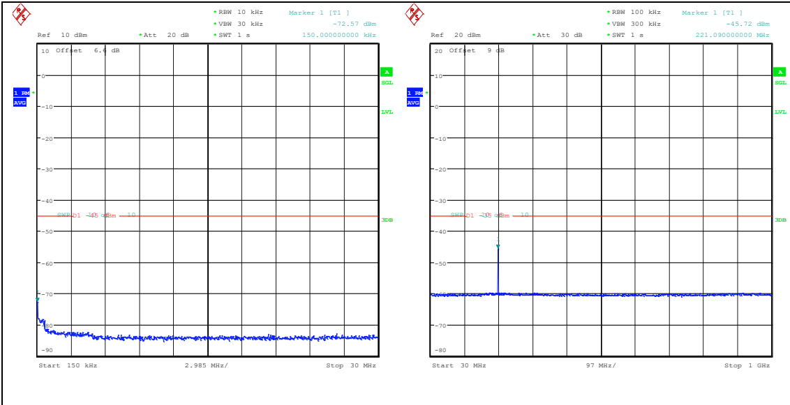
Band41(2535-2655)-10MHz-16QAM-40090-1RB# 0-0.15~30-PASS Band41(2535-2655)-10MHz-16QAM-40090-1RB#0 -30~1000-PASS
