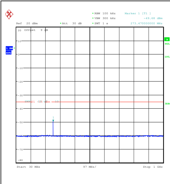
Band41(2535-2655)-5MHz-QPSK-40590-1RB#0-30~1000-PASS
