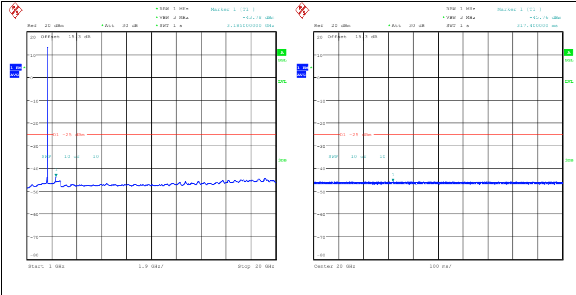
Band41(2535-2655)-5MHz-16QAM-40065-1RB#0 -1000~20000-PASS
