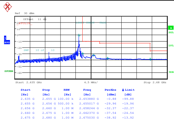
Band41_20MHz_QPSK_41140_1RB#0
