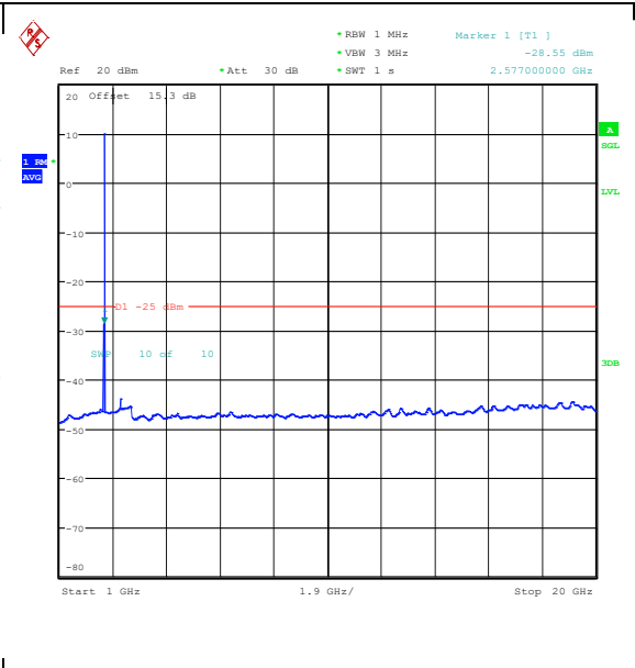
Band41(2535-2655)-5MHz-QPSK-40590-1RB#0-000~20000-PASS
