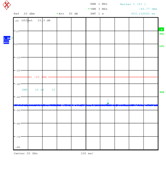
Band41(2535-2655)-20MHz-16QAM-41140-1RB#0 -20000~27000-PASS
