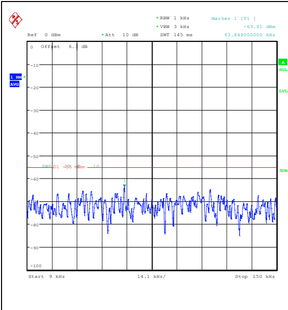
Band41(2535-2655)-10MHz-QPSK-40590-1RB#0 -0.009~0.15-PASS
