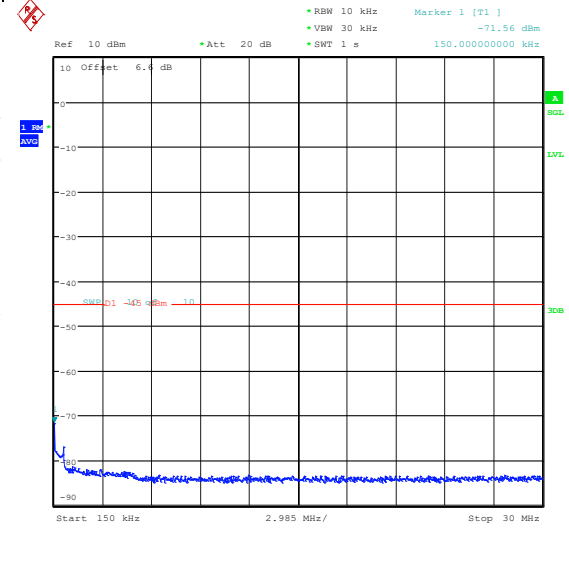
Band41(2535-2655)-15MHz-QPSK-40590-1RB#0-0.15~30-PASS
