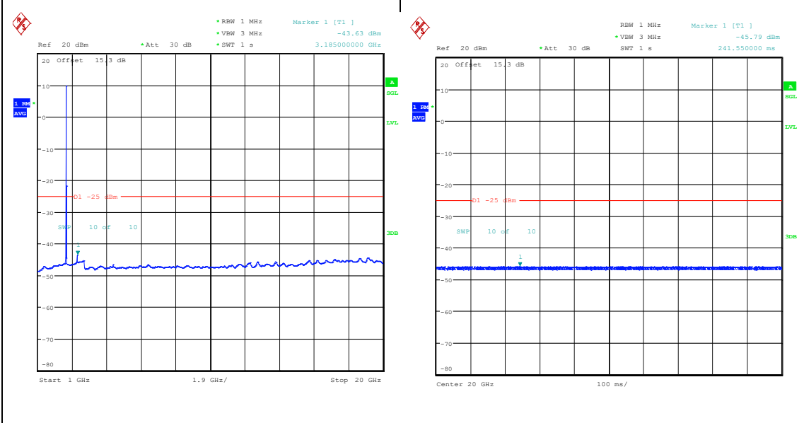
Band41(2535-2655)-15MHz-16QAM-40590-1RB# 0-1000~20000-PASS Band41(2535-2655)-15MHz-16QAM-40590-1RB#0 -20000~27000-PASS
