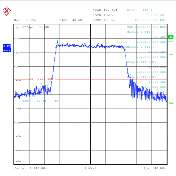
Band41(2535-2655)-20MHz-16QAM-41140-100RB #0-PASS
