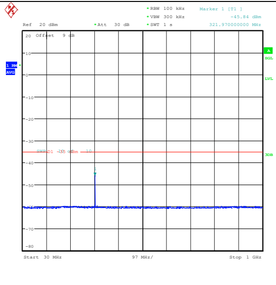
Band41(2535-2655)-20MHz-16QAM-41140-1RB#0 -30~1000-PASS
