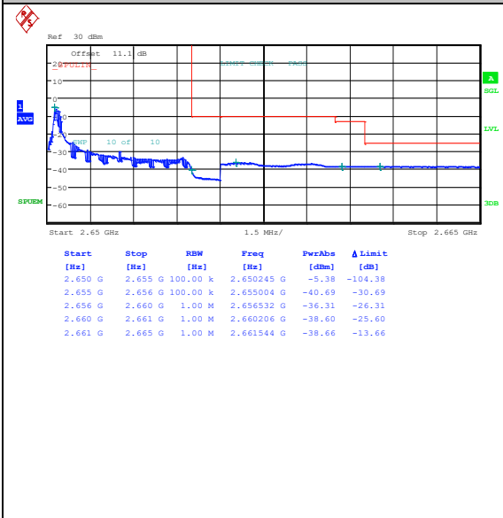
Band41_5MHz_QPSK_41215_1RB#0
