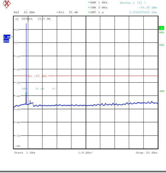
Band41(2535-2655)-5MHz-QPSK-41215-1RB#0-1.000~20000-PASS
