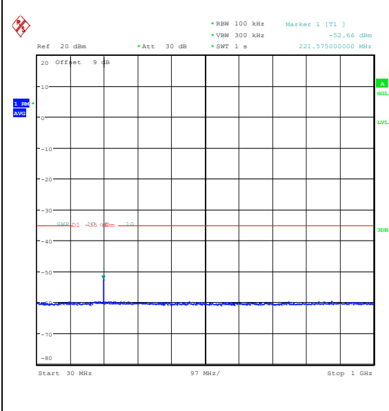
Band41(2535-2655)-15MHz-QPSK-40115-1RB#0-30~1000-PASS
