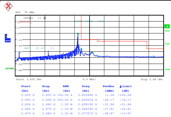
Band41_20MHz_16QAM_41140_1RB#0
