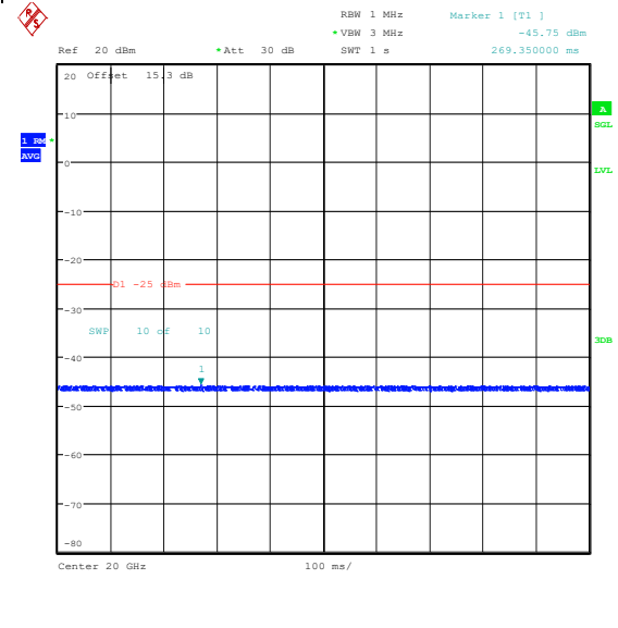
Band41(2535-2655)-5MHz-16QAM-40590-1RB#0- 20000~27000-PASS
