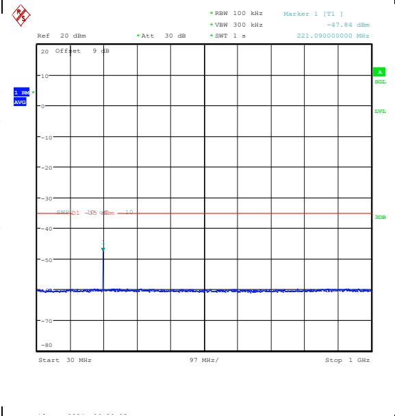
Band41(2535-2655)-5MHz-16QAM-40065-1RB#0-30~1000-PASS
