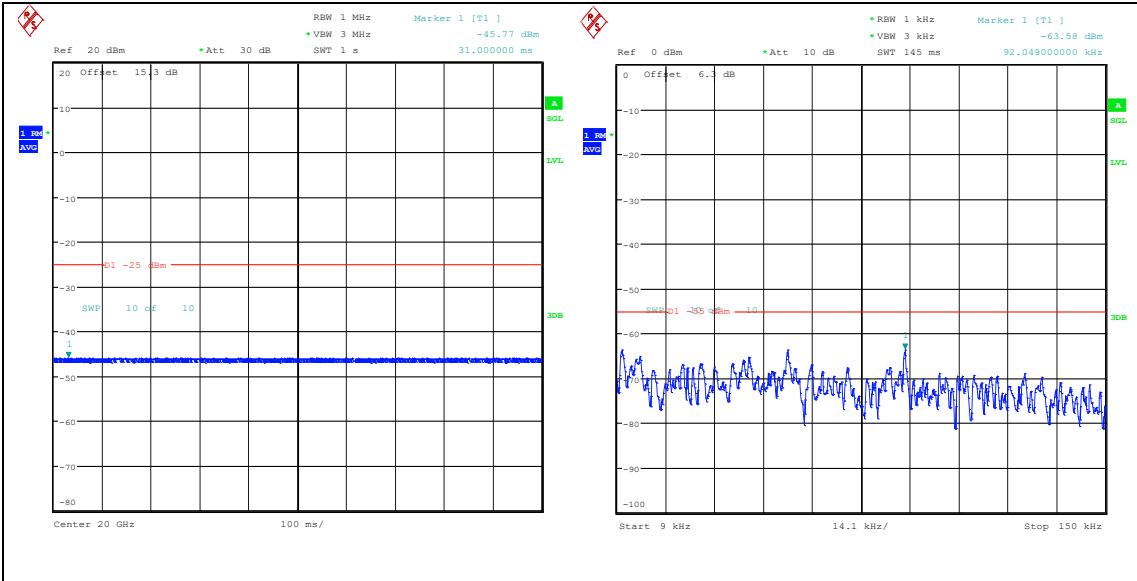
Band41(2535-2655)-15MHz-QPSK-40115-1RB#0-20000~27000-PASS
