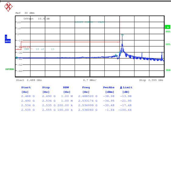
Band41_20MHz_16QAM_40140_1RB#0
