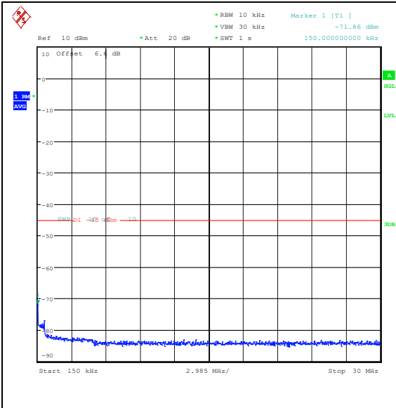
Band41(2535-2655)-20MHz-16QAM-41140-1RB# 0-0.15~30-PASS
