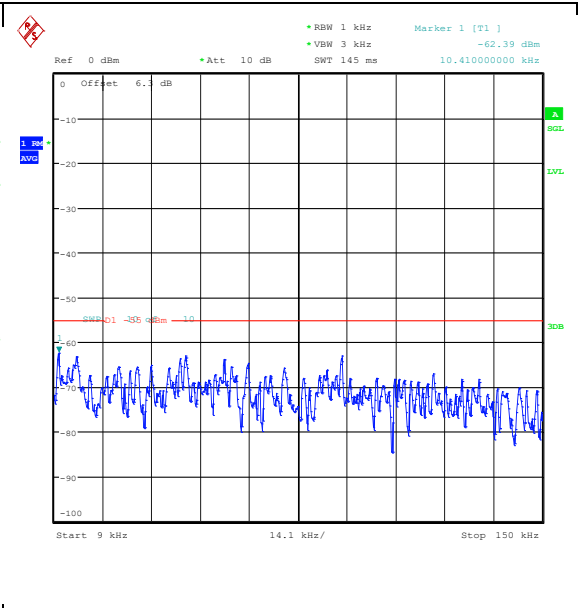
Band41(2535-2655)-15MHz-16QAM-41165-1RB#0-0.009~0.15-PASS
