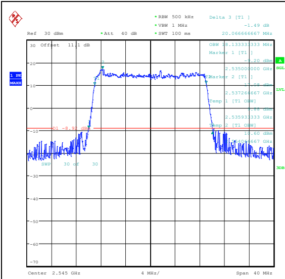
Band41(2535-2655)-20MHz-QPSK-40140-100RB #0-PASS
