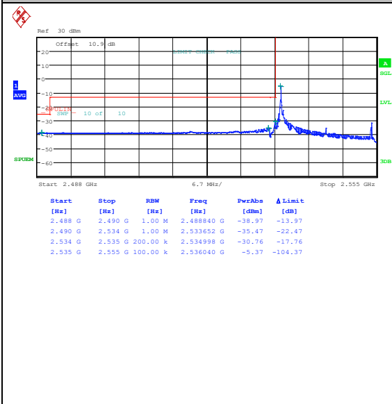
Band41_20MHz_QPSK_40140_1RB#0
