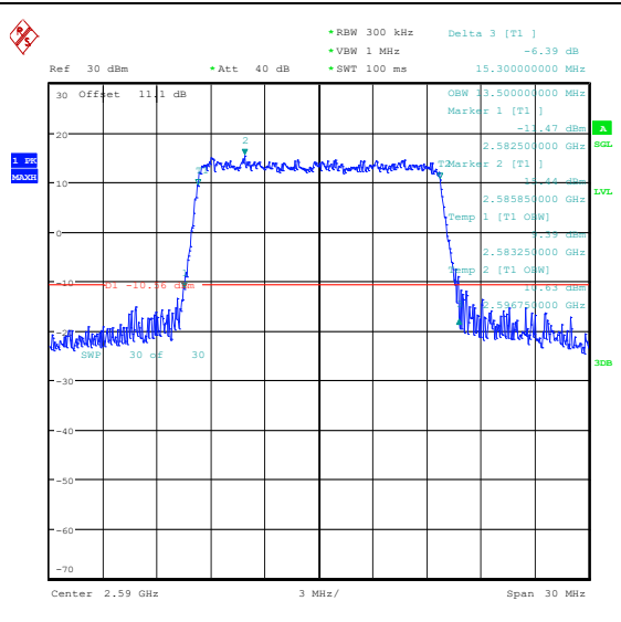
Band41(2535-2655)-15MHz-16QAM-40590-75RB#
