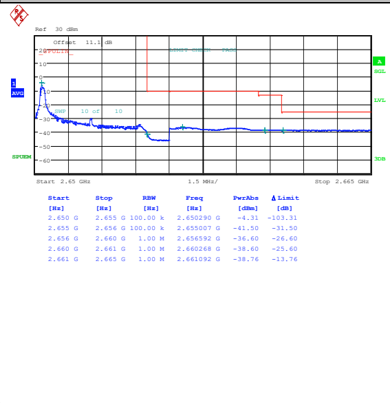
Band41_5MHz_16QAM_41215_1RB#0
