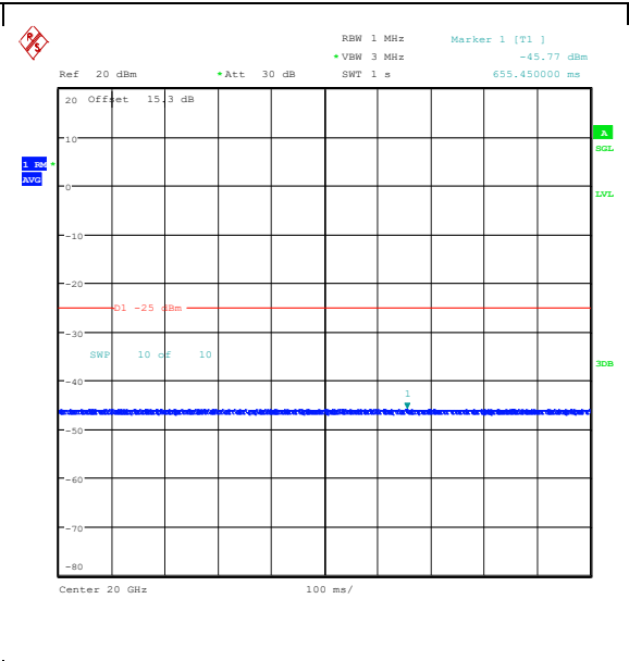
Band41(2535-2655)-20MHz-16QAM-40590-1RB#0 -20000~27000-PASS
