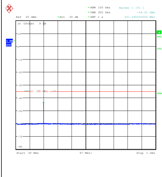
Band41(2535-2655)-5MHz-QPSK-40065-1RB#0-30~1000-PASS
