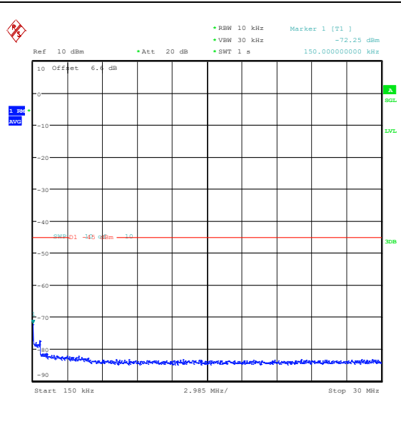
Band41(2535-2655)-5MHz-QPSK-41215-1RB#0-0.15~30-PASS
