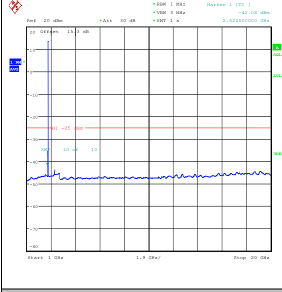
Band41(2535-2655)-10MHz-16QAM-41190-1RB#0 0-1000~20000-PASS
