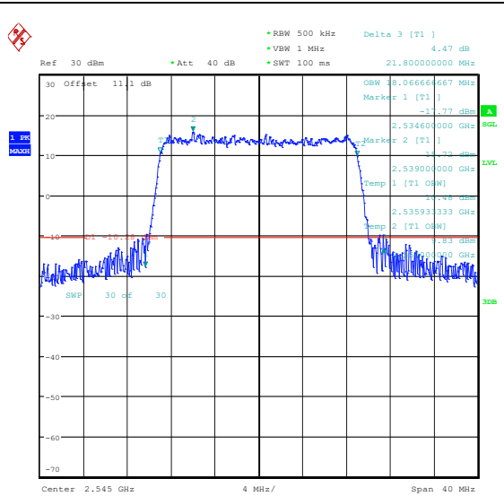
Band41(2535-2655)-20MHz-16QAM-40140-100RB #0-PASS
