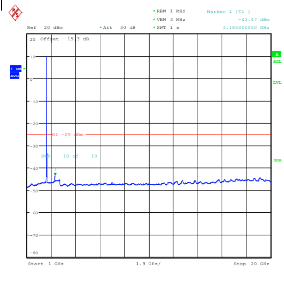
Band41(2535-2655)-15MHz-QPSK-40115-1RB#0-1000~20000-PASS
