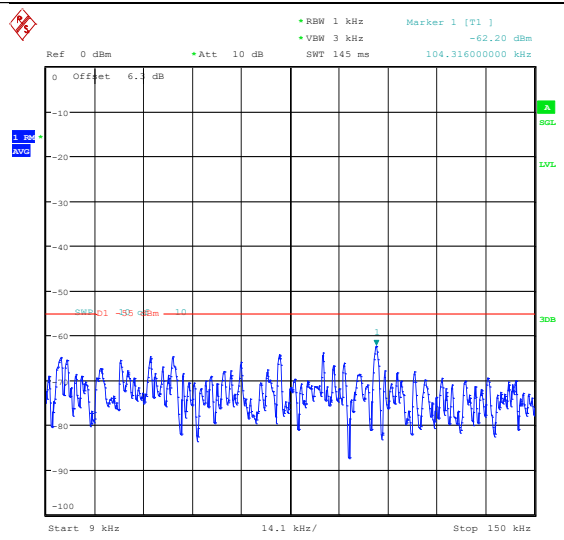
Band41(2535-2655)-20MHz-16QAM-40590-1RB#0 -0.009~0.15-PASS
