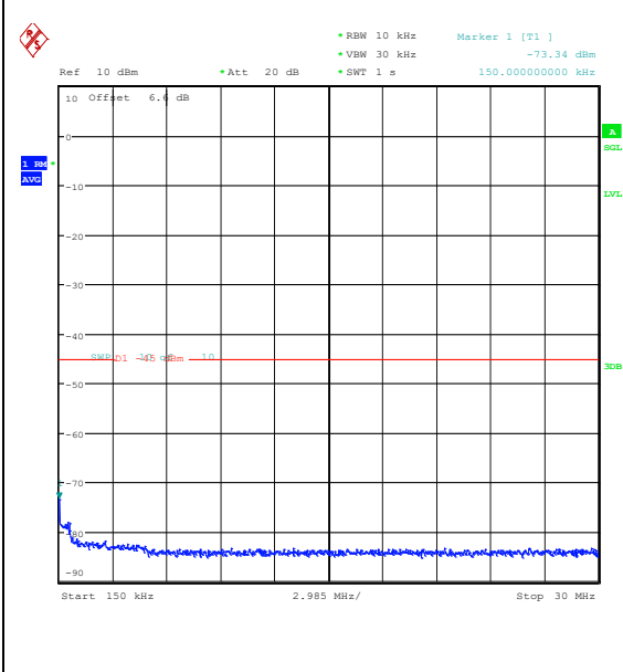
Band41(2535-2655)-5MHz-16QAM-40065-1RB#0-0.15~30-PASS
