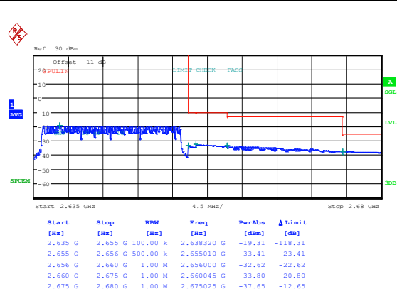
Band41_20MHz_QPSK_41140_1RB#99
