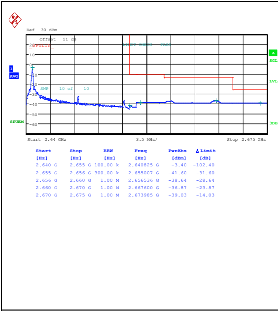
Band41_15MHz_QPSK_41165_1RB#0
