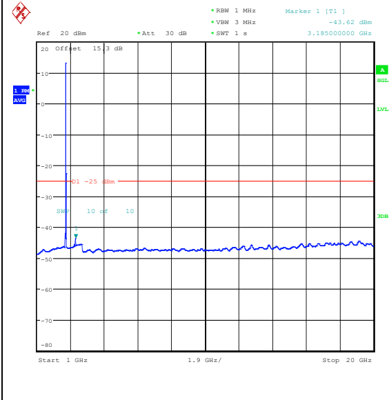
Band41(2535-2655)-20MHz-16QAM-41140-1RB# 0-1000~20000-PASS
