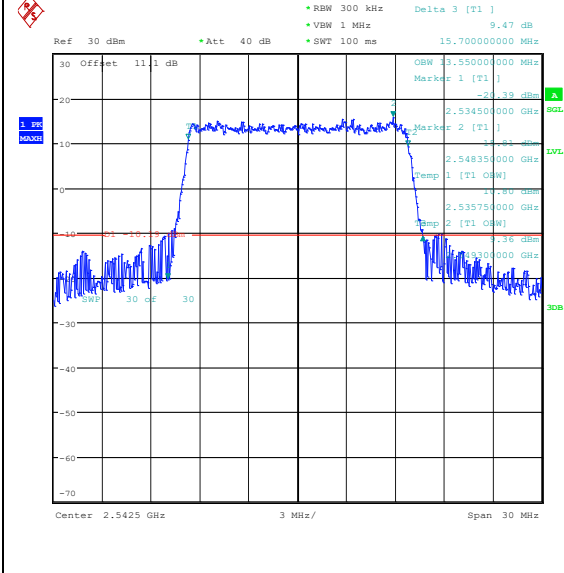
Band41(2535-2655)-15MHz-QPSK-40115-75RB# 0-PASS
