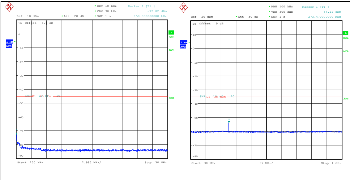
Band41(2535-2655)-5MHz-16QAM-40590-1RB#0 -0.15~30-PASS
