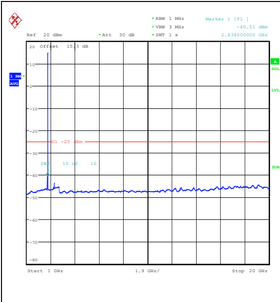
Band41(2535-2655)-5MHz-16QAM-41215-1RB#0 -1000~20000-PASS
