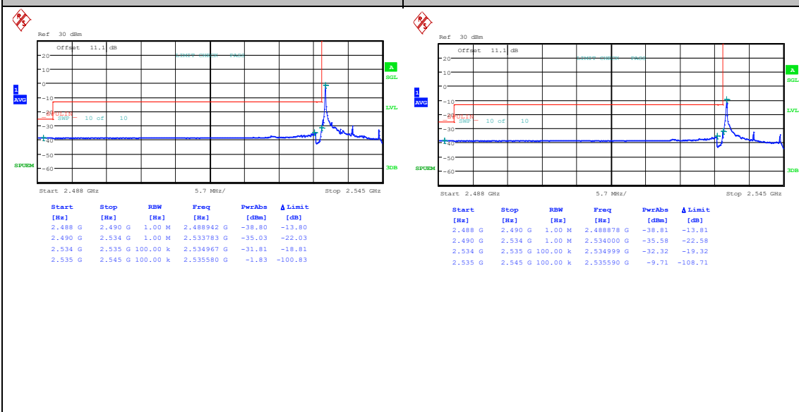
Band41_5MHz_QPSK_41215_25RB#0
