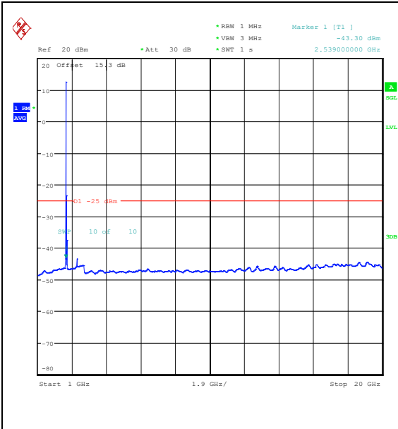
Band41(2535-2655)-20MHz-16QAM-40590-1RB# 0-1000~20000-PASS
