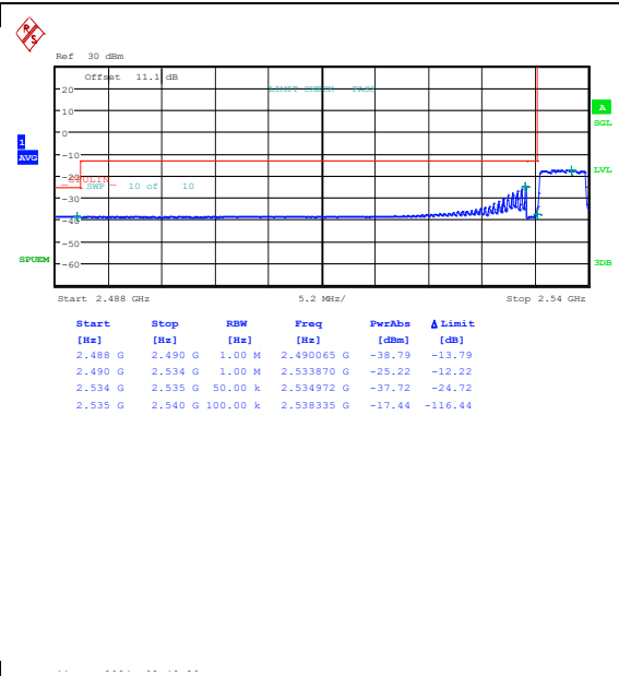
Band41_5MHz_16QAM_40065_25RB#0
