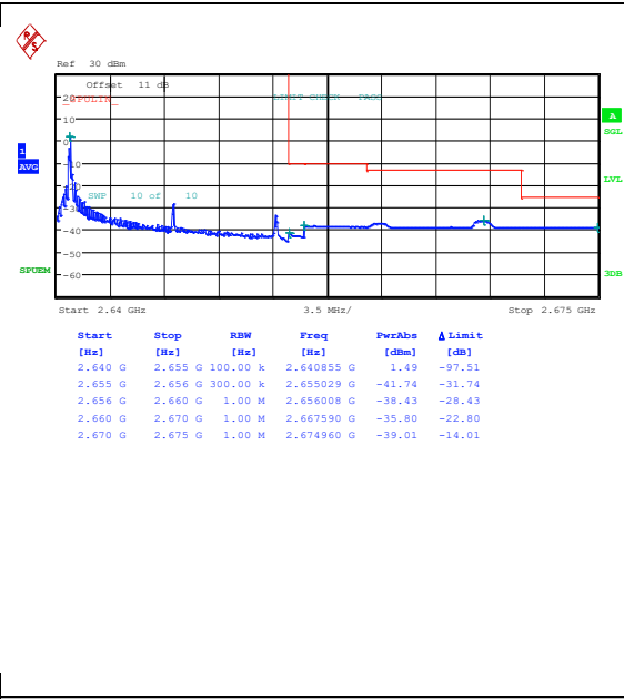
Band41_15MHz_16QAM_41165_1RB#0
