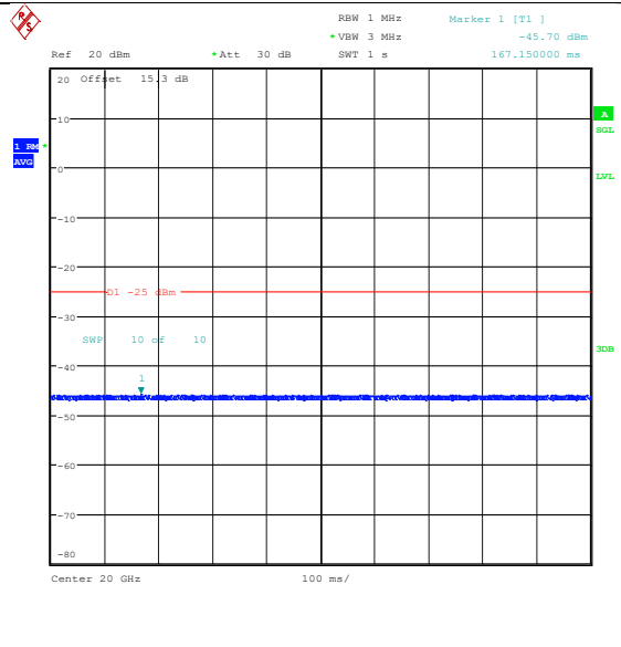
Band41(2535-2655)-10MHz-16QAM-40590-1RB# -20000-27000-PASS
