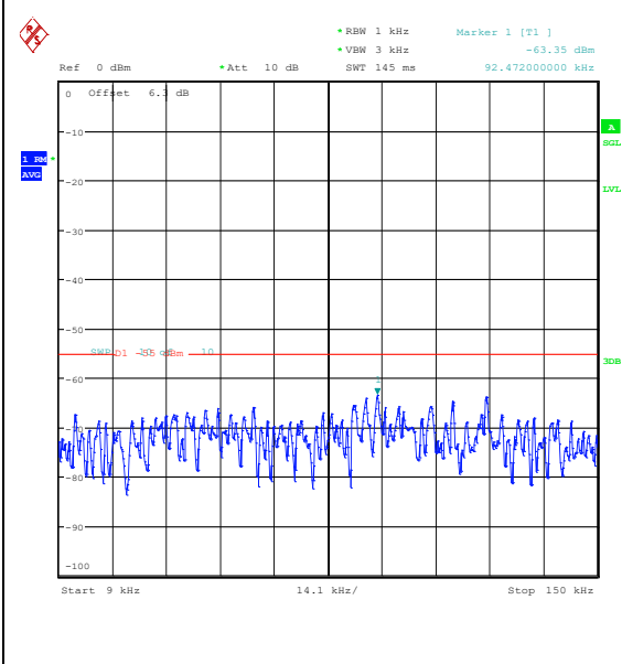
Band41(2535-2655)-5MHz-QPSK-40590-1RB#0- 0.009~0.15-PASS
