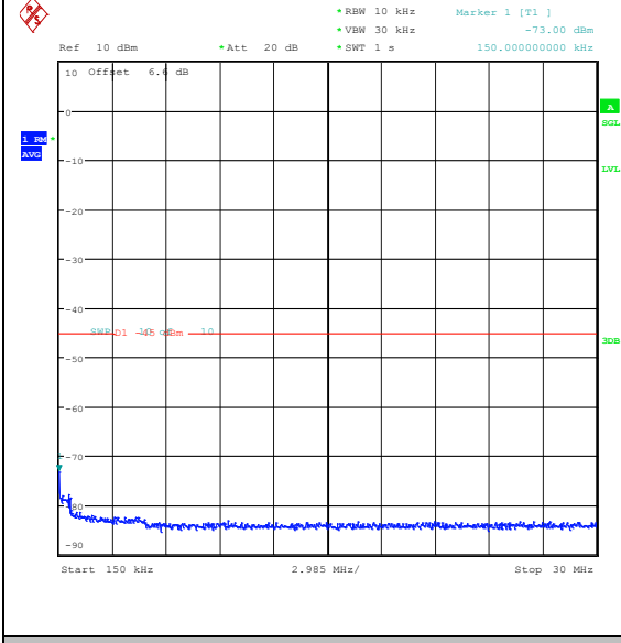
Band41(2535-2655)-10MHz-16QAM-40590-1RB#0 0-0.15~30-PASS
