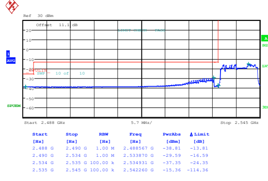
Band41_10MHz_16QAM_40090_1RB#49
