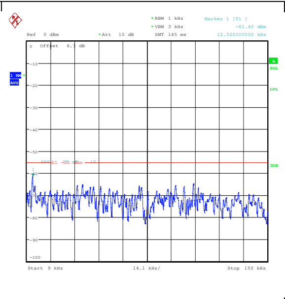
Band41(2535-2655)-10MHz-16QAM-40590-1RB#0 -0.009~0.15-PASS
