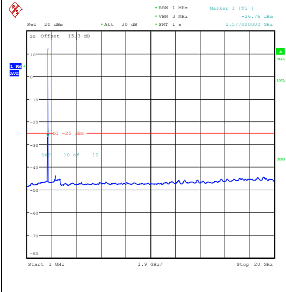
Band41(2535-2655)-5MHz-16QAM-40590-1RB#0 -1000~20000-PASS
