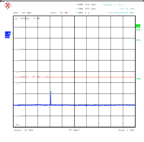
Band41(2535-2655)-15MHz-16QAM-41165-1RB#0-30~1000-PASS
