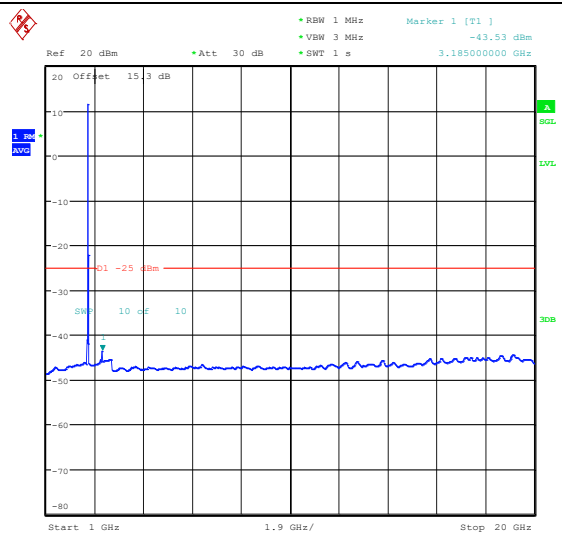
Band41(2535-2655)-20MHz-QPSK-41140-1RB#0-1000~20000-PASS
