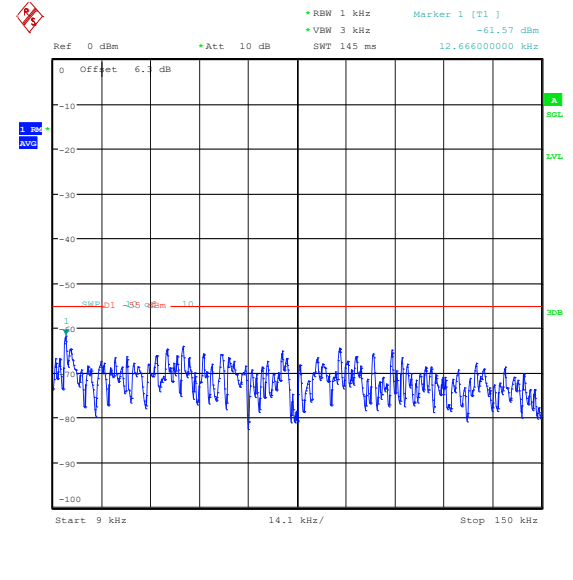
Band41(2535-2655)-10MHz-16QAM-41190-1RB#0-0.009~0.15-PASS
