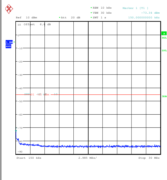
Band41(2535-2655)-5MHz-16QAM-41215-1RB#0-0.15~30-PASS
