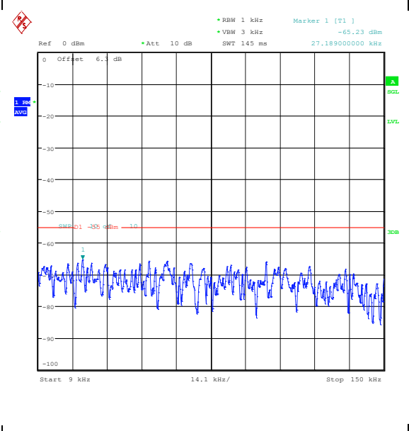
Band41(2535-2655)-5MHz-16QAM-40590-1RB#0-0.009~0.15-PASS
