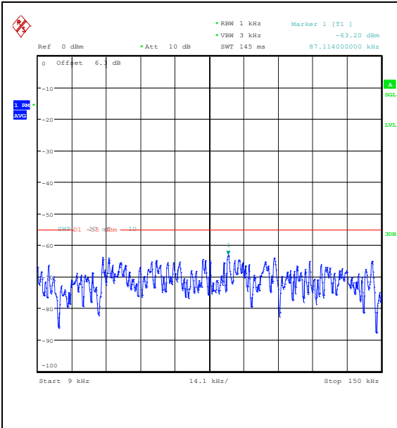
Band41(2535-2655)-5MHz-QPSK-41215-1RB#0-0.009~0.15-PASS
