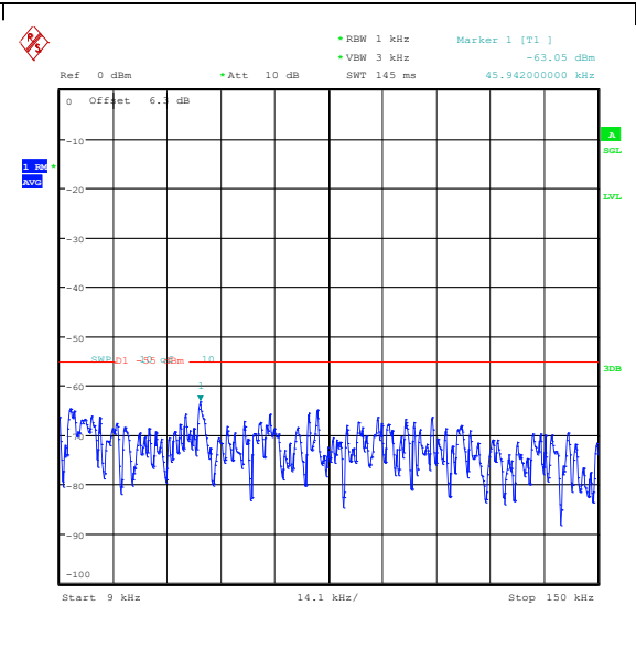
Band41(2535-2655)-5MHz-16QAM-40065-1RB#0-0.009~0.15-PASS
