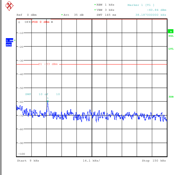
Band26_1.4MHz_QPSK_27033_1RB#0_0.009~0.15_0.009~0.15
