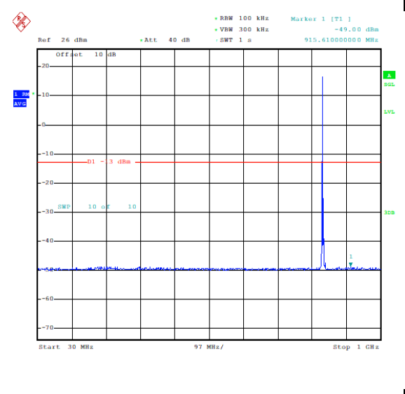
Band26_5MHz_16QAM_26915_1RB#0_30~1000_30~1000
