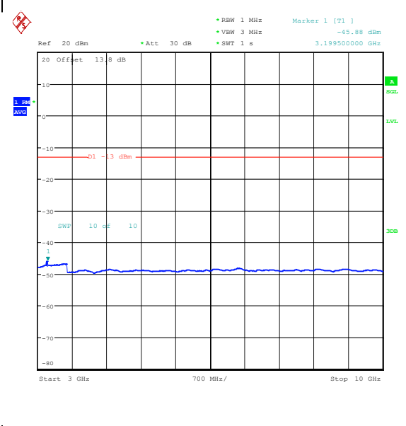
Band26_1.4MHz_16QAM_26915_1RB#5_3000~1 0000_3000~10000
