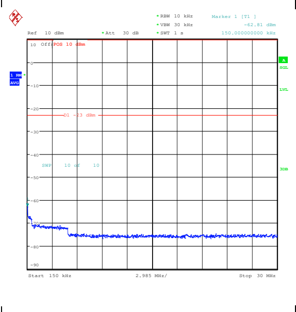
Band26_5MHz_QPSK_27015_1RB#0_0.15~30_0.15~30
