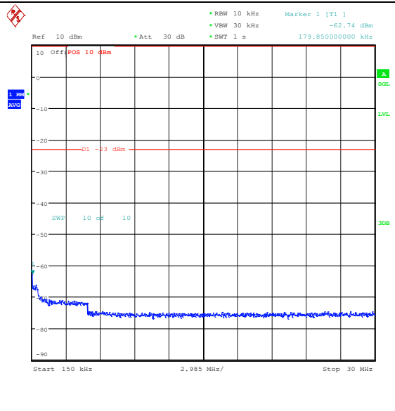
Band26_1.4MHz_QPSK_26915_6RB#0_0.15~30_0.15~30
