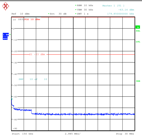
Band26_3MHz_QPSK_27025_1RB#0_0.15~30_0_15~30
