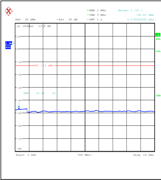
Band26_3MHz_QPSK_26915_1RB#14_3000~10000_3000~10000
