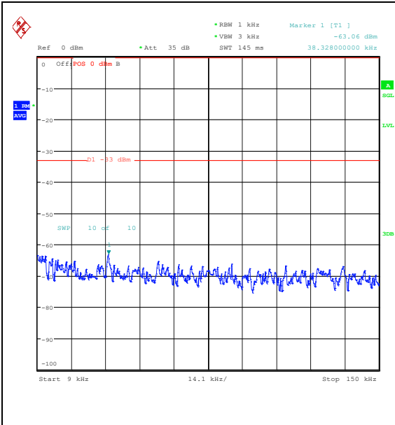
Band26_3MHz_QPSK_26805_1RB#0_0.009~0.15_5_0.009~0.15
