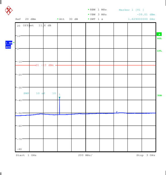
Band26_10MHz_QPSK_26740_1RB#0_1000~3000_0_1000~3000
