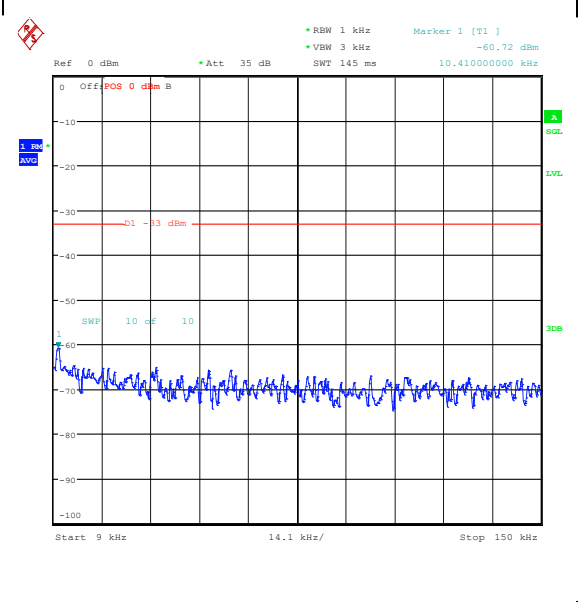
Band26_1.4MHz_16QAM_26915_1RB#5_0.009~0.15_0.009~0.15
