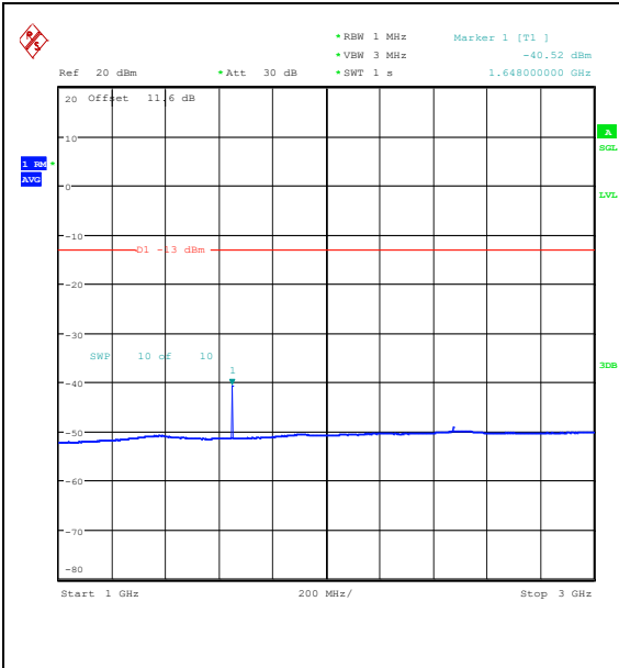
Band26_3MHz_16QAM_26805_1RB#0_1000~3000_00_1000~3000
