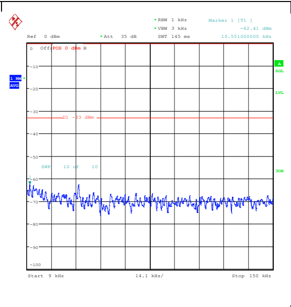
Band26_1.4MHz_16QAM_26915_6RB#0_0.009~0.15_0.009~0.15
