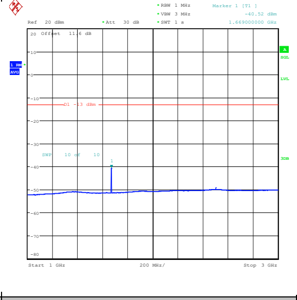
Band26_5MHz_QPSK_26915_1RB#0_1000~3000_1000~3000
