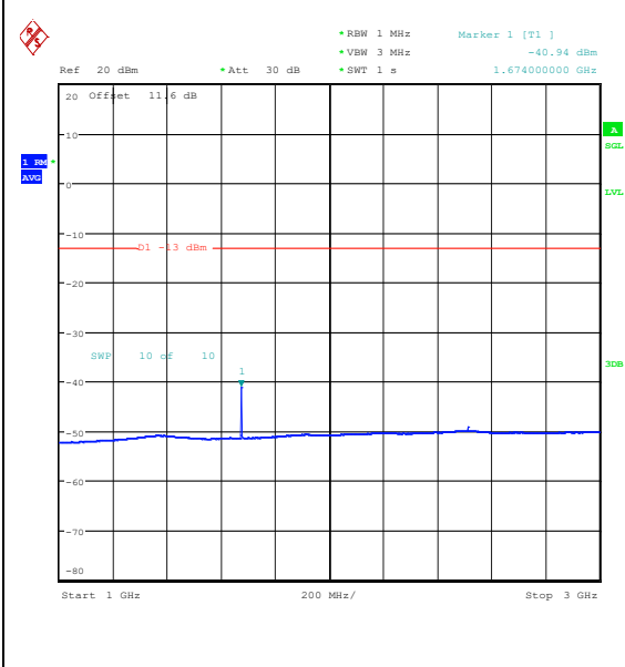
Band26_1.4MHz_16QAM_26915_1RB#5_1000~ 3000_1000~3000
