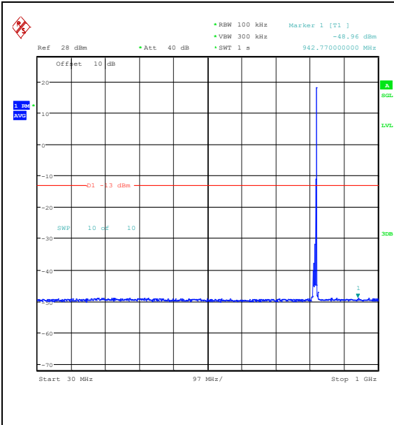
Band26_10MHz_QPSK_26740_1RB#49_30~100 0_30~1000
