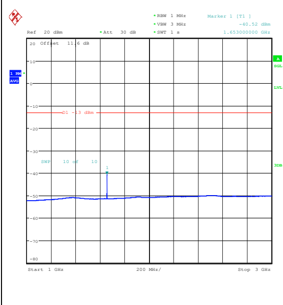
Band26_3MHz_16QAM_26805_1RB#14_1000~3 000_1000~3000
