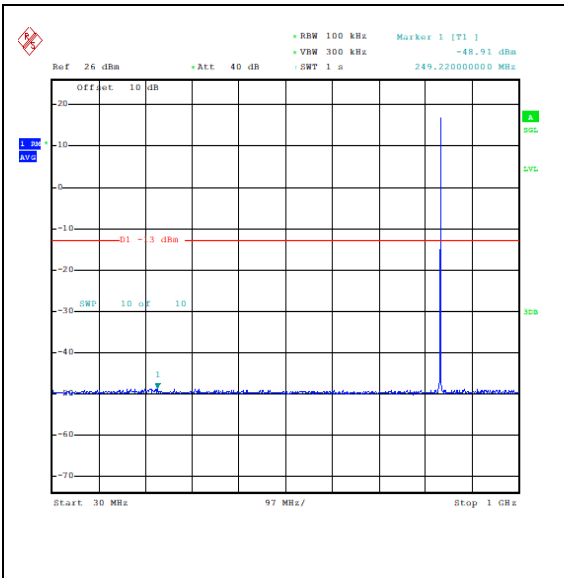
Band26_1.4MHz_QPSK_26915_1RB#5_30~1000_30~1000
