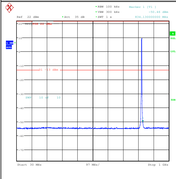
Band26_3MHz_QPSK_26805_15RB#0_30~1000_30~1000
