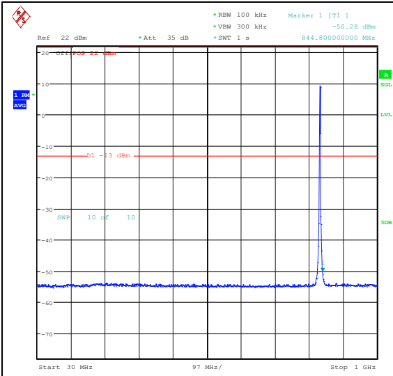
Band26_3MHz_QPSK_26915_15RB#0_30~1000_30~1000
