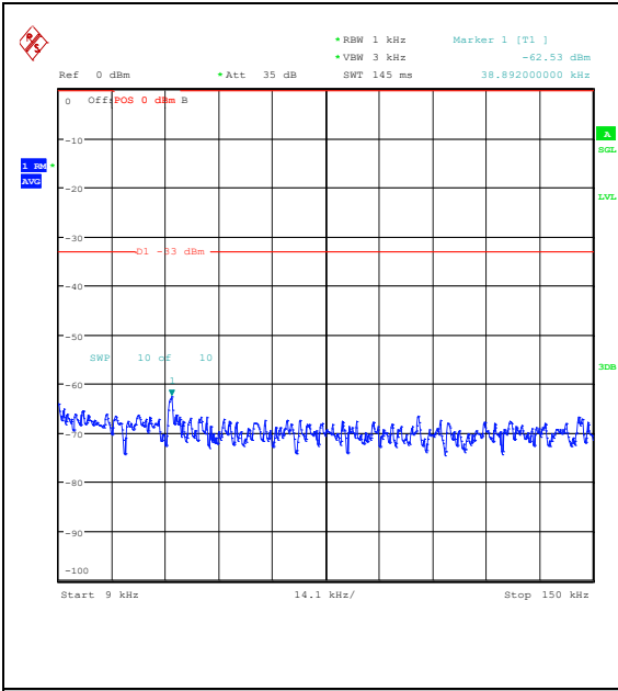
Band26_1.4MHz_QPSK_26797_1RB#5_0.009~0.15_0.009~0.15
