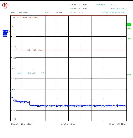
Band26_3MHz_QPSK_26915_1RB#14_0.15~30_0.15~30
