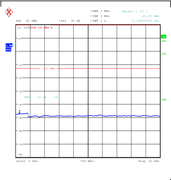
Band26_5MHz_16QAM_26915_25RB#0_3000~10000_3000~10000
