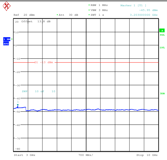
Band26_5MHz_16QAM_26815_1RB#24_3000~10000_3000~10000
