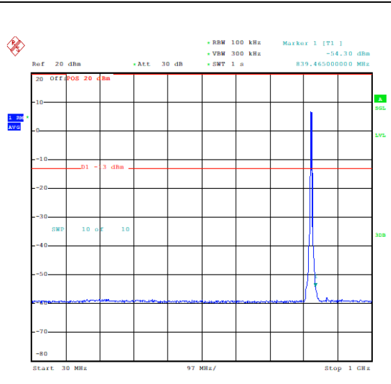
Band26_5MHz_16QAM_26815_25RB#0_30~1000 _30~1000
