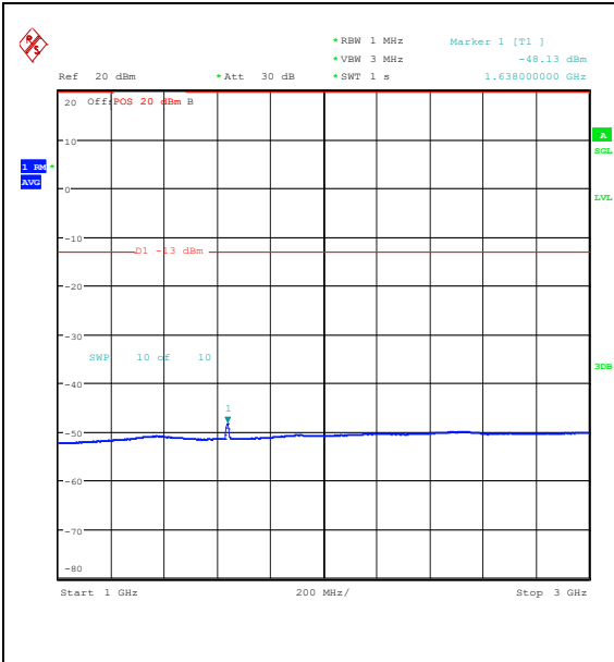
Band26_10MHz_16QAM_26740_50RB#0_1000~3000_1000~3000
