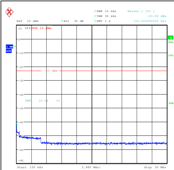
Band26_5MHz_16QAM_26815_25RB#0_0.15~3 0_0.15~30
