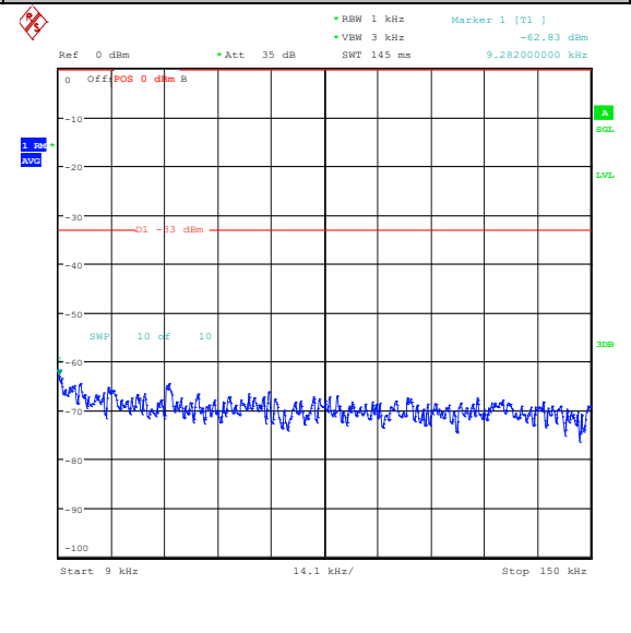
Band26_5MHz_16QAM_26815_1RB#0_0.009~0.15_5_0.009~0.15
