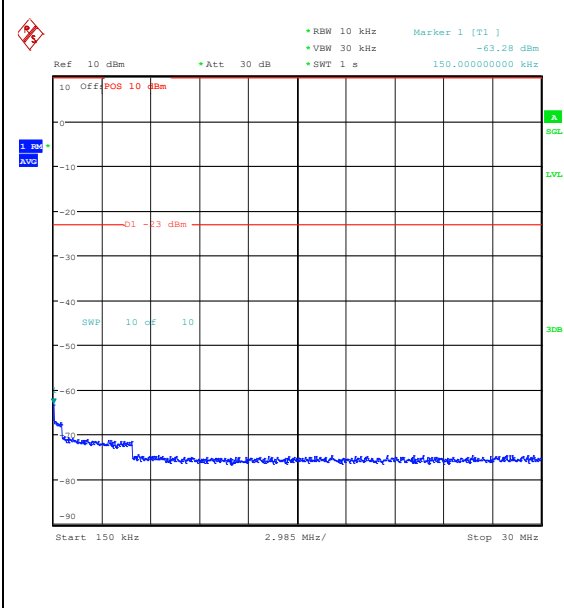
Band26_1.4MHz_16QAM_26797_1RB#5_0.15~30_0.15~30
