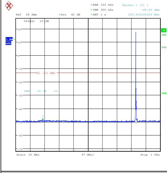
Band26_5MHz_QPSK_26915_1RB#0_30~1000_30~1000
