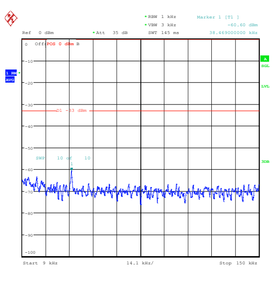
Band26_1.4MHz_16QAM_27033_6RB#0_0.009~0.15_0.009~0.15
