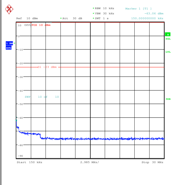
Band26_1.4MHz_16QAM_26915_6RB#0_0.15~30_0.15~30
