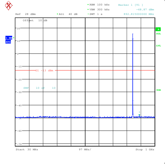
Band26_3MHz_16QAM_27025_1RB#0_30~1000_30~1000
