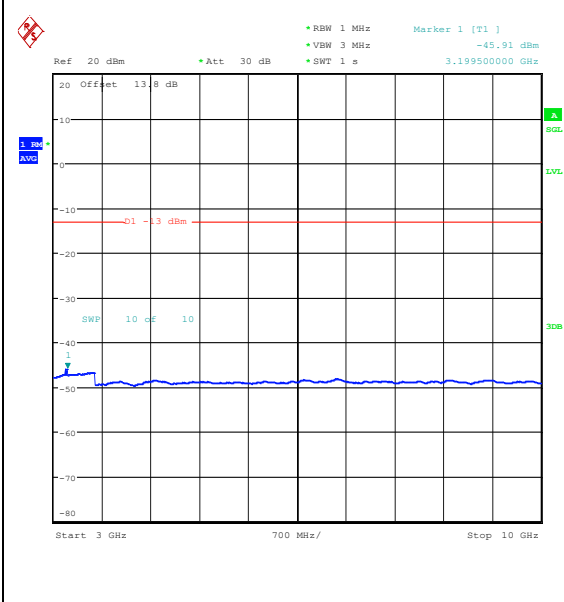
Band26_1.4MHz_QPSK_26915_1RB#5_3000~10000_00_3000~10000
