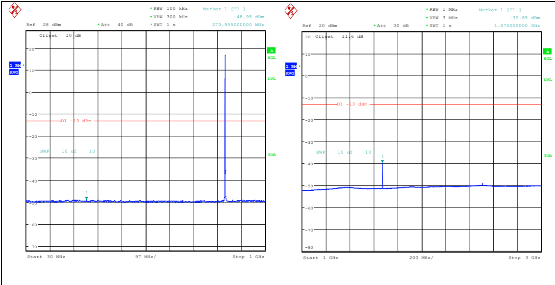
Band26_3MHz_QPSK_26915_1RB#0_30~1000_30~1000
