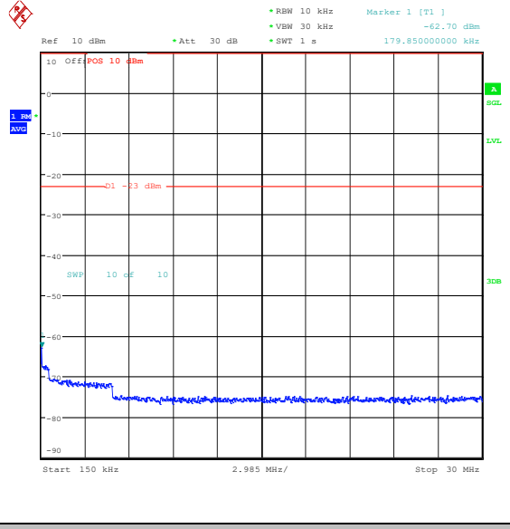
Band26_1.4MHz_QPSK_26915_1RB#5_0.15~30_0.15~30
