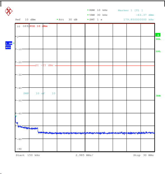
Band26_3MHz_QPSK_26805_15RB#0_0.15~30_0.15~30
