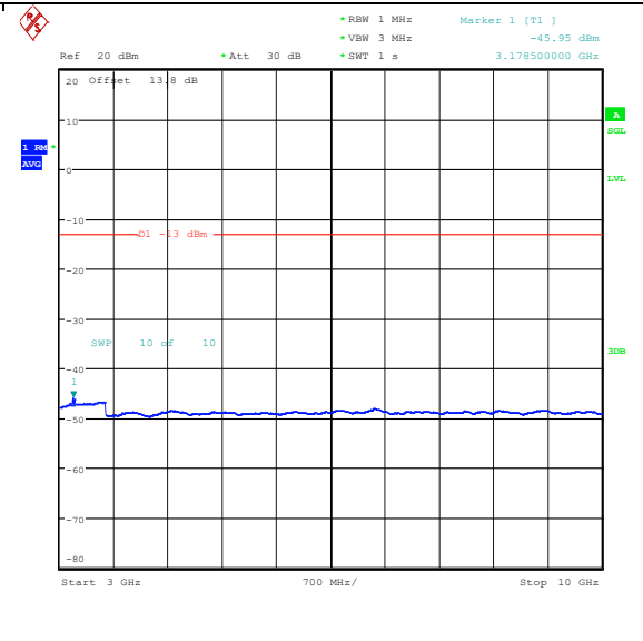
Band26_3MHz_16QAM_26915_1RB#14_3000~10000_3000~10000
