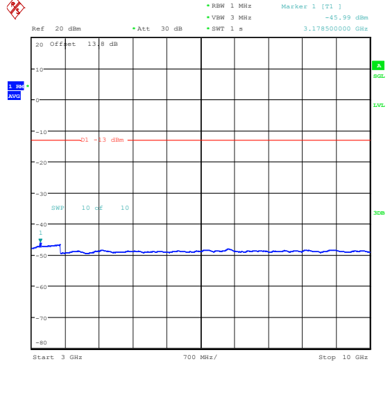
Band26_5MHz_16QAM_26915_1RB#24_3000~10 000_3000~10000
