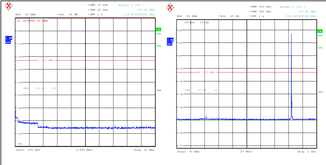
Band26_5MHz_16QAM_26815_1RB#0_0.15~30_0.15~30 Band26_5MHz_16QAM_26815_1RB#0_30~1000_30~1000
