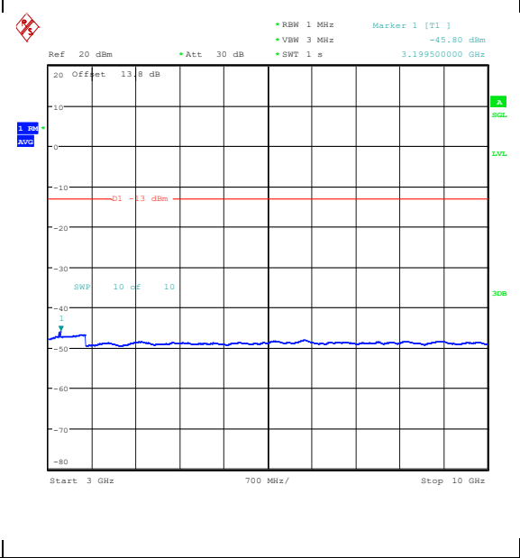
Band26_5MHz_16QAM_27015_1RB#0_3000~10000_3000~10000
