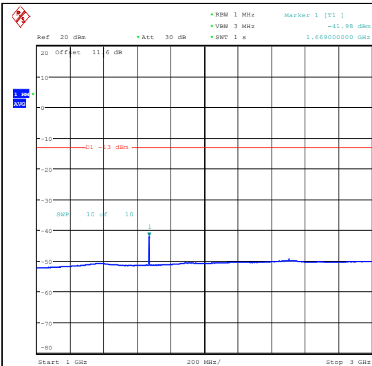
Band26_5MHz_16QAM_26915_1RB#0_1000~3000_1000~3000
