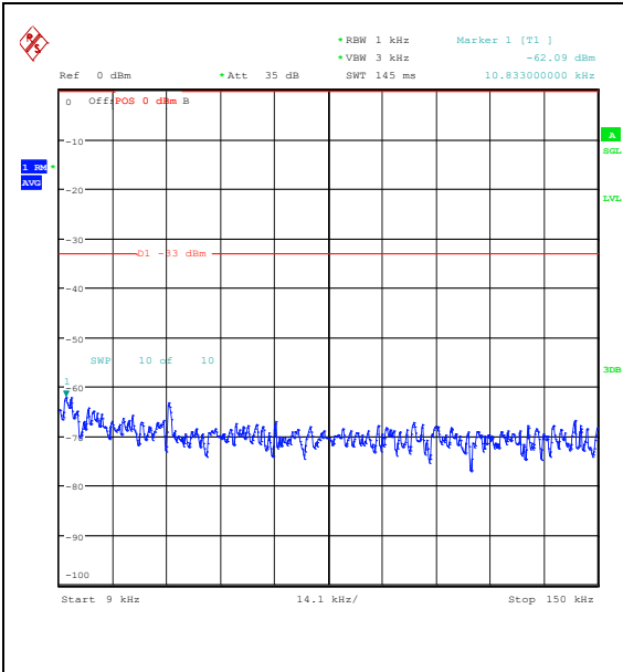
Band26_3MHz_QPSK_26805_15RB#0_0.009~0.15_0.009~0.15
