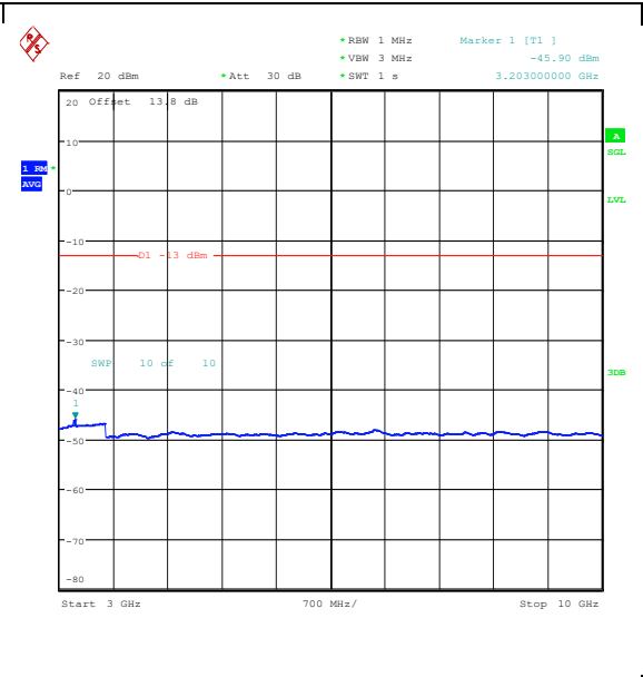
Band26_10MHz_16QAM_26740_1RB#0_3000~10000_3000~10000
