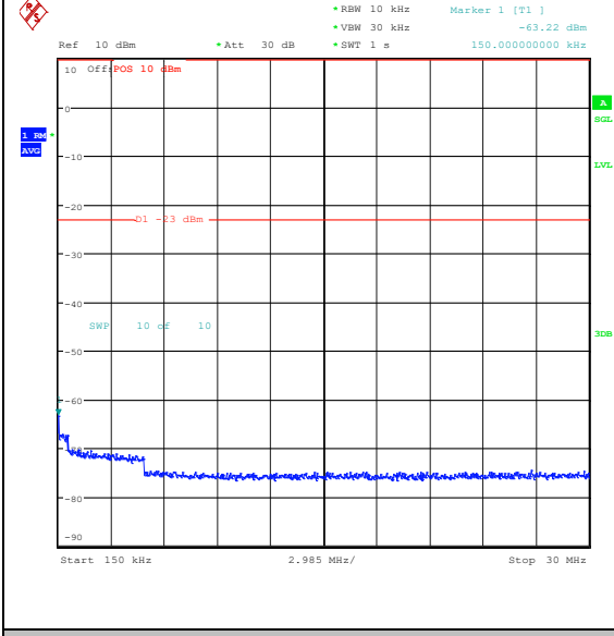
Band26_5MHz_16QAM_26915_25RB#0_0.15~3_0.15~30
