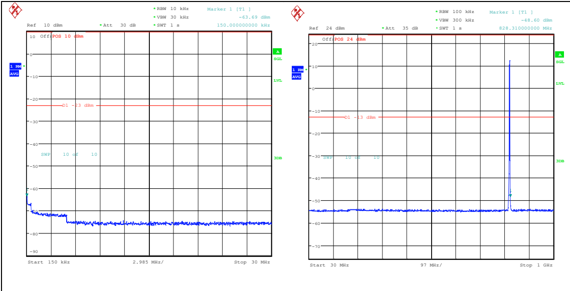
Band26_1.4MHz_16QAM_26797_6RB#0_0.15~3 0_0.15~30
