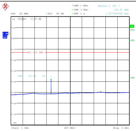
Band26_5MHz_QPSK_26915_1RB#24_1000~3000_0_1000~3000
