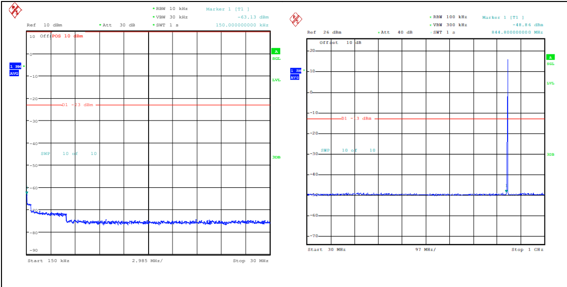
Band26_1.4MHz_16QAM_27033_1RB#0_0.15~3 0_0.15~30
