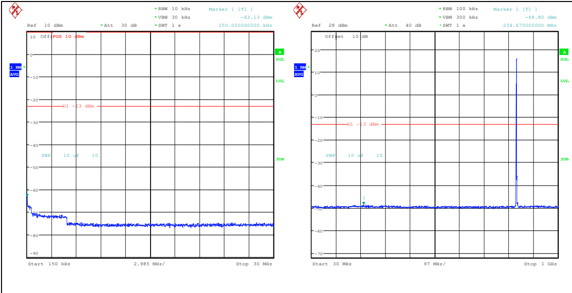
Band26_3MHz_16QAM_26915_1RB#0_0.15~30_0.15~30 Band26_3MHz_16QAM_26915_1RB#0_30~1000_30~1000
