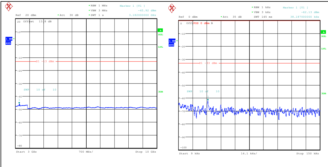
Band26_5MHz_QPSK_26815_1RB#24_3000~10000_3000~10000 Band26_5MHz_16QAM_26815_1RB#24_0.009~0.15_0.009~0.15
