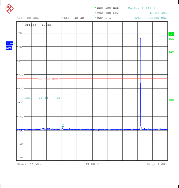
Band26_3MHz_16QAM_26805_1RB#0_30~1000_30~1000
