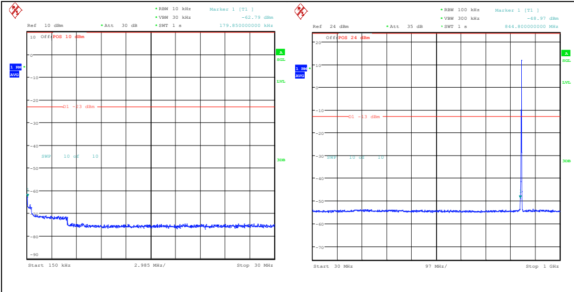
Band26_1.4MHz_16QAM_27033_6RB#0_0.15~3 0_0.15~30
