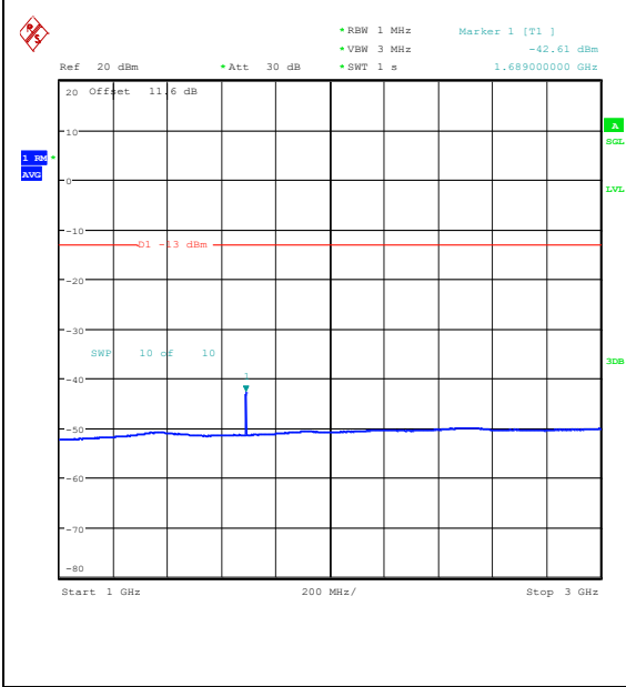
Band26_5MHz_16QAM_27015_1RB#0_1000~3000_1000~3000
