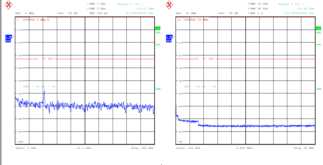
Band26_3MHz_QPSK_26915_1RB#0_0.009~0.15_5_0.009~0.15 Band26_3MHz_QPSK_26915_1RB#0_0.15~30_0_15~30
