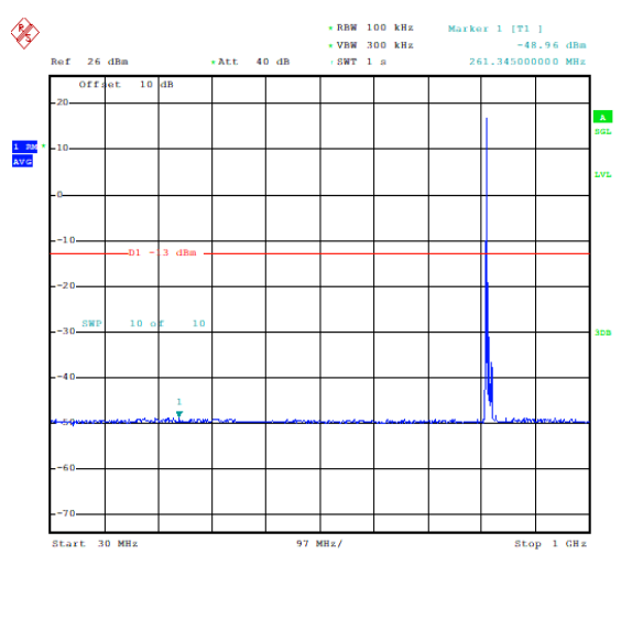
Band26_10MHz_16QAM_26740_1RB#0_30~1000_30~1000
