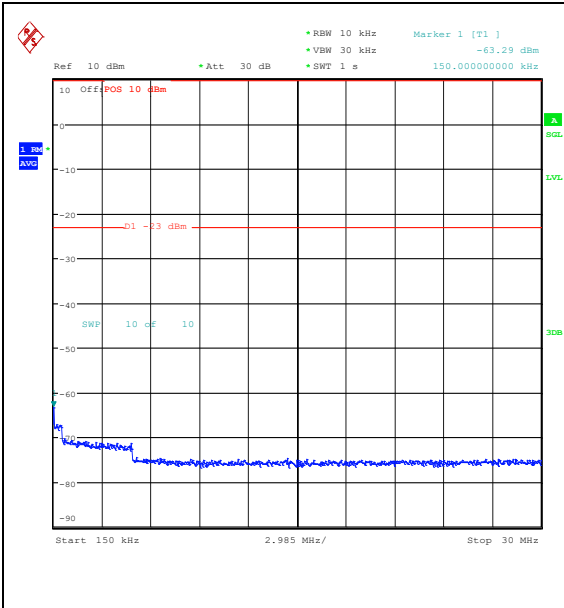
Band26_3MHz_16QAM_26805_1RB#14_0.15~3 0_0.15~30
