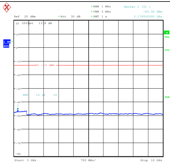
Band26_5MHz_16QAM_26915_1RB#0_3000~10000_3000~10000
