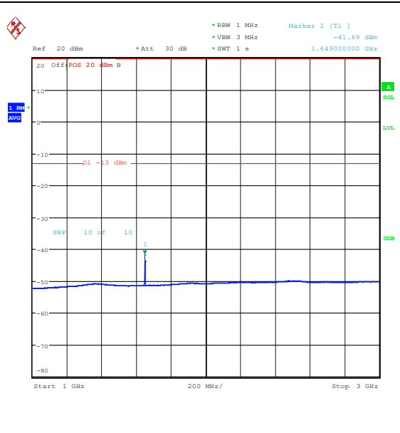
Band26_1.4MHz_QPSK_26797_6RB#0_1000~3000 00_1000~3000
