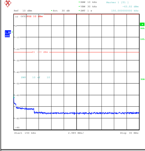
Band26_3MHz_16QAM_26915_1RB#14_0.15~3_0_0.15~30
