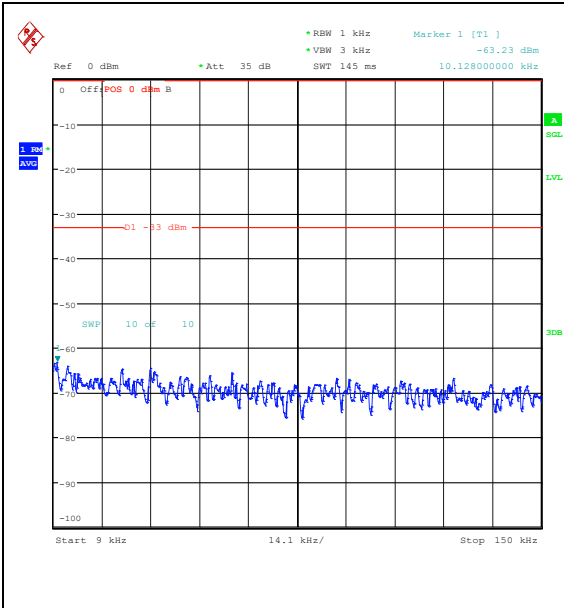
Band26_5MHz_QPSK_26915_1RB#0_0.009~0.15_5_0.009~0.15
