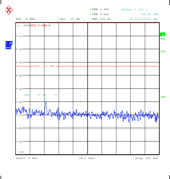
Band26_5MHz_16QAM_27015_1RB#0_0.009~0.15_5_0.009~0.15
