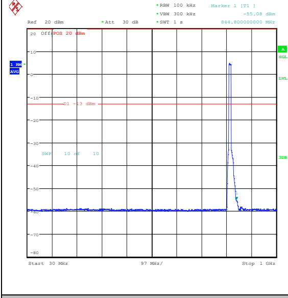
Band26_10MHz_QPSK_26740_50RB#0_30~100_0_30~1000
