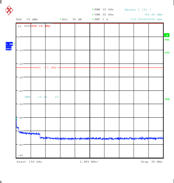
Band26_5MHz_QPSK_26815_1RB#0_0.15~30_0.15~30
