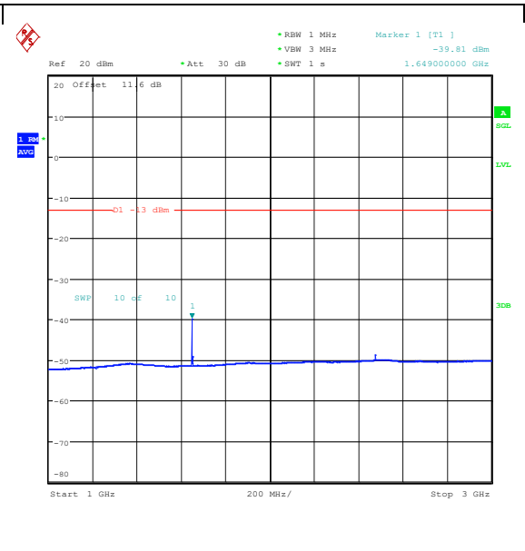
Band26_5MHz_QPSK_26815_1RB#0_1000~3000_1000~3000
