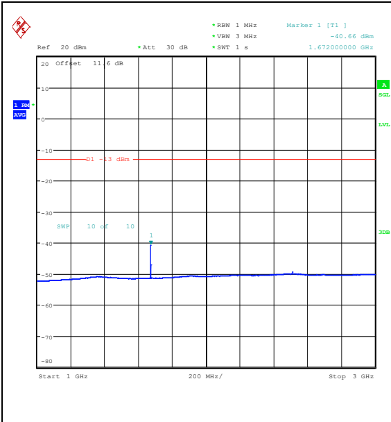
Band26_1.4MHz_16QAM_26915_1RB#0_1000~3000_1000~3000
