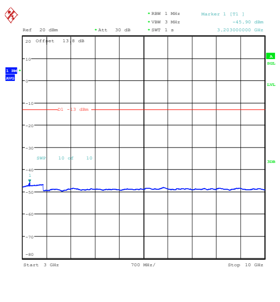
Band26_3MHz_16QAM_26805_1RB#14_3000~10 000_3000~10000
