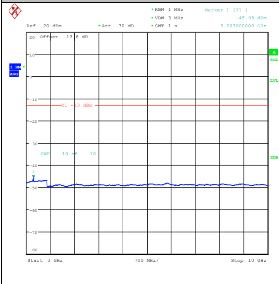
Band26_3MHz_QPSK_26805_1RB#14_3000~10 000_3000~10000
