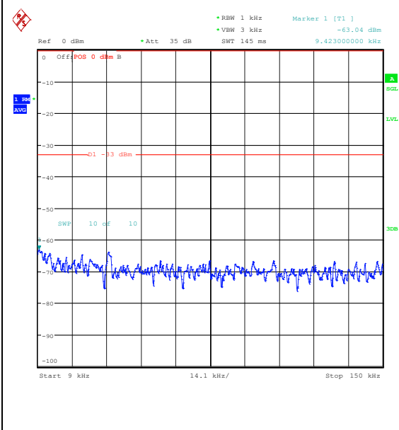
Band26_1.4MHz_QPSK_27033_6RB#0_0.009~0.15_0.009~0.15
