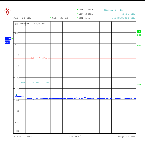
Band26_1.4MHz_16QAM_27033_1RB#5_3000~10000_3000~10000
