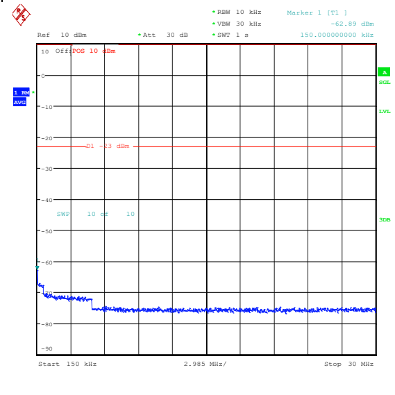
Band26_1.4MHz_QPSK_27033_1RB#0_0.15~30_0.15~30
