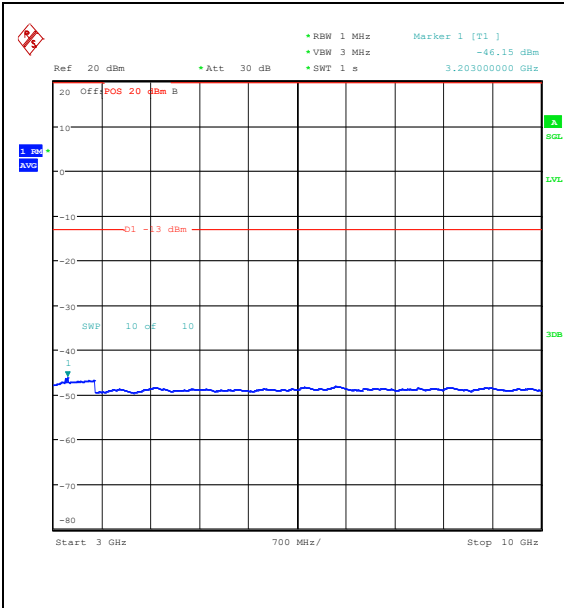
Band26_3MHz_QPSK_26805_15RB#0_3000~10000_3000~10000
