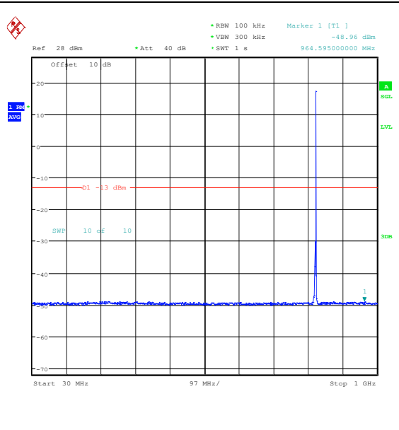
Band26_3MHz_16QAM_26805_1RB#14_30~1000 _30~1000
