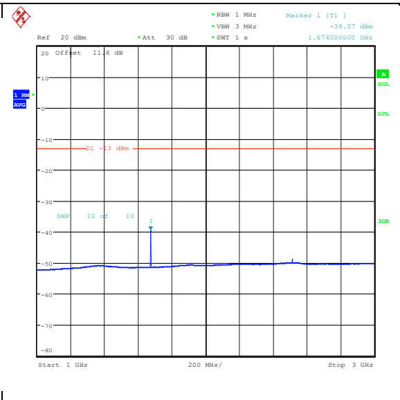
Band26_1.4MHz_QPSK_26915_1RB#5_1000~3000_00_1000~3000
