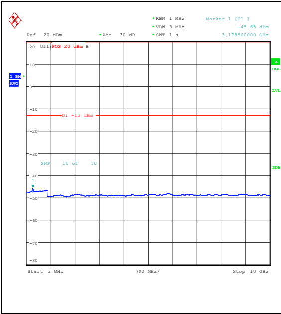
Band26_3MHz_QPSK_27025_15RB#0_3000~10000_3000~10000
