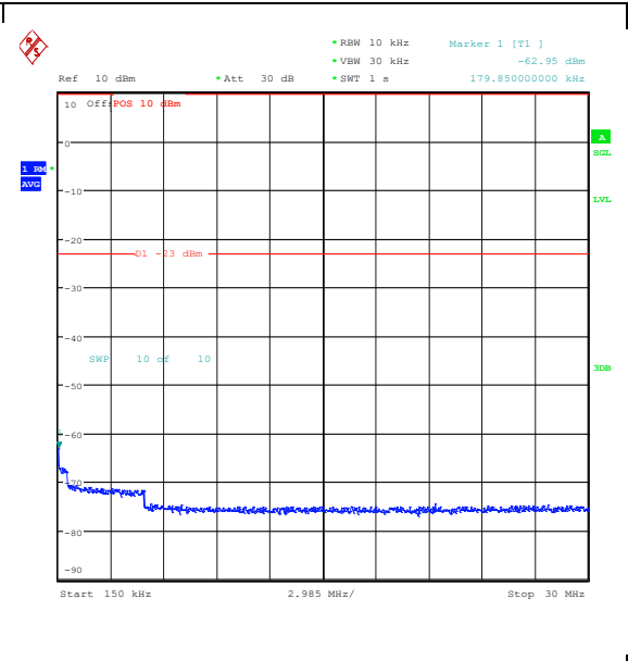
Band26_5MHz_QPSK_26915_1RB#0_0.15~30_0_15~30
