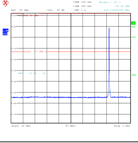
Band26_3MHz_16QAM_26805_15RB#0_30~1000_30~1000
