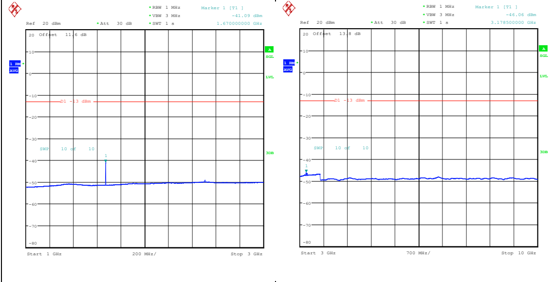
Band26_3MHz_16QAM_26915_1RB#0_1000~3000_1000~3000 Band26_3MHz_16QAM_26915_1RB#0_3000~10000_3000~10000
