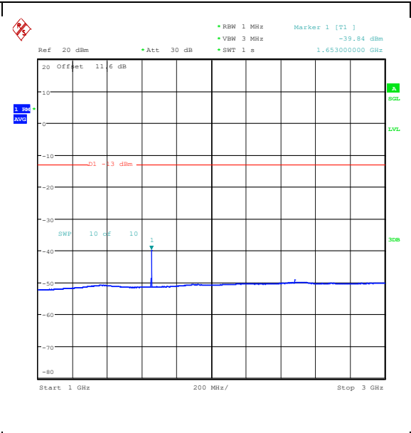
Band26_3MHz_QPSK_26805_1RB#14_1000~300 0_1000~3000
