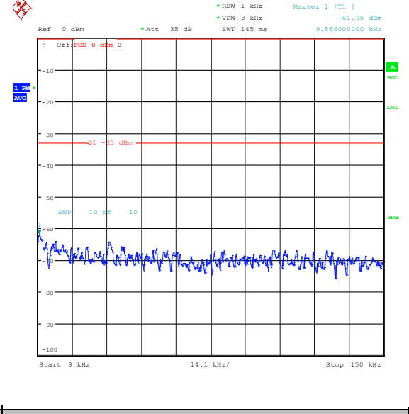
Band26_1.4MHz_16QAM_26797_1RB#0_0.009~0.15_0.009~0.15
