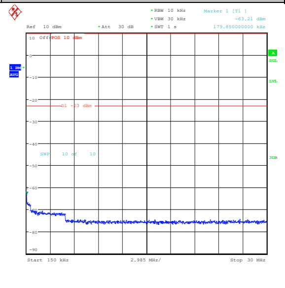
Band26_10MHz_QPSK_26740_1RB#49_0.15~30_0.15~30
