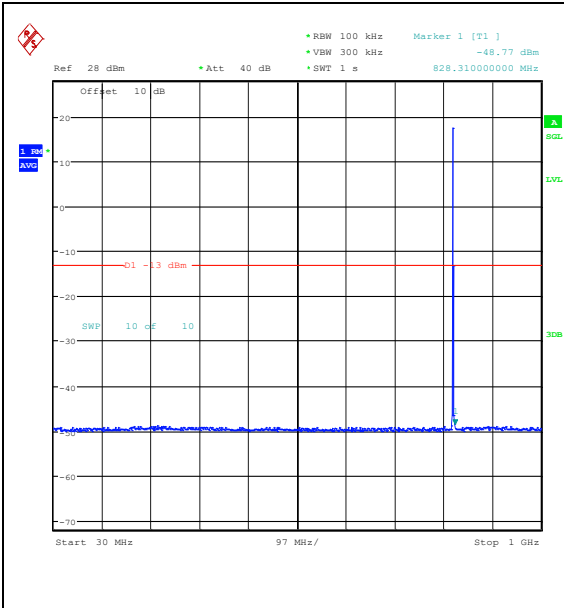
Band26_1.4MHz_QPSK_26797_1RB#0_30~1000_30~1000
