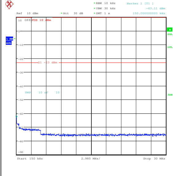
Band26_3MHz_16QAM_27025_1RB#0_0.15~30_0.15~30
