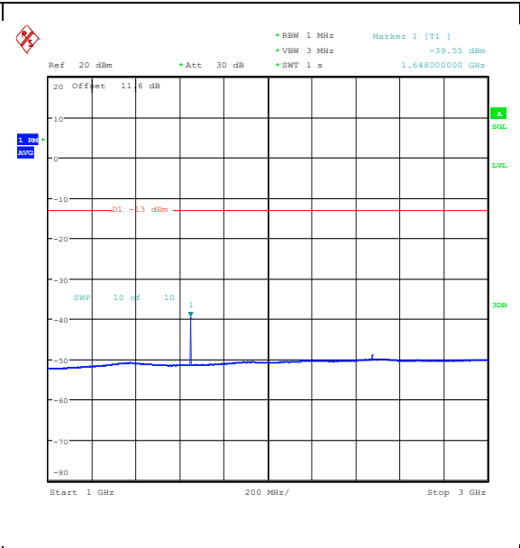
Band26_1.4MHz_QPSK_26797_1RB#0_1000~3000_00_1000~3000
