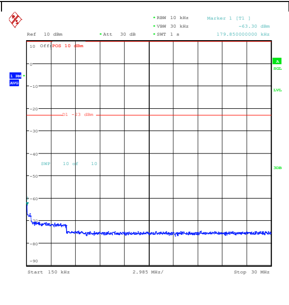
Band26_3MHz_QPSK_26805_1RB#0_0.15~30_0.15~30
