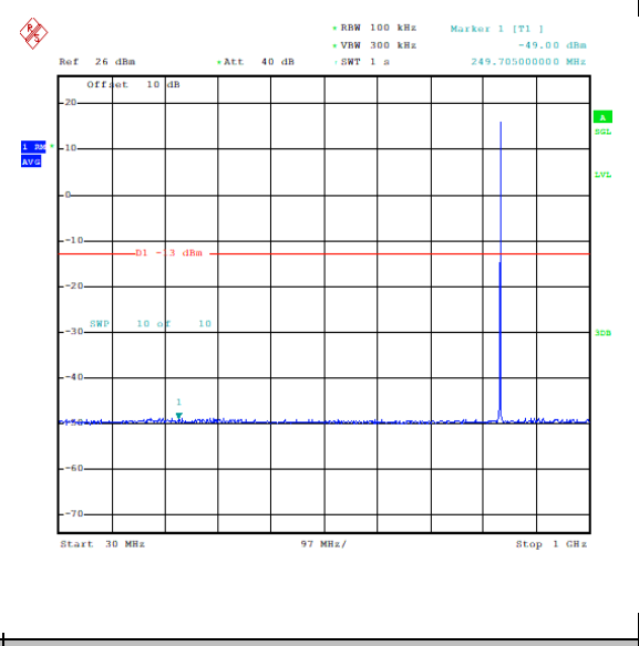
Band26_1.4MHz_16QAM_26915_1RB#0_30~1000_30~1000
