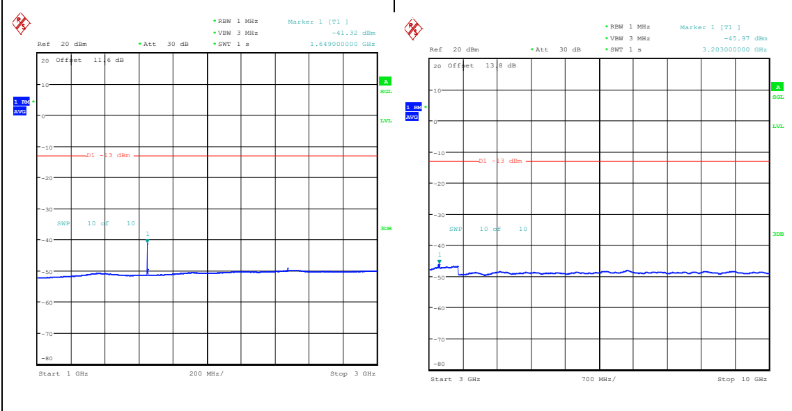
Band26_5MHz_16QAM_26815_1RB#0_1000~3000_1000~3000 Band26_5MHz_16QAM_26815_1RB#0_3000~1000_3000~10000
