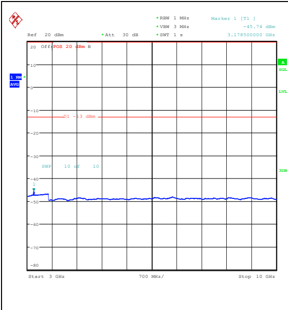
Band26_1.4MHz_QPSK_26915_6RB#0_3000~1000_3000~10000
