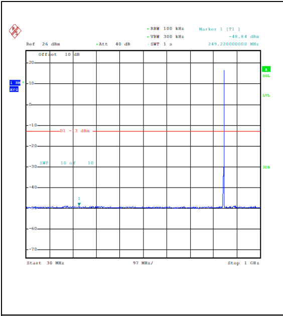
Band26_3MHz_QPSK_27025_1RB#14_30~1000_30~1000
