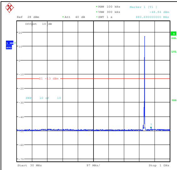
Band26_5MHz_QPSK_26915_1RB#24_30~1000_30~1000
