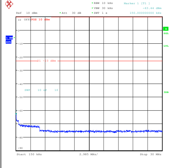
Band26_5MHz_16QAM_26915_1RB#0_0.15~30_0.15~30
