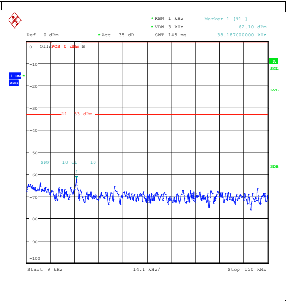
Band26_5MHz_16QAM_26915_1RB#0_0.009~0.15_5_0.009~0.15
