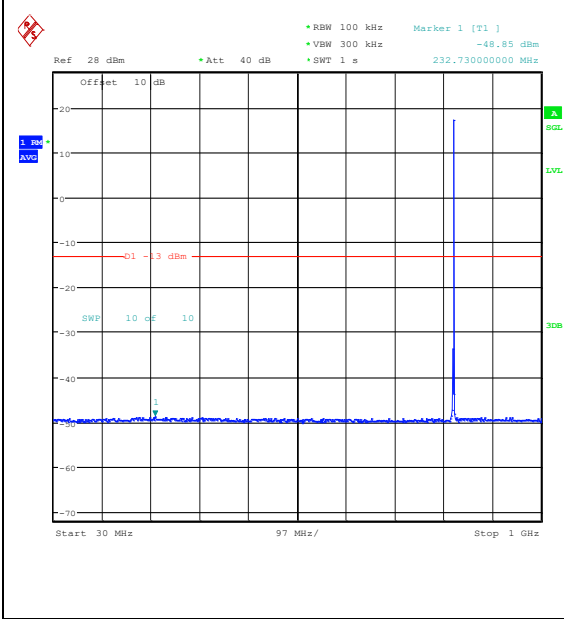
Band26_1.4MHz_QPSK_26797_1RB#5_30~1000_30~1000
