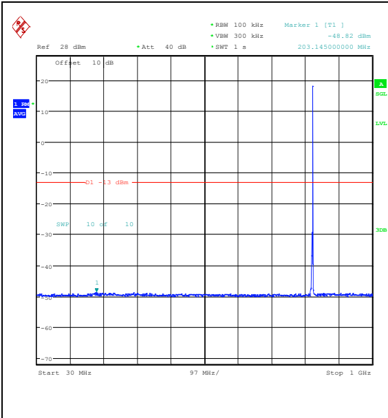
Band26_3MHz_QPSK_26805_1RB#14_30~1000
