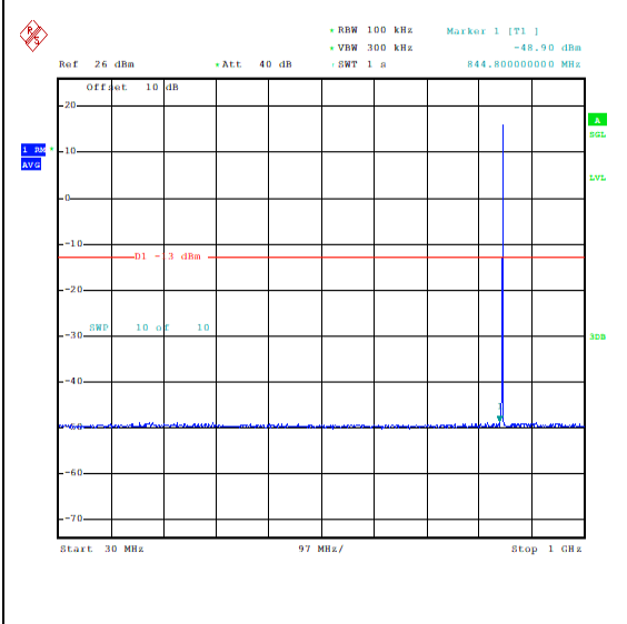
Band26_1.4MHz_QPSK_27033_1RB#5_30-1000_30-1000
