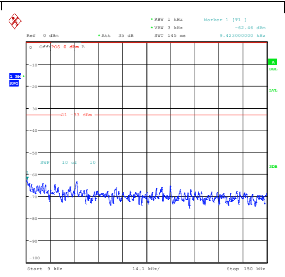
Band26_3MHz_16QAM_26805_1RB#0_0.009~0.15_5_0.009~0.15
