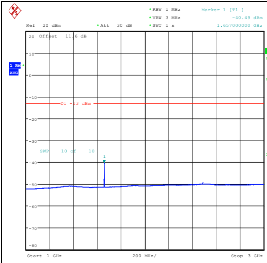
Band26_5MHz_16QAM_26815_1RB#24_1000~3000_1000~3000
