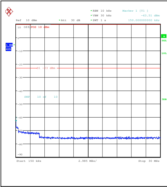
Band26_5MHz_16QAM_27015_1RB#0_0.15~30_0.15~30
