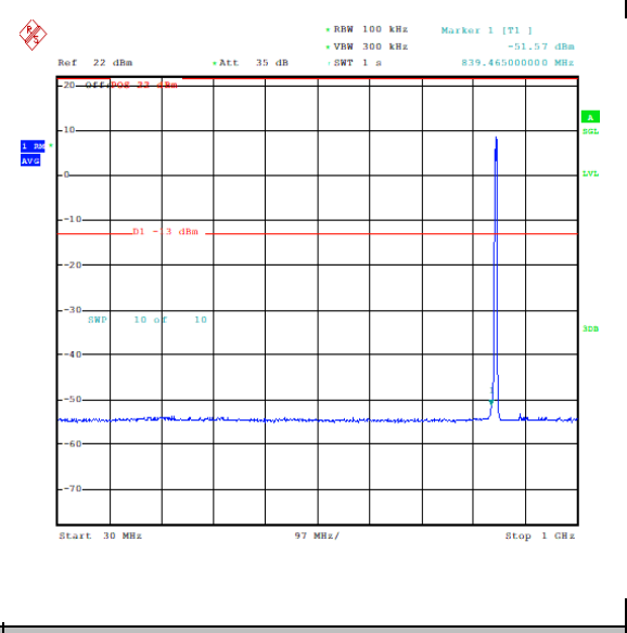
Band26_3MHz_16QAM_27025_15RB#0_30~1000_30~1000
