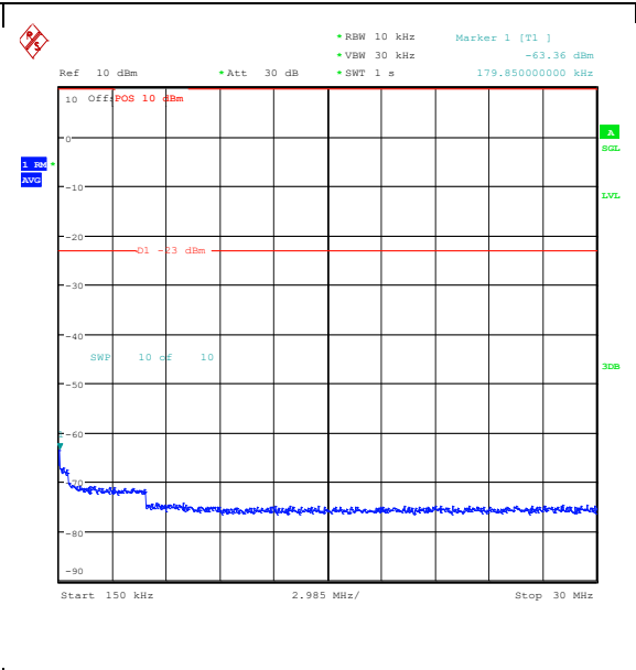
Band26_10MHz_QPSK_26740_50RB#0_0.15~30_0.15~30
