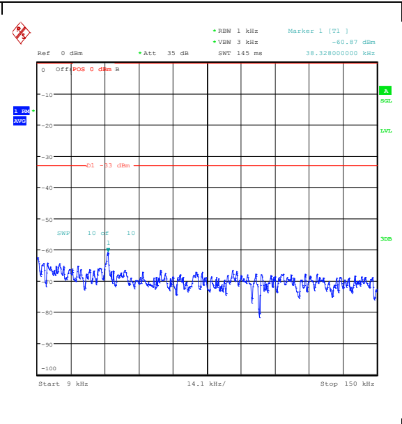
Band26_5MHz_16QAM_26915_25RB#0_0.009~0.15_0.009~0.15
