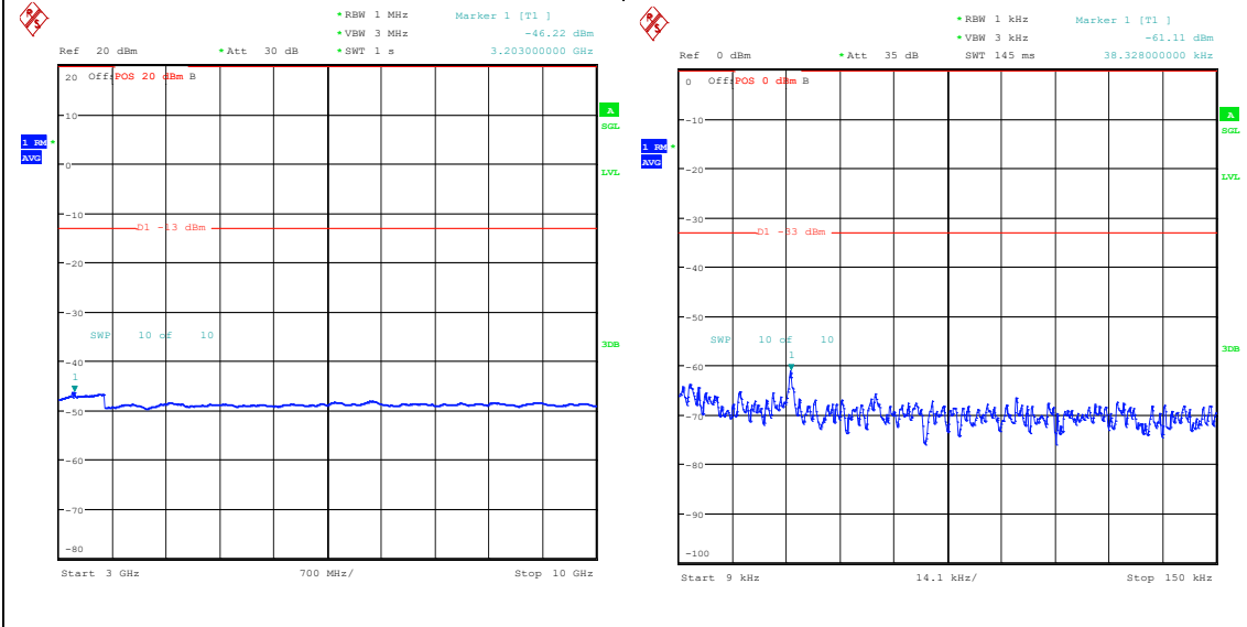
Band26_5MHz_QPSK_26815_25RB#0_3000~10000_3000~10000 Band26_5MHz_16QAM_26815_25RB#0_0.009~0.15_0.009~0.15
