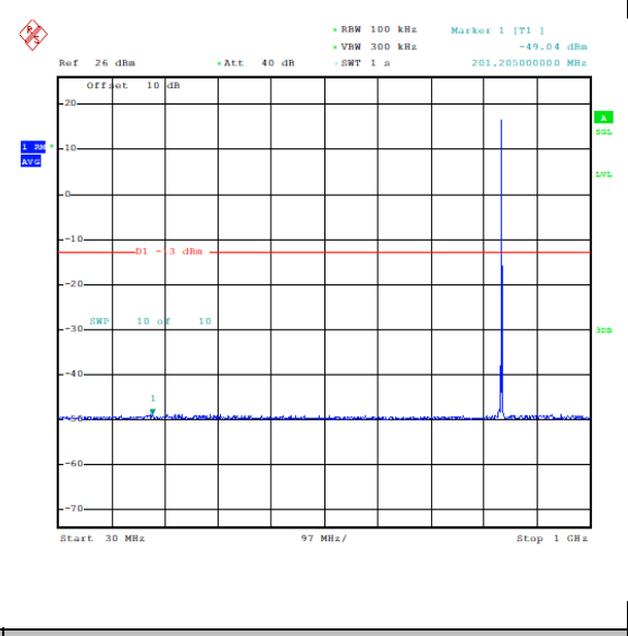
Band26_3MHz_16QAM_26915_1RB#14_30~1000_30~1000
