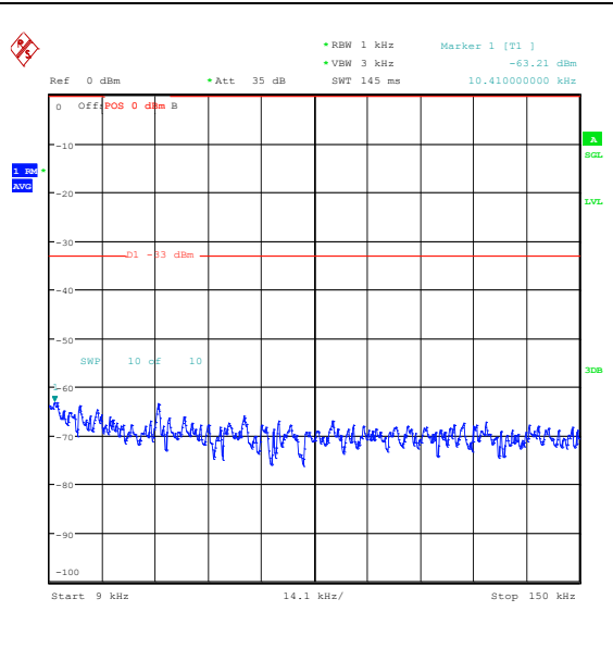
Band26_3MHz_16QAM_26805_15RB#0_0.009~0.15_0.009~0.15
