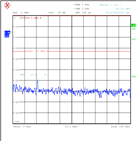
Band26_1.4MHz_QPSK_26915_6RB#0_0.009~0.15_0.009~0.15
