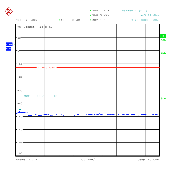
Band26_3MHz_16QAM_26805_1RB#0_3000~10000_00_3000~10000
