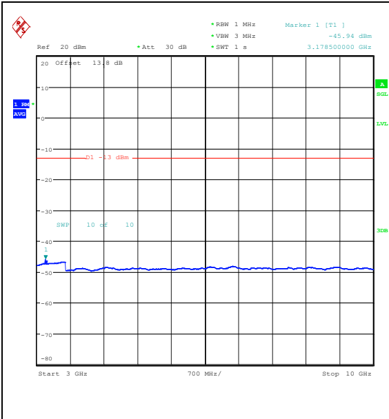
Band26_3MHz_QPSK_27025_1RB#0_3000~10000_00_3000~10000
