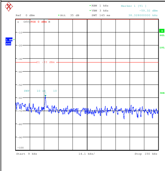
Band26_10MHz_QPSK_26740_1RB#49_0.009~0.15_0.15_0.009~0.15
