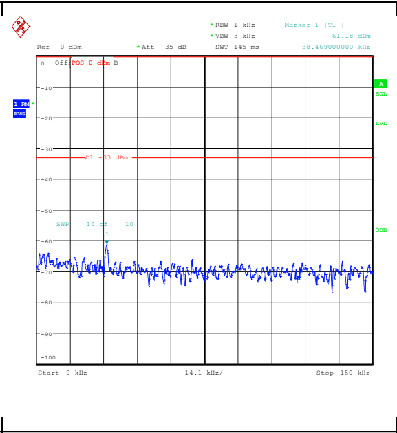
Band26_3MHz_16QAM_26915_1RB#14_0.009~0.15_15_0.009~0.15
