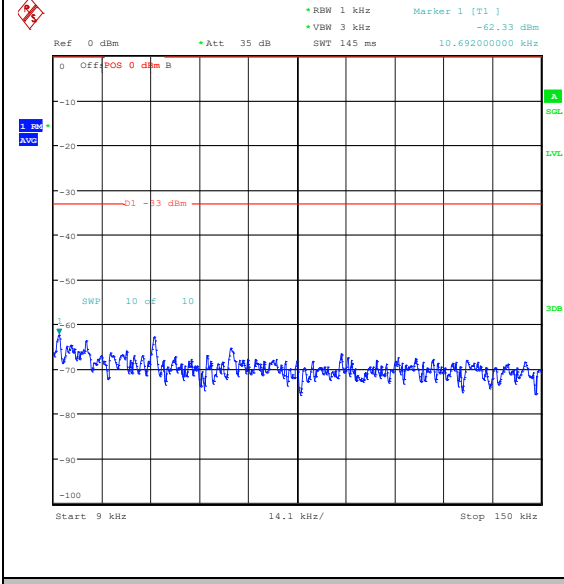
Band26_1.4MHz_QPSK_26915_1RB#5_0.009~0.15_0.009~0.15
