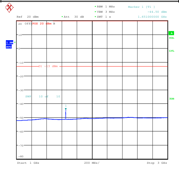
Band26_3MHz_QPSK_26805_15RB#0_1000~3000_0_1000~3000
