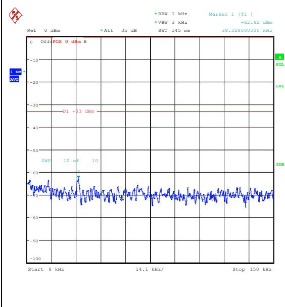
Band26_3MHz_QPSK_26805_1RB#14_0.009~0.15_0.009~0.15
