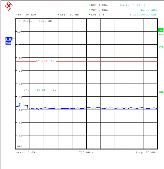
Band26_5MHz_QPSK_26815_1RB#0_3000~10000_00_3000~10000
