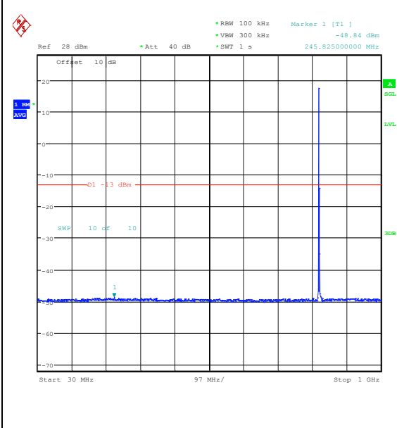
Band26_3MHz_QPSK_26805_1RB#0_30~1000_30~1000
