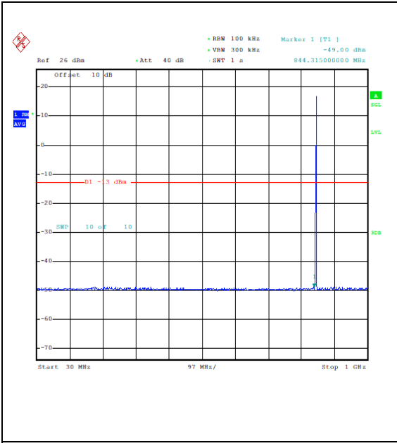
Band26_1.4MHz_QPSK_27033_1RB#0_30~1000_30~1000
