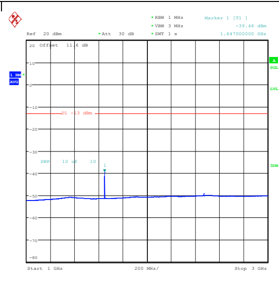
Band26_10MHz_QPSK_26740_1RB#49_1000~3000 00_1000~3000
