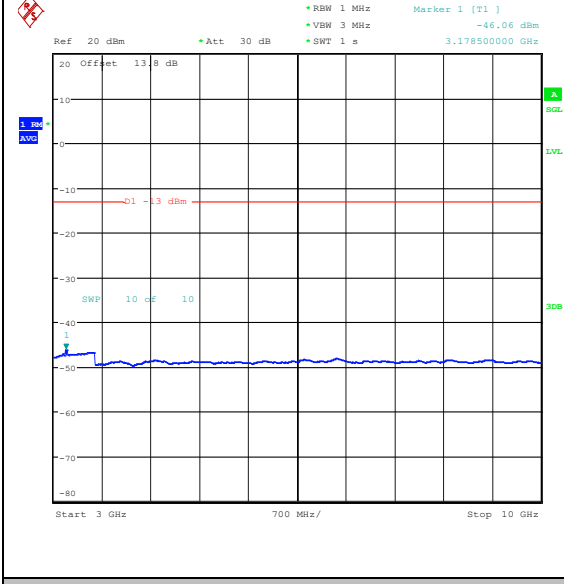
Band26_3MHz_QPSK_27025_1RB#14_3000~10_000_3000~10000
