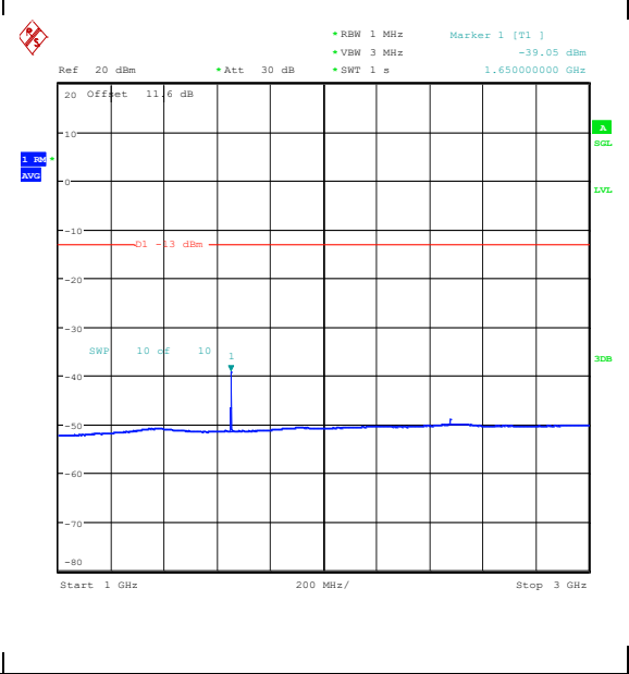
Band26_1.4MHz_QPSK_26797_1RB#5_1000~3000_00_1000~3000
