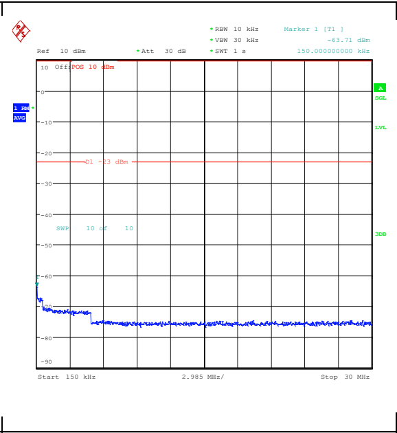
Band26_1.4MHz_QPSK_26797_1RB#5_0.15~30_0.15~30
