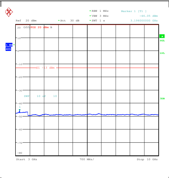
Band26_3MHz_16QAM_27025_15RB#0_3000~10000_3000~10000
