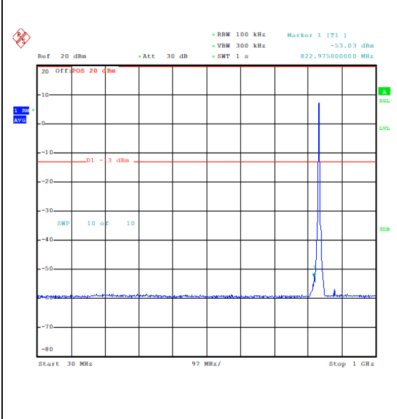
Band26_5MHz_QPSK_26915_25RB#0_30~1000_30~1000
