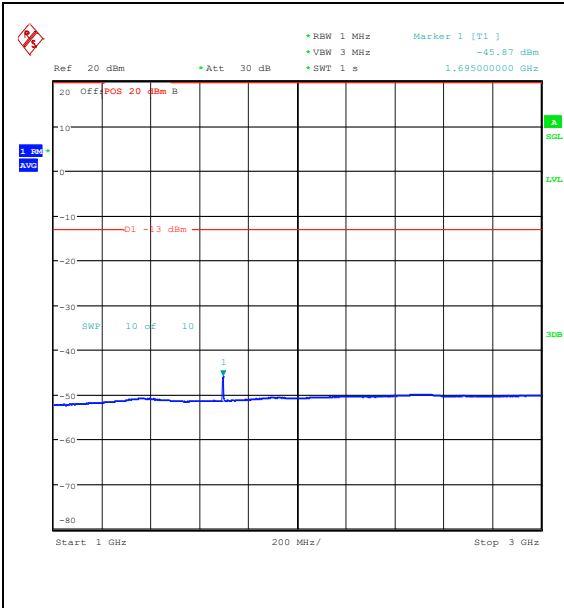
Band26_3MHz_16QAM_27025_15RB#0_1000~3000_1000~3000
