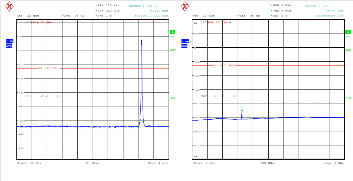
Band26_5MHz_QPSK_26815_25RB#0_30~1000_30~1000 Band26_5MHz_QPSK_26815_25RB#0_1000~3000_0_1000~3000
