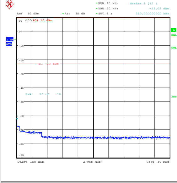
Band26_1.4MHz_16QAM_26915_1RB#0_0.15~30_0.15~30
