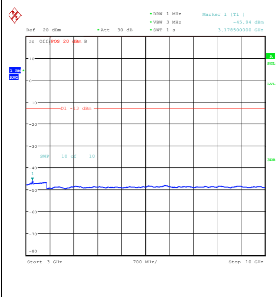
Band26_1.4MHz_QPSK_27033_6RB#0_3000~10000_000_3000~10000
