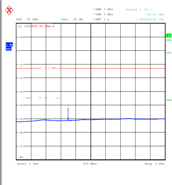
Band26_1.4MHz_16QAM_27033_6RB#0_1000~ 3000_1000~3000
