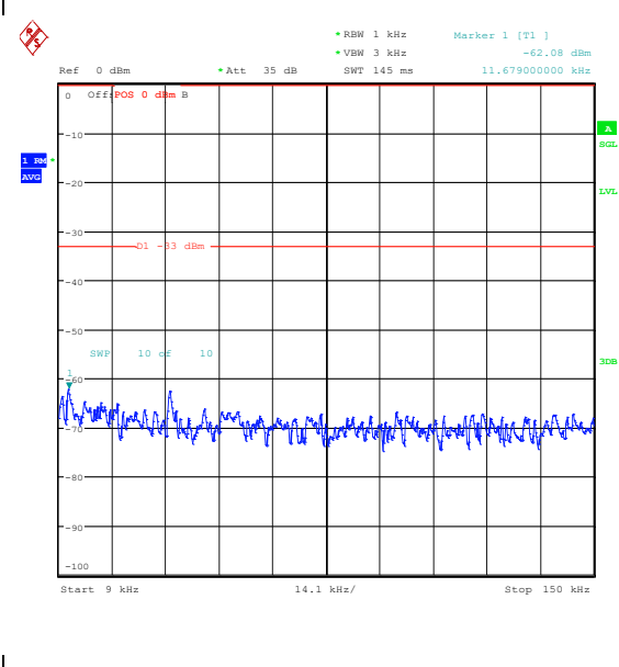
Band26_10MHz_16QAM_26740_1RB#49_0.009~0.15 0.15_0.009~0.15
