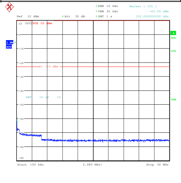
Band26_3MHz_QPSK_27025_1RB#14_0.15~0.30_0.15~30
