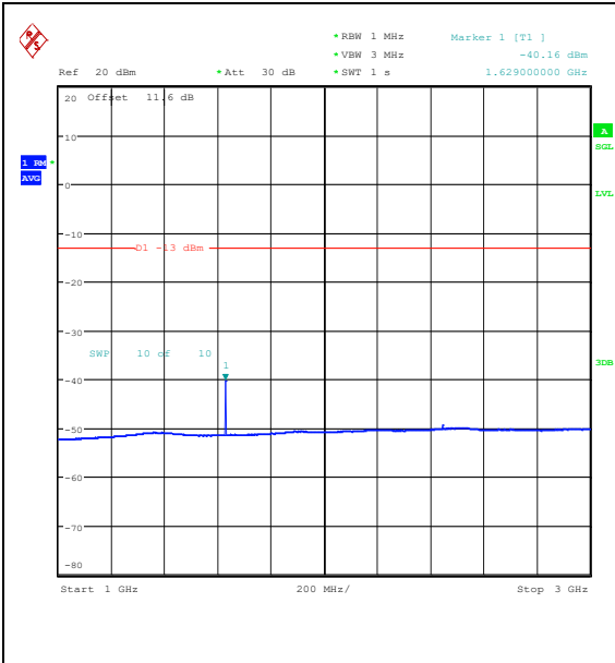
Band26_10MHz_16QAM_26740_1RB#0_1000~3000_1000~3000
