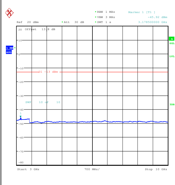
Band26_3MHz_QPSK_26915_1RB#0_3000~10000_00_3000~10000
