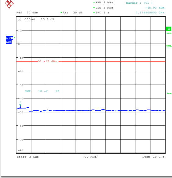
Band26_1.4MHz_QPSK_27033_1RB#0_3000~10000_000_3000~10000
