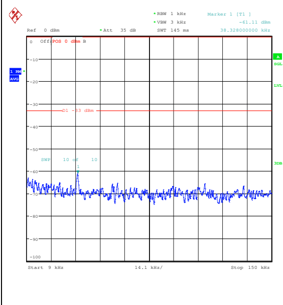
Band26_5MHz_QPSK_27015_1RB#0_0.009~0.15_5_0.009~0.15
