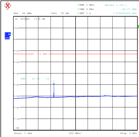
Band26_1.4MHz_16QAM_26797_1RB#5_1000~3000_1000~3000
