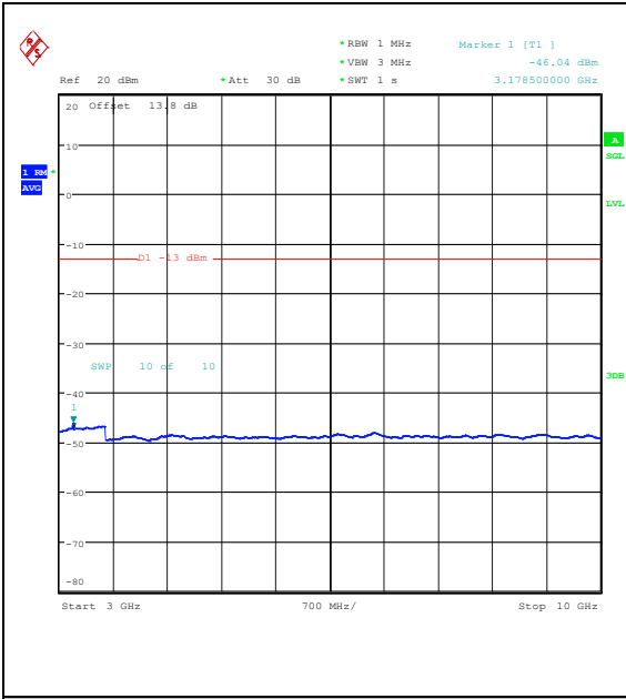
Band26_1.4MHz_QPSK_26915_1RB#0_3000~10000_3000~10000
