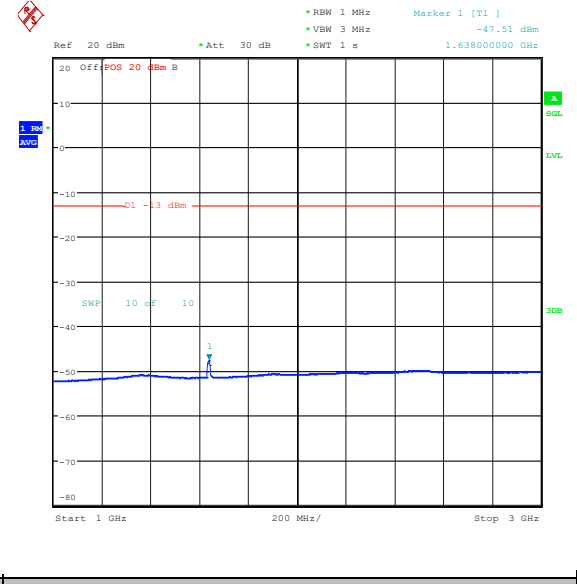
Band26_10MHz_QPSK_26740_50RB#0_1000~3000_00_1000~3000
