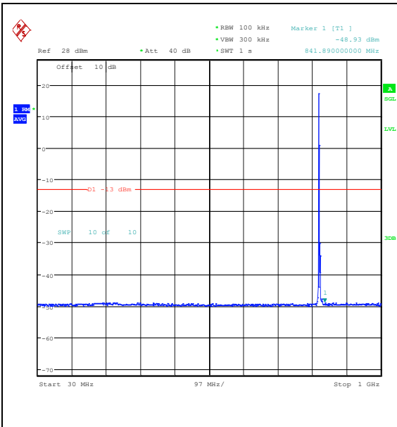
Band26_5MHz_QPSK_26815_1RB#0_30~1000_30~1000
