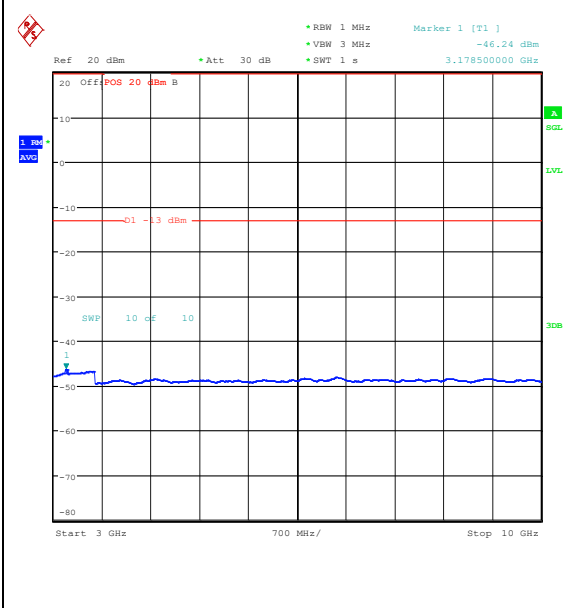
Band26_1.4MHz_QPSK_26797_6RB#0_3000~10000 000_3000~10000
