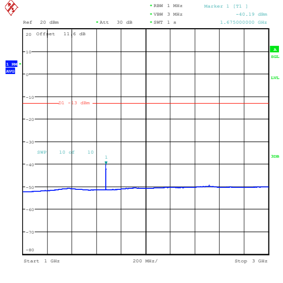
Band26_3MHz_QPSK_26915_1RB#14_1000~3000_0_1000~3000
