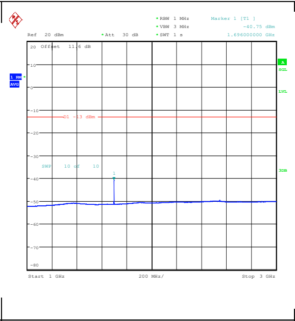
Band26_1.4MHz_QPSK_27033_1RB#0_1000~3000_00_1000~3000
