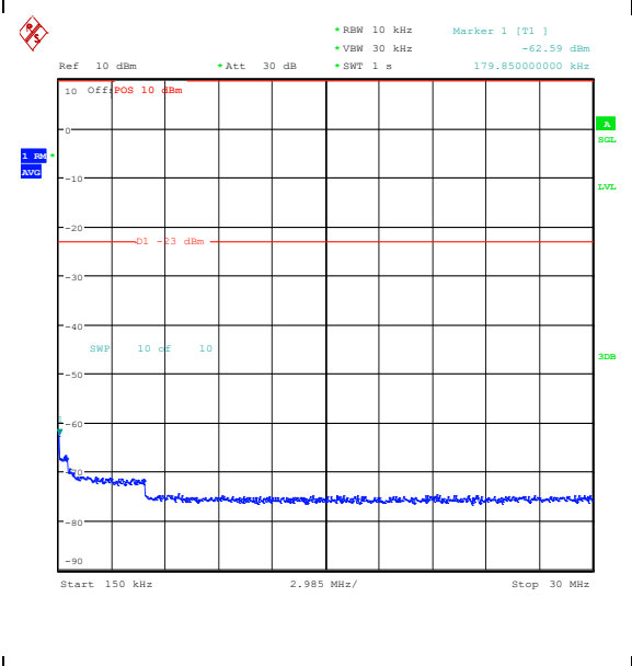
Band26_1.4MHz_QPSK_27033_6RB#0_0.15~30_0.15~30
