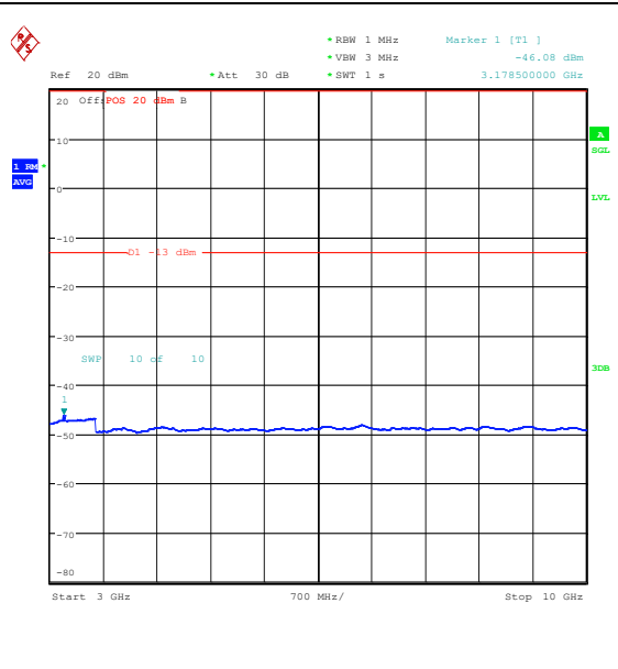
Band26_10MHz_16QAM_26740_50RB#0_3000~10000_3000~10000
