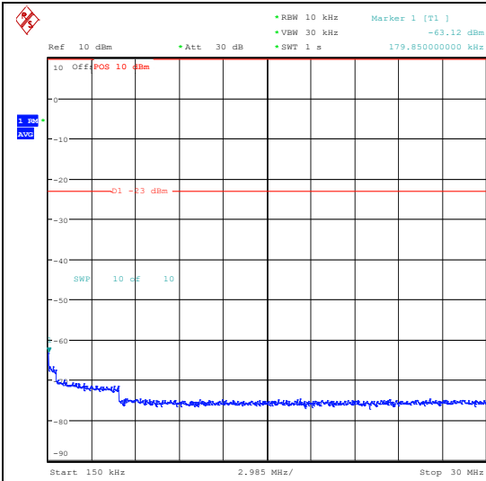
Band26_3MHz_16QAM_26915_15RB#0_0.15~3 0_0.15~30
