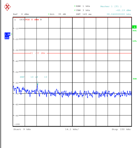
Band26_5MHz_QPSK_26815_1RB#0_0.009~0.15_5_0.009~0.15
