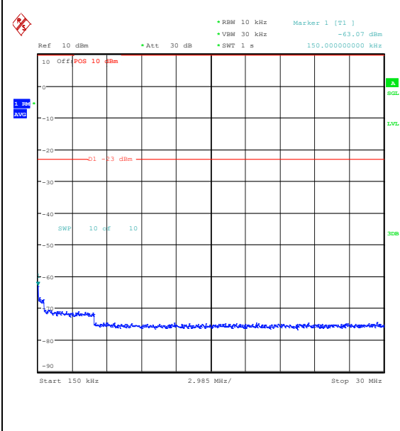
Band26_3MHz_16QAM_26805_1RB#0_0.15~30_0.15~30
