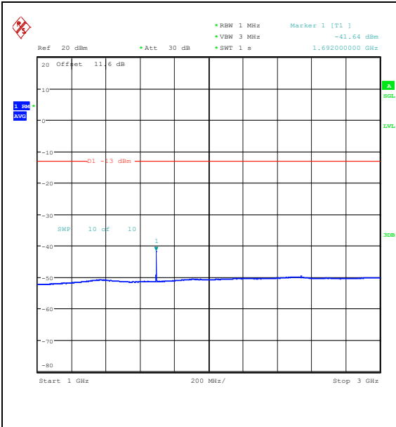
Band26_3MHz_16QAM_27025_1RB#0_1000~3000_00_1000~3000
