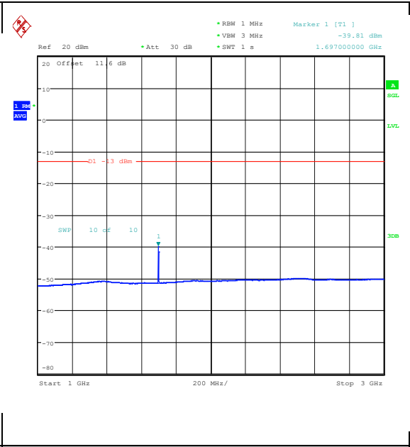
Band26_3MHz_QPSK_27025_1RB#14_1000~300_0_1000~3000
