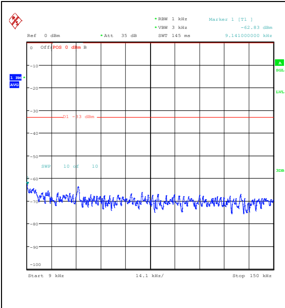
Band26_10MHz_QPSK_26740_50RB#0_0.009~0.15_0.009~0.15
