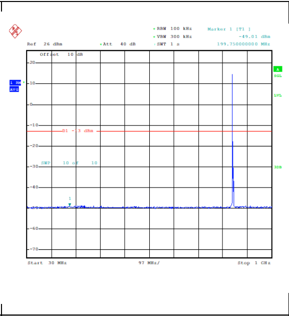
Band26_5MHz_16QAM_27015_1RB#0_30~1000_30~1000
