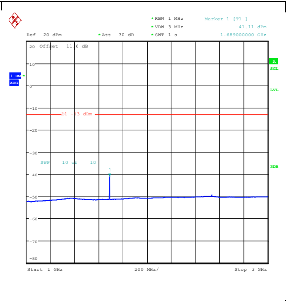
Band26_5MHz_QPSK_27015_1RB#0_1000~3000_1000~3000
