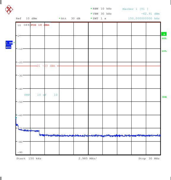
Band26_3MHz_QPSK_26805_1RB#14_0.15~30_0.15~30
