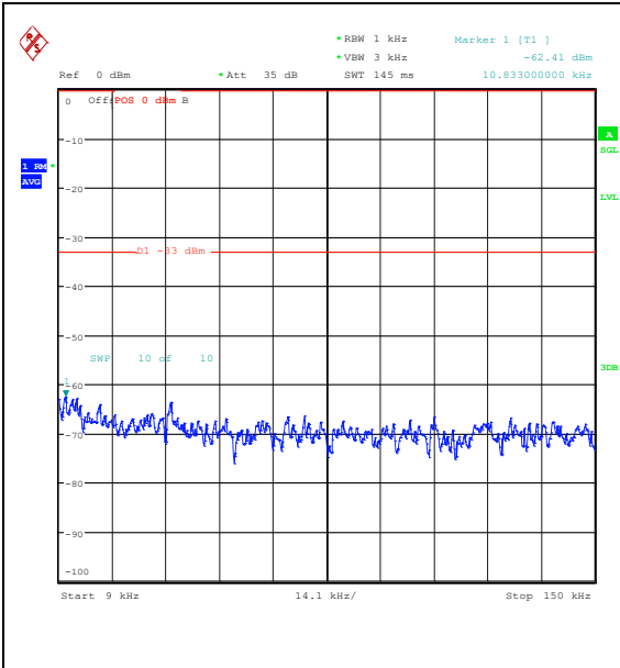
Band26_10MHz_QPSK_26740_1RB#0_0.009~0.15_0.009~0.15
