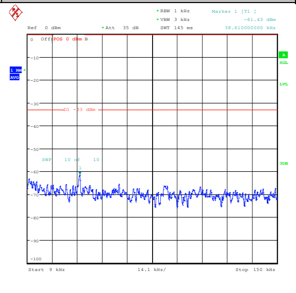
Band26_3MHz_16QAM_26805_1RB#14_0.009~0.15 15_0.009~0.15
