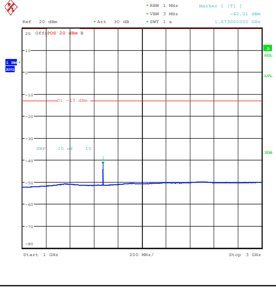
Band26_1.4MHz_QPSK_26915_6RB#0_1000~3000_1000~3000
