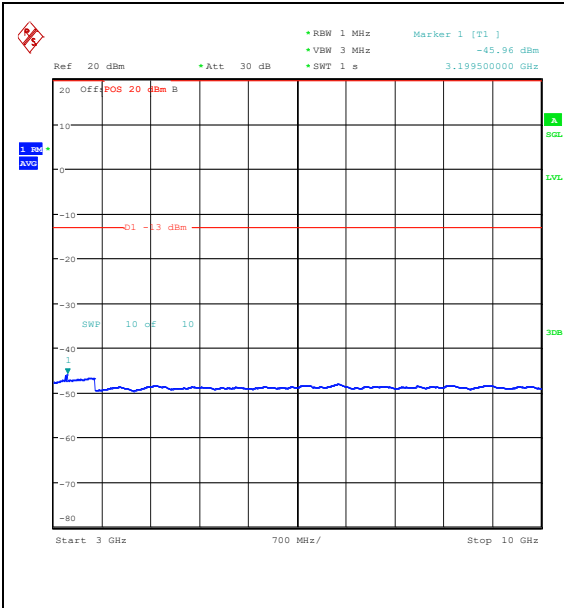
Band26_5MHz_QPSK_26915_25RB#0_3000~10000_3000~10000
