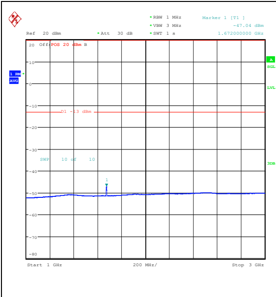
Band26_5MHz_16QAM_26915_25RB#0_1000~3000_1000~3000
