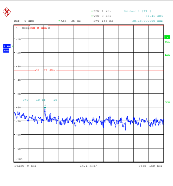
Band26_10MHz_16QAM_26740_1RB#0_0.009~0.15_0.009~0.15
