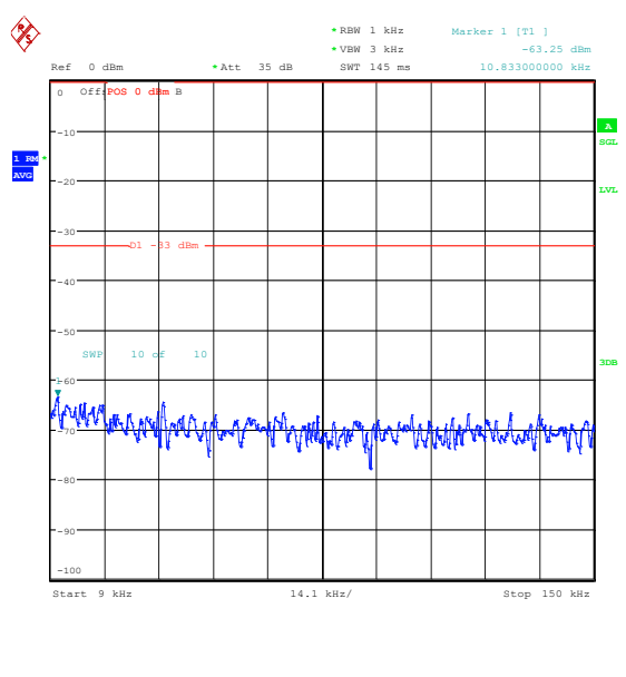
Band26_1.4MHz_16QAM_26797_6RB#0_0.009~0.15 .15_0.009~0.15
