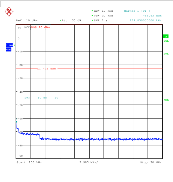
Band26_10MHz_QPSK_26740_1RB#0_0.15~30_0.15~30
