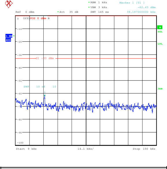
Band26_1.4MHz_16QAM_27033_1RB#0_0.009~0.15_0.009~0.15
