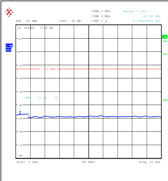
Band26_1.4MHz_QPSK_26797_1RB#5_3000~1000_3000~10000
