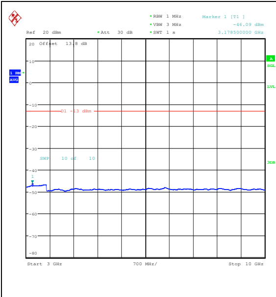
Band26_5MHz_QPSK_26915_1RB#0_3000~10000_00_3000~10000
