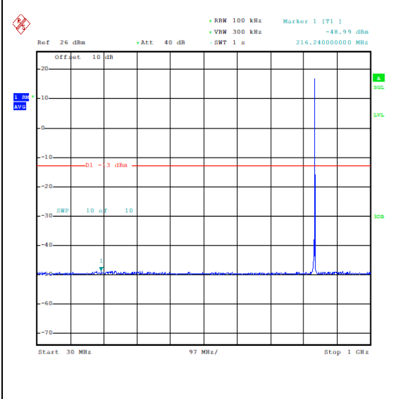
Band26_3MHz_QPSK_26915_1RB#14_30~1000_30~1000
