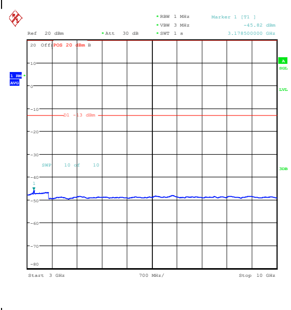
Band26_1.4MHz_16QAM_27033_6RB#0_3000~1 0000_3000~10000
