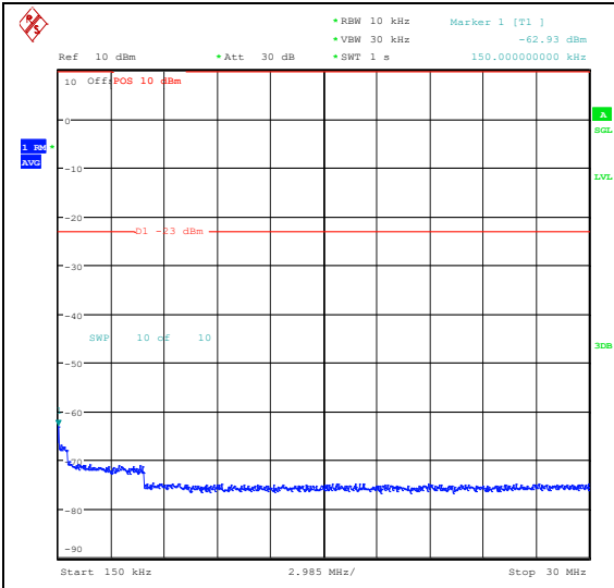
Band26_10MHz_16QAM_26740_1RB#49_0.15~30_0.15~30
