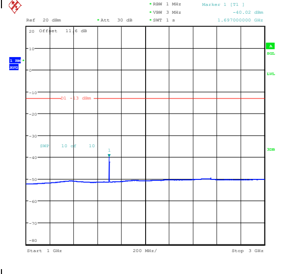
Band26_1.4MHz_QPSK_27033_1RB#5_1000-3000_00_1000-3000
