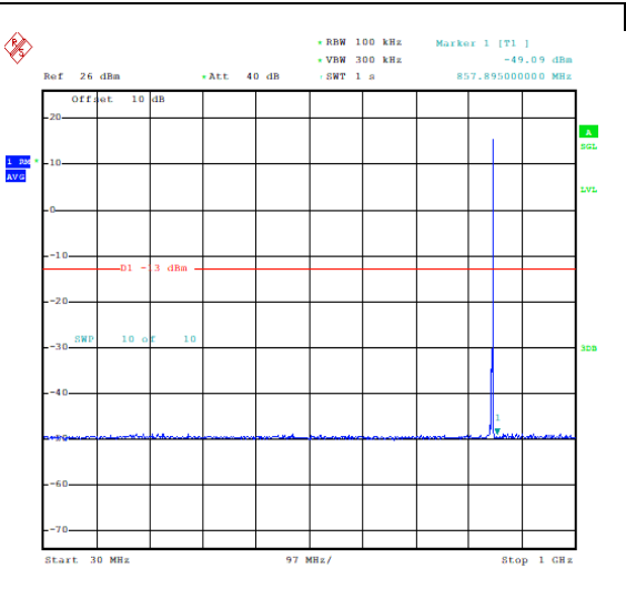
Band26_3MHz_16QAM_27025_1RB#14_30~1000 _30~1000
