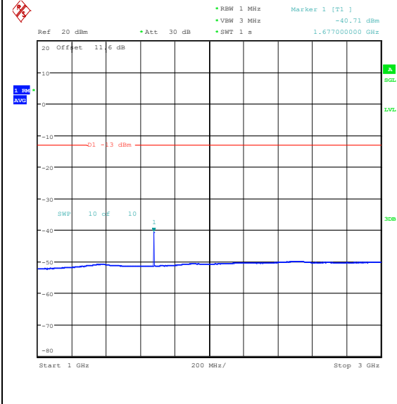
Band26_5MHz_16QAM_26915_1RB#24_1000~3 000_1000~3000
