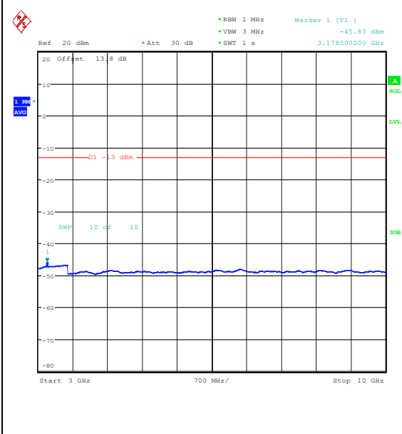
Band26_5MHz_QPSK_27015_1RB#0_3000~10000_3000~10000
