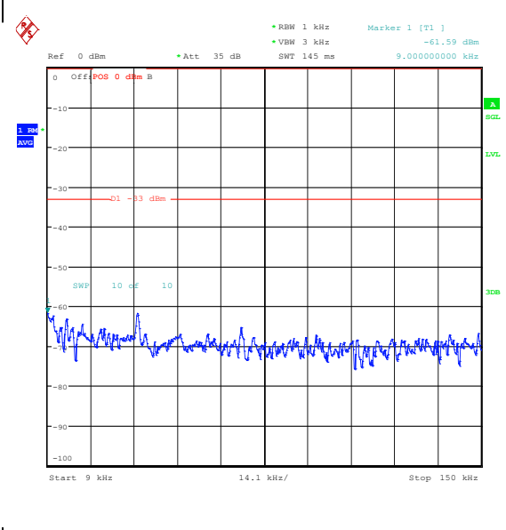
Band26_3MHz_16QAM_26915_1RB#0_0.009~0.15_5_0.009~0.15
