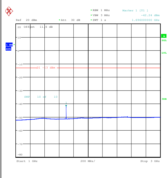
Band26_1.4MHz_16QAM_27033_1RB#0_1000~ 3000_1000~3000
