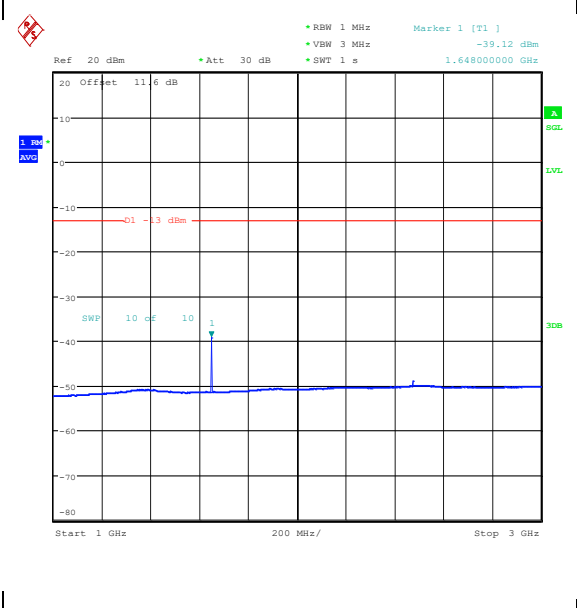
Band26_3MHz_QPSK_26805_1RB#0_1000~3000_1000~3000
