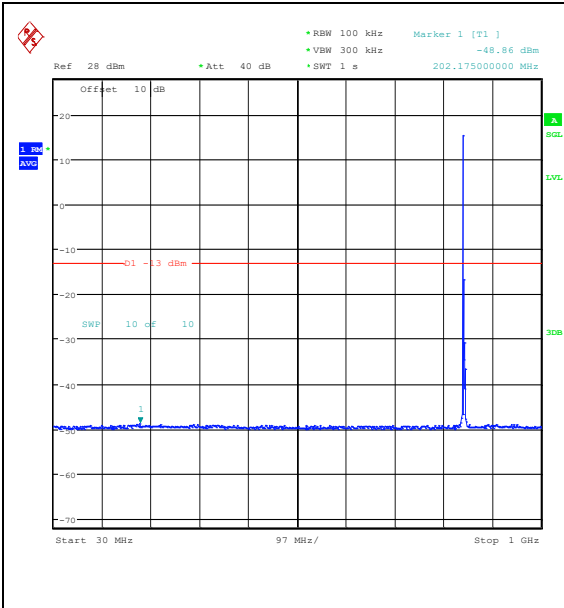
Band26_5MHz_QPSK_27015_1RB#0_30~1000_30~1000
