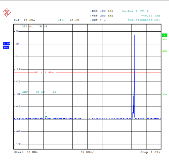
Band26_10MHz_16QAM_26740_1RB#49_30~1000_30~1000
