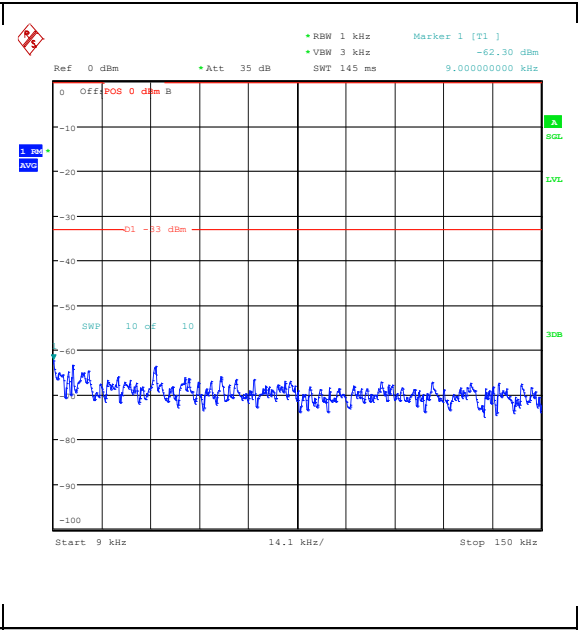
Band26_3MHz_16QAM_27025_15RB#0_0.009~0.15_0.009~0.15
