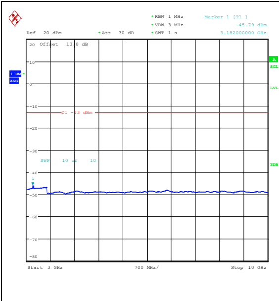
Band26_10MHz_QPSK_26740_1RB#0_3000~10000_3000~10000
