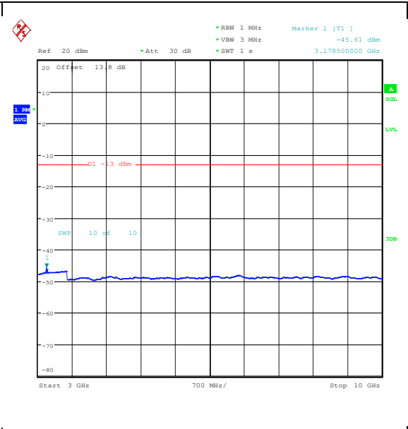
Band26_3MHz_16QAM_27025_1RB#0_3000~10000_00_3000~10000
