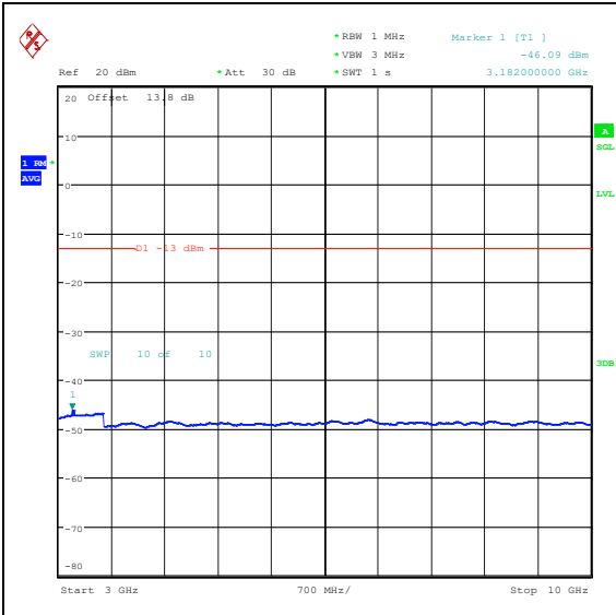
Band26_3MHz_QPSK_26805_1RB#0_3000~10000_00_3000~10000
