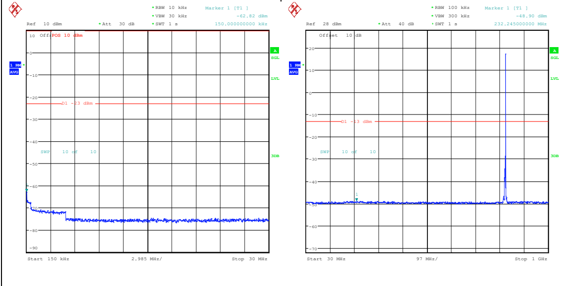
Band26_5MHz_16QAM_26815_1RB#24_0.15~30_0.15~30 Band26_5MHz_16QAM_26815_1RB#24_30~1000_30~1000
