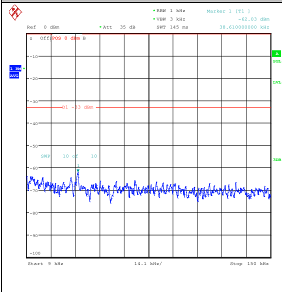
Band26_3MHz_QPSK_27025_1RB#14_0.009~0.15_15_0.009~0.15
