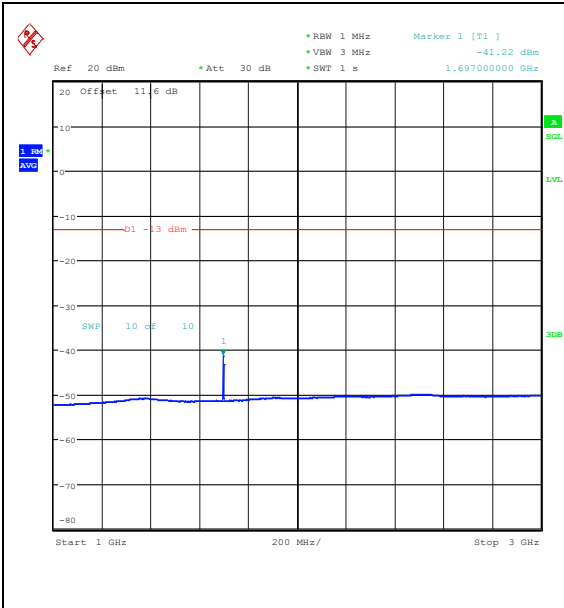
Band26_1.4MHz_16QAM_27033_1RB#5_1000~3000_1000~3000
