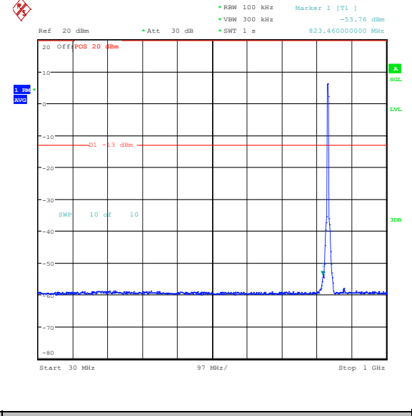
Band26_5MHz_16QAM_26915_25RB#0_30~1000_30~1000
