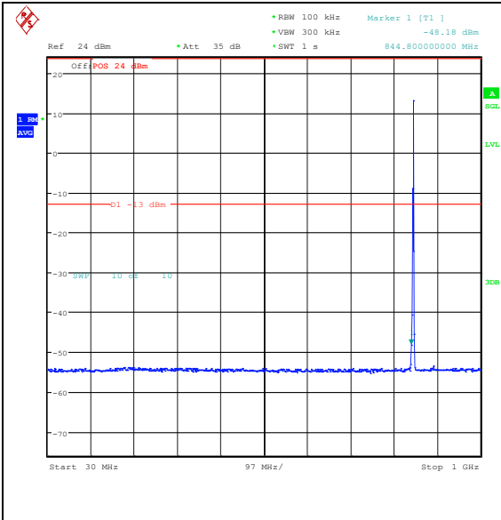
Band26_1.4MHz_QPSK_27033_6RB#0_30~1000_30~1000
