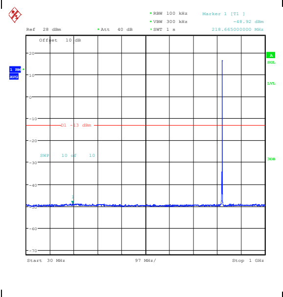
Band26_1.4MHz_16QAM_26797_1RB#5_30~100_0_30~1000
