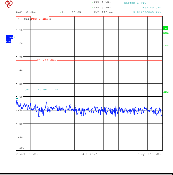
Band26_3MHz_16QAM_27025_1RB#14_0.009~0.15_0.009~0.15
