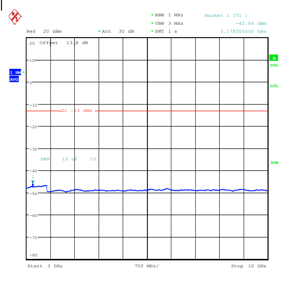
Band26_1.4MHz_16QAM_27033_1RB#0_3000~1 0000_3000~10000
