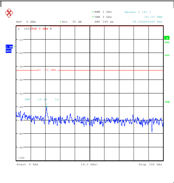
Band26_3MHz_16QAM_27025_1RB#0_0.009~0.15_5_0.009~0.15
