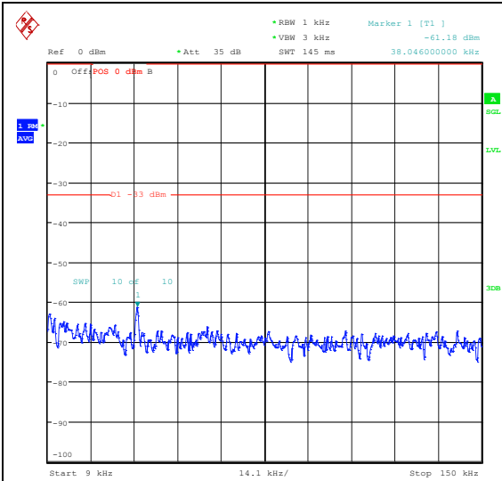
Band26_3MHz_QPSK_27025_1RB#0_0.009~0.15_5_0.009~0.15
