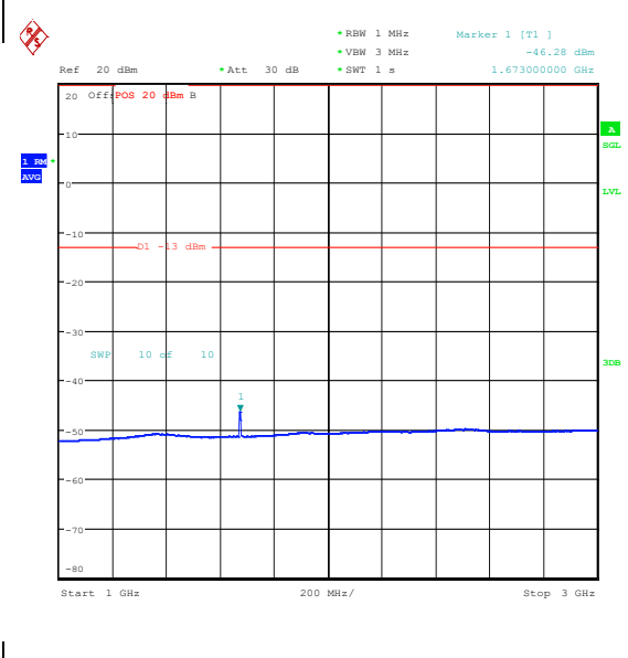
Band26_5MHz_QPSK_26915_25RB#0_1000~3000_0_1000~3000
