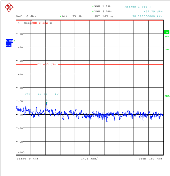
Band26_3MHz_QPSK_26915_1RB#14_0.009~0.15_0.009~0.15
