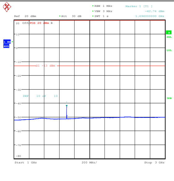
Band26_1.4MHz_QPSK_27033_6RB#0_1000~3000_00_1000~3000
