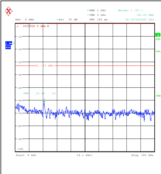
Band26_1.4MHz_QPSK_27033_1RB#5_0.009-0.15_0.009-0.15
