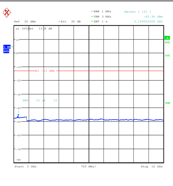
Band26_1.4MHz_16QAM_26915_1RB#0_3000~10000_3000~10000
