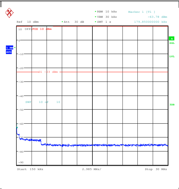
Band26_1.4MHz_QPSK_27033_1RB#5_0.15-30_0.15-30
