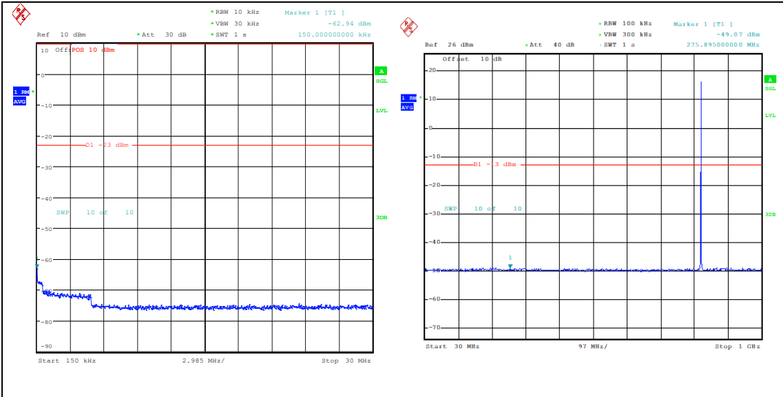
Band26_1.4MHz_16QAM_26797_1RB#0_0.15~3 0_0.15~30
