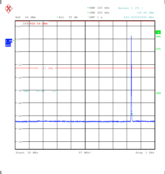
Band26_1.4MHz_16QAM_26915_6RB#0_30~1000_30~1000
