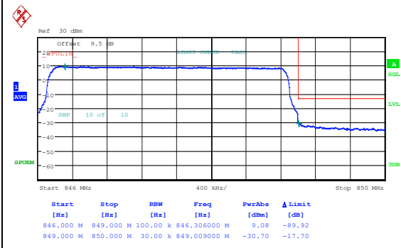
Band26_3MHz_QPSK_27025_1RB#14
