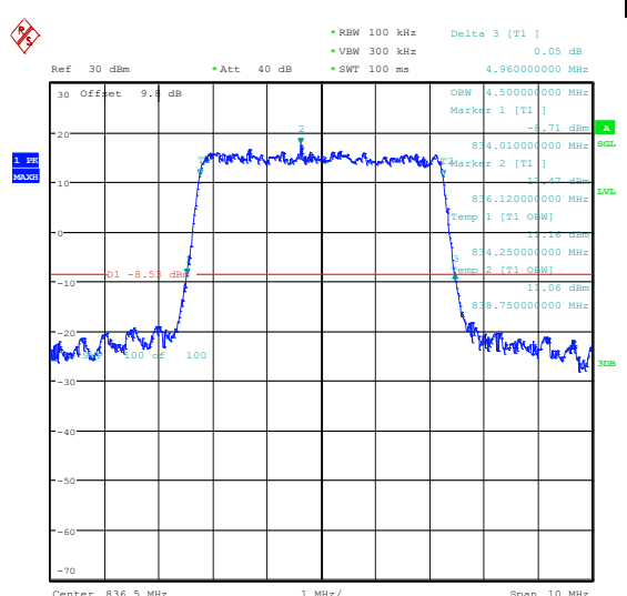
Band26(824-849)-5MHz-16QAM-26815-25RB#0-P ASS
