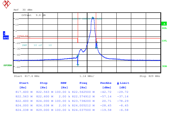
Band26_1.4MHz_16QAM_26783_1RB#0
