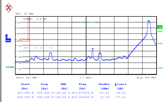
Band26_10MHz_QPSK_26840_1RB#0
