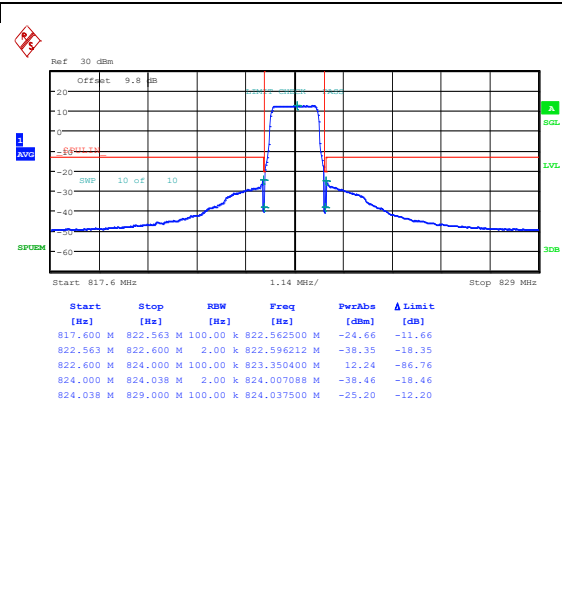
Band26_1.4MHz_16QAM_26783_6RB#0
