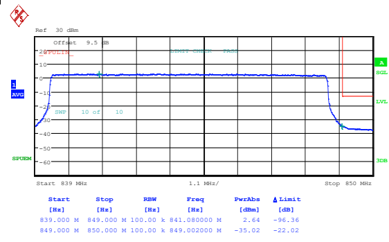
Band26_10MHz_16QAM_26990_1RB#49
