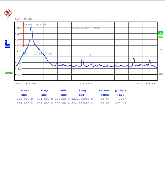
Band26_15MHz_16QAM_26865_1RB#0
