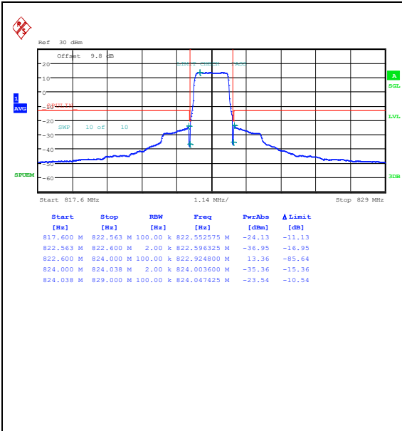
Band26_1.4MHz_QPSK_26783_6RB#0
