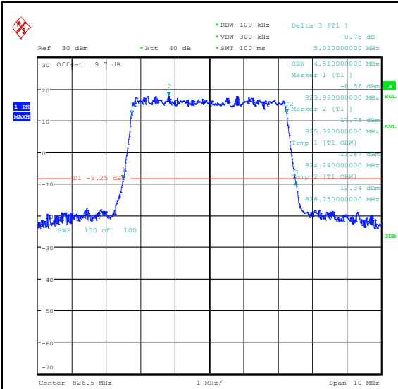
Band26(824-849)-5MHz-QPSK-26815-25RB#0-P ASS
