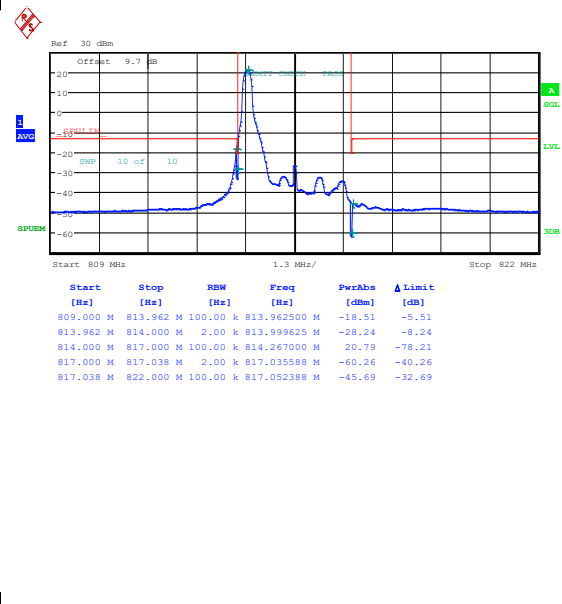
Band26_3MHz_16QAM_26705_1RB#0
