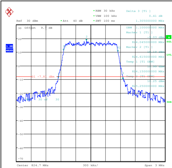
Band26(824-849)-1.4MHz-QPSK-26797-6RB#0-P ASS
