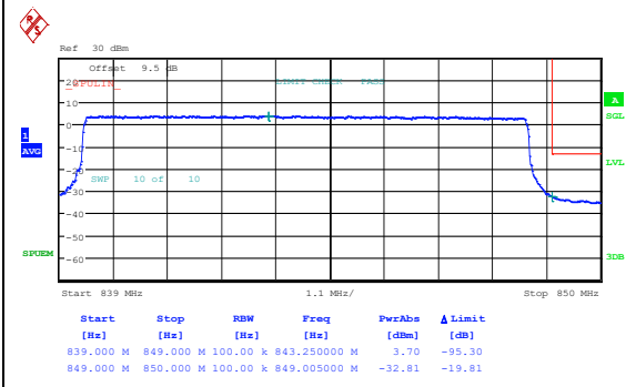
Band26_10MHz_QPSK_26990_1RB#49
