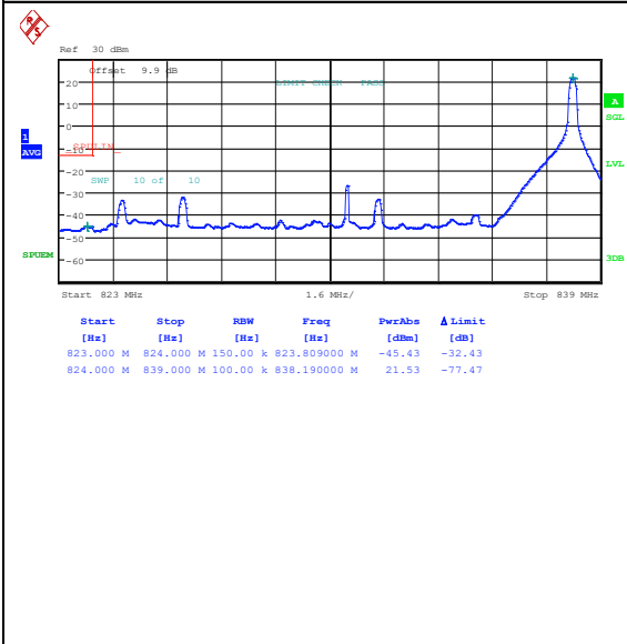
Band26_15MHz_QPSK_26865_1RB#74
