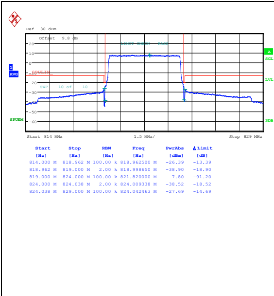
Band26_5MHz_QPSK_26765_25RB#0
