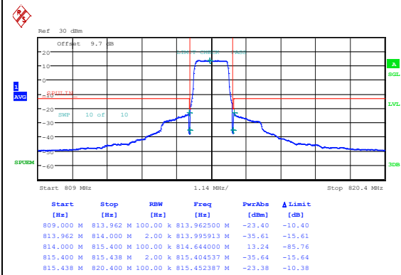
Band26_1.4MHz_QPSK_26697_1RB#5
