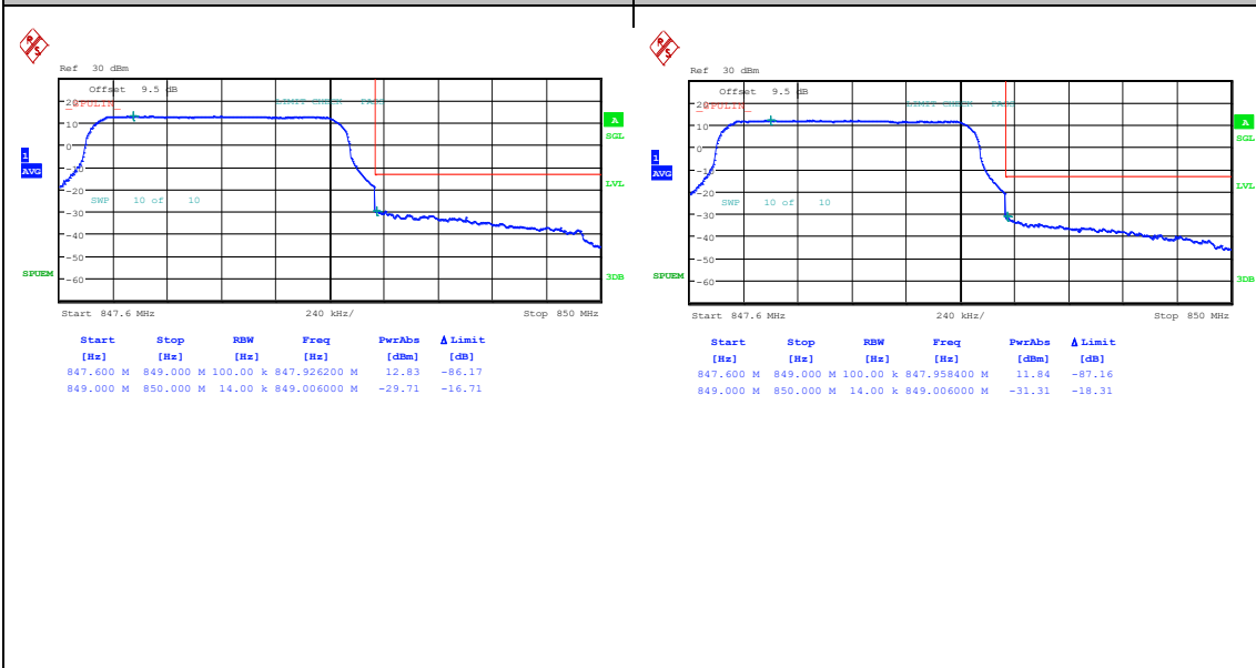
Band26_1.4MHz_QPSK_27033_1RB#5
