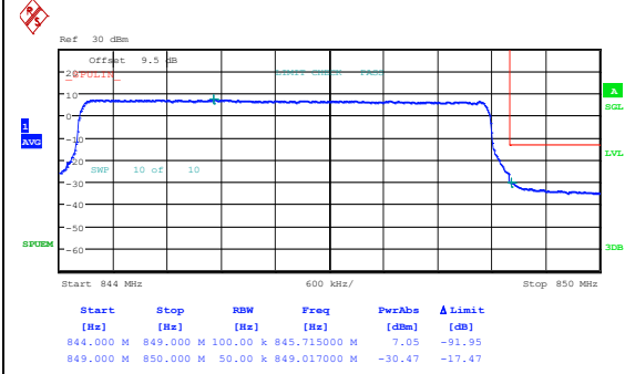
Band26_5MHz_QPSK_27015_1RB#24
