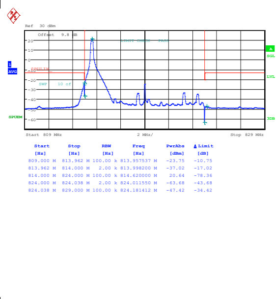
Band26_10MHz_16QAM_26740_1RB#0
