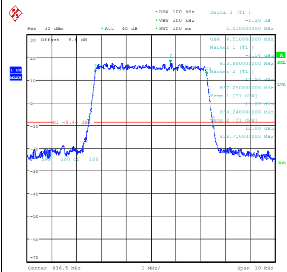
Band26(824-849)-5MHz-QPSK-26815-25RB#0-P ASS
