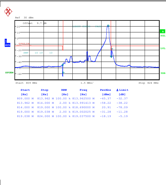
Band26_5MHz_16QAM_26715_1RB#24
