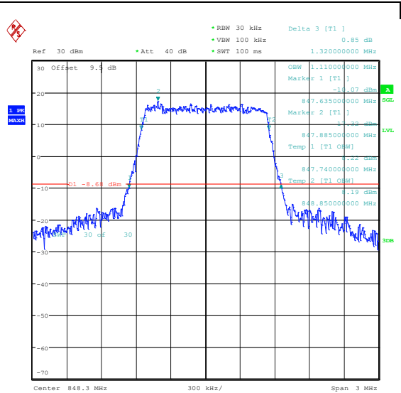
Band26(824-849)-1.4MHz-16QAM-27033-6RB#0-P PASS
