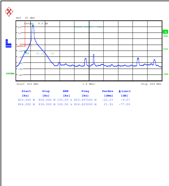
Band26_15MHz_QPSK_26865_1RB#0
