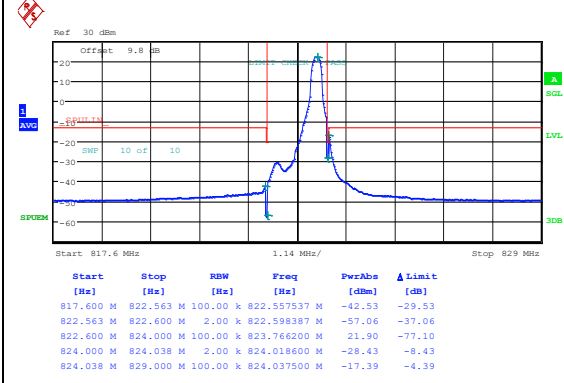
Band26_1.4MHz_QPSK_26783_1RB#0
