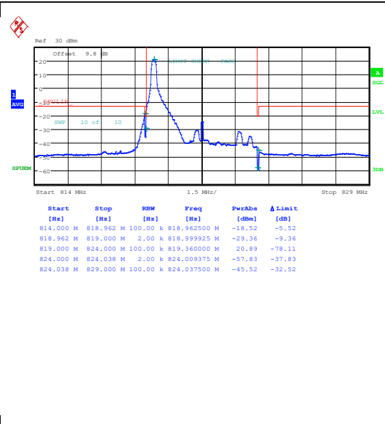
Band26_5MHz_16QAM_26765_1RB#0
