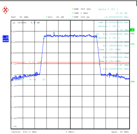
Band26(824-849)-15MHz-16QAM-26865-75RB#0-P PASS
