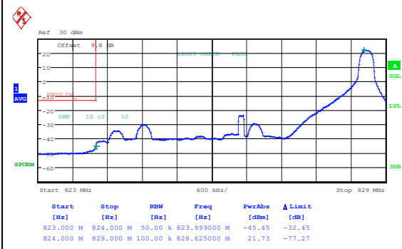
Band26_5MHz_QPSK_26815_1RB#0
