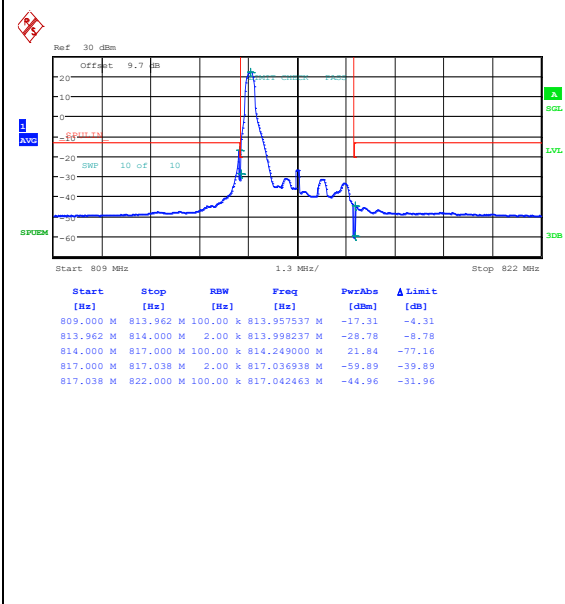
Band26_3MHz_QPSK_26705_1RB#0
