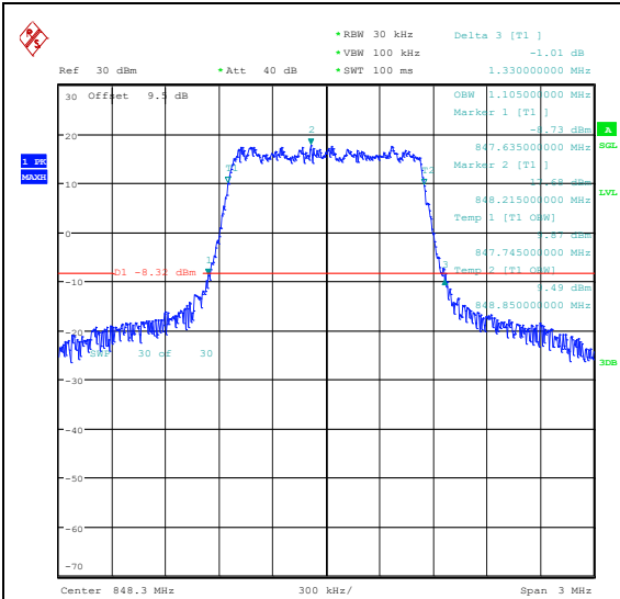
Band26(824-849)-1.4MHz-QPSK-27033-6RB#0-P ASS
