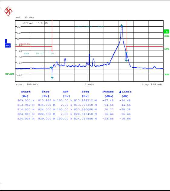
Band26_10MHz_16QAM_26740_1RB#49
