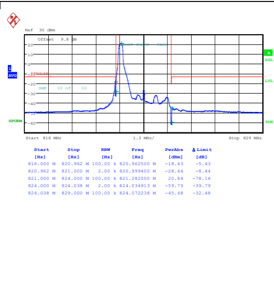
Band26_3MHz_16QAM_26775_1RB#0
