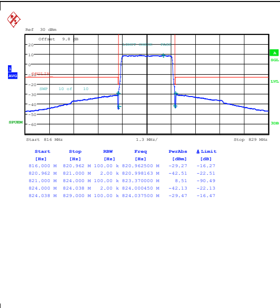
Band26_3MHz_16QAM_26775_15RB#0
