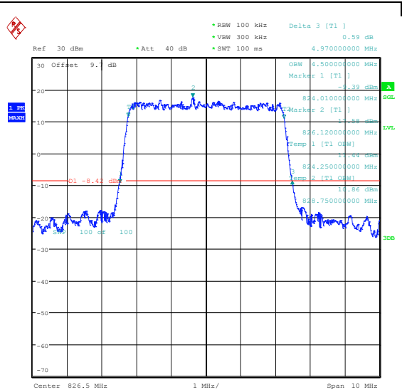
Band26(824-849)-5MHz-16QAM-26815-25RB#0-P ASS
