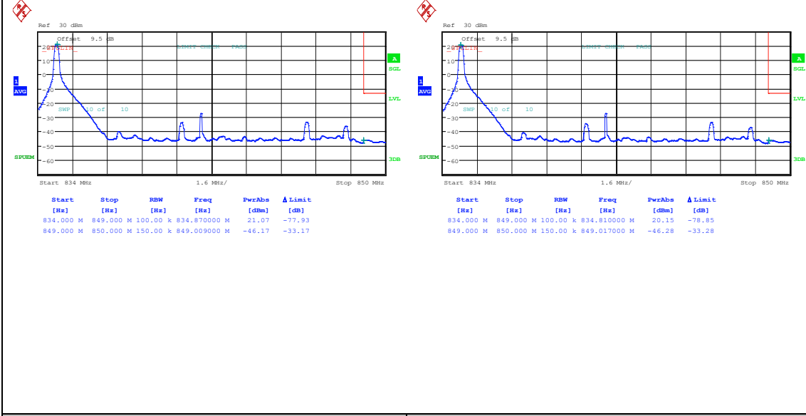
Band26_15MHz_QPSK_26965_1RB#0 Band26_15MHz_16QAM_26965_1RB#0
