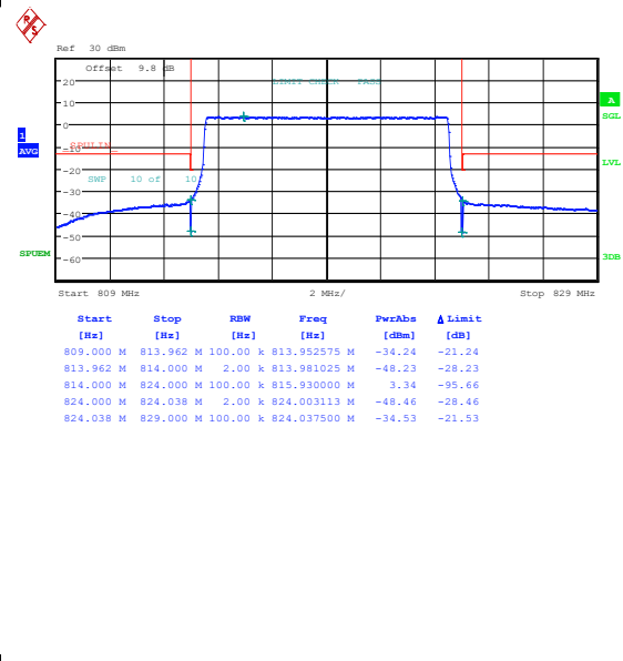
Band26_10MHz_16QAM_26740_50RB#0
