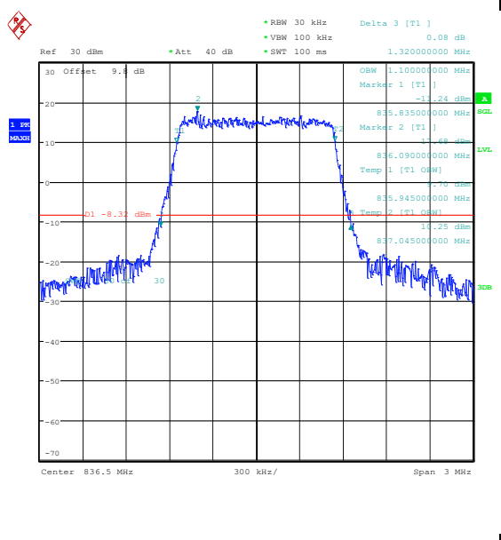
Band26(824-849)-1.4MHz-16QAM-26915-6RB#0-P PASS
