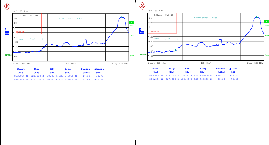
Band26_3MHz_QPSK_26805_1RB#14
