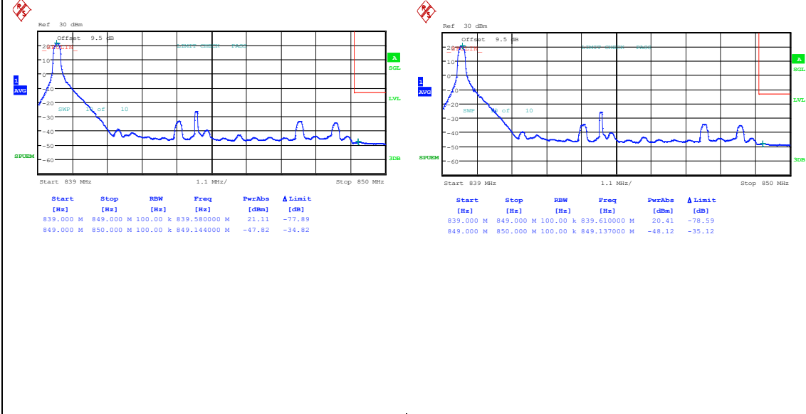
Band26_10MHz_QPSK_26990_1RB#0 Band26_10MHz_16QAM_26990_1RB#0
