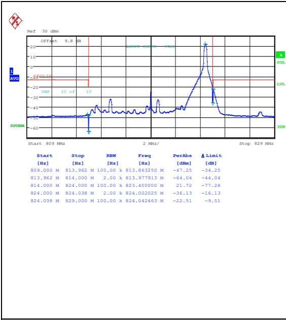
Band26_10MHz_QPSK_26740_1RB#49
