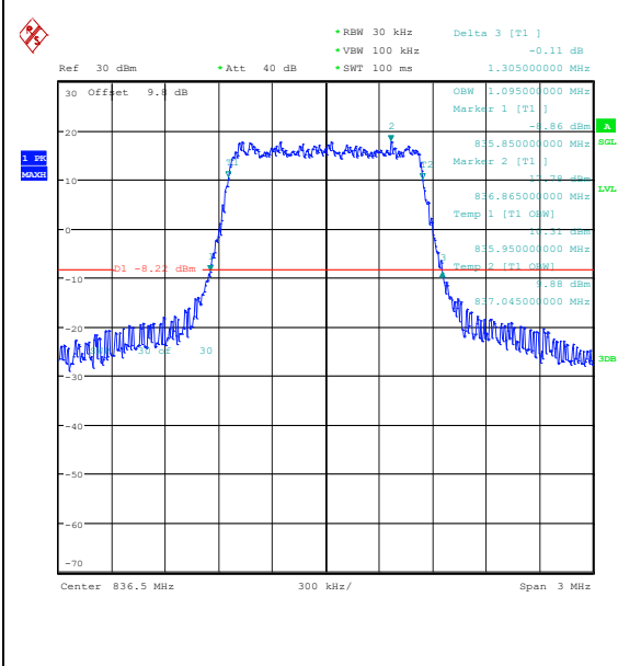
Band26(824-849)-1.4MHz-QPSK-26915-6RB#0-P ASS
