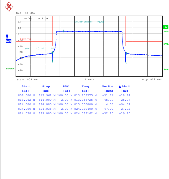
Band26_10MHz_QPSK_26740_50RB#0
