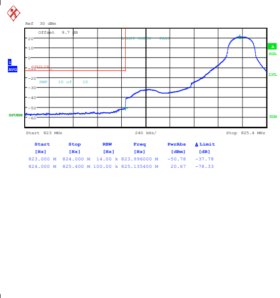
Band26_1.4MHz_16QAM_26797_1RB#5
