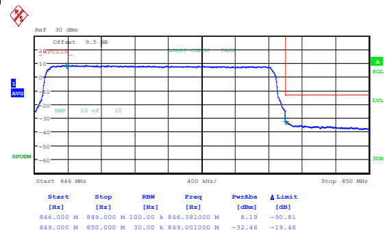
Band26_3MHz_16QAM_27025_1RB#14
