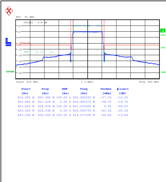
Band26_3MHz_QPSK_26775_15RB#0
