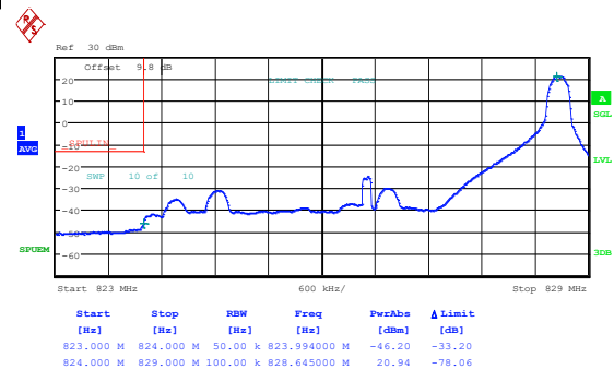
Band26_5MHz_16QAM_26815_1RB#0
