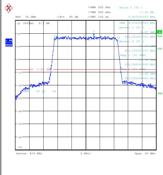
Band26(814-824)-10MHz-QPSK-26740-50RB#0-P ASS
