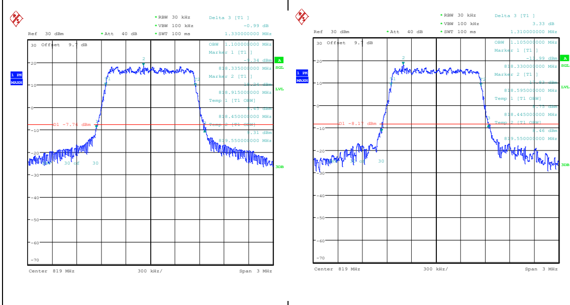
Band26(814-824)-1.4MHz-QPSK-26740-6RB#0-P ASS Band26(814-824)-1.4MHz-16QAM-26740-6RB#0-P PASS
