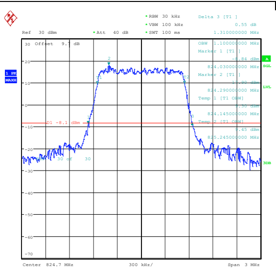
Band26(824-849)-1.4MHz-16QAM-26797-6RB#0-P PASS
