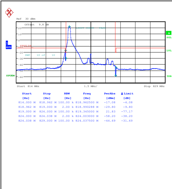
Band26_5MHz_QPSK_26765_1RB#0
