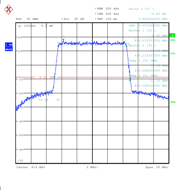
Band26(814-824)-10MHz-16QAM-26740-50RB#0-P PASS
