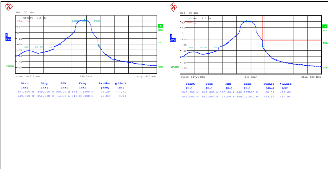
Band26_1.4MHz_QPSK_27033_1RB#5
