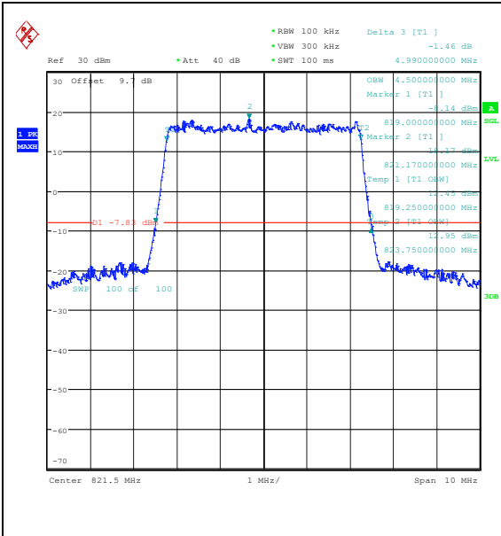
Band26(814-824)-5MHz-QPSK-26765-25RB#0-P ASS
