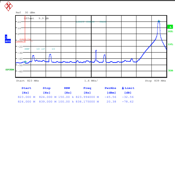
Band26_15MHz_16QAM_26865_1RB#74
