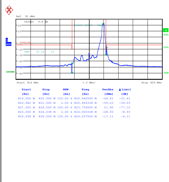
Band26_3MHz_QPSK_26775_1RB#14
