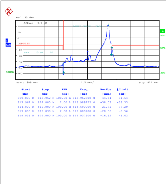
Band26_5MHz_QPSK_26715_1RB#24
