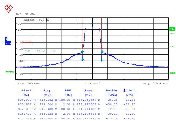
Band26_1.4MHz_16QAM_26697_1RB#5
