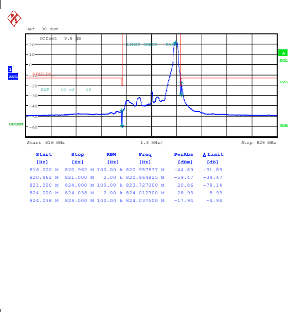
Band26_3MHz_16QAM_26775_1RB#14
