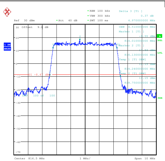
Band26(814-824)-5MHz-16QAM-26715-25RB#0-P
