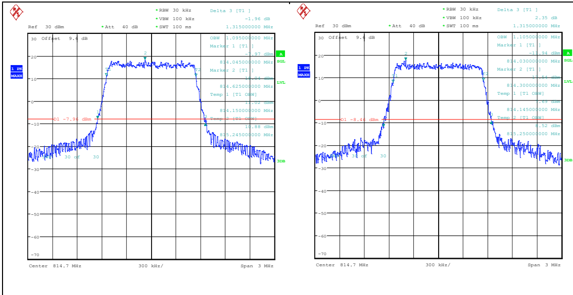
Band26(814-824)-1.4MHz-QPSK-26697-6RB#0-P ASS Band26(814-824)-1.4MHz-16QAM-26697-6RB#0-P PASS
