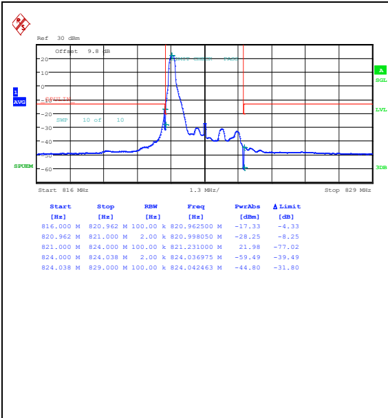
Band26_3MHz_QPSK_26775_1RB#0
