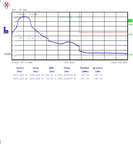
Band26_1.4MHz_16QAM_27033_1RB#0
