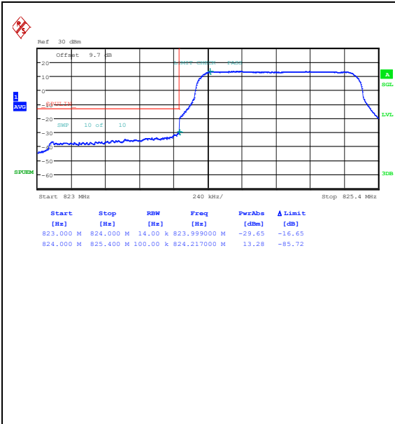
Band26_1.4MHz_QPSK_26797_6RB#0
