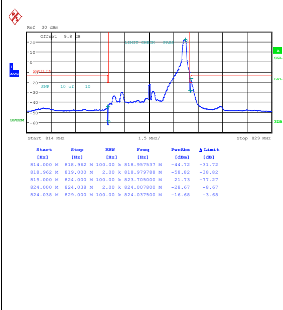
Band26_5MHz_QPSK_26765_1RB#24
