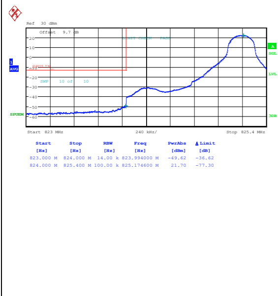
Band26_1.4MHz_QPSK_26797_1RB#5
