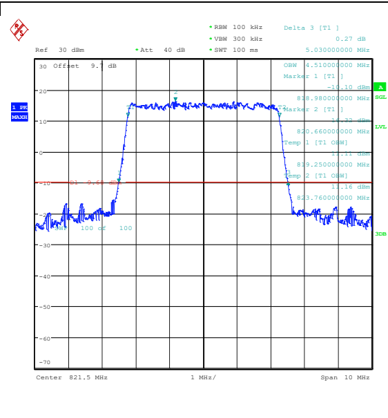
Band26(814-824)-5MHz-16QAM-26765-25RB#0-P ASS
