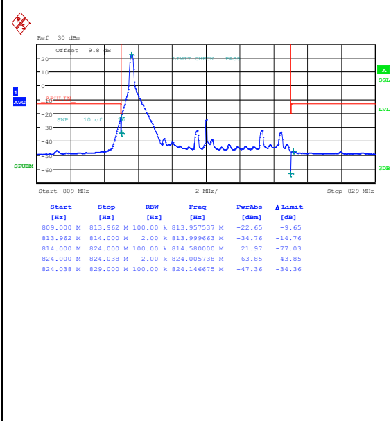
Band26_10MHz_QPSK_26740_1RB#0
