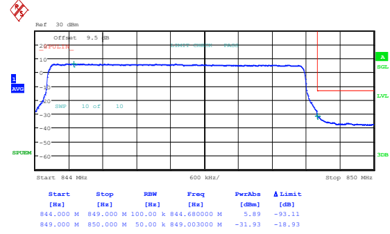
Band26_5MHz_16QAM_27015_1RB#24
