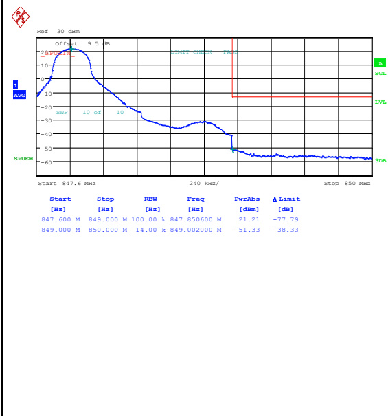
Band26_1.4MHz_QPSK_27033_1RB#0
