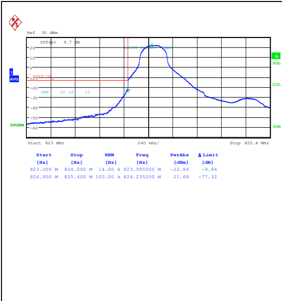
Band26_1.4MHz_QPSK_26797_1RB#0
