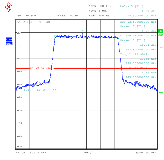
Band26(824-849)-15MHz-QPSK-26865-75RB#0-P ASS
