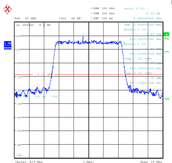
Band26(814-824)-5MHz-16QAM-26715-25RB#0-P
