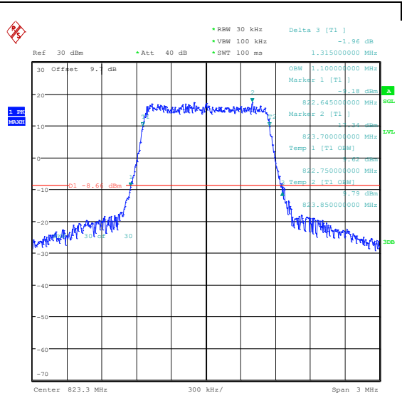
Band26(814-824)-1.4MHz-16QAM-26783-6RB#0-P PASS
