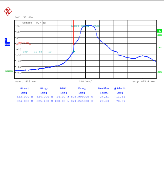
Band26_1.4MHz_16QAM_26797_1RB#0
