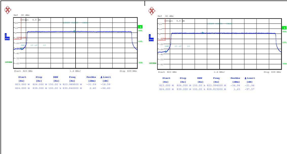
Band26_15MHz_QPSK_26865_75RB#0 Band26_15MHz_16QAM_26865_75RB#0
