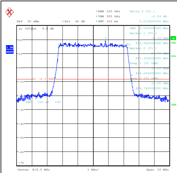
Band26(814-824)-5MHz-QPSK-26715-25RB#0-P
