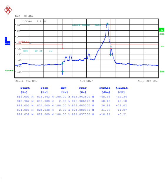
Band26_5MHz_16QAM_26765_1RB#24
