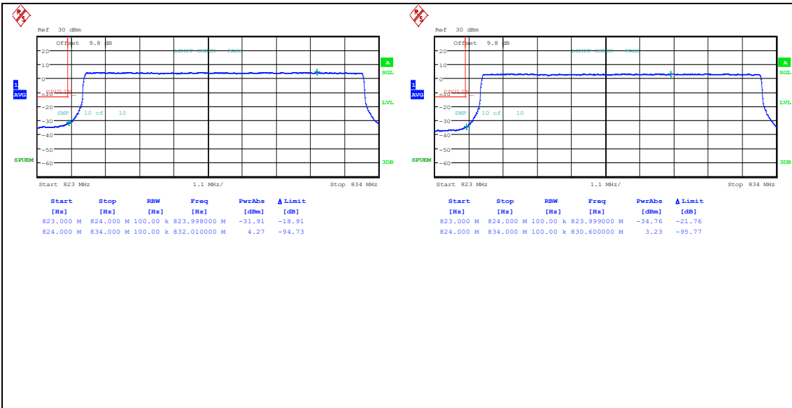
Band26_10MHz_QPSK_26840_50RB#0 Band26_10MHz_16QAM_26840_50RB#0
