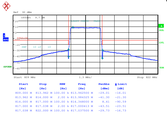
Band26_3MHz_16QAM_26705_1RB#14
