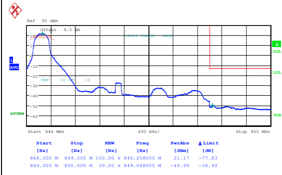
Band26_3MHz_QPSK_26805_15RB#0
