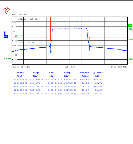
Band26_5MHz_16QAM_26765_25RB#0
