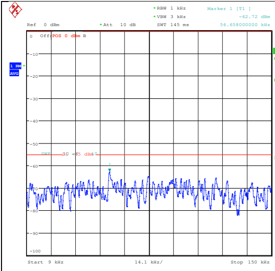
Band41_15MHz_QPSK_40115_1RB#74_0.009~0.15_0.009~0.15
