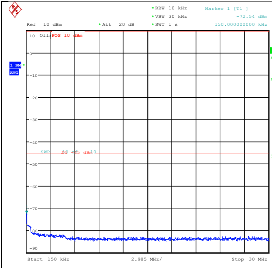
Band41_20MHz_16QAM_40140_1RB#99_0.15~30_0.15~30
