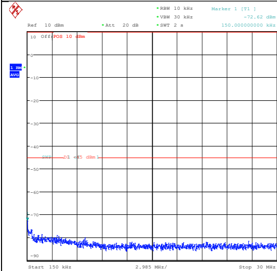
Band41_10MHz_QPSK_41190_50RB#0_20000~27000_20000~27000
