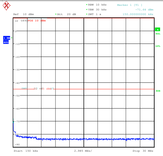
Band41_20MHz_QPSK_40140_1RB#0_0.15~30_0.15~30
