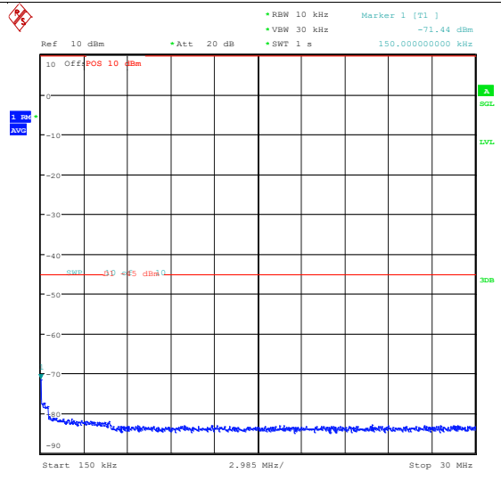
Band41_15MHz_QPSK_40115_1RB#74_0.15~30_0.15~30
