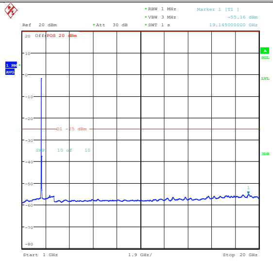
Band41_20MHz_QPSK_40140_100RB#0_0.15~3_0_0.15~30
