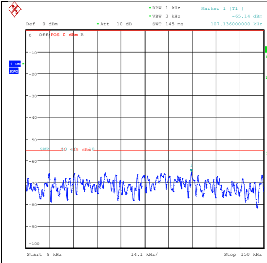
Band41_15MHz_QPSK_40590_1RB#0_0.009~0.15_0.009~0.15
