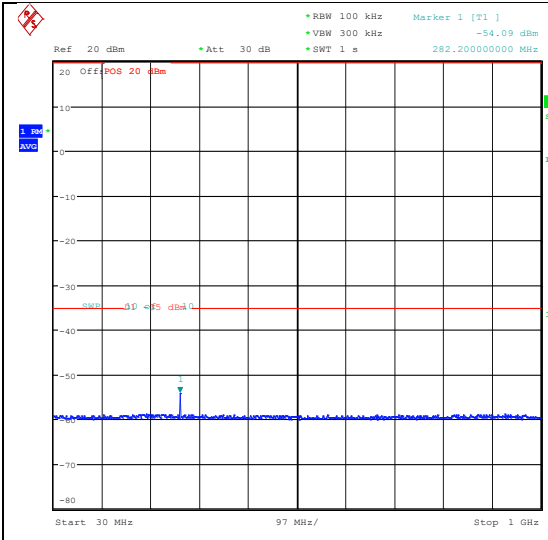
Band41_15MHz_QPSK_40590_1RB#74_30~100 0_30~1000
