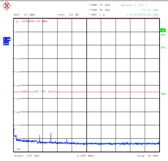
Band41_15MHz_QPSK_40590_75RB#0_0.15~30_0.15~30
