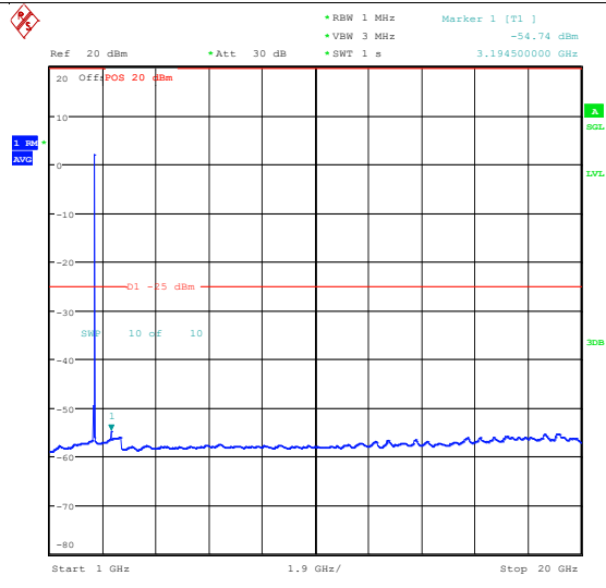
Band41_15MHz_QPSK_40590_1RB#74_1000~20000 000_1000~20000
