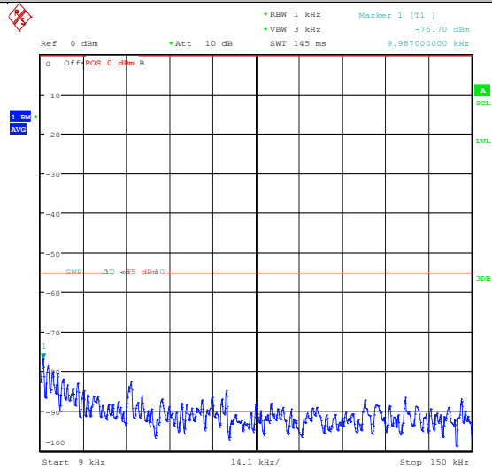
Band41_20MHz_QPSK_40590_100RB#0_1000~2 0000_1000~20000
