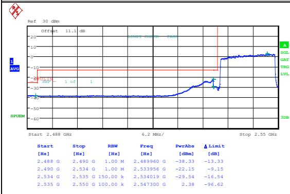
Band41_15MHz_QPSK_40115_1RB#74
