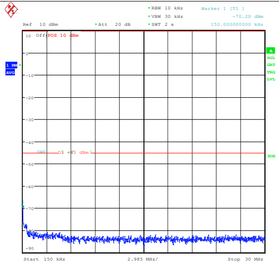
Band41_10MHz_QPSK_40590_1RB#49_0.15~30_0.15~30
