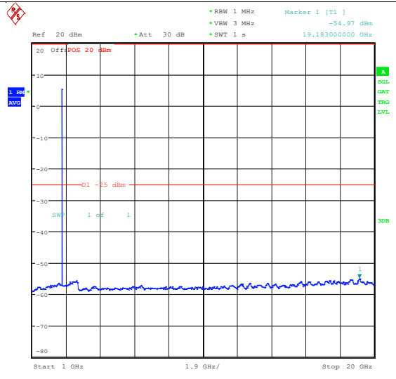
Band41_5MHz_QPSK_41215_1RB#0_1000~2000_0_1000~20000
