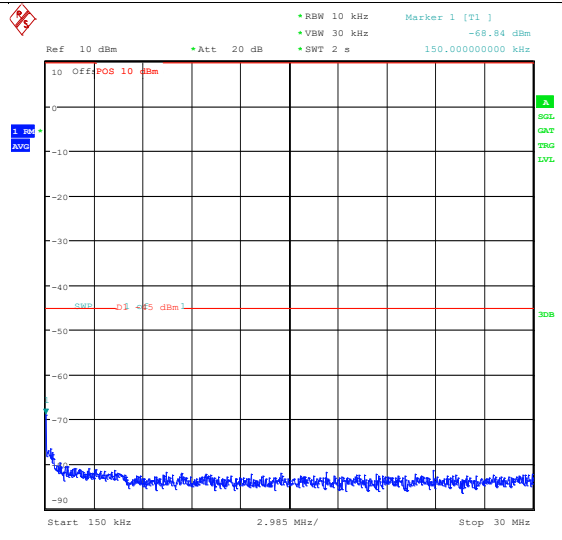
Band41_5MHz_QPSK_40590_1RB#0_0.15~30_0. 15~30
