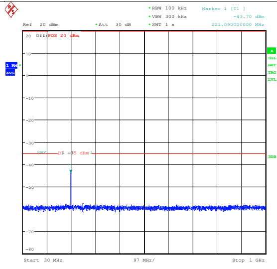
Band41_5MHz_16QAM_40065_1RB#0_30~1000_ 30~1000
