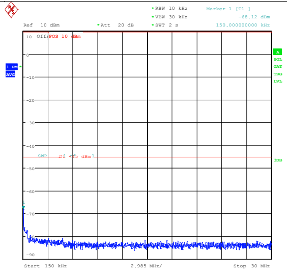
Band41_10MHz_QPSK_40090_1RB#0_0.15~30_0.15~30
