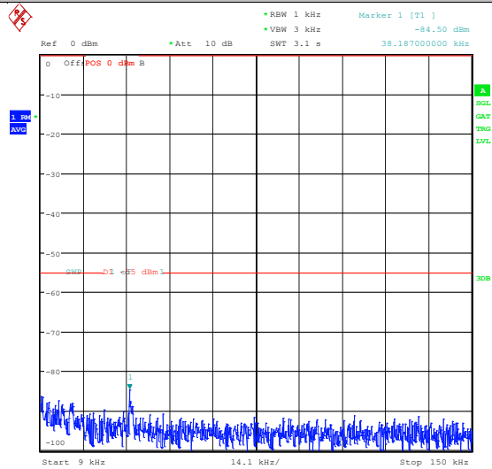
Band41_5MHz_QPSK_41215_25RB#0_1000~200 00_1000~20000
