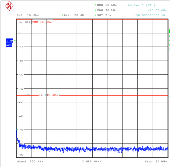
Band41_5MHz_16QAM_40590_1RB#24_0.15~3 0_0.15~30
