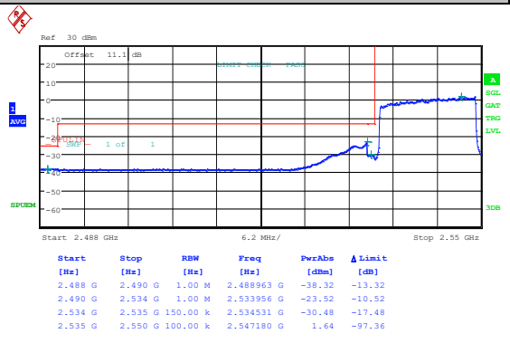
Band41_15MHz_16QAM_40115_1RB#74
