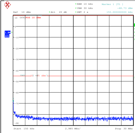
Band41_5MHz_16QAM_40065_1RB#0_0.15~30 _0.15~30
