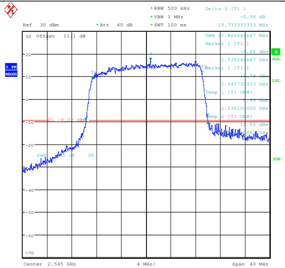
Band41(2535-2655)-15MHz-16QAM-41165-75RB# 0-PASS
