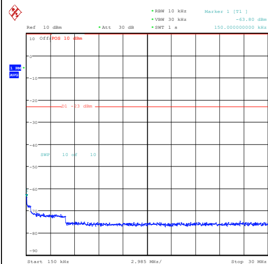
Band26_3MHz_QPSK_26805_1RB#0_3000~10000_00_3000~10000
