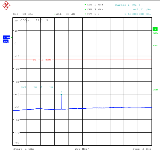
Band26_1.4MHz_QPSK_27033_1RB#0_1000~3000 00_1000~3000
