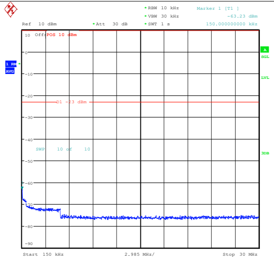
Band26_3MHz_QPSK_26705_1RB#0_0.15~30_0_15~30
