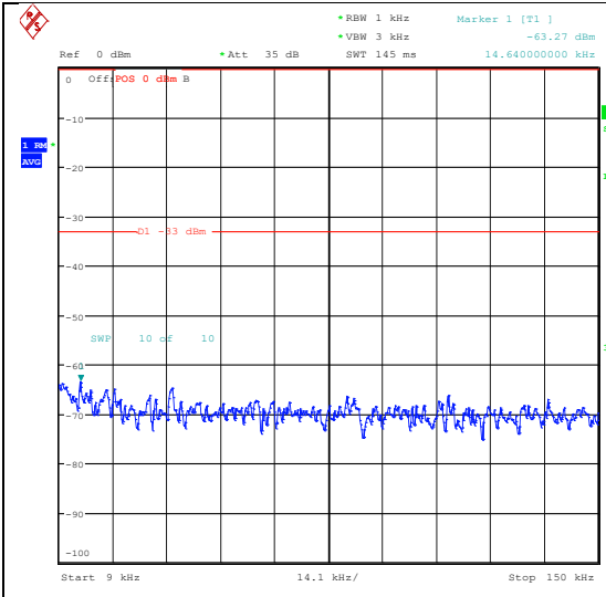
Band26_5MHz_QPSK_26915_1RB#0_0.009~0.1 5_0.009~0.15
