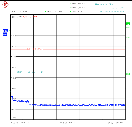
Band26_15MHz_QPSK_26915_1RB#0_0.15~30_0.15~30
