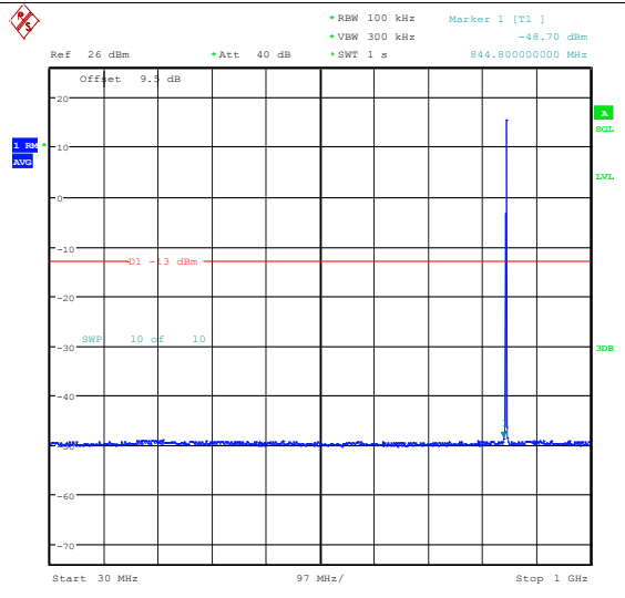
Band26_1.4MHz_16QAM_27033_1RB#0_30~100 0_30~1000
