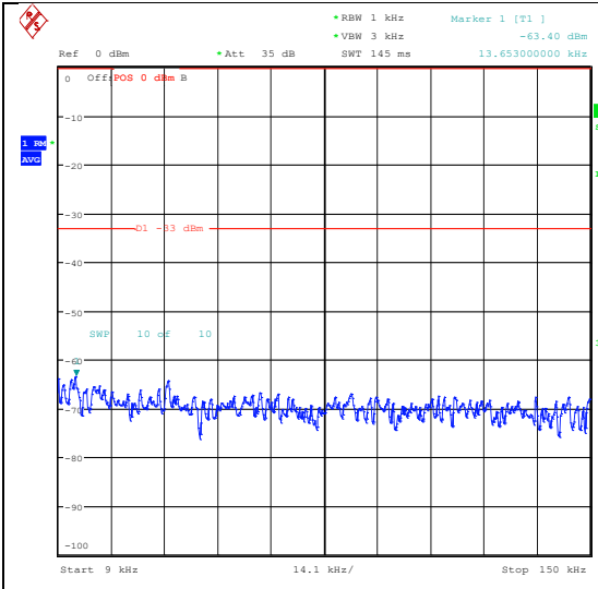
Band26_3MHz_QPSK_26805_1RB#0_0.009~0.15 5_0.009~0.15
