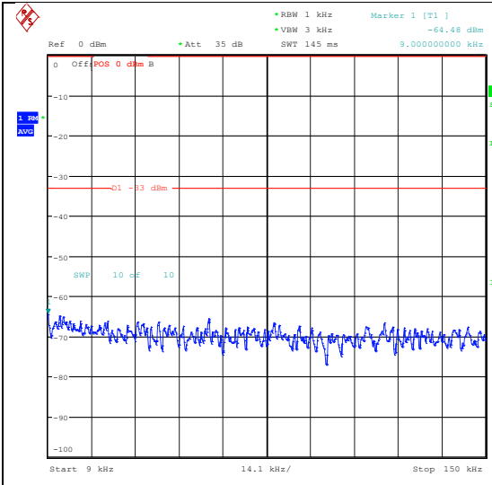
Band26_3MHz_QPSK_26705_1RB#0_0.009~0.15_5_0.009~0.15
