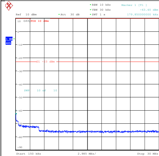
Band26_3MHz_QPSK_27025_1RB#0_3000~10000_00_3000~10000
