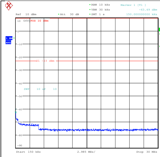
Band26_5MHz_16QAM_26715_1RB#0_0.15~30 _0.15~30
