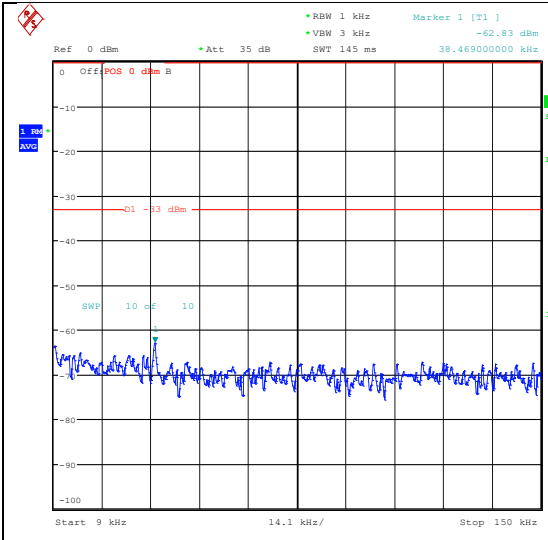
Band26_10MHz_QPSK_26840_1RB#0_0.009~0.15_0.009~0.15
