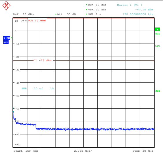
Band26_3MHz_QPSK_26805_1RB#0_0.15~30_0. 15~30
