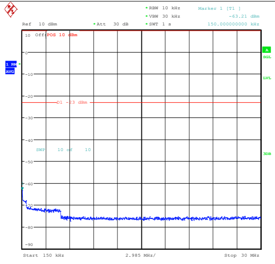
Band26_1.4MHz_QPSK_26915_1RB#0_0.15~30_0.15~30
