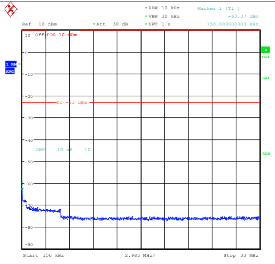
Band26_5MHz_QPSK_26915_1RB#0_0.15~30_0. 15~30
