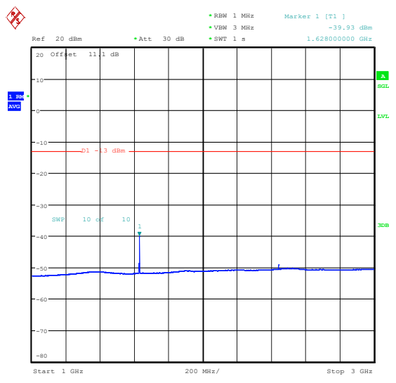
Band26_3MHz_QPSK_26705_1RB#0_0.15~30_0_15~30
