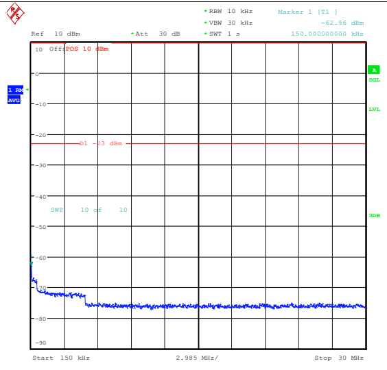
Band26_10MHz_QPSK_26840_1RB#0_0.15~30_0.15~30
