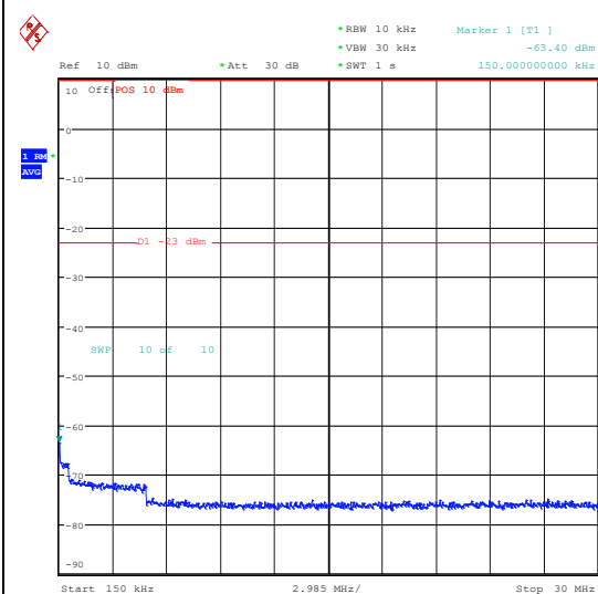
Band26_10MHz_QPSK_26840_1RB#0_3000~10000_000_3000~10000
