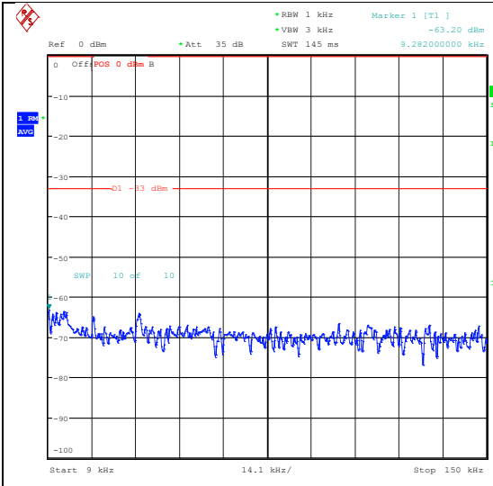
Band26_1.4MHz_QPSK_26915_1RB#0_0.009~0.15_0.009~0.15
