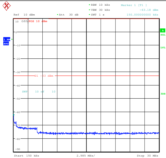
Band25_3MHz_16QAM_26055_1RB#0_3000~2000_00_3000~20000
