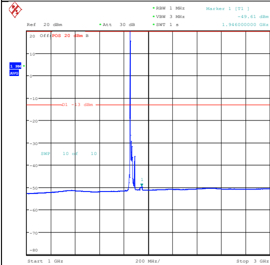
Band25_20MHz_16QAM_26140_1RB#0_0.15~3 0_0.15~30
