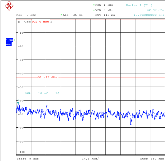
Band25_5MHz_16QAM_26365_1RB#0_1000~3000_00_1000~3000
