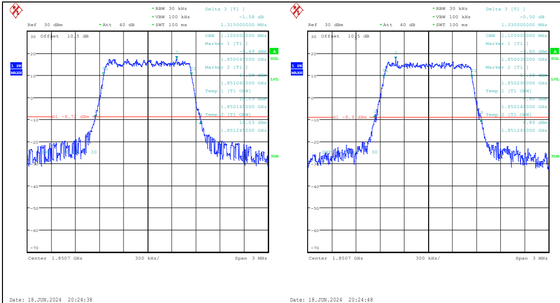
Band25-1.4MHz-QPSK-26047-6RB#0-PASS Band25-1.4MHz-16QAM-26047-6RB#0-PASS
