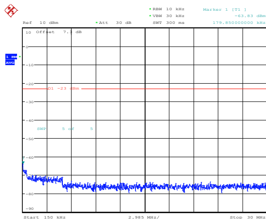
Band66-20MHz-16QAM-132322-1RB#0-Range2:0.15~30MHz
