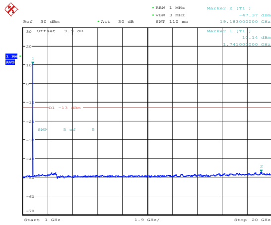
Band66-3MHz-16QAM-132322-1RB#0-Range4:1000~20000MHz
