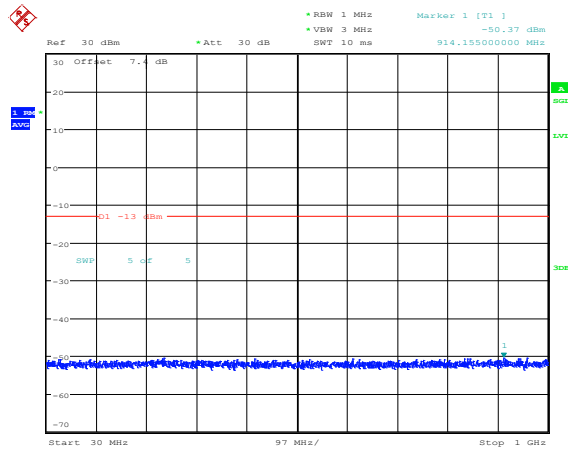
Band66-3MHz-QPSK-132657-1RB#0-Range3:30~1000MHz
