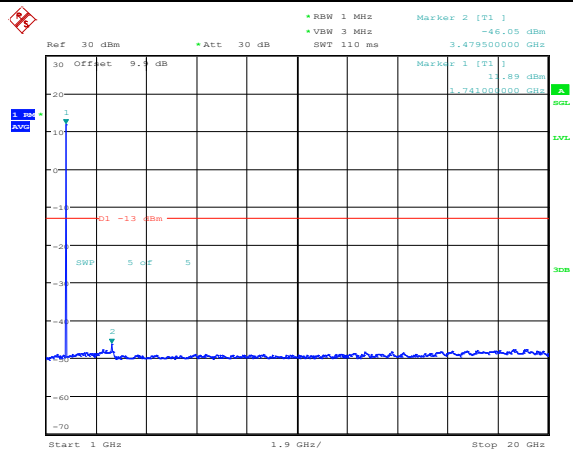
Band66-5MHz-QPSK-132322-1RB#0-Range4:1000~20000MHz
