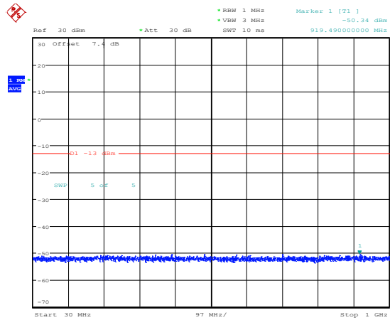
Band66-15MHz-QPSK-132047-1RB#0-Range3:30~1000MHz
