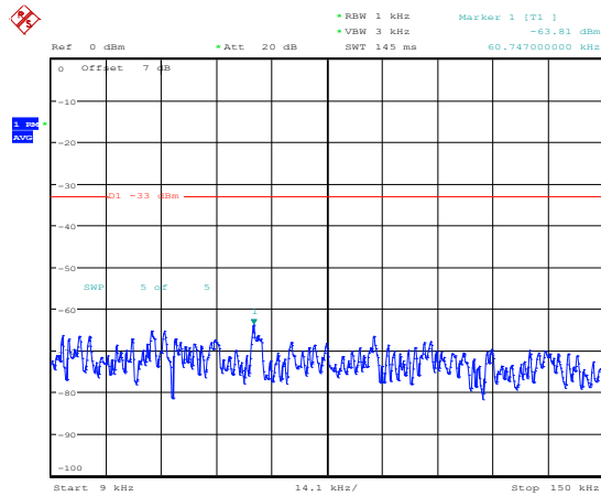
Band66-3MHz-16QAM-132657-1RB#0-Range1:0.009~0.15MHz
