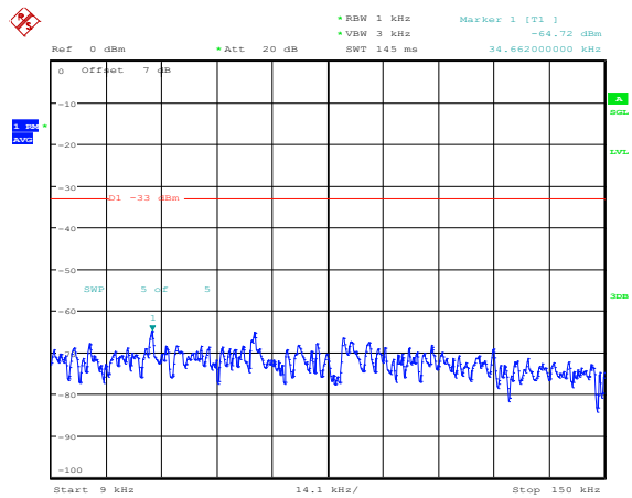
Band66-20MHz-16QAM-132572-1RB#0-Range1:0.009~0.15MHz
