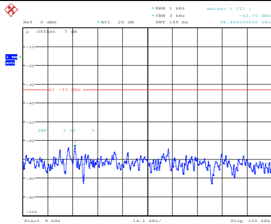
Band66-20MHz-16QAM-132322-1RB#0-Range1:0.009~0.15MHz
