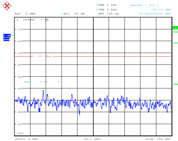
Band66-10MHz-16QAM-132622-1RB#0-Range1:0.009~0.15MHz
