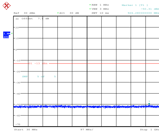
Band66-5MHz-16QAM-132647-1RB#0-Range3:30~1000MHz
