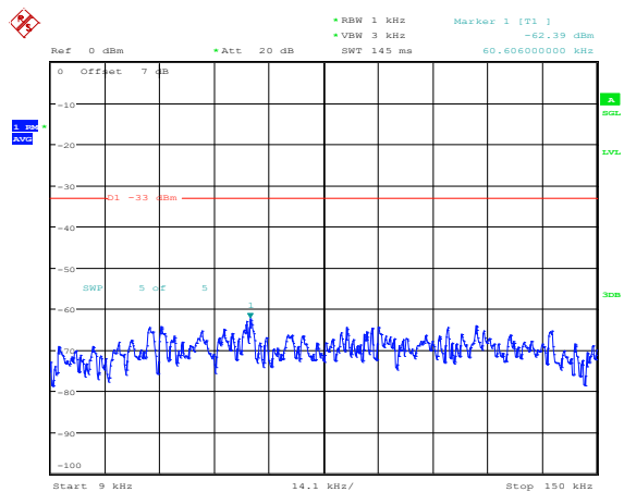
Band66-5MHz-QPSK-132647-1RB#0-Range1:0.009~0.15MHz
