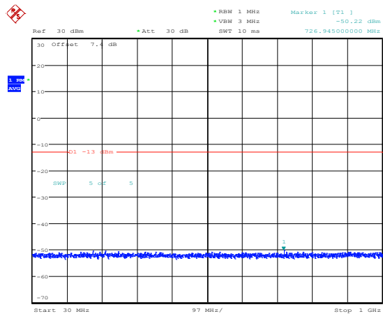
Band66-5MHz-16QAM-131997-1RB#0-Range3:30~1000MHz
