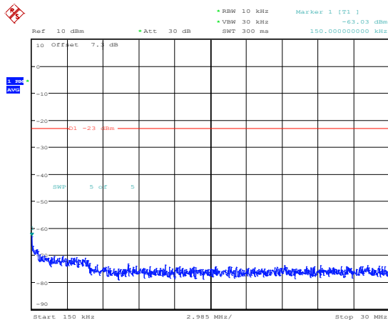
Band66-10MHz-16QAM-132322-1RB#0-Range2:0.15~30MHz
