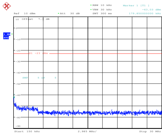
Band66-15MHz-QPSK-132047-1RB#0-Range2:0.15~30MHz
