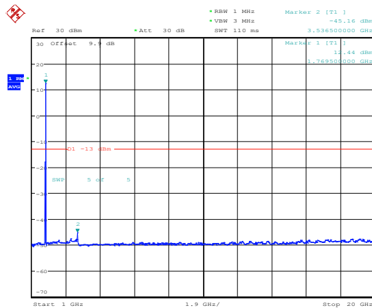
Band66-10MHz-QPSK-132622-1RB#0-Range4:1000~20000MHz
