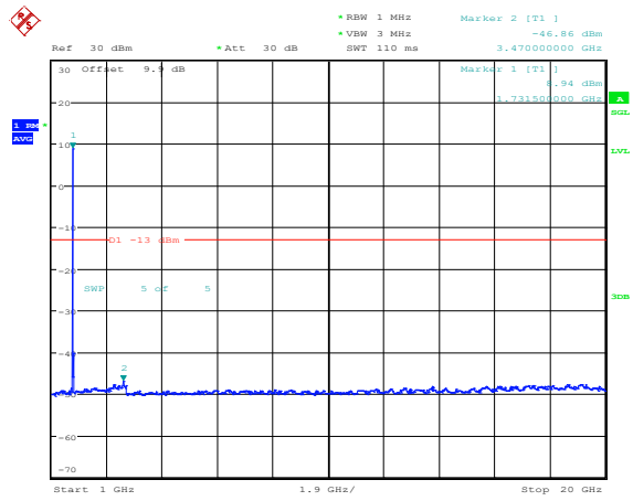
Band66-20MHz-16QAM-132322-1RB#0-Range4:1000~20000MHz
