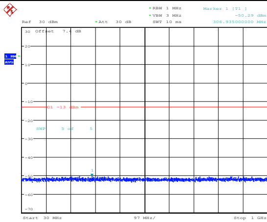
Band66-5MHz-QPSK-132647-1RB#0-Range3:30~1000MHz
