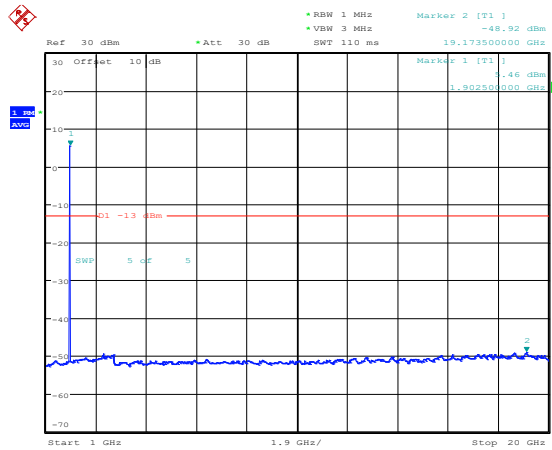
Band2-1.4MHz-16QAM-19193-1RB#0-Range4:1000~20000MHz
