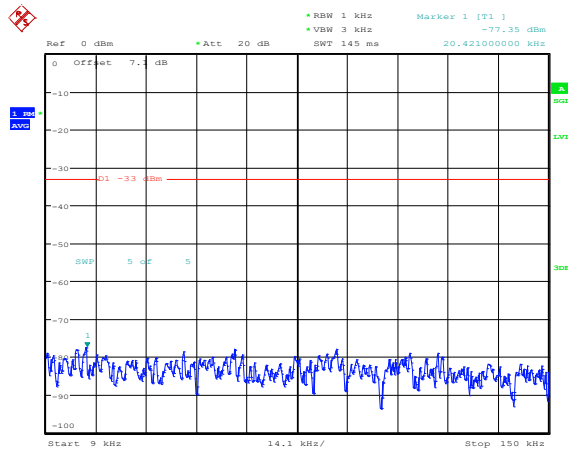
Band2-1.4MHz-16QAM-18900-1RB#0-Range1:0.009~0.15MHz
