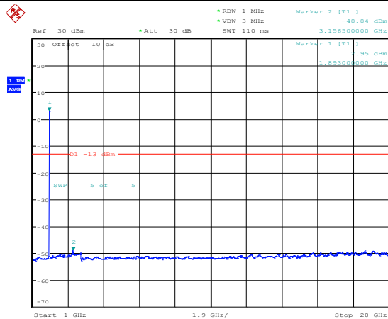
Band2-10MHz-16QAM-19150-1RB#0-Range4:1000~20000MHz
