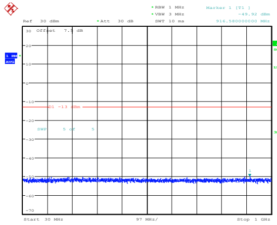
Band2-5MHz-16QAM-19175-1RB#0-Range3:30~1000MHz
