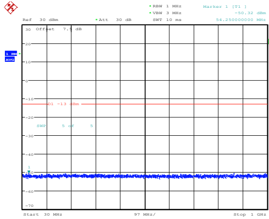
Band2-15MHz-16QAM-18675-1RB#0-Range3:30~1000MHz
