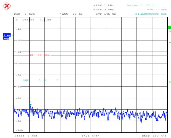
Band2-20MHz-16QAM-18900-1RB#0-Range1:0.009~0.15MHz
