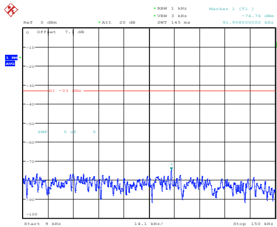
Band2-1.4MHz-16QAM-19193-1RB#0-Range1:0.009~0.15MHz
