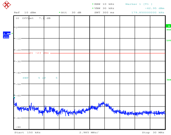
Band2-1.4MHz-16QAM-18900-1RB#0-Range2:0.15~30MHz
