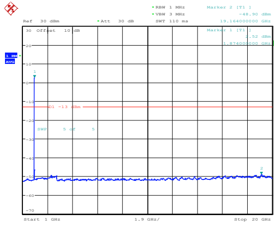
Band2-1.4MHz-16QAM-18900-1RB#0-Range4:1000~20000MHz
