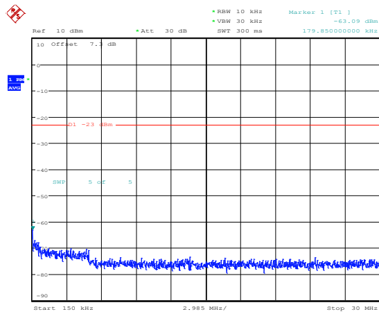
Band25-20MHz-16QAM-26140-1RB#0-Range2:0.15~30MHz
