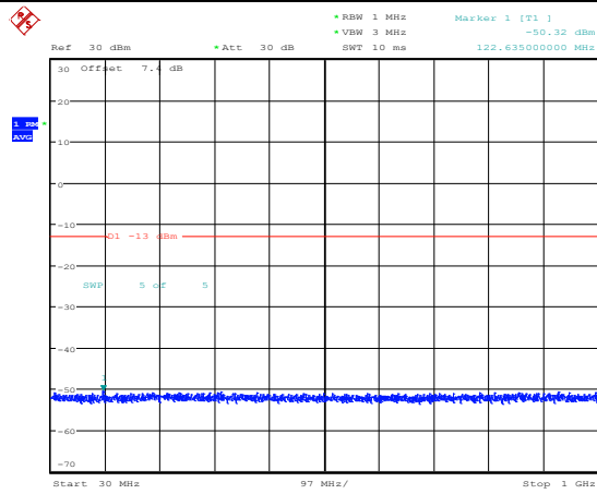
Band25-15MHz-16QAM-26615-1RB#0-Range3:30~1000MHz
