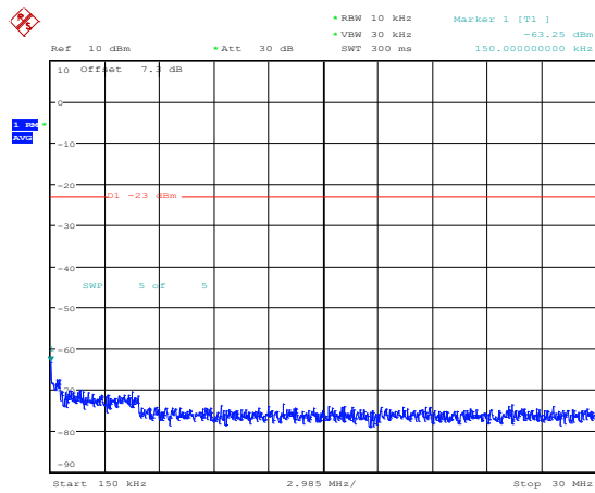
Band25-15MHz-16QAM-26115-1RB#0-Range2:0.15~30MHz
