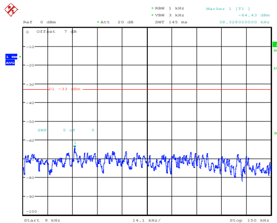
Band25-20MHz-16QAM-26590-1RB#0-Range1:0.009~0.15MHz
