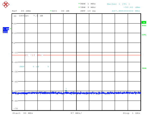
Band25-10MHz-QPSK-26090-1RB#0-Range3:30~1000MHz
