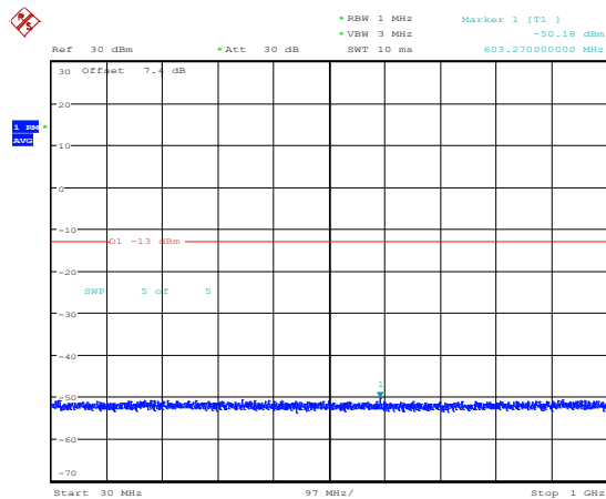
Band25-10MHz-16QAM-26090-1RB#0-Range3:30~1000MHz
