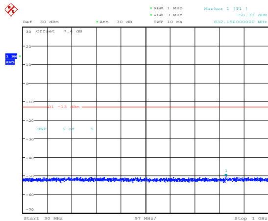
Band25-15MHz-16QAM-26115-1RB#0-Range3:30~1000MHz
