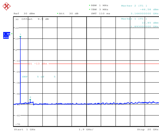
Band25-15MHz-16QAM-26615-1RB#0-Range4:1000~20000MHz
