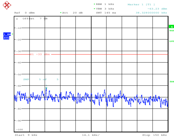
Band25-10MHz-16QAM-26640-1RB#0-Range1:0.009~0.15MHz
