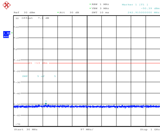
Band25-20MHz-16QAM-26140-1RB#0-Range3:30~1000MHz
