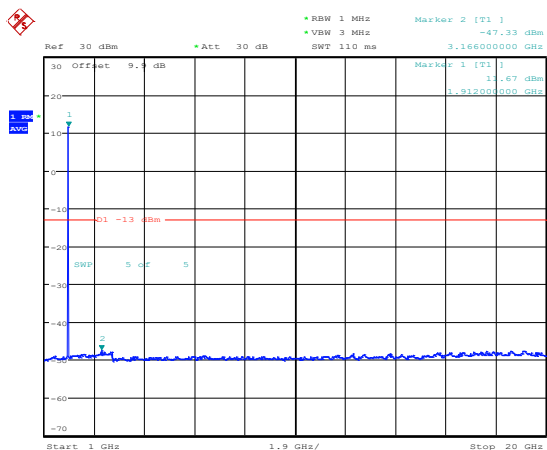
Band25-3MHz-16QAM-26675-1RB#0-Range4:1000~20000MHz
