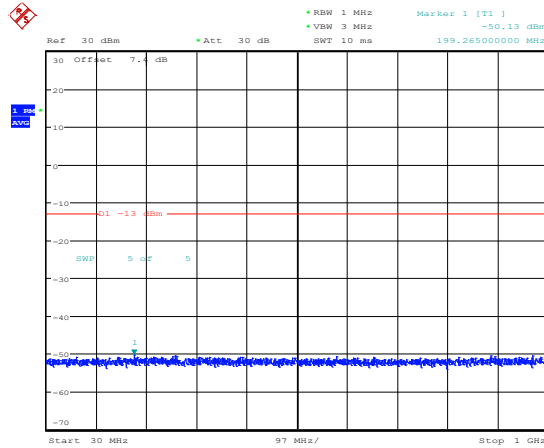
Band25-5MHz-16QAM-26065-1RB#0-Range3:30~1000MHz
