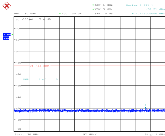
Band25-20MHz-QPSK-26140-1RB#0-Range3:30~1000MHz
