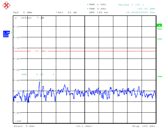
Band25-5MHz-QPSK-26665-1RB#0-Range1:0.009~0.15MHz
