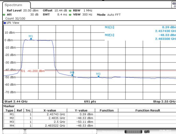
11N20SISO_Ant1_High_2462_Peak
