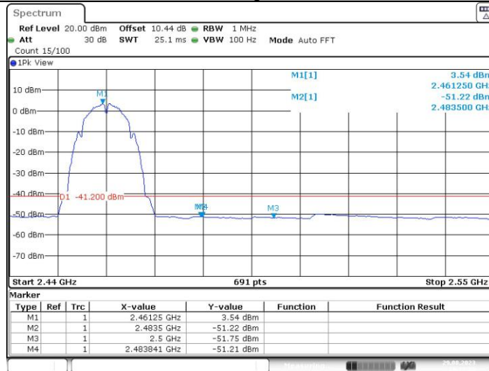
11B_Ant1_High_2462_Peak
