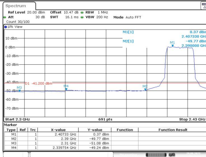
11G_Ant1_Low_2412_Peak
