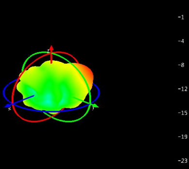
Ant2: 2450Mhz
