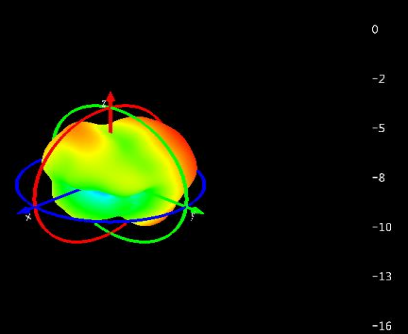
Ant2: 1575Mhz
