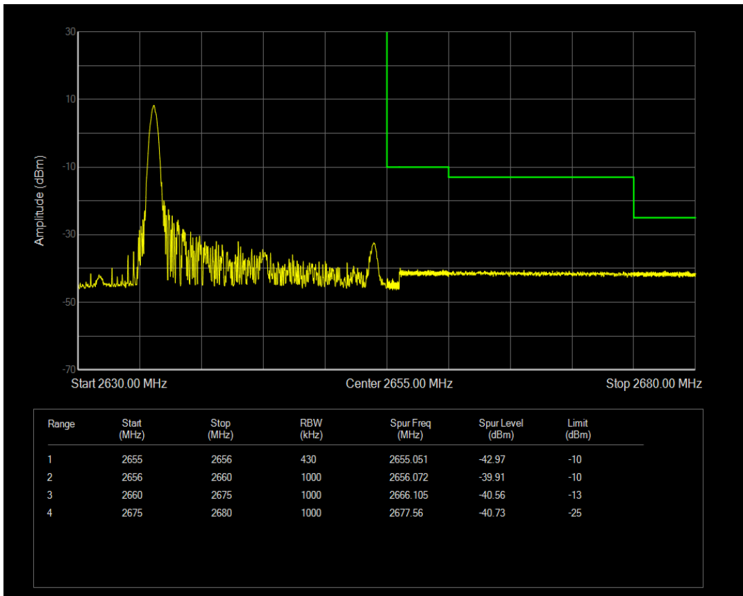
Band41(2535-2655) 16QAM BW=20MHz Channel=41140 RB Size=1 Position=#Max
