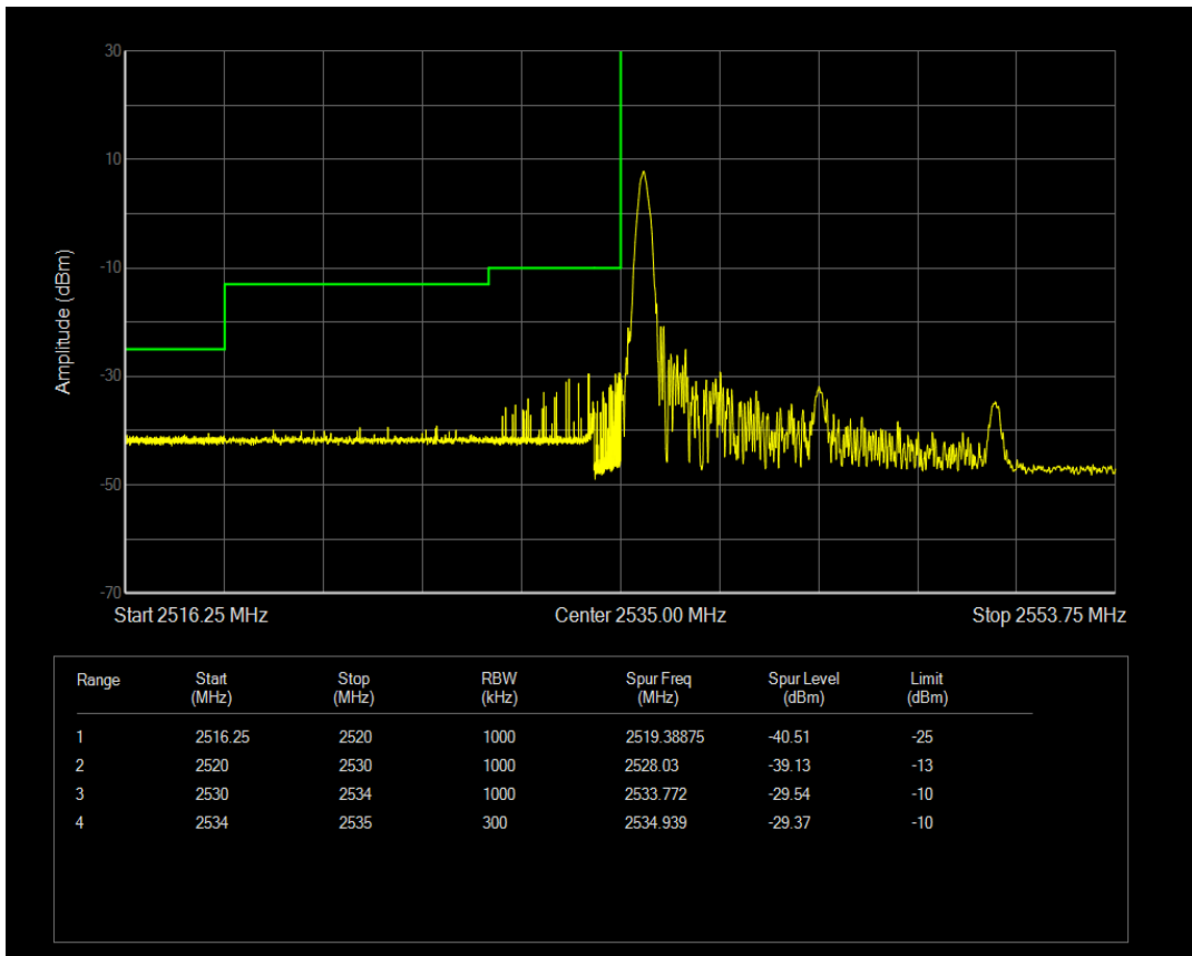
Band41(2535-2655) 16QAM BW=15MHz Channel=40115 RB Size=1 Position=#Max
