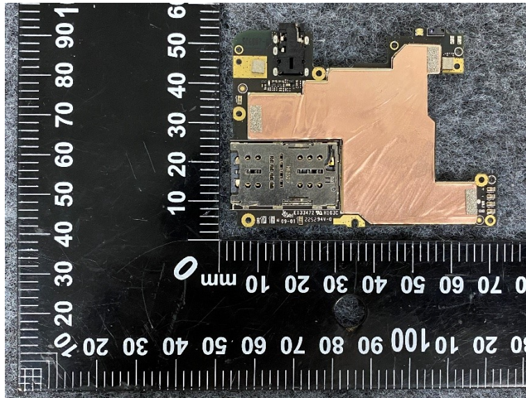
EUT View
