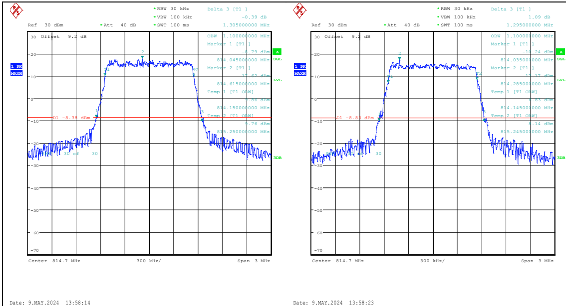
Band26(814-824)-1.4MHz-QPSK-26697-6RB#0-P Band26(814-824)-1.4MHz-16QAM-26697-6RB#0- ASS PASS
