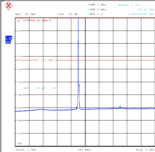
Band25_15MHz_16QAM_26615_1RB#0_0.15~3 0_0.15~30
