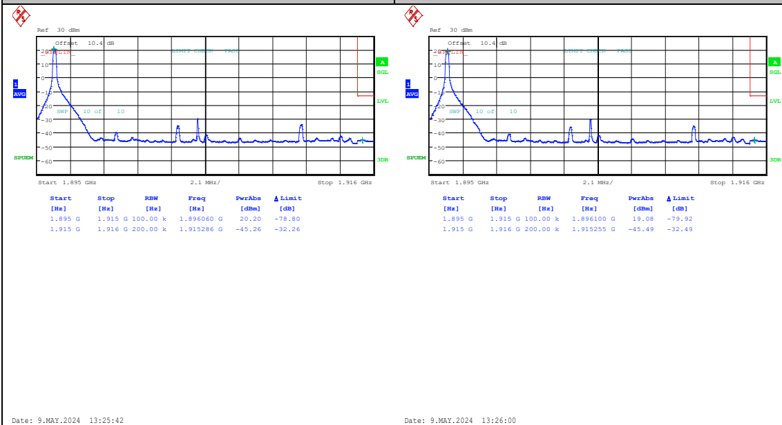
Band25_20MHz_QPSK_26590_1RB#0 Band25_20MHz_16QAM_26590_1RB#0
