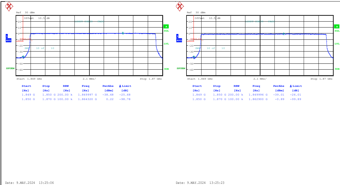
Band25_20MHz_QPSK_26140_100RB#0 Band25_20MHz_16QAM_26140_100RB#0
