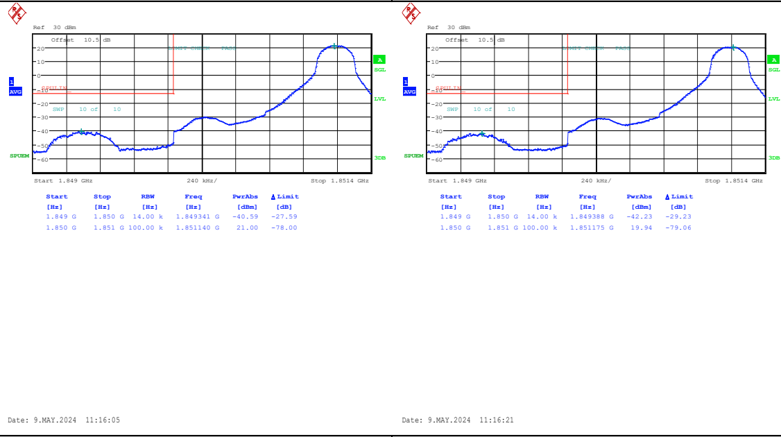
Band25_1.4MHz_QPSK_26047_1RB#5 Band25_1.4MHz_16QAM_26047_1RB#5
