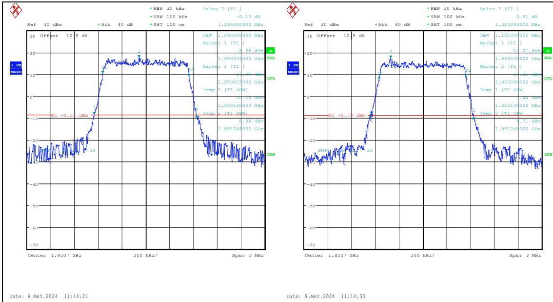
Band25-1.4MHz-QPSK-26047-6RB#0-PASS Band25-1.4MHz-16QAM-26047-6RB#0-PASS
