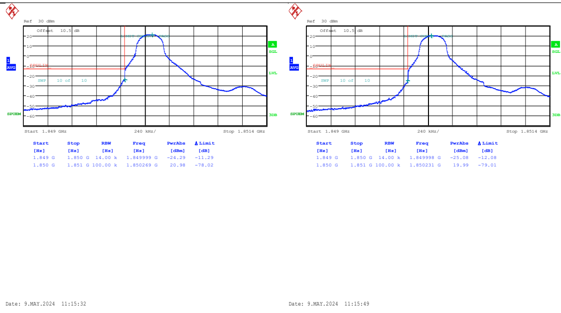
Band25_1.4MHz_QPSK_26047_1RB#0 Band25_1.4MHz_16QAM_26047_1RB#0
