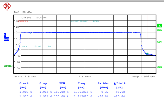
Band25_15MHz_16QAM_26615_1RB#74
