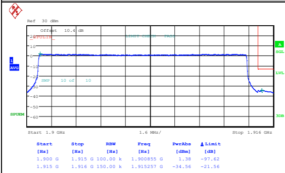
Band25_15MHz_QPSK_26615_1RB#74
