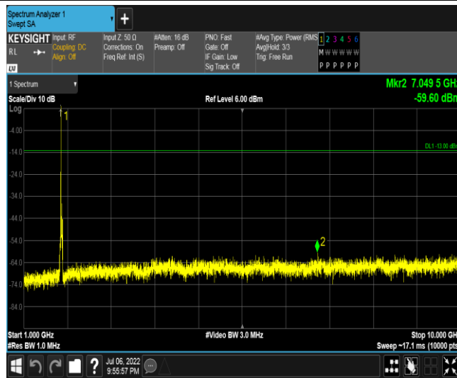
Band66-20MHz-16QAM-132572-1RB#0-Range3:1000~10000MHz
