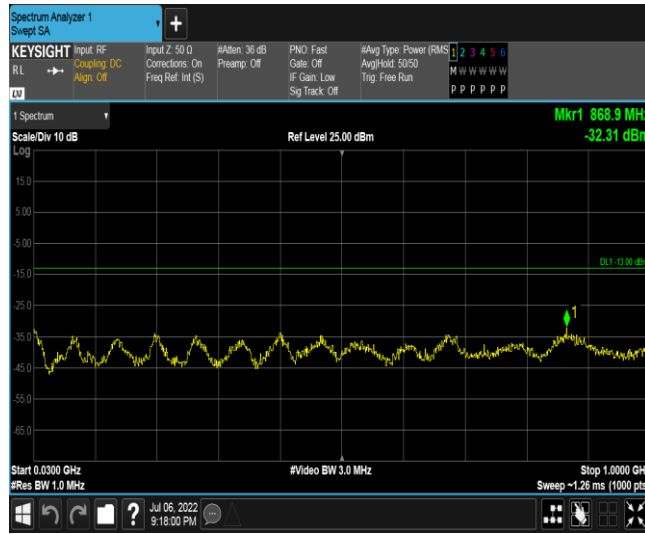
Band66-20MHz-16QAM-132572-1RB#0-Range2:30~1000MHz
