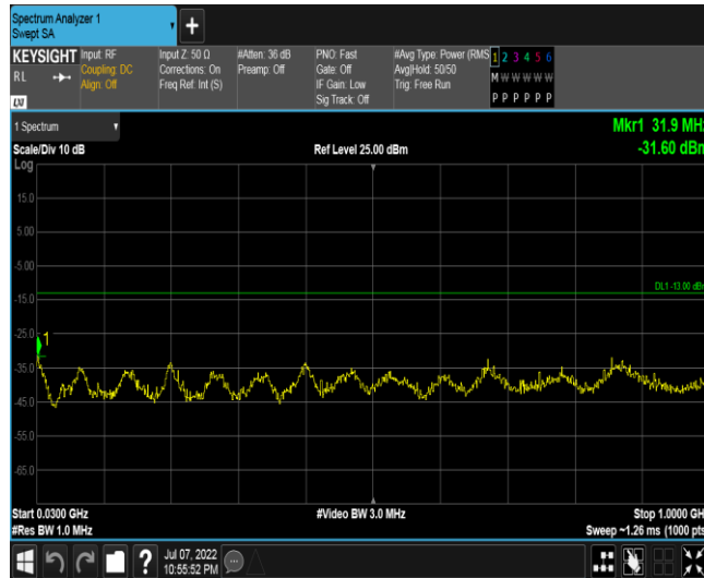
Band66-10MHz-16QAM-132322-1RB#0-Range1:30~1000MHz
