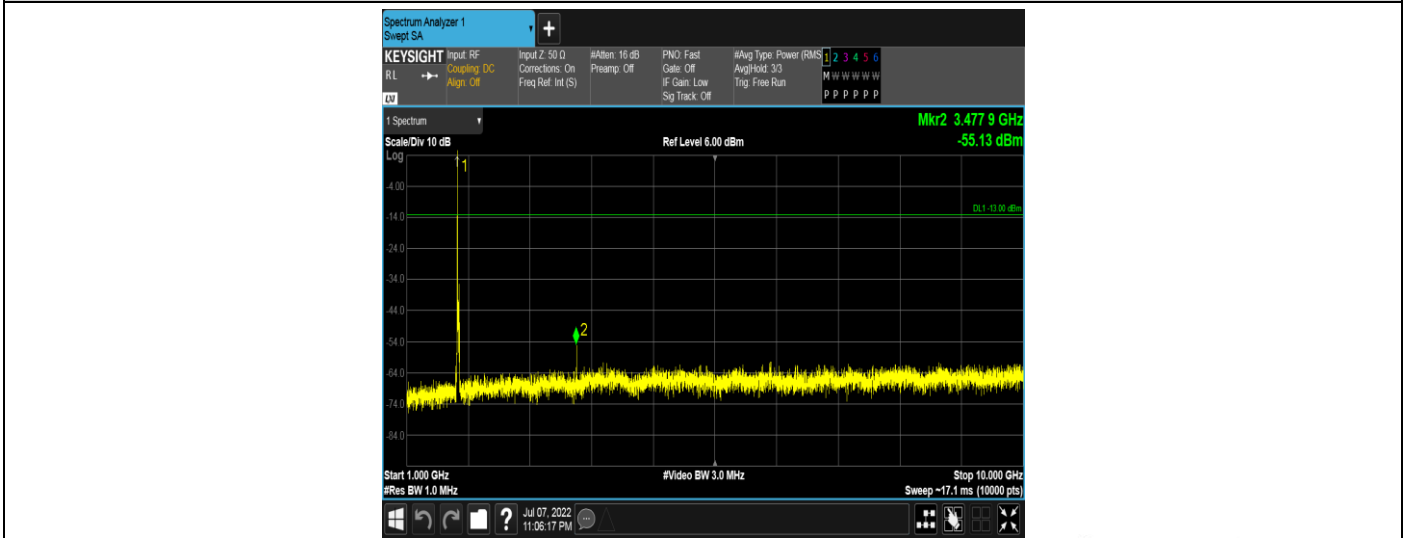
Band66-15MHz-QPSK-132322-1RB#0-Range3:1000~10000MHz
