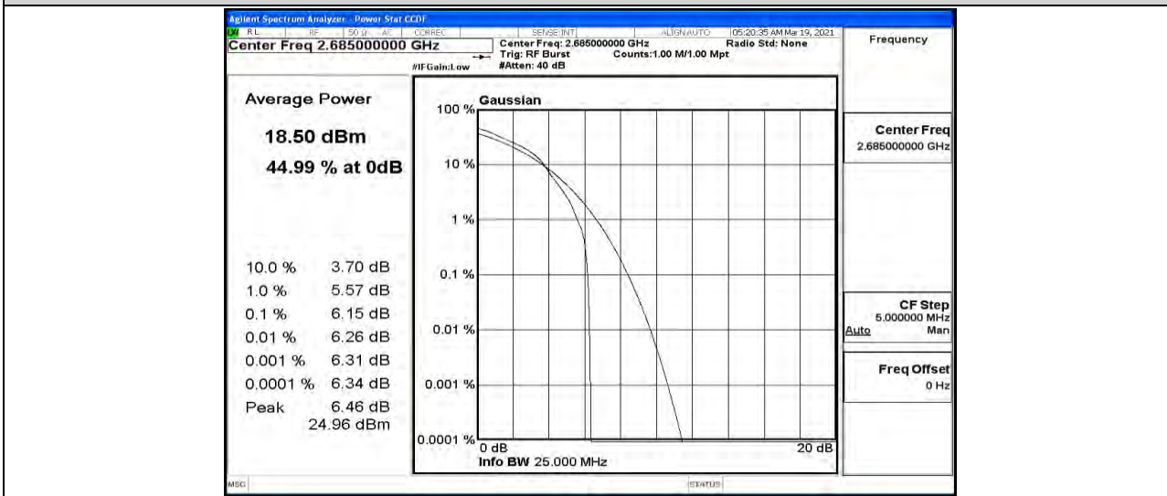
Band41-10MHz-16QAM-41540-50RB#0
