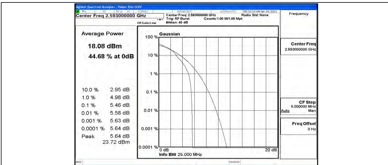
Band41-20MHz-16QAM-40620-100RB#0
