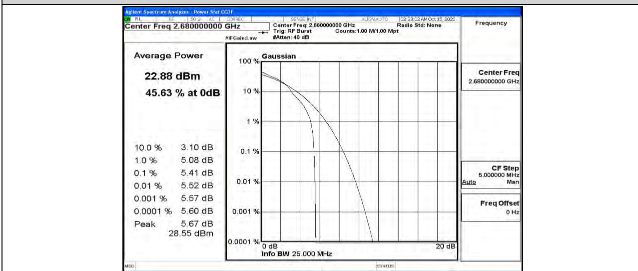
Band41-20MHz-16QAM-41490-100RB#0
