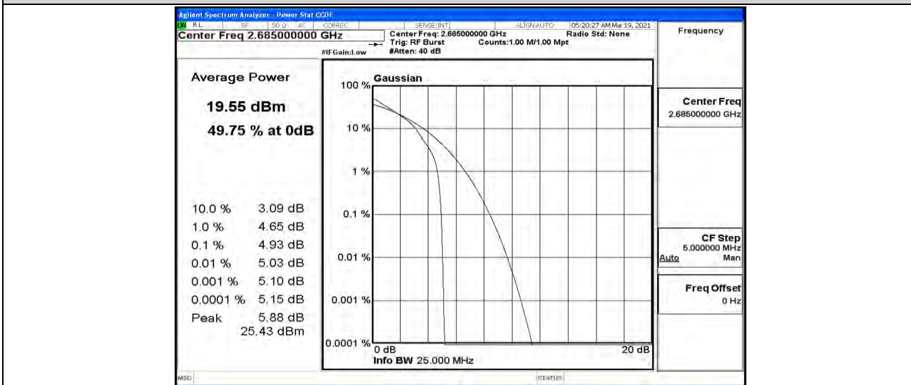
Band41-10MHz-QPSK-41540-50RB#0
