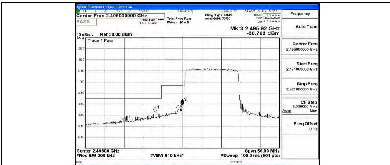
Band41-15MHz-16QAM-41515-75RB#0
