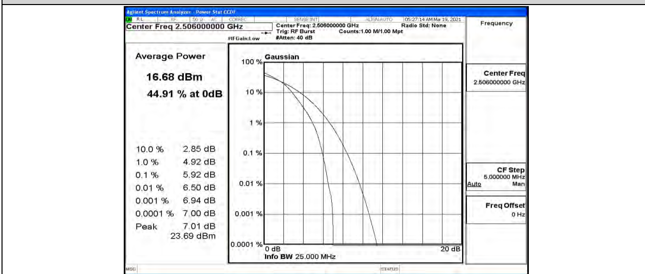
Band41-20MHz-QPSK-40620-1RB#0
