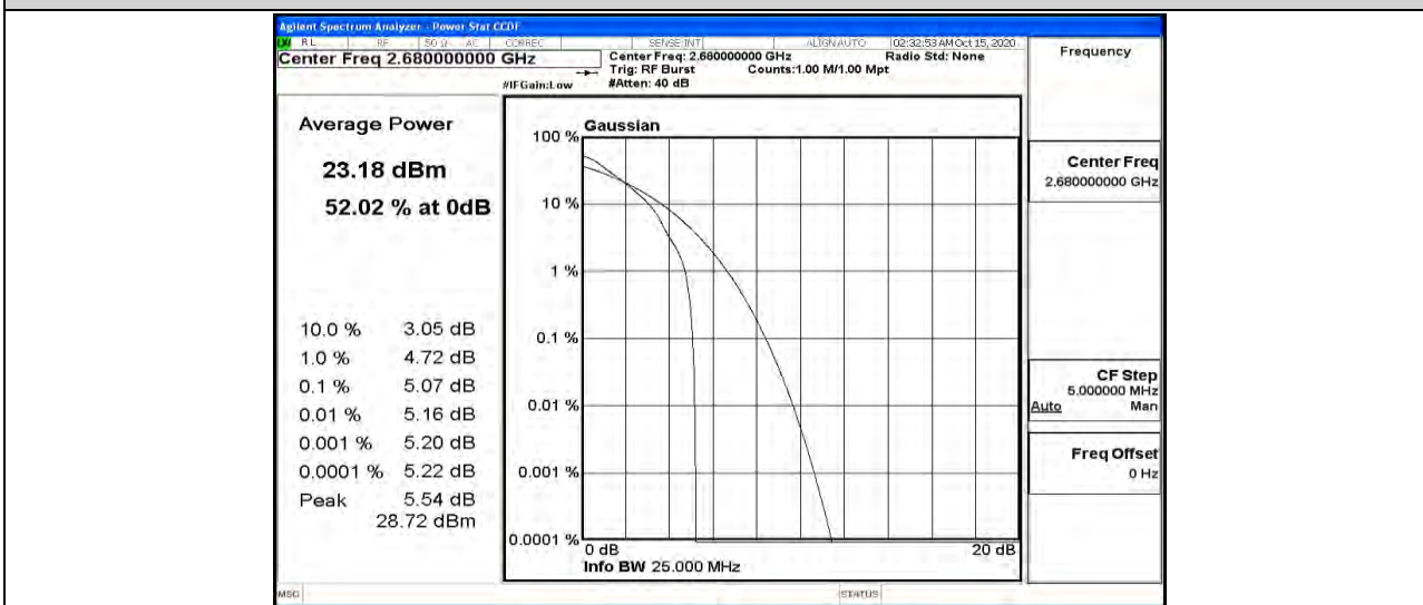
Band41-20MHz-QPSK-41490-100RB#0
