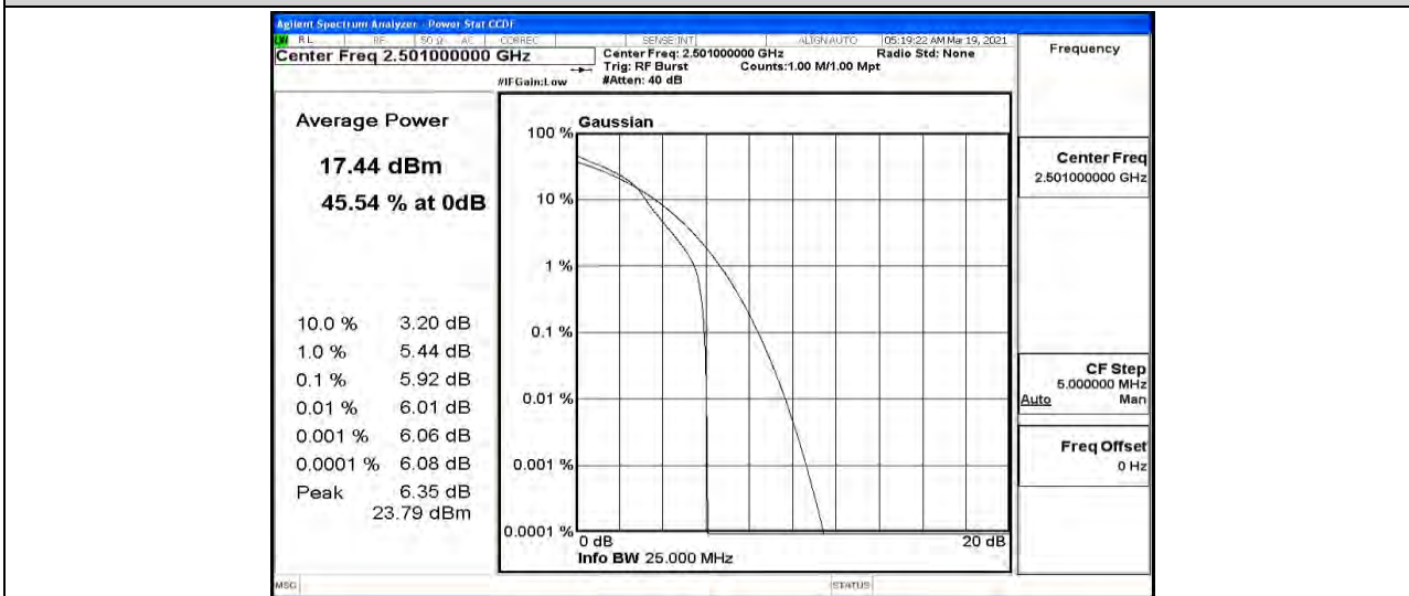
Band41-10MHz-16QAM-39700-50RB#0
