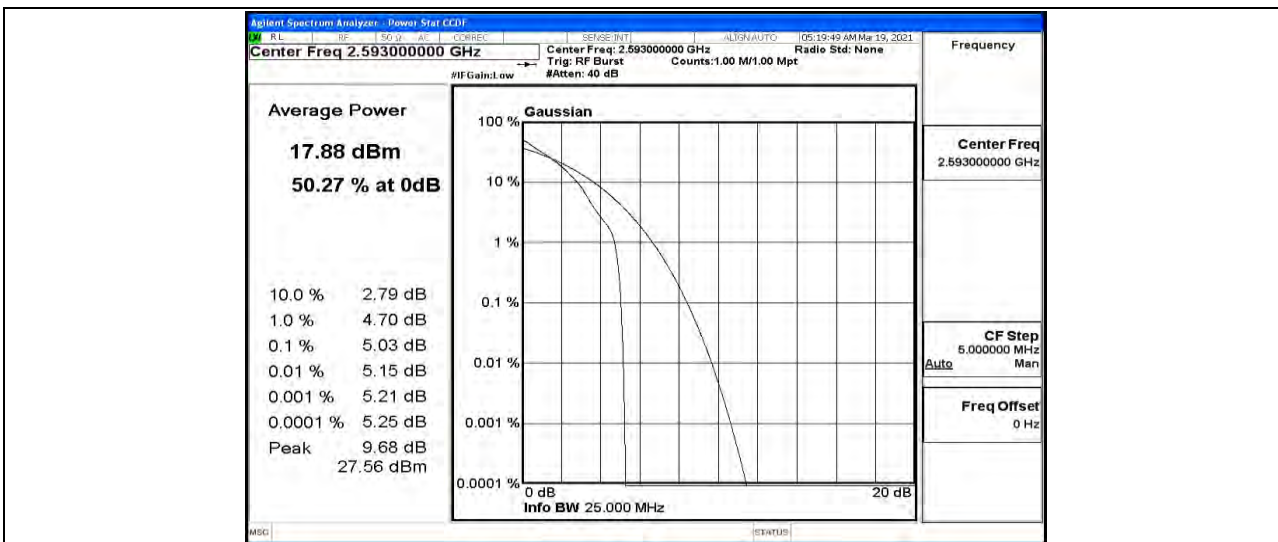
Band41-10MHz-QPSK-40620-50RB#0
