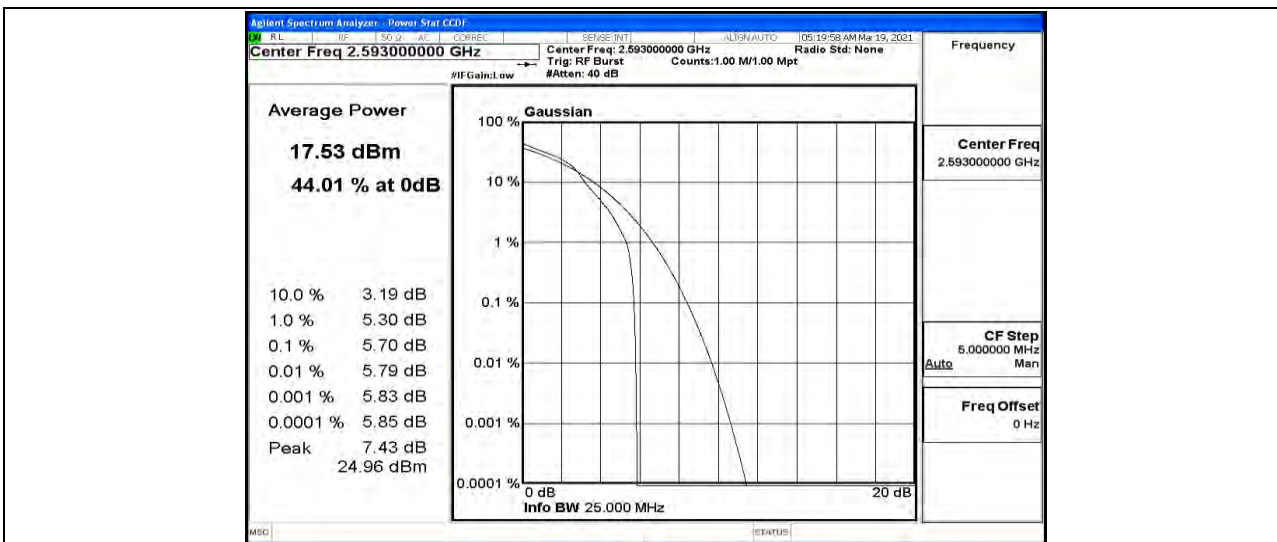
Band41-10MHz-16QAM-40620-50RB#0
