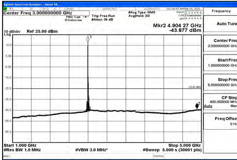
15MHz-QPSK-M-1RB#0-Range5:5000~12000MHz
