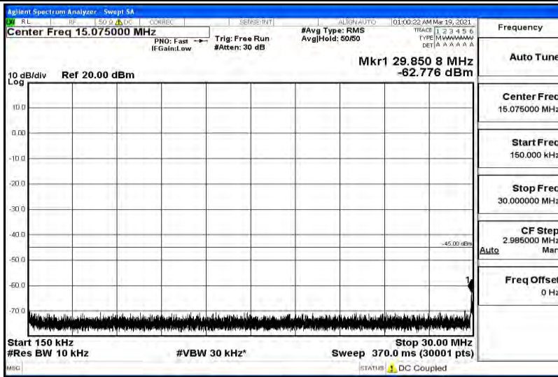
20MHz-QPSK-M-1RB#0-Range3:30~1000MHz
