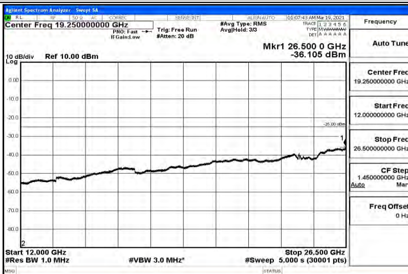
20MHz-16QAM-H-1RB#0-Range6:12000~26500MHz
