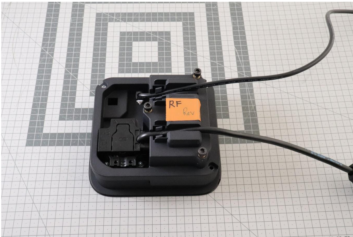
Photograph 3. The EUT
