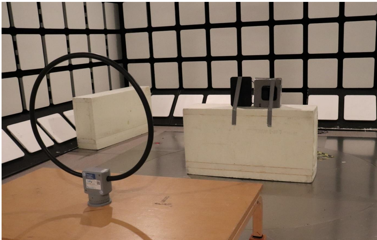
Photograph 4. Radiated Emissions 0.009 - 30 MHz
