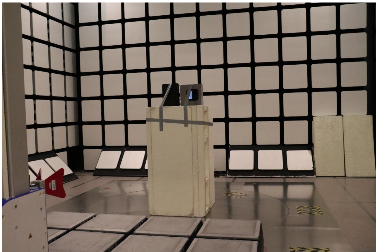
Photograph 6. Radiated Emissions 1 – 18 GHz
