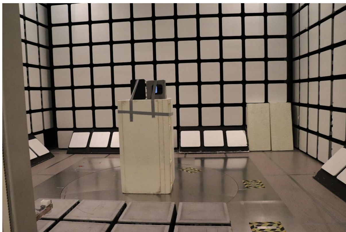
Photograph 7. Radiated Emissions 18 – 26.5 GHz
