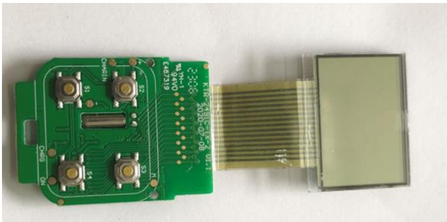
PCB view for all models
