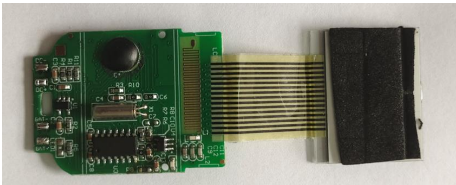
PCB view for all models
