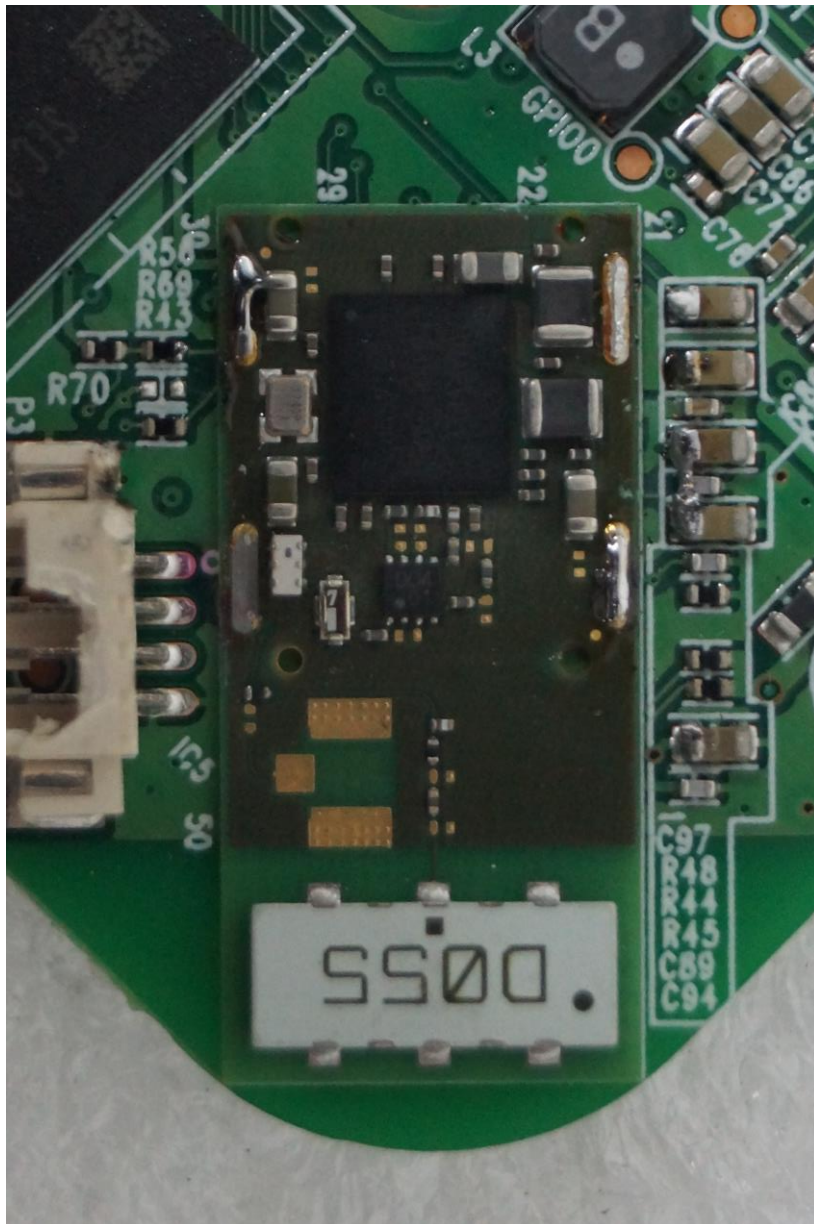
< RF module inside view >
