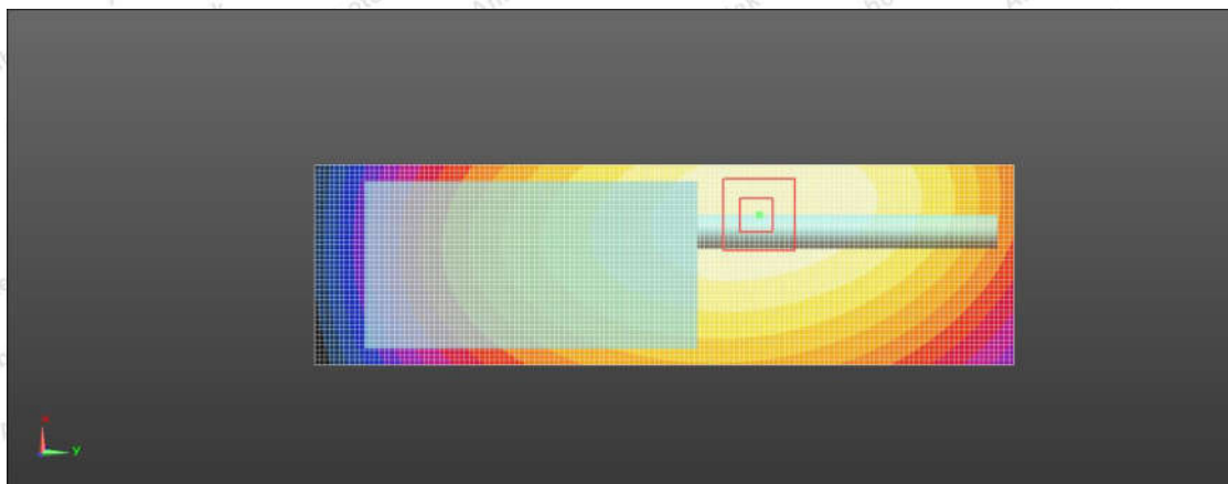
Figure 34: PMR_FM12.5KHz_Body Worn_0mm
