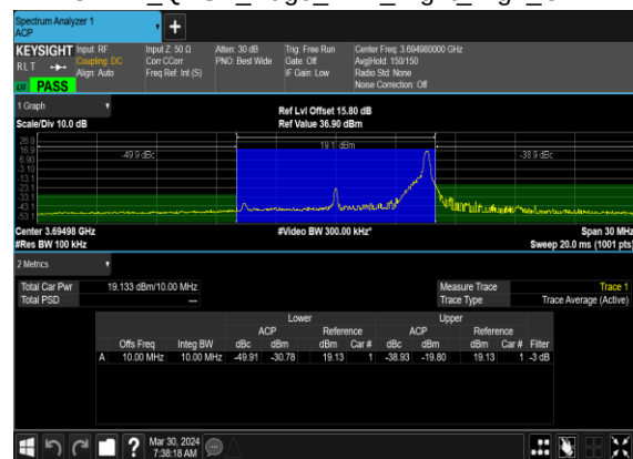
N48(10M)_DFT-s- OFDM_QPSK_Edge_1RB_Right_High_CH
