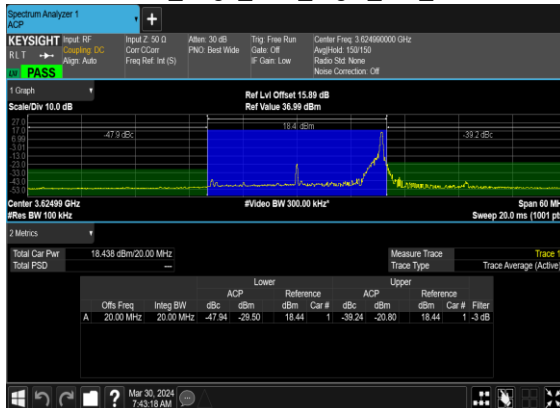
N48(20M)_DFT-s-OFDM_PI_2- BPSK_Edge_1RB_Right_Mid_CH
