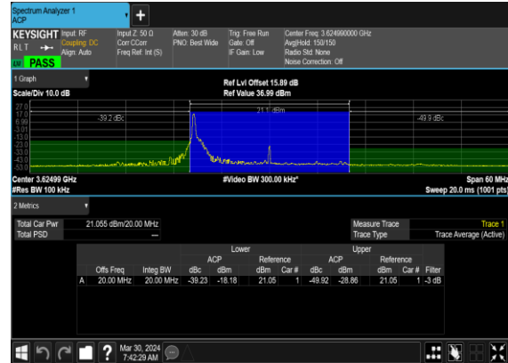
N48(20M)_DFT-s-OFDM_PI_2- BPSK_Edge_1RB_Left_Mid_CH
