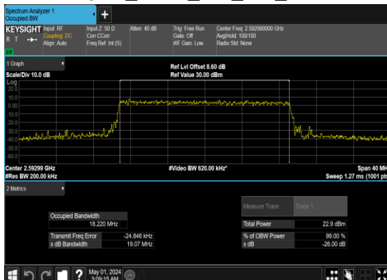
B2_N41(20M)_CP-OFDM_256 QAM_Outer_Full_Mid_CH
