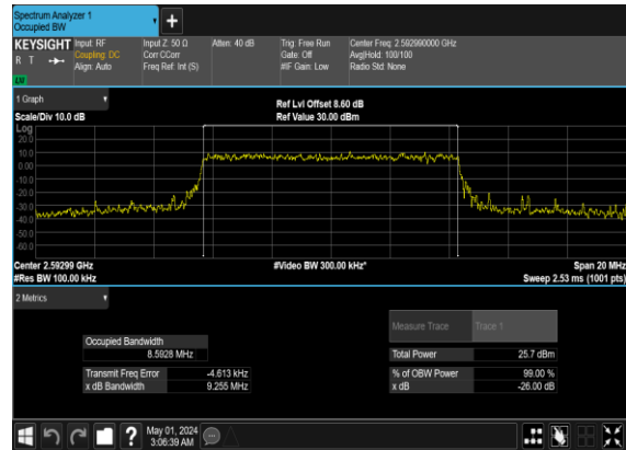
B2_N41(10M)_CP-OFDM_16 QAM_Outer_Full_Mid_CH
