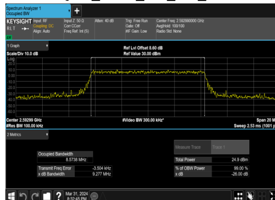
N41(10M)_CP-OFDM_256 QAM_Outer_Full_Mid_CH
