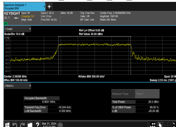
N41(10M)_CP-OFDM_16 QAM_Outer_Full_Mid_CH
