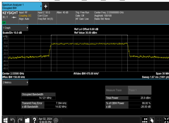
N7(15M)_CP-OFDM_64 QAM_Outer_Full_Mid_CH
