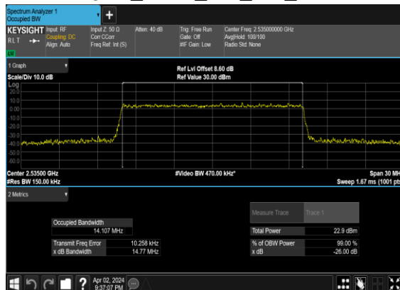
N7(15M)_CP-OFDM_256 QAM_Outer_Full_Mid_CH
