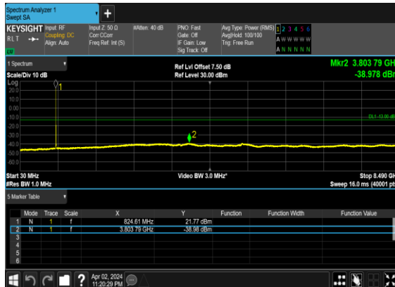
OFDM_BPSK_Edge_1RB_Left_Low_CH
