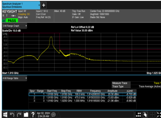
N25(45M)_DFT-s- OFDM_BPSK_Edge_1RB_Right_High_CH
