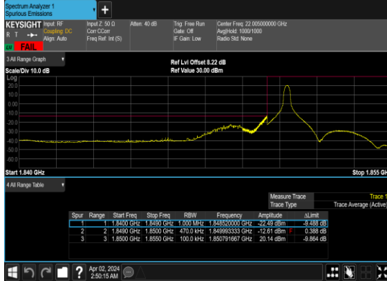
N25(45M)_DFT-s- OFDM_QPSK_Edge_1RB_Left_Low_CH
