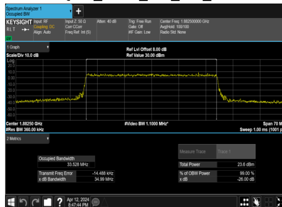
B66_N25(35M)_CP-OFDM_256 QAM_Outer_Full_Mid_CH
