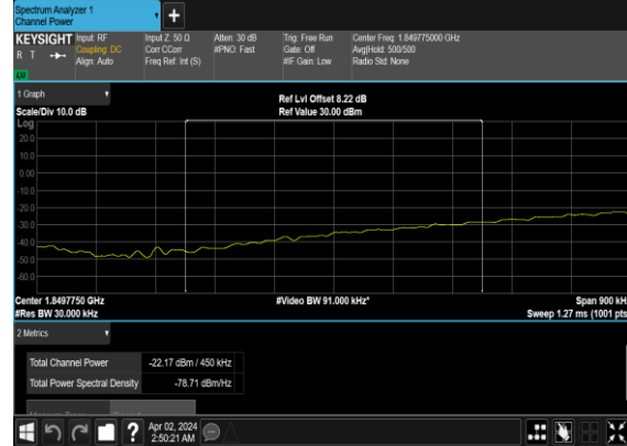
N25(45M)_DFT-s- OFDM_QPSK_Edge_1RB_Left_Low_CH_chp_PASS
