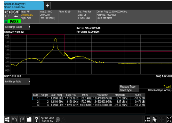
N25(45M)_DFT-s- OFDM_QPSK_Edge_1RB_Right_High_CH
