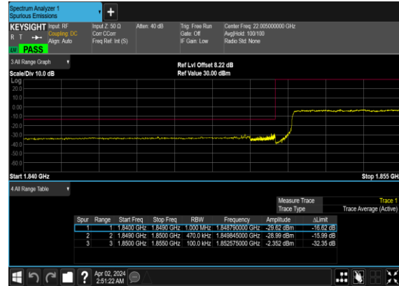
N25(45M)_DFT-s- OFDM_QPSK_Outer_Full_Low_CH
