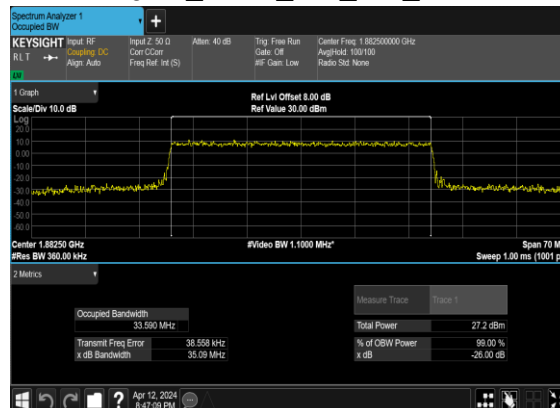
B66_N25(35M)_CP-OFDM_16 QAM_Outer_Full_Mid_CH
