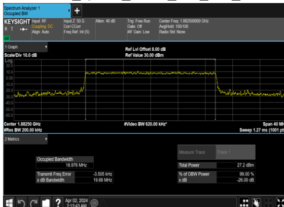
N25(20M)_CP- OFDM_QPSK_Outer_Full_Mid_CH
