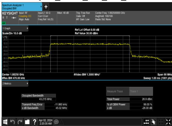
N25(45M)_CP-OFDM_16 QAM_Outer_Full_Mid_CH
