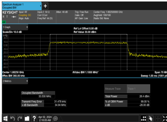
N25(35M)_CP-OFDM_64 QAM_Outer_Full_Mid_CH
