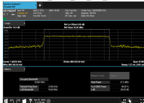
N25(20M)_CP-OFDM_16 QAM_Outer_Full_Mid_CH
