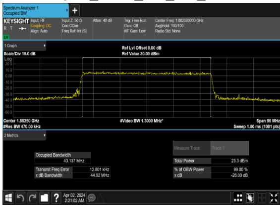
N25(45M)_CP-OFDM_256 QAM_Outer_Full_Mid_CH
