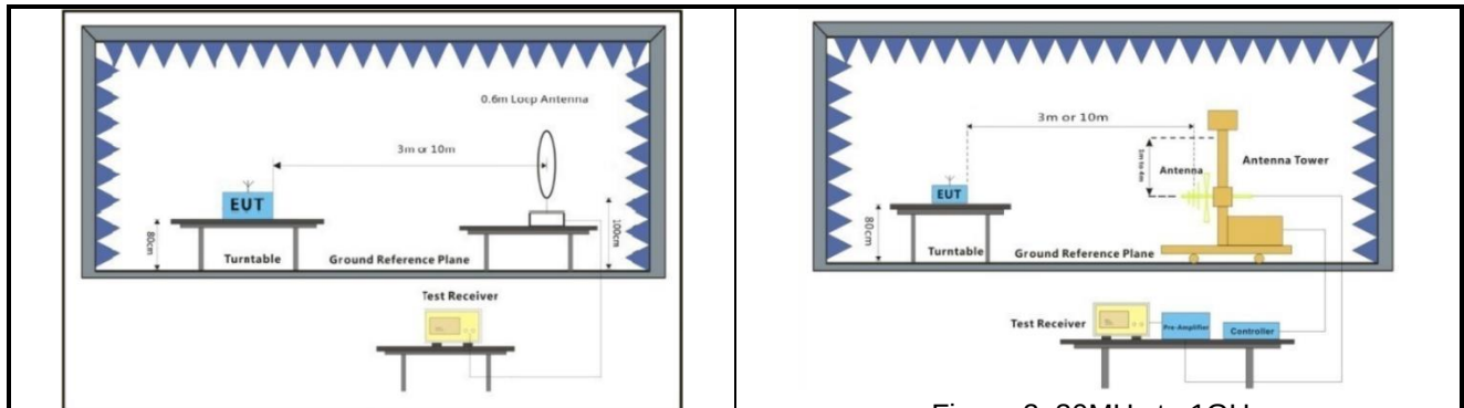
Figure 2. 30MHz to 1GHz
