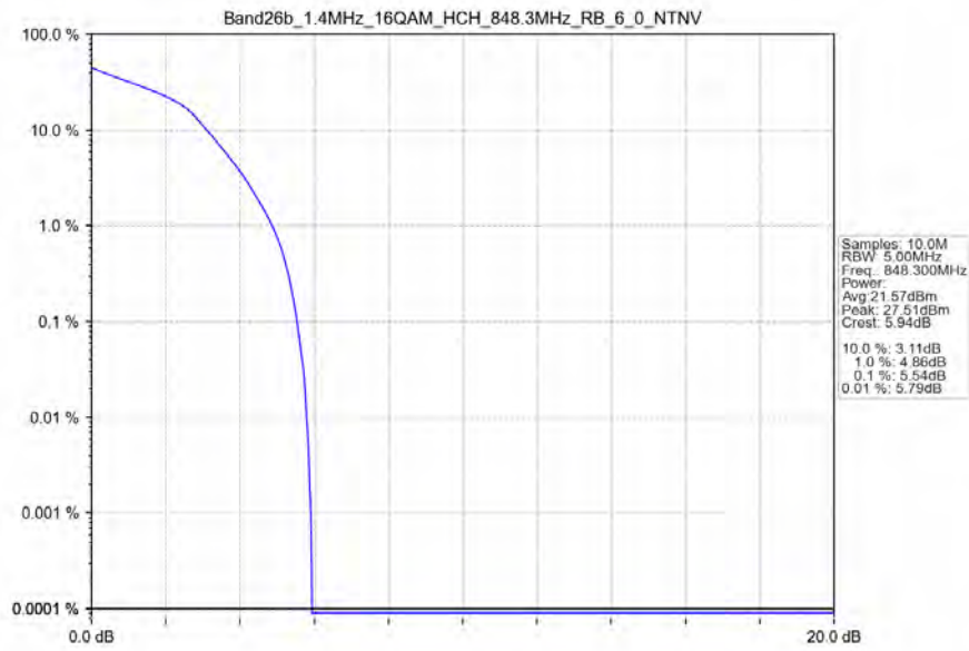
Band26b_1.4MHz_16QAM_HCH_848.3MHz_RB_6_0_NTNV
