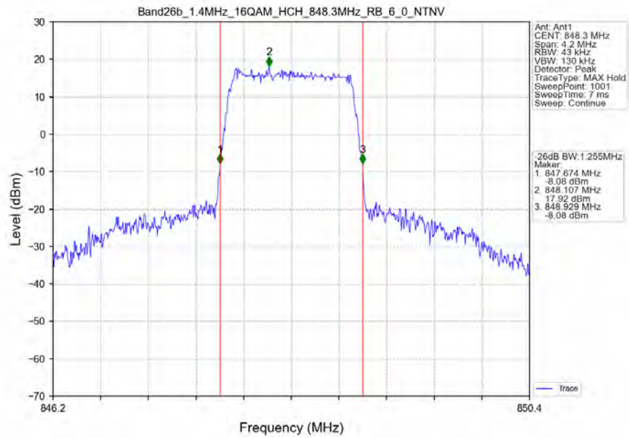
Band26b 1.4MHz 16QAM HCH 848.3MHz RB 6 0 NTV
