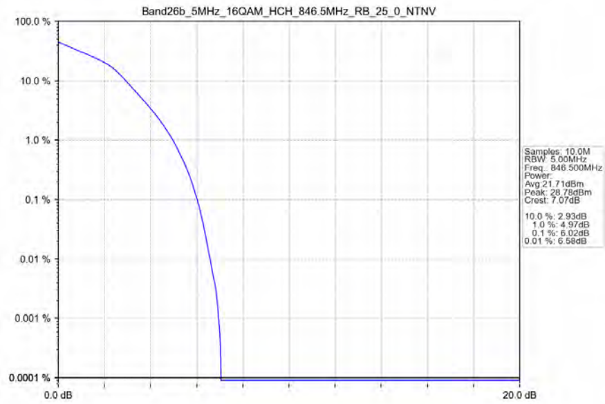
Band26b_5MHz_16QAM_HCH_846.5MHz_RB_25_0_NTNV
