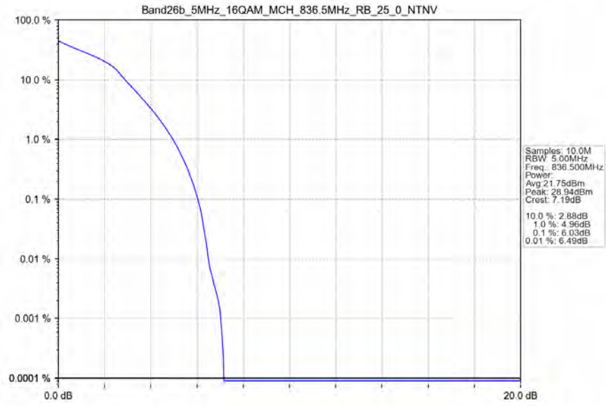
Band26b_5MHz_16QAM_MCH_836.5MHz_RB_25_0_NTNV
