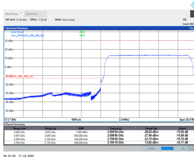
1-N77-3700-3980-PC2-30-10-L-3-DFT-PI2BPSK-Outer_Full-24@0-Ant0-1--PASS-see graph
