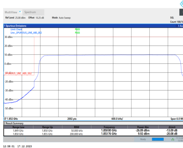
1-N2-PC3-15-5-L-3-DFT-PI2BPSK-Outer_Full-25@0-Ant0-1-seegraph-PASS-see graph
