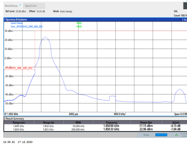
1-N2-PC3-15-5-L-1-DFT-PI2BPSK-Edge_1RB_Left-1@0-Ant0-1-seegraph-PASS-see graph
