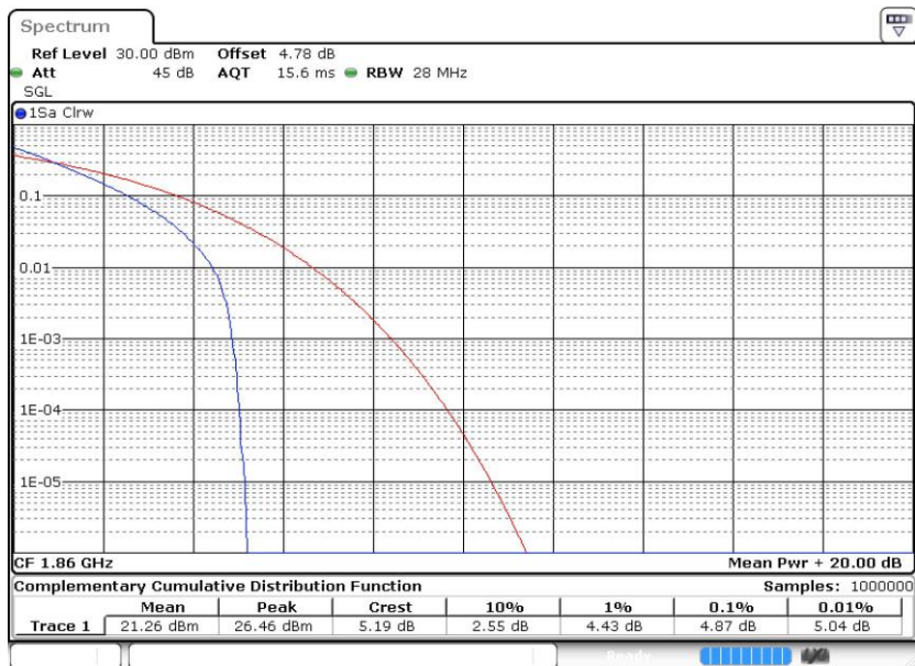
Band25-20MHz-QPSK-26140-100RB#0
