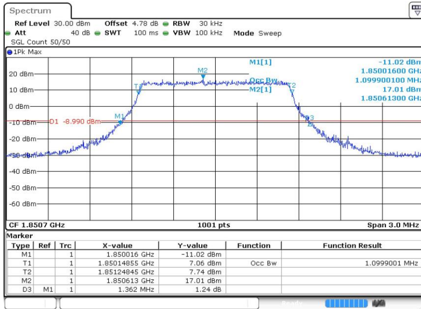
Band25-1.4MHz-QPSK-26047-6RB#0
