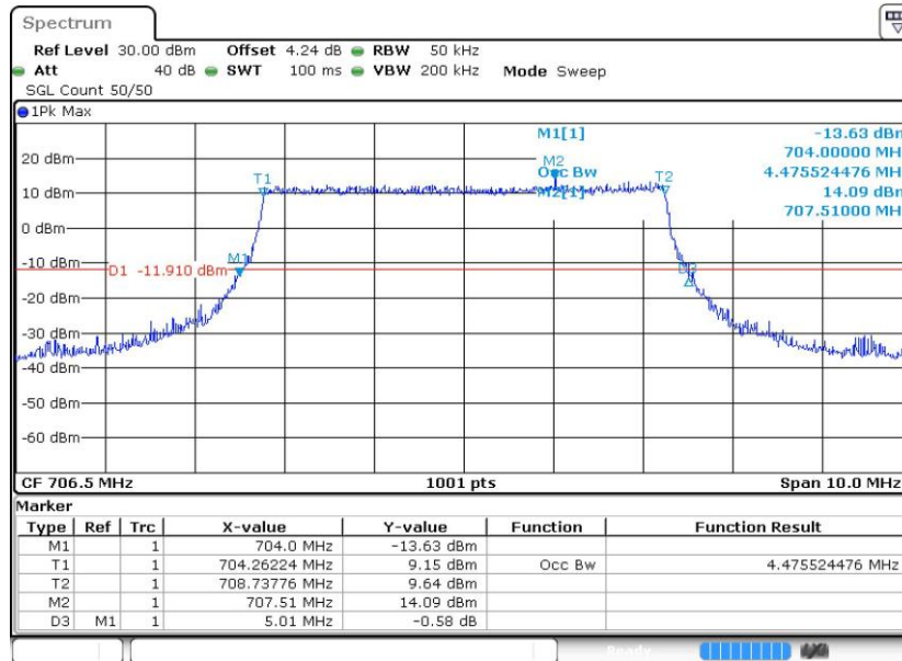
Band17-5MHz-QPSK-23755-25RB#0
