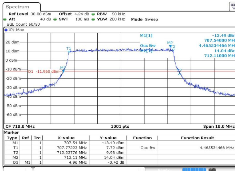
Band17-5MHz-QPSK-23790-25RB#0
