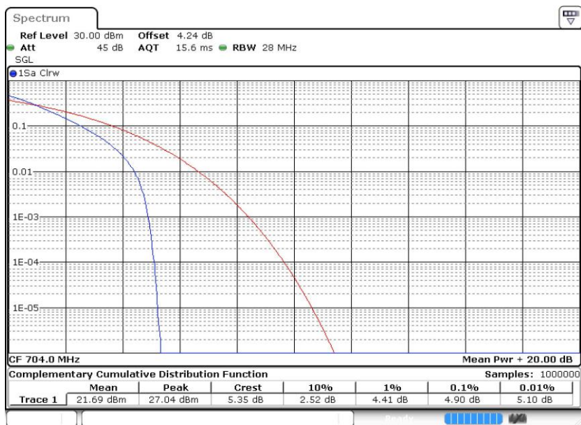
Band12-10MHz-QPSK-23060-50RB#0
