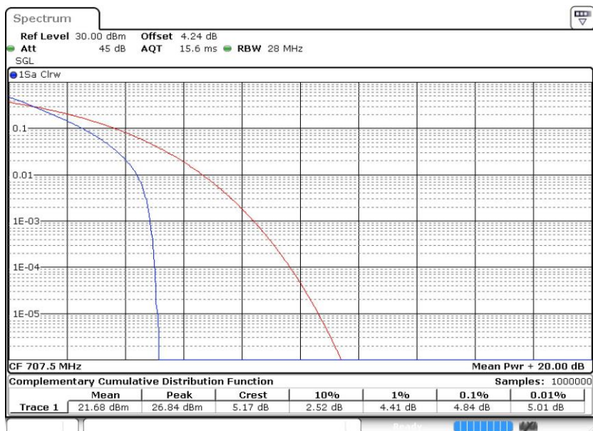
Band12-10MHz-QPSK-23095-50RB#0
