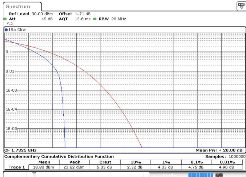
Band4-20MHz-QPSK-20175-100RB#0
