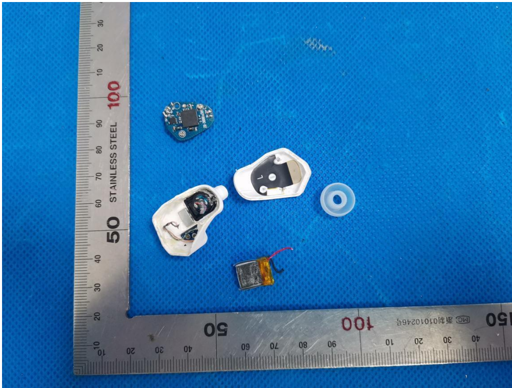
Left earphone OPEN VIEW OF EUT
