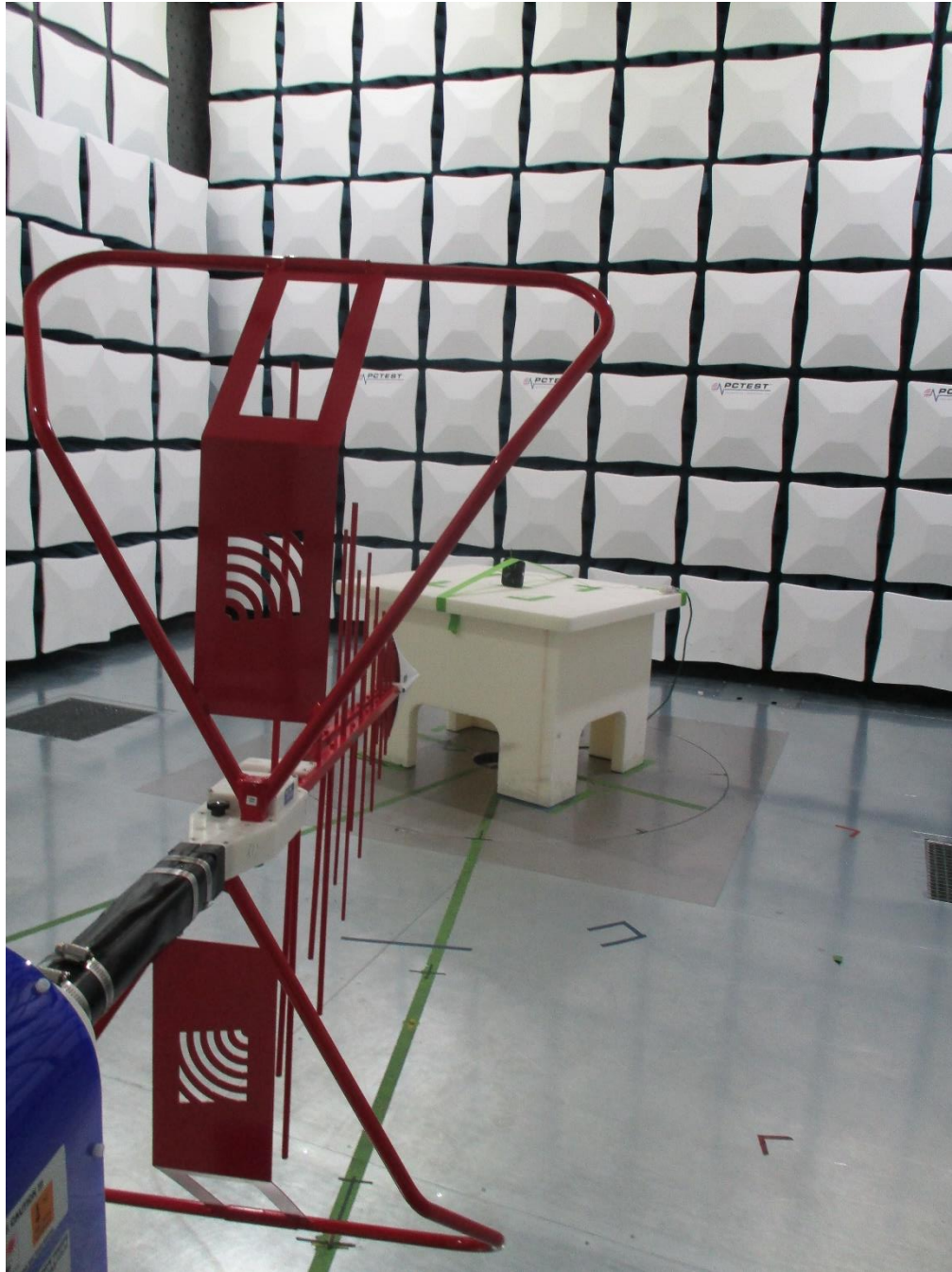
Figure 5: 30MHz-1GHz Test Setup (Front View)
