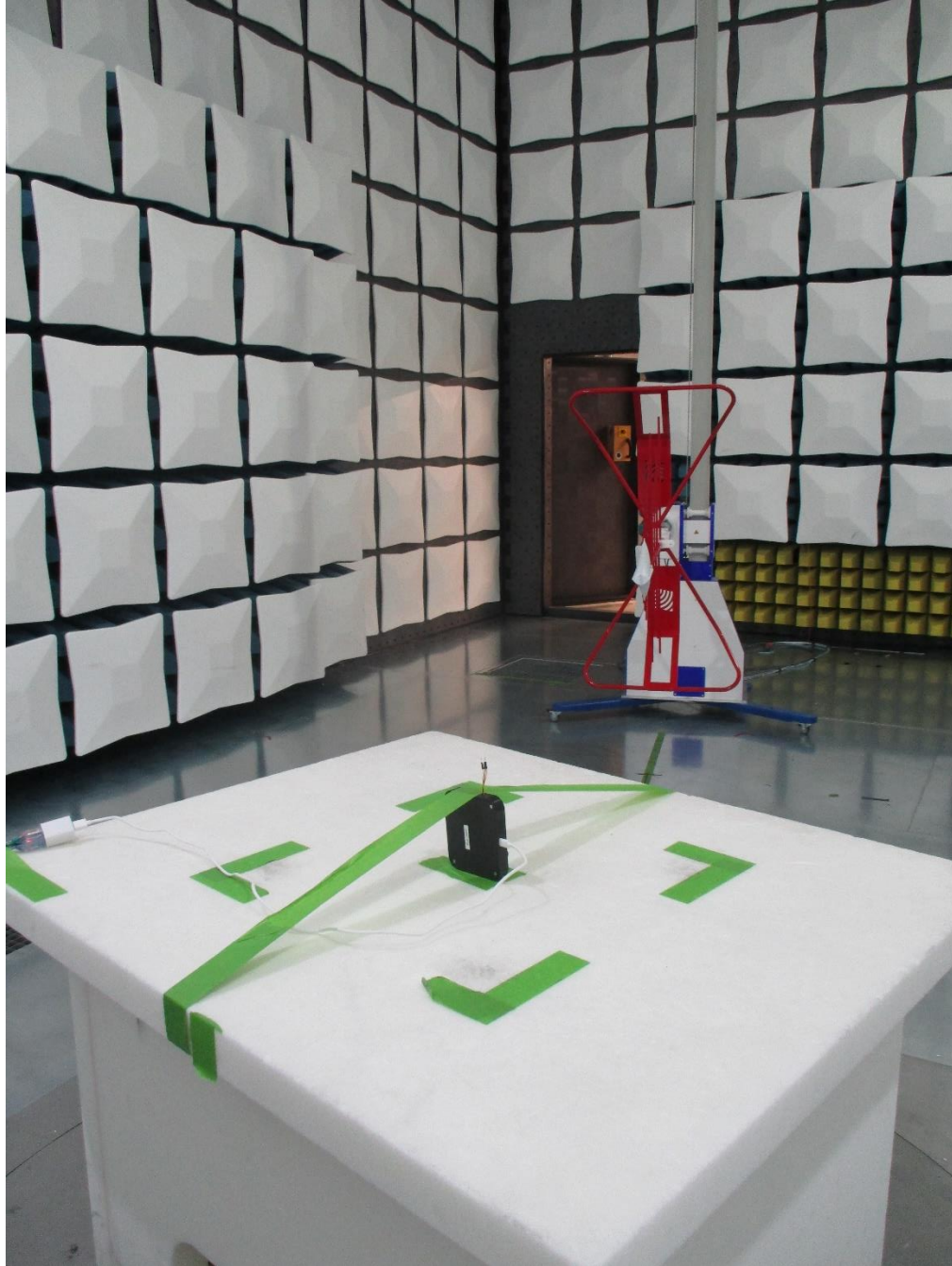
Figure 6: 30MHz-1GHz Test Setup (Rear View)
