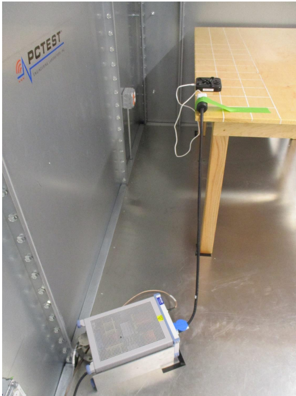
Figure 2: AC Line Conducted Emissions (Side View)
