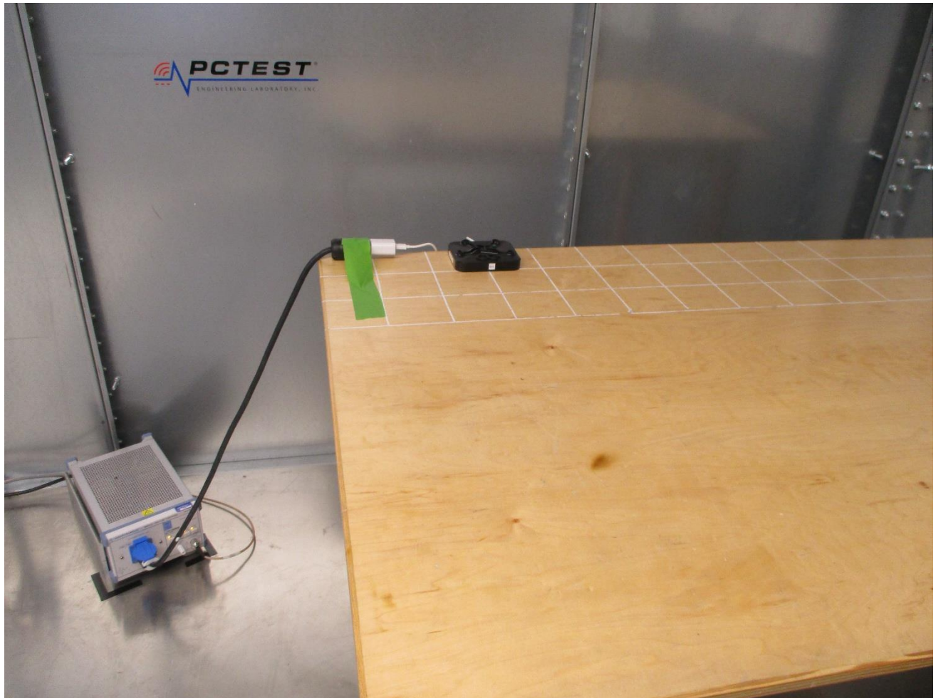
Figure 1: AC Line Conducted Emissions (Front View)
