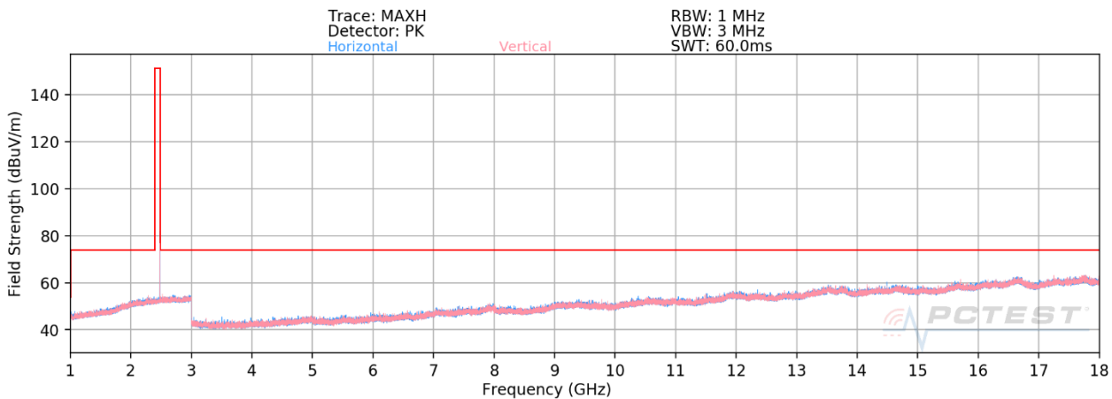
Plot 7-17. Radiated Spurious Emissions Pre-Scan 1-18GHz (1Mbps Ch. 39)
