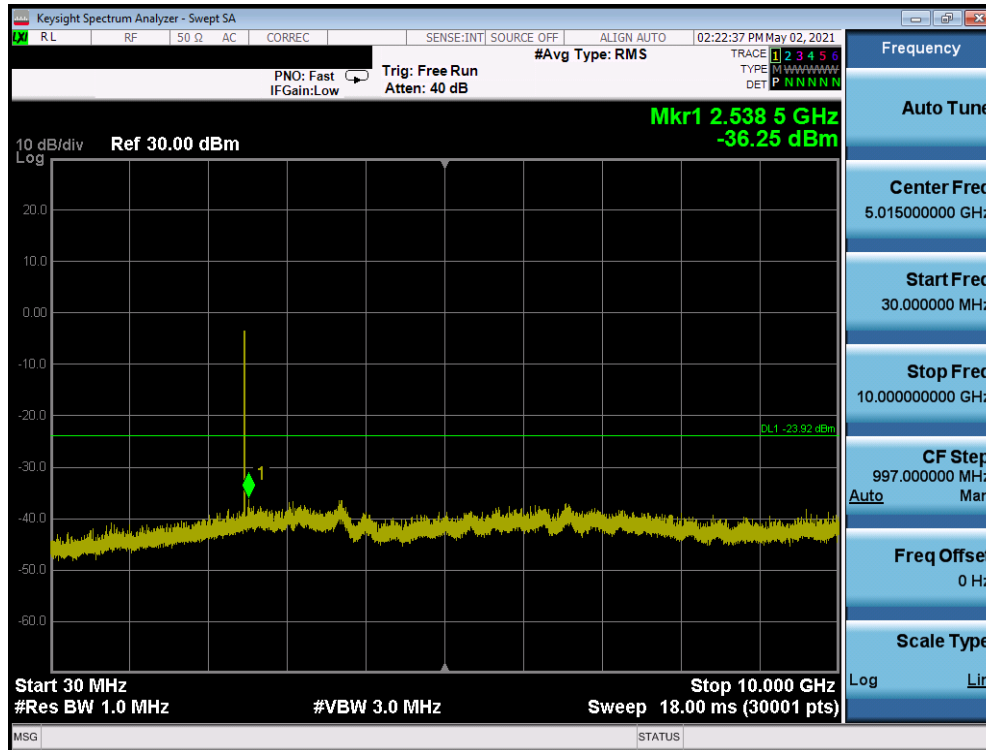
Plot 7-13. Conducted Spurious Plot (Bluetooth (LE), 1Mbps, Ch. 39)
