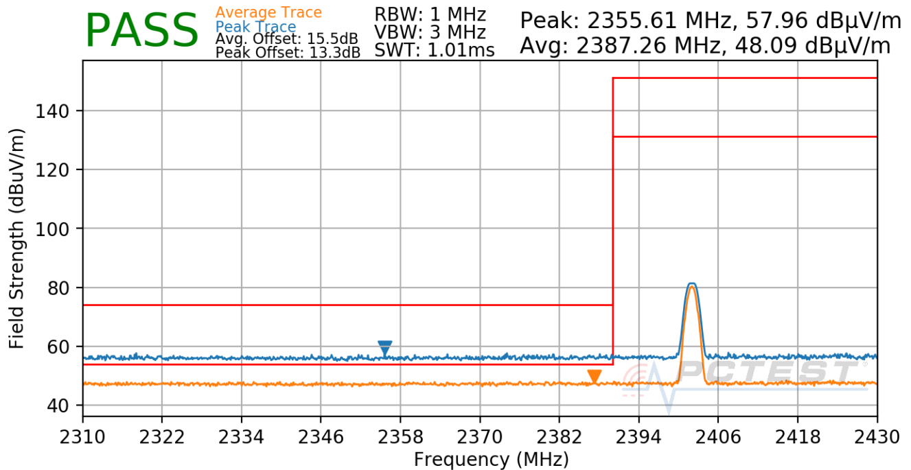
Plot 7-20. Radiated Restricted Lower Band Edge Measurement (1Mbps, Ch.0)
