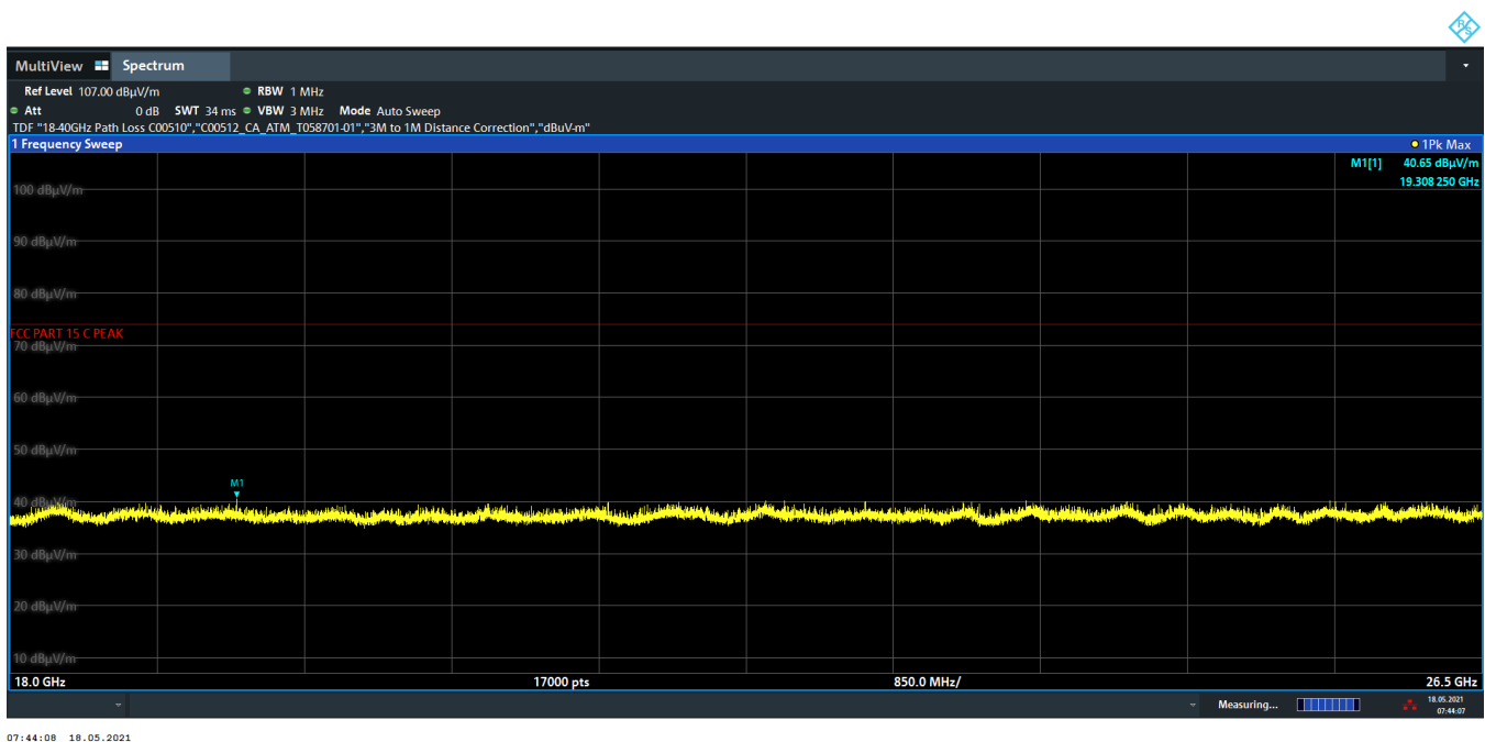
Plot 7-19. Radiated Spurious Pre-Scan Above 18GHz (1Mbps, Ch.19, Pol. V)
