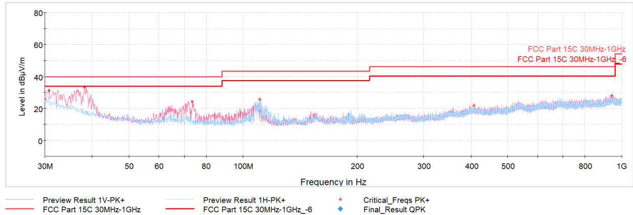
Plot 7-22. Radiated Spurious Emissions Pre-Scan 30MHz-1GHz (1Mbps, Ch.19, with AC/DC Adapter)
