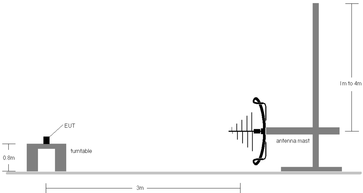
Figure 7-8. Radiated Test Setup < 1GHz
