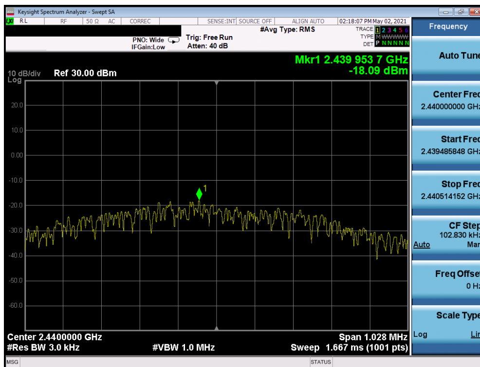
Plot 7-5. Power Spectral Density Plot (Bluetooth (LE), 1Mbps, Ch. 19)
