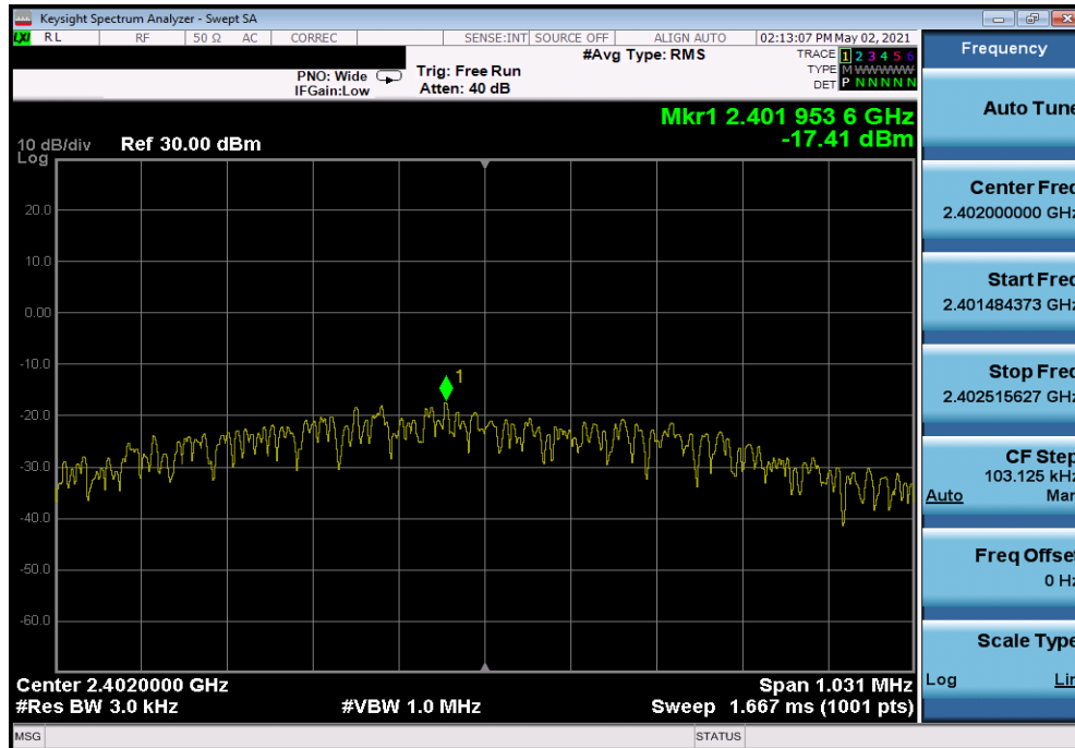
Plot 7-4. Power Spectral Density Plot (Bluetooth (LE), 1Mbps, Ch. 0)
