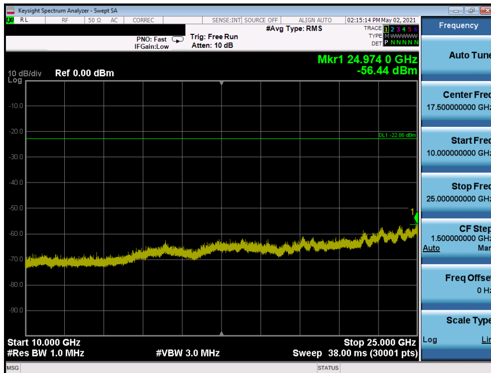
Plot 7-10. Conducted Spurious Plot (Bluetooth (LE), 1Mbps, Ch. 0)
