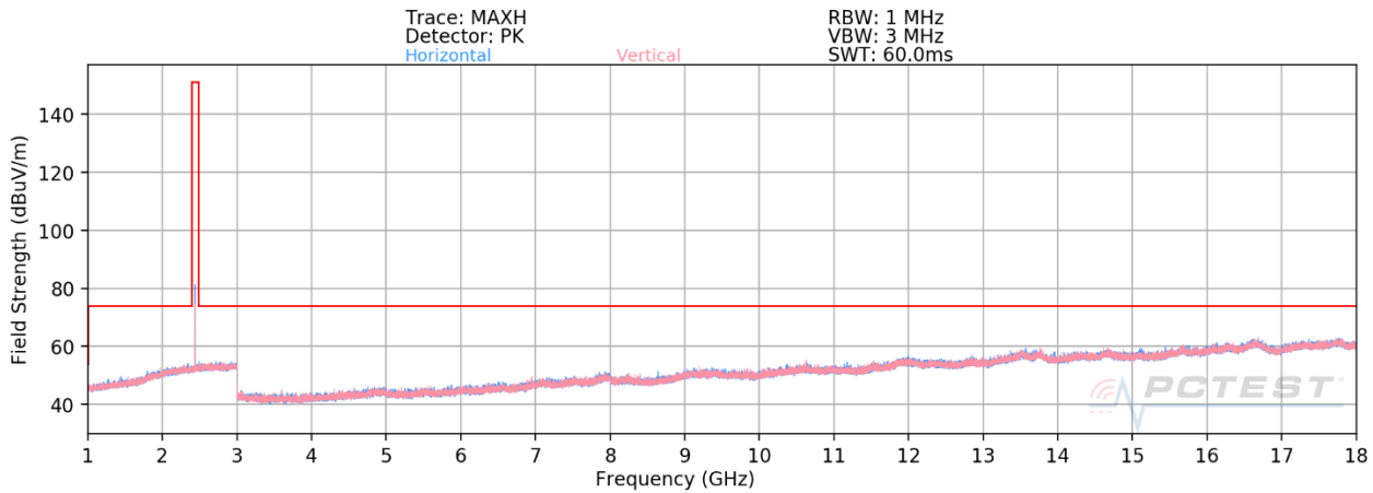
Plot 7-16. Radiated Spurious Emissions Pre-Scan 1-18GHz (1Mbps, Ch. 19)
