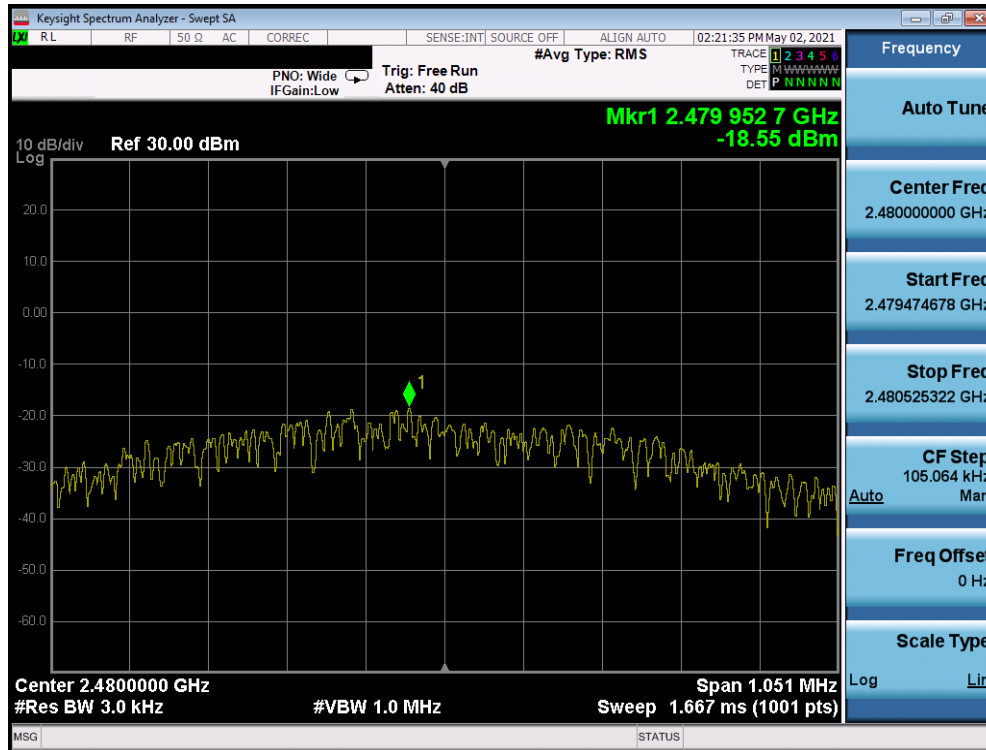
Plot 7-6. Power Spectral Density Plot (Bluetooth (LE), 1Mbps, Ch. 39)
