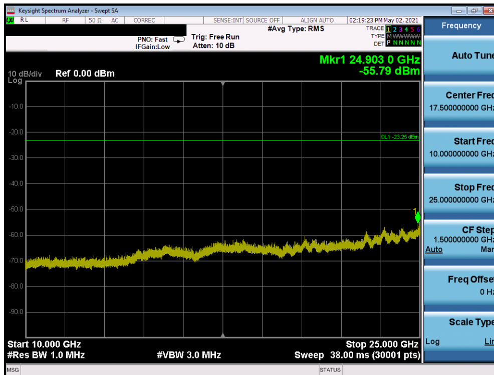
Plot 7-12. Conducted Spurious Plot (Bluetooth (LE), 1Mbps, Ch. 19)
