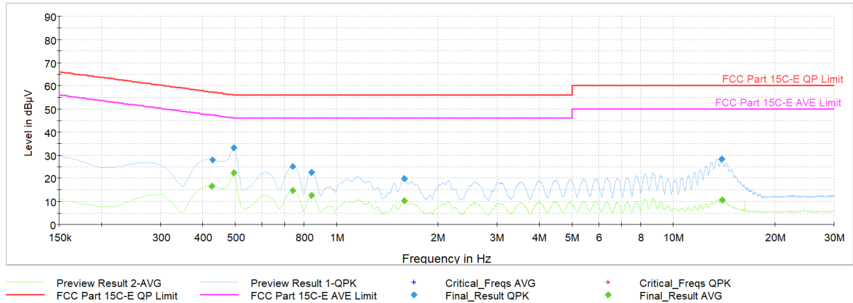
Plot 7-23. AC Line Conducted Plot with Bluetooth LE (L1 - 1Mbps, Ch.19, with AC/DC adapter)
