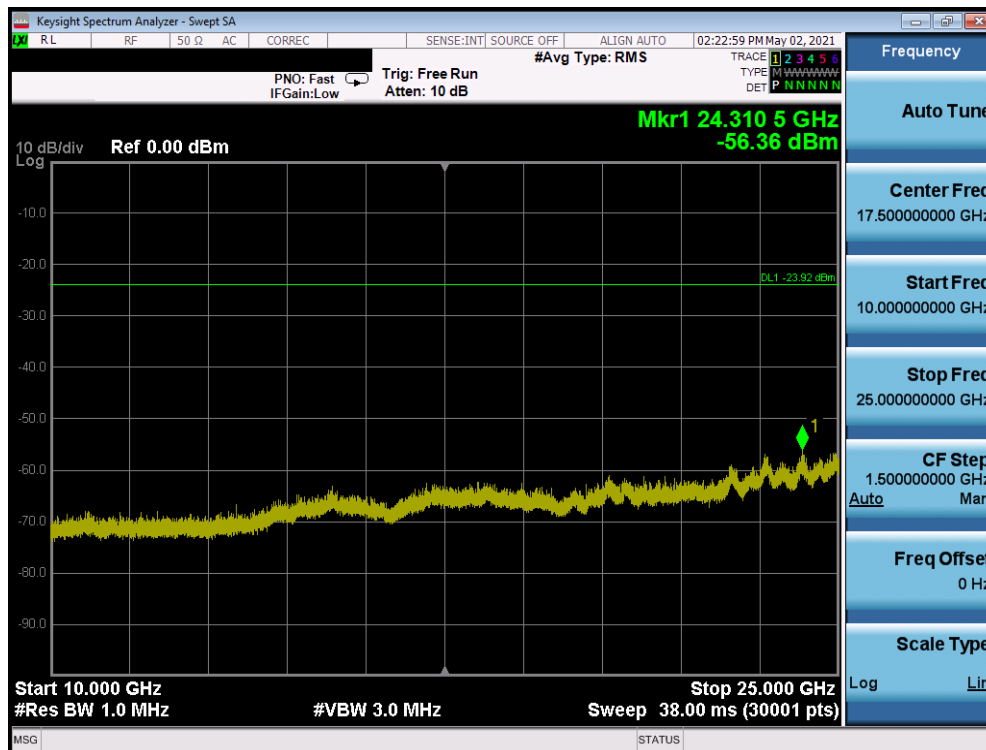
Plot 7-14. Conducted Spurious Plot (Bluetooth (LE), 1Mbps, Ch. 39)
