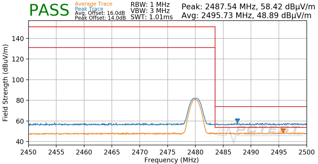
Plot 7-21. Radiated Restricted Upper Band Edge Measurement (1Mbps, Ch.39)
