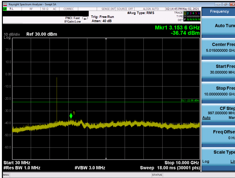
Plot 7-9. Conducted Spurious Plot (Bluetooth (LE), 1Mbps, Ch. 0)
