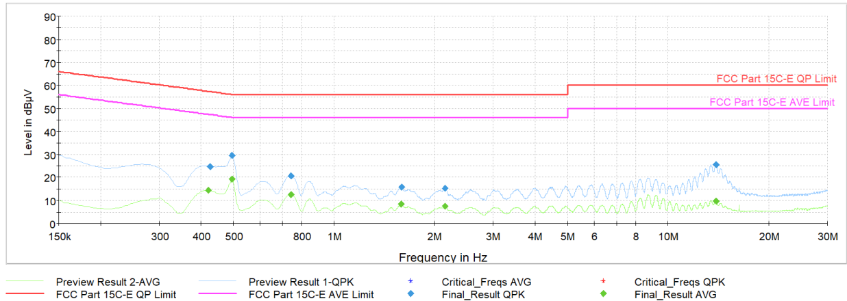
Plot 7-24. AC Line Conducted Plot with Bluetooth LE (N - 1Mbps, Ch.19, with AC/DC adapter)
