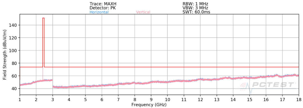
Plot 7-15. Radiated Spurious Emissions Pre-Scan 1-18GHz (1Mbps, Ch. 0)
