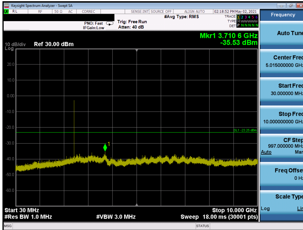
Plot 7-11. Conducted Spurious Plot (Bluetooth (LE), 1Mbps, Ch. 19)
