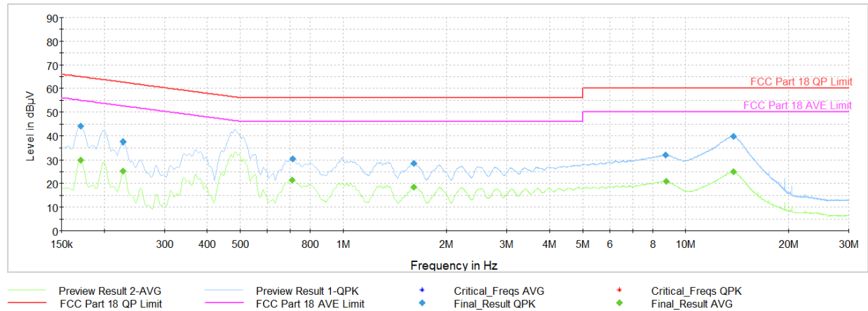
Plot 6-5 AC Line-Conducted Plot with WPT (L1, with AC/DC adapter)
